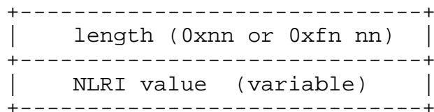
Figure 1: Flow-spec NLRI for IPv4
