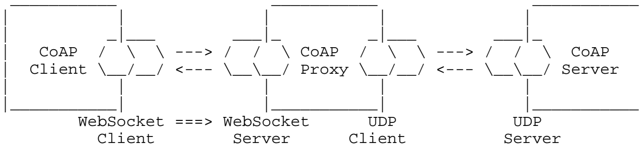
Figure 11: CoAP Client (WebSocket client) accesses CoAP Server (UDP server) via a CoAP proxy (WebSocket server/UDP client)
