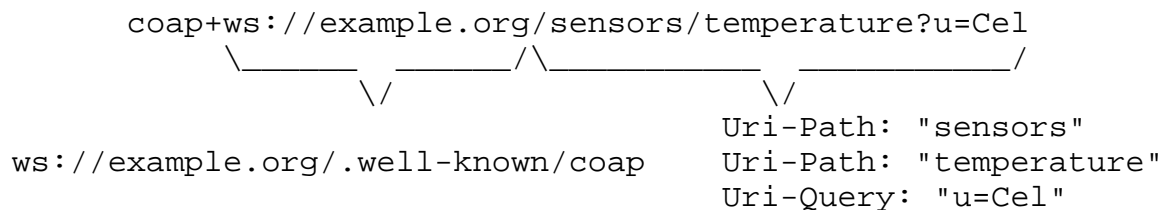
Figure 10: The "coap+ws" URI Scheme
