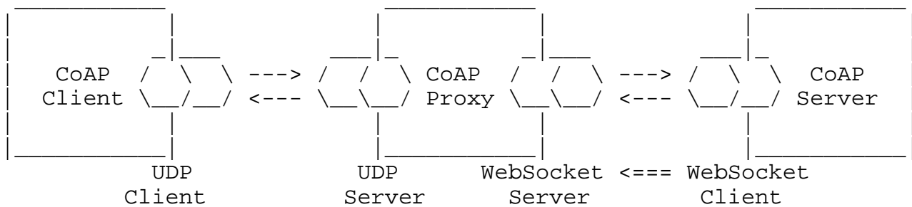
Figure 12: CoAP Client (UDP client) accesses sleepy CoAP Server (WebSocket client) via a CoAP proxy (UDP server/WebSocket server)
