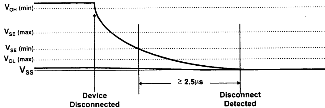
Figure 6-1: Disconnect Detection
