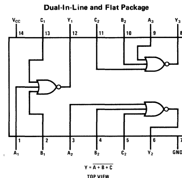
DM5427/DM7427
