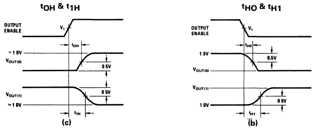
Waveform 52
