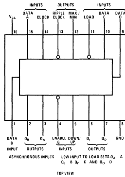
Dual-In-Line and Flat Package
