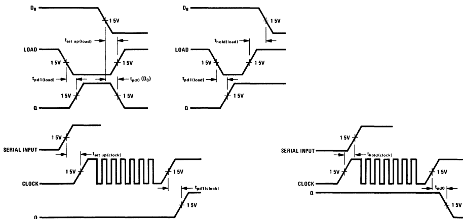
Waveform 30
