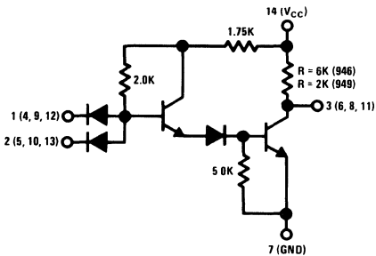
DM946/DM949
