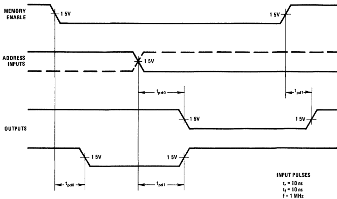
Waveform 13
