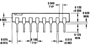
Package 5 16 Lead Molded DIP (N)
