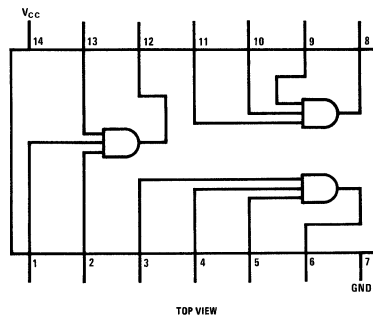
Dual-In-Line Package
