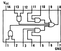
DM54H52/DM74H52 expandable 2-2-2-3-input AND-OR gate
