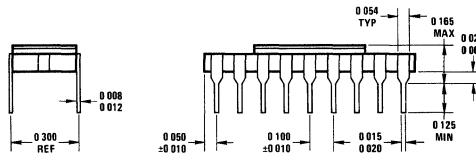
Package 12A 18 Lead Cavity DIP (J)
