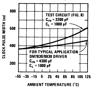
FIGURE 5. Typical Clock Pulse Variations vs Ambient Temperature
