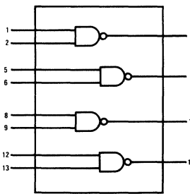
DM957/DM958
