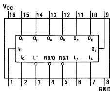
DM5448/DM7448
