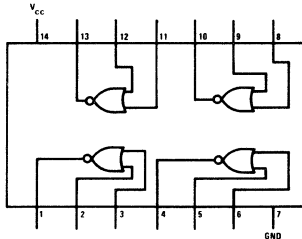
DM54L02/DM74L02
