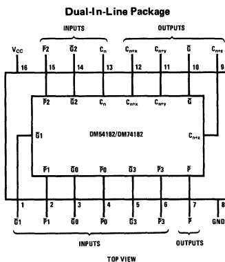
DM54182/DM74182 PIN DESIGNATIONS
