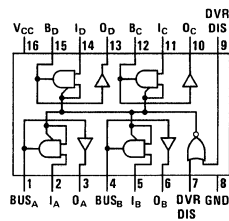
TOP VIEW DM7839/DM8839
