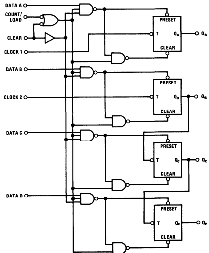
DM54197/DM74197
