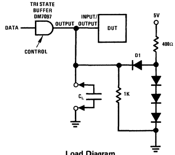
Load Diagram
