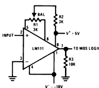
Zero Crossing Detector driving MOS logic
