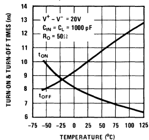
Turn-On & Turn-Off Time vs Temperature
