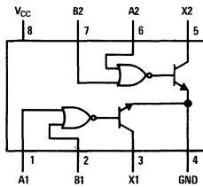
LM75463
