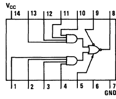
DM54H55/DM74H55 expandable 2-wide 4-input AND-OR-INVERT gate
