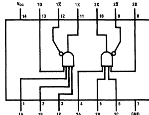
DM5460/DM7460
