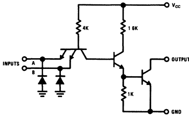
DM5401/DM7401, DM5403/DM7403
