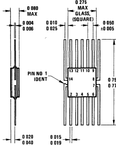
Package 15 14 Lead Flat Package (F)
