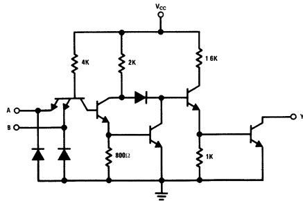
DM5409, DM7409
