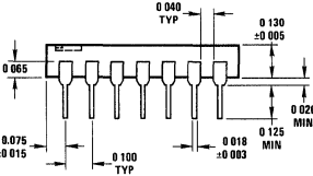
Package 3 14 Lead Molded DIP (N)
