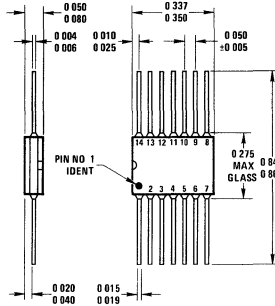
Package 18 14 Lead Flat Package (W)
