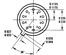
Package 22 10 Lead Metal Can Package (H) (Hybrids Only)
