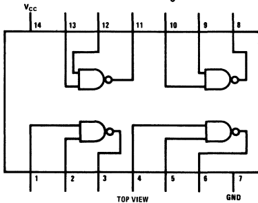
DM7810/DM8810
