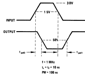
Waveform 4
