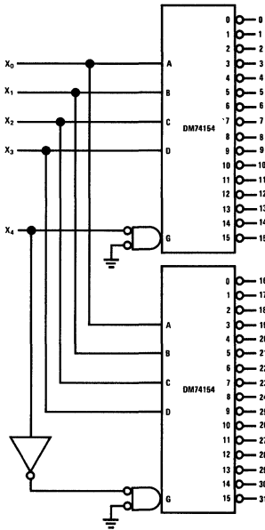
DM74154 Expanded to Perform 1 Out of 32 Decode Function
