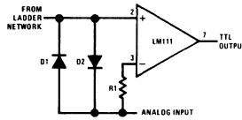
Using Clamp Diodes to Improve Response
