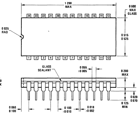
Package 13 24 Lead Cavity DIP (J)
