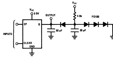
Test Circuit 22
