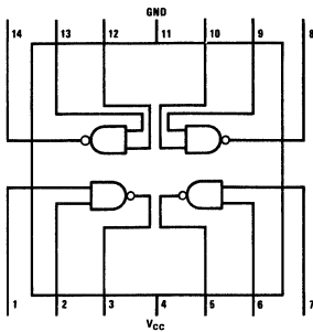
DM54L00/DM74L00 DM54L01/DM74L01
