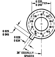
Package 21 10 Lead Metal Can Package (H)
