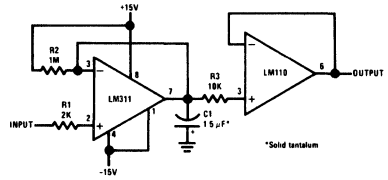
Negative Peak Detector *Solid tantalum
