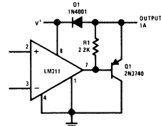
Comparator and Solenoid Driver
