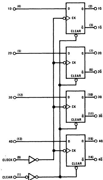
DM54175/DM74175
