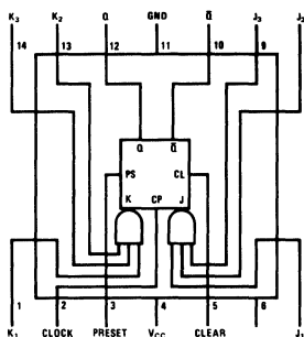
DM54L72/DM74L72
