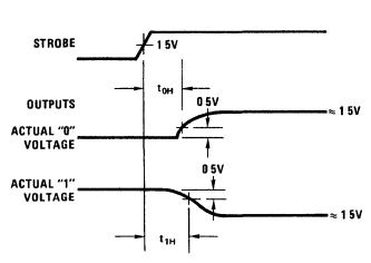
t_{0H} & t_{1H}
