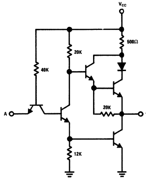
DM54L04/DM74L04
