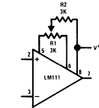
Offset Balancing
