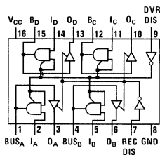
TOP VIEW DM7833/DM8833
