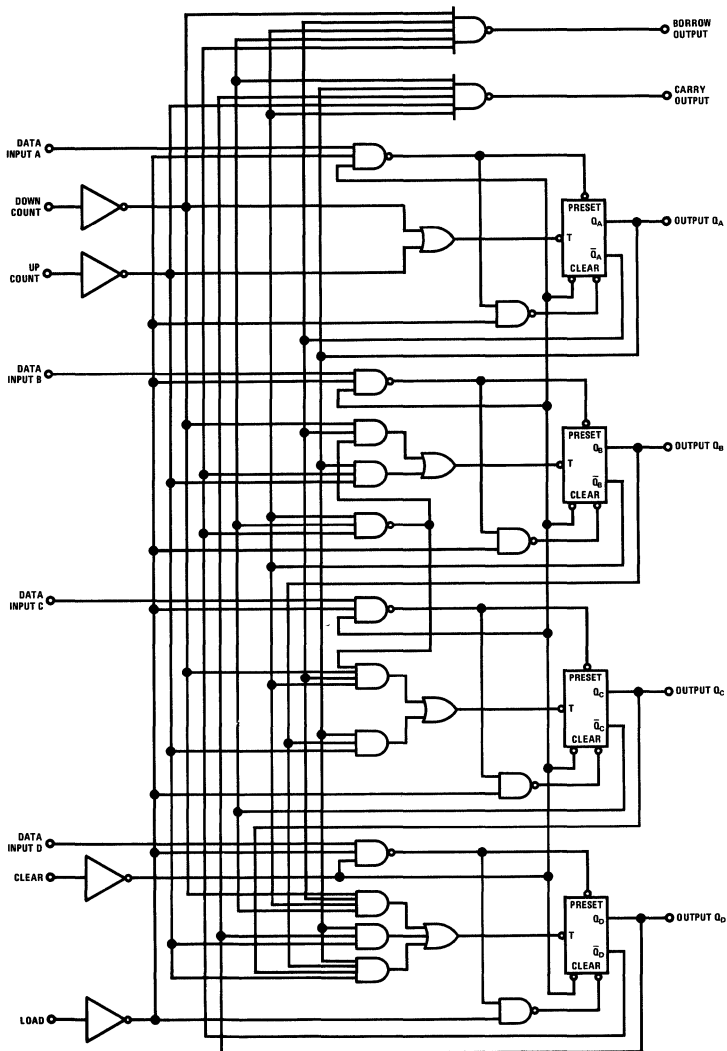
DM54L192/DM74L192
