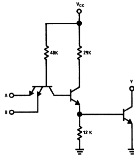
DM54L01/DM74L01 DM54L03/DM74L03
