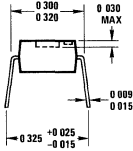
Package 1 8 Lead Molded Mini DIP (N)
