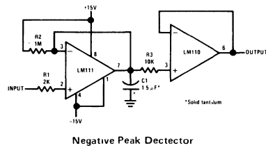
Negative Peak Detector
