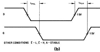
Waveform 47
