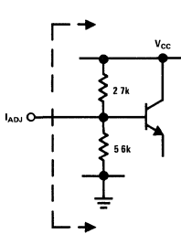
Test Circuit 17
