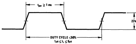
Programming Pulse
