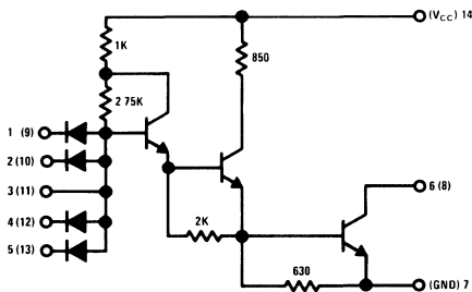
DM944
