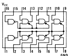
DM70L95/DM80L95
