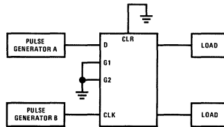
FIGURE 4. Use Waveforms D
