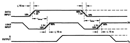
Voltage Waveforms 1
