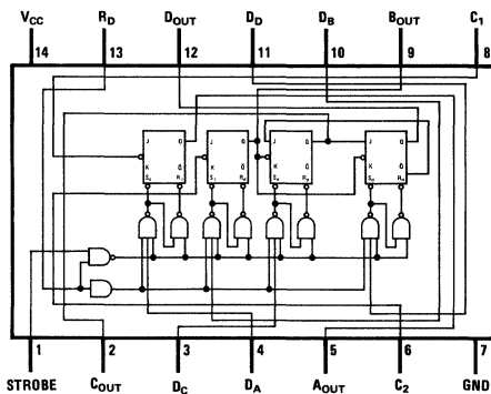
DM7288/DM8288
