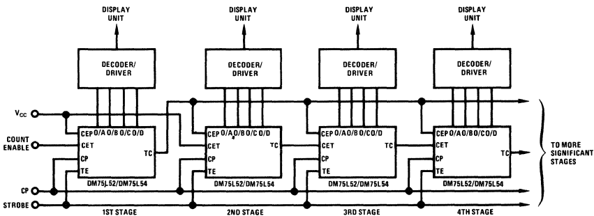
Multi-Stage Synchronous Counter with Visual Display
