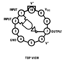
10 Pin TO-100 Package
