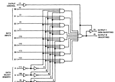
DM74S251
