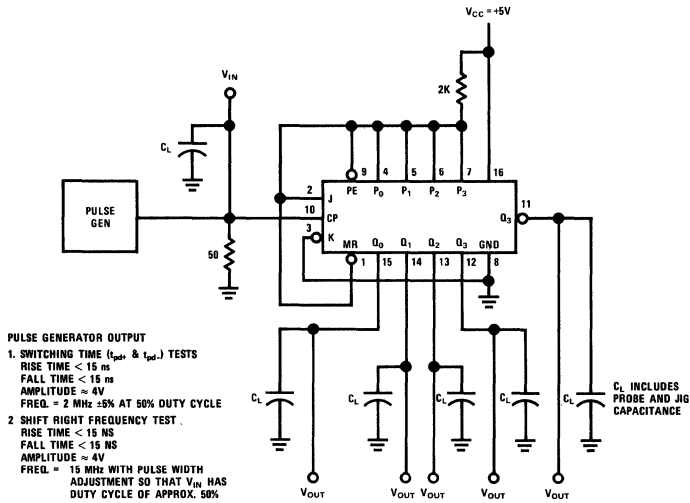
Test Circuit 9
