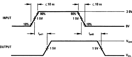
Waveform 3
