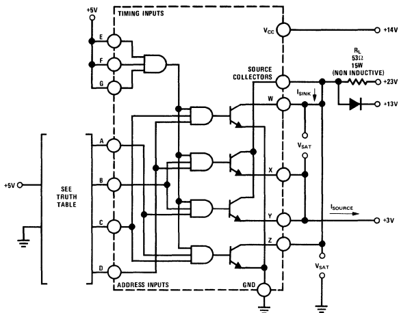
FIGURE 2. V_{SAT}
