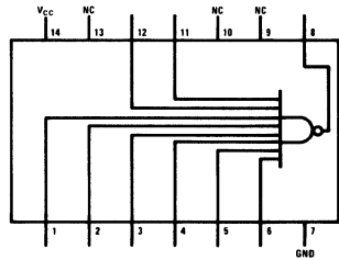
DM54L30/DM74L30
