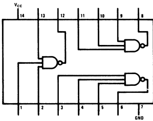
DM54L10/DM74L10
