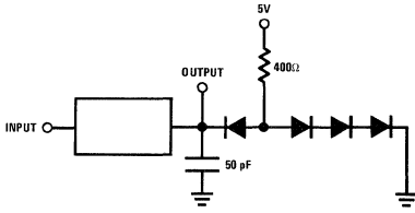
Test Circuit 1
