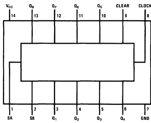
Dual-In-Line Package DM76L70/DM86L70 (DM54L164/DM74L164)
