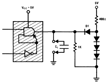
Test Circuit 3
