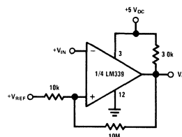
Comparator with Hysteresis
