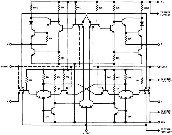
DM54L73/DM74L73, DM54L78/DM74L78
