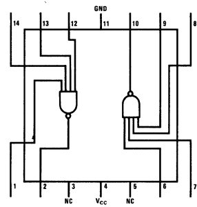
DM54L20/DM74L20
