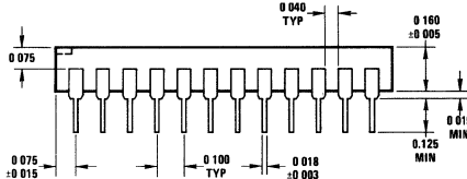
Package 7 24 Lead Molded DIP (N)
