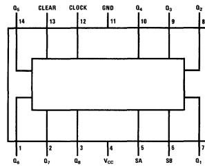
Flat Package DM76L70/DM86L70
