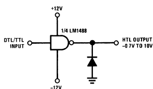
DTL/TTL-to-HTL Translator
