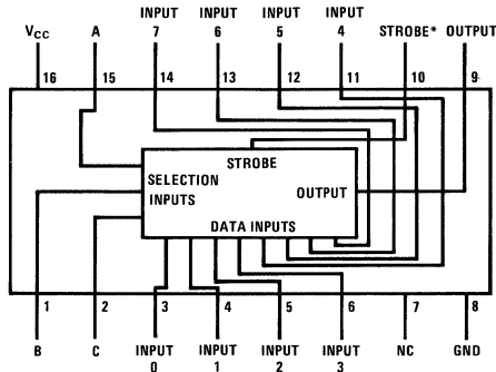
DM7211 Dual-In-Line and Flat Packages
