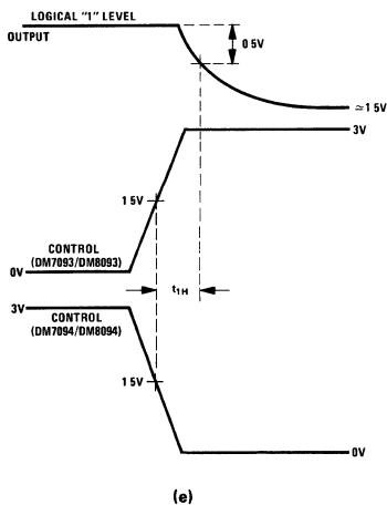
Waveform 10
