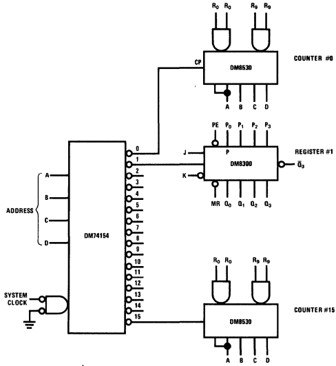
Demultiplexing System Clock
