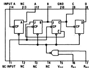
DM5492/DM7492
