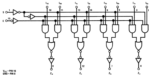
DM71L22/DM81L22
