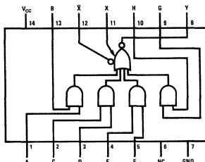
DM5453/DM7453, DM5454/DM7454
