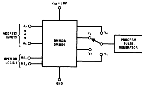
Programming Connections
