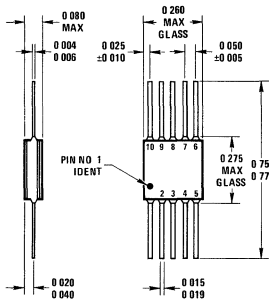
Package 14 10 Lead Flat Package (F)
