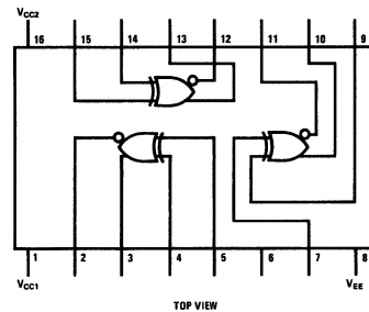
Dual-In-Line Package
