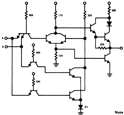
DM54L86/DM74L86
