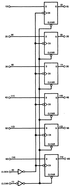
DM54174/DM74174
