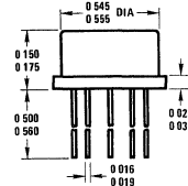
Package 22 10 Lead Metal Can Package (H) (Hybrids Only)
