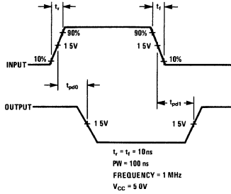
Waveform 1
