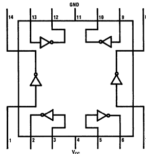
DM54L04/DM74L04
