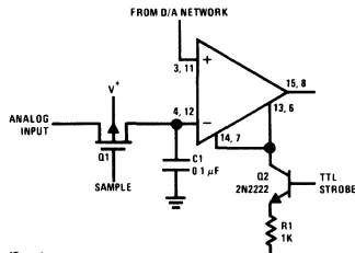
Strobing both Input* and Output Stages
