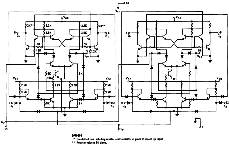
DM9097/DM9099 (DM9097 shown)
