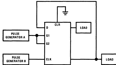
FIGURE 2. Use Waveforms B
