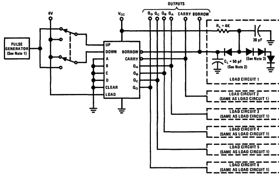
Test Circuit 1
