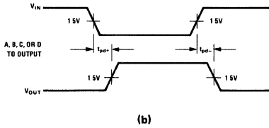
Waveform 18
