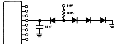
Test Circuit 5
