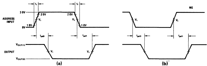
Waveform 52
