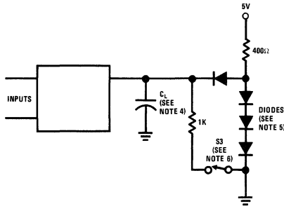
Figure 2 (Load Circuit)
