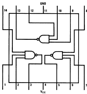
DM54L10/DM74L10
