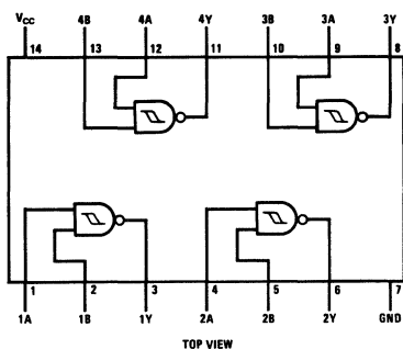
Dual-In-Line and Flat Package DM54132/DM74132
