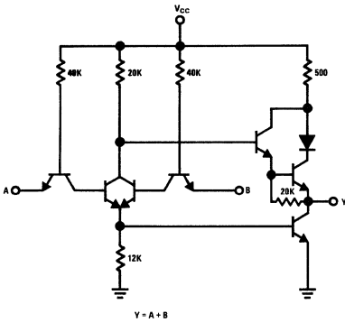
DM54L02/DM74L02
