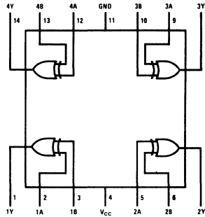
DM54L86/DM74L86
