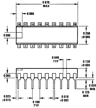
Package 6A 18 Lead Molded DIP (N)
