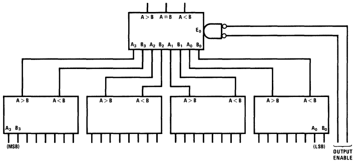
Figure X. 16-Bit Comparator, Maximum Logic Expansion: A < B , A > B , A \equiv B , A \sim B
