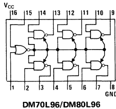
DM70L96/DM80L96
