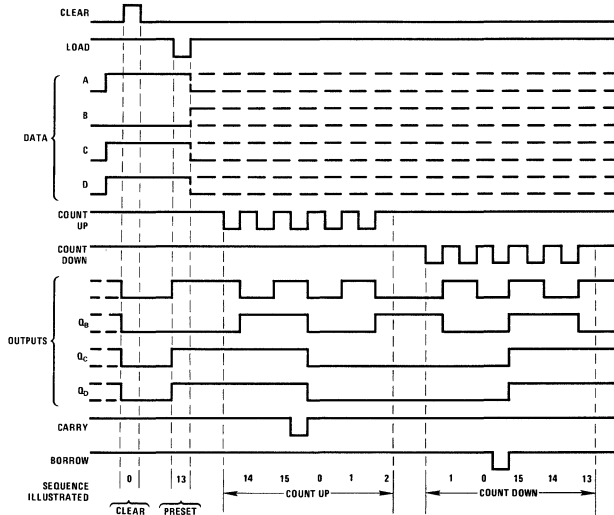
DM54L193/DM74L193
