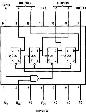
Flat Package DM54L93/DM74L93
