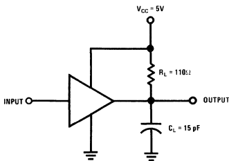
Test Circuit 4
