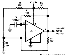
100 kHz Free Running Multivibrator
