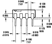
Package 1 8 Lead Molded Mini DIP (N)
