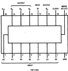
Dual-In-Line Package
