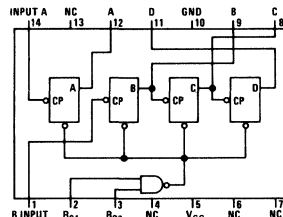
DM5493/DM7493
