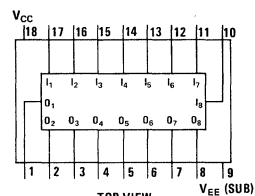
DM7897/DM8897
