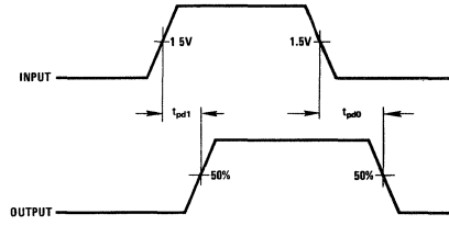
Waveform 35
