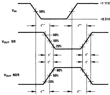
Waveform 41
