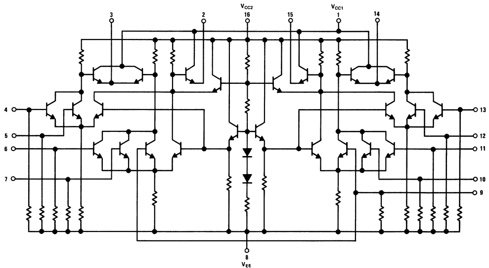
Dual-In-Line Package
