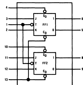
DM9097/DM9099
