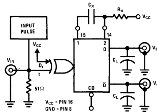
Test Circuit 21
