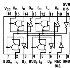
TOP VIEW DM7835/DM8835
