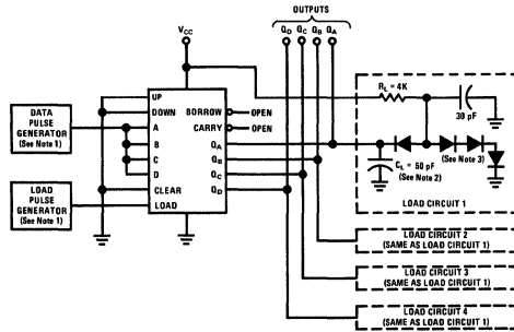
Test Circuit 1
