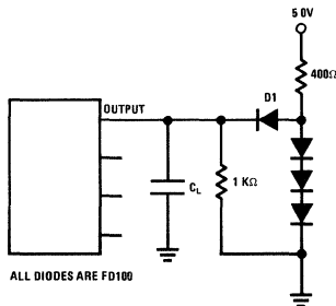
Test Circuit 15
