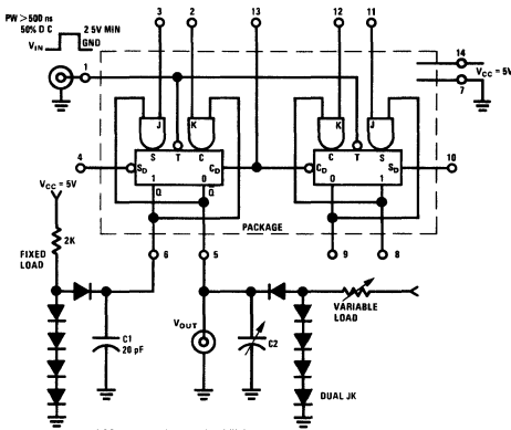
DM9097/DM9099
