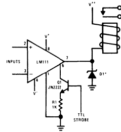
Relay Driver with Strobe
