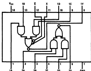
DM5450/DM7450, DM5451/DM7451
