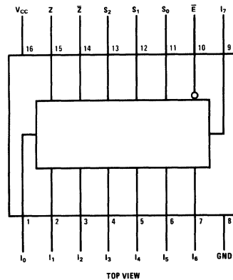
Dual-In-Line and Flat Package
