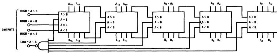
Figure X. 16-Bit Comparator, Maximum Logic Expansion: A < B , A > B , A \equiv B , A \sim B
