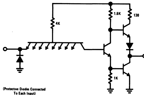
DM5430
