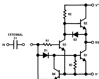
FIGURE 3. Simplified MH0026
