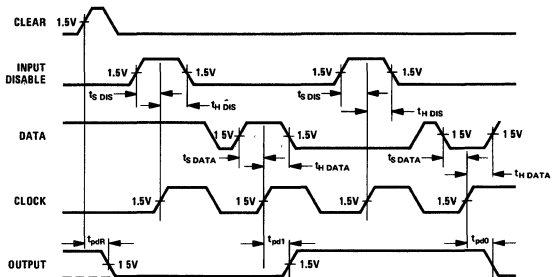
Waveform 25
