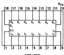
DM7889/DM8889
