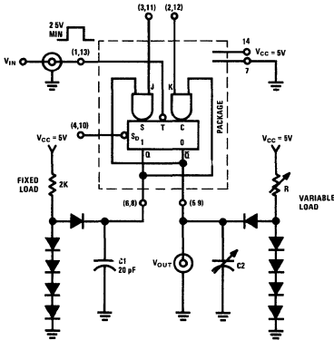
DM9093/DM9094 (one-half circuit shown)
