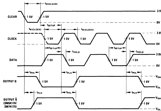
Waveform 56
