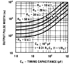
Output Pulse Width vs Timing Resistance and Capacitance for C_X < 10^3 \text{ pF}
