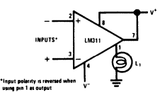
Driving Ground-Referred Load *Input polarity is reversed when using pin 1 as output
