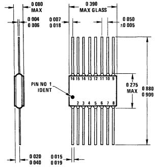
Package 16 16 Lead Flat Package (F)
