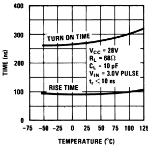
Turn On And Rise Time
