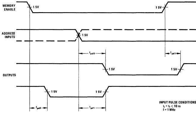
Waveform 31
