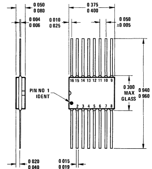
Package 19 16 Lead Flat Package (W)
