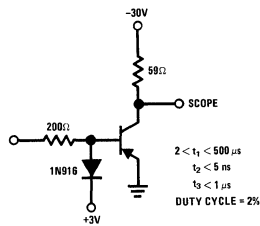
FIGURE 1. Turn-On Equivalent Test Circuit
