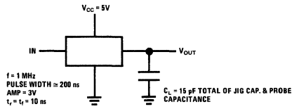
Test Circuit 14
