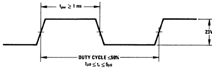
Programming Pulse
