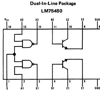
Positive Logic: \overline{A \cdot S} = X
