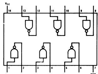
DM54L04/DM74L04
