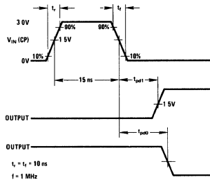
Waveform 19
