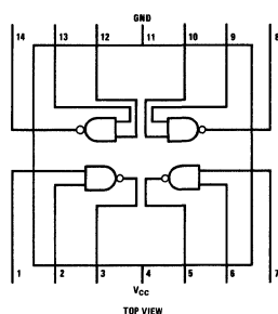
Flat Package
