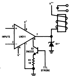
Relay Driver with Strobe *Absorbs inductive kickback of relay and protects IC from reverse voltage transients on V** line
