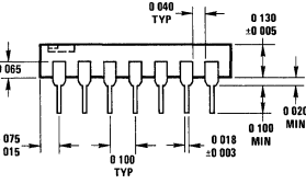
Package 4 14 Lead Molded DIP (N-01) (Staggered Leads)
