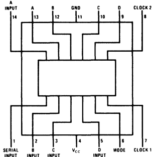
DM54L95/DM74L95
