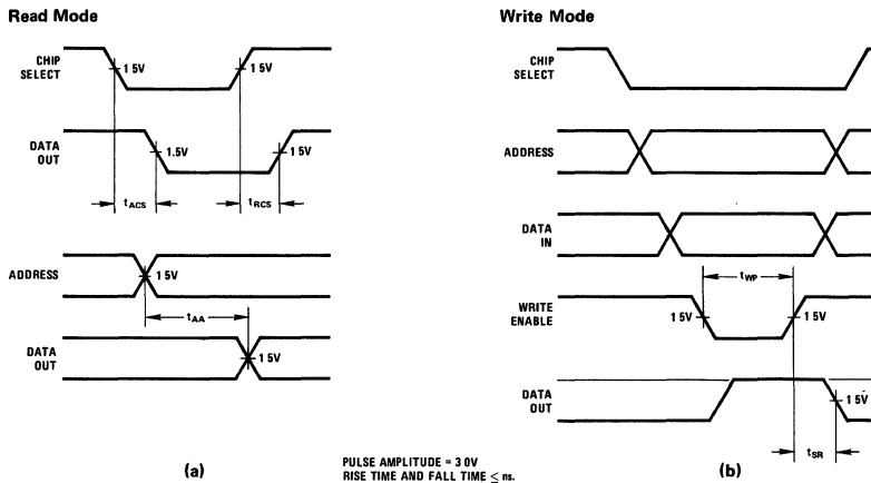
Waveform 33
