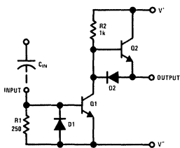
FIGURE 1. MH0025 Schematic (One-Half Circuit)
