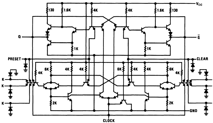
DM5472/DM7472
