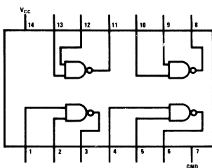
DM54L00/DM74L00 DM54L03/DM74L03
