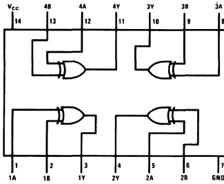
DM54L86/DM74L86
