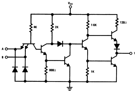
DM5408, DM7408
