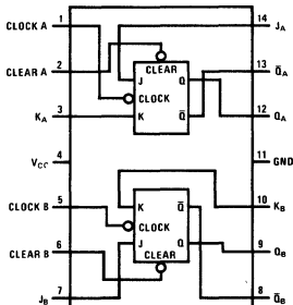
DM5473/DM7473
