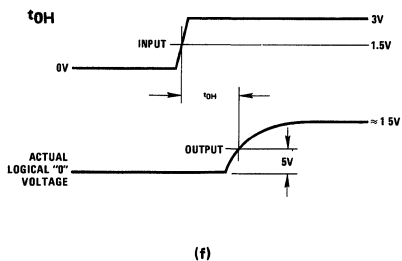
Waveform 26
