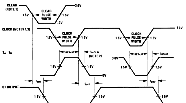
Waveform 28
