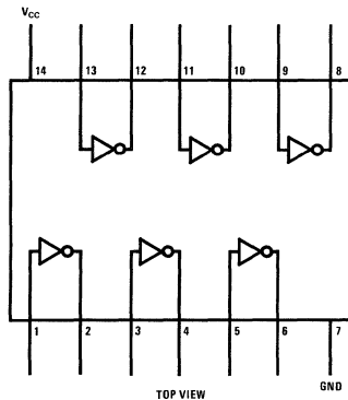
Dual-In-Line and Flat Package
