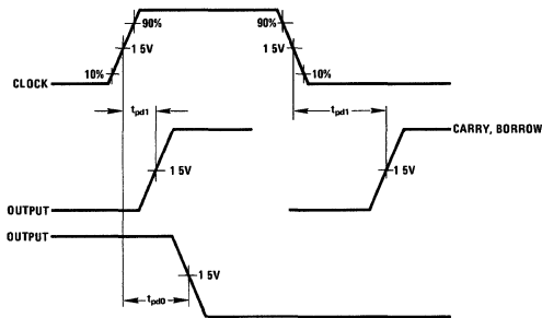
Waveform 28
