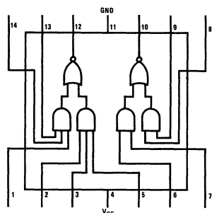
DM54L51/DM74L51
