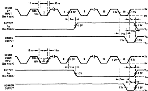
Voltage Waveforms 2
