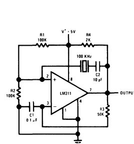
Crystal Oscillator
