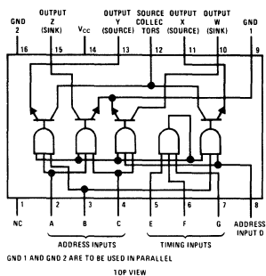
Dual-In-Line Package (J)
