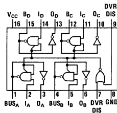
TOP VIEW DM7834/DM8834
