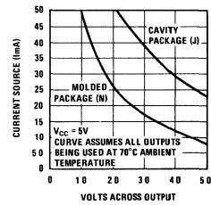
Max Power Dissipation Curve
