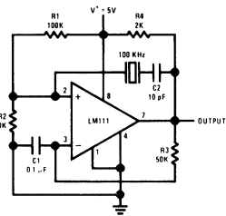
Crystal Oscillator
