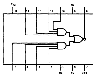
DM54L55/DM74L55
