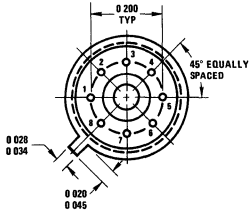
Package 20 8 Lead Metal Can Package (H)
