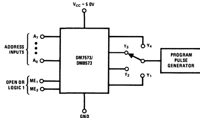
Programming Connections
