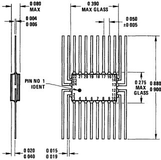
Package 17 24 Lead Flat Package (F)
