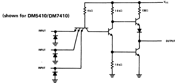
DM5410/DM7410
