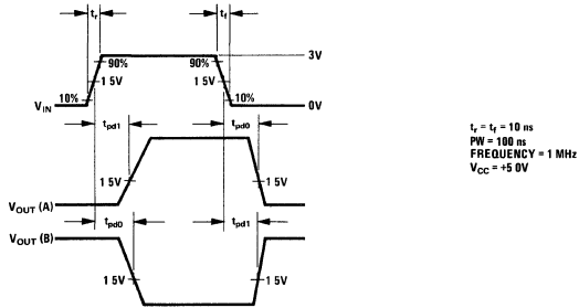
Waveform 15
