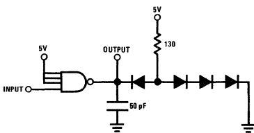
Test Circuit 6
