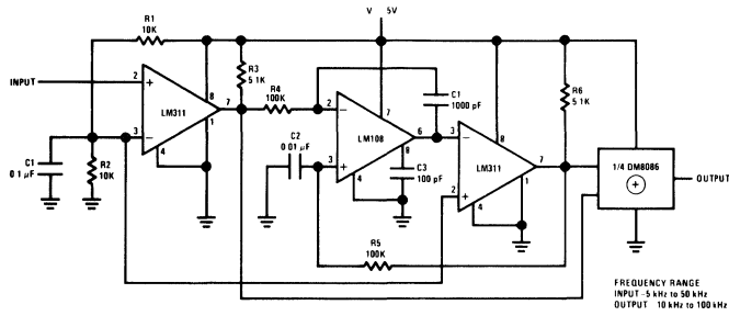
Frequency Doubler
