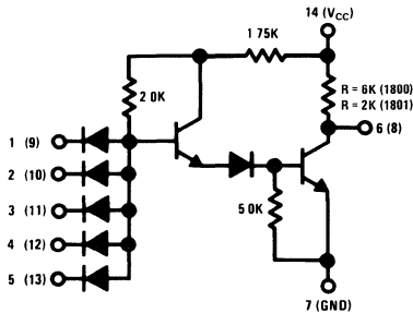
DM1800/DM1801
