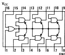
DM70L97/DM80L97
