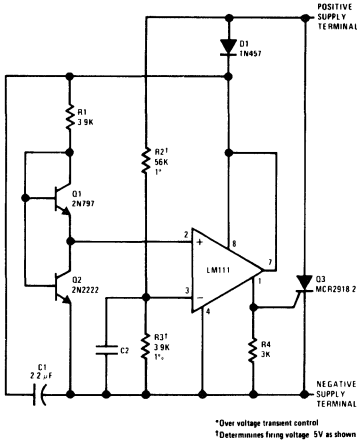
Crowbar Over-Voltage Protector
