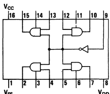
TOP VIEW DM75493
