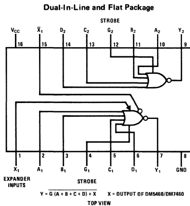
DM5423/DM7423
