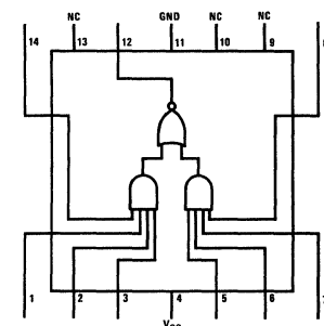
DM54L55/DM74L55
