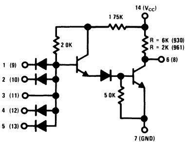
DM930/DM961
