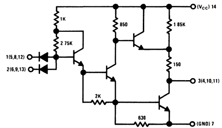
DM957
