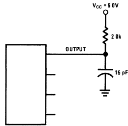
Test Circuit 18
