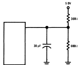
Test Circuit 7
