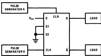
FIGURE 3. Use Waveforms C
