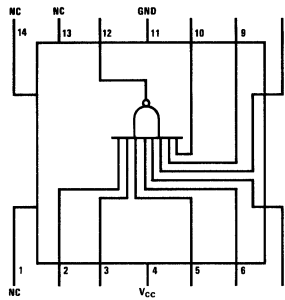
DM54L30/DM74L30
