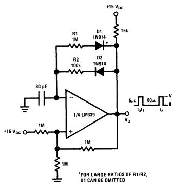
Pulse Generator
