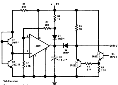
Precision Squarer
