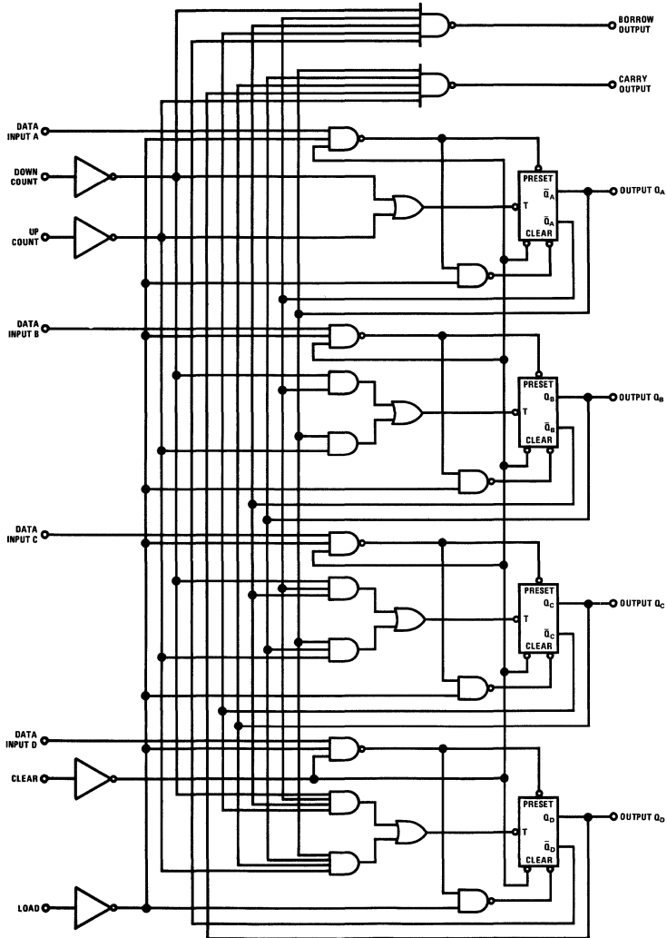
DM54L193/DM74L193
