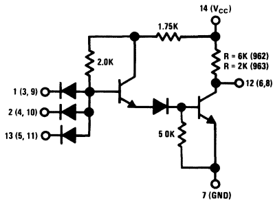
DM962/DM963
