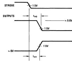
t_{H0} & t_{H1}
