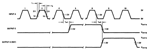
Note 1: The pulse generator has the following characteristics: V_{OH} = 2V , t_r = t_f \leq 10 ns, f_r = 0.5 MHz, P_{RR} = 1 MHz, Z_{OUT} = 50\Omega . Note 2: All loads are 1K200 or equivalent. Note 3: C_L includes probe and jig capacitance. Note 4: t_{SU} = t_{H} = t_{PD} . Note 5: Voltage values are with respect to ground terminal.
