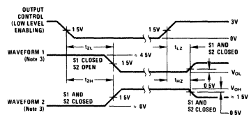
DM74S251
