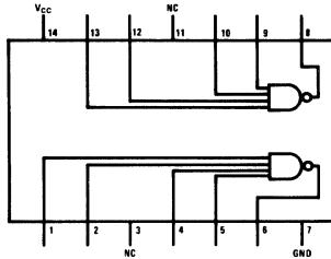
DM54L20/DM74L20
