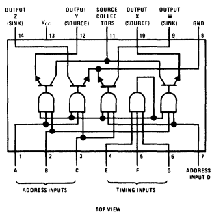
Dual-In-Line Package (N)
