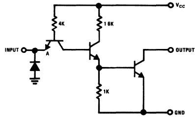
DM5405/DM7405
