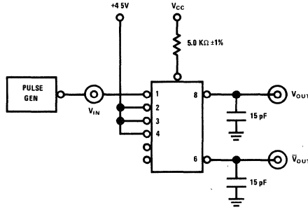
Test Circuit 8
