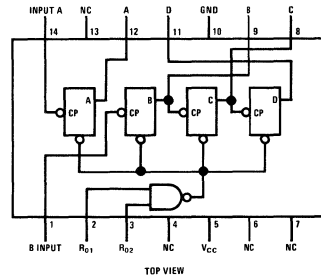
Dual-In-Line Package DM76L93/DM86L93
