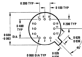
Package 24 12 Lead TO-8 Metal Can Package (G)
