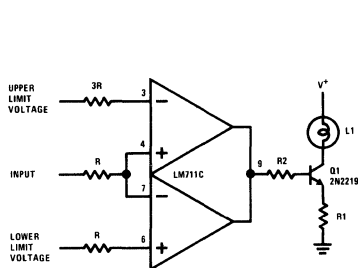
Double-Ended Limit Detector With Lamp Driver
