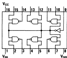
TOP VIEW DM75494
