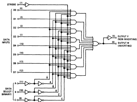
DM74S151
