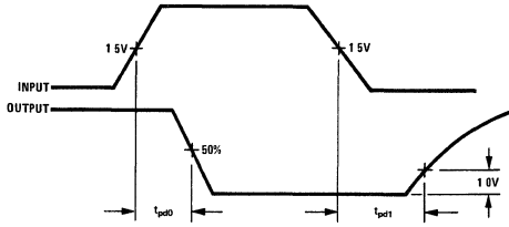
Waveform 34
