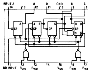
DM5490/DM7490
