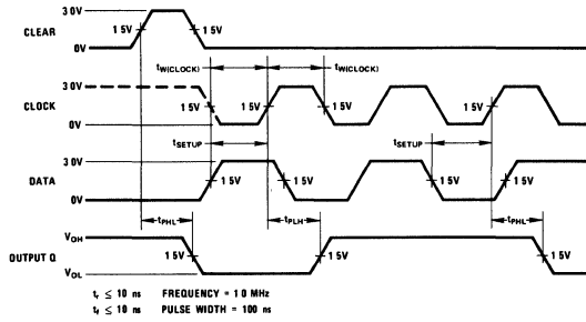
Waveform 49
