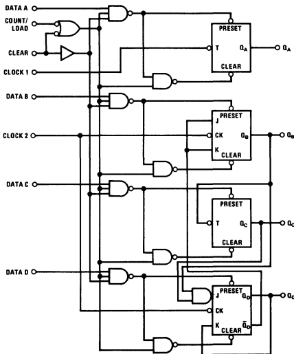
DM54196/DM74196
