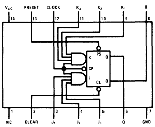
DM54L72/DM74L72
