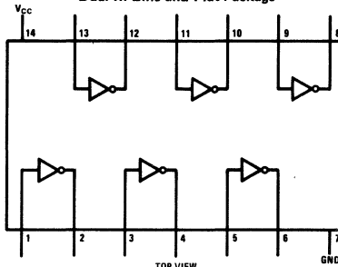
DM7812/DM8812
