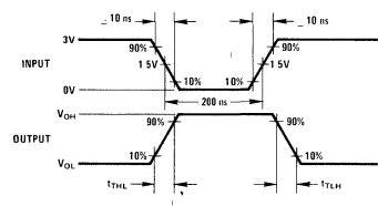
VOLTAGE WAVEFORMS
