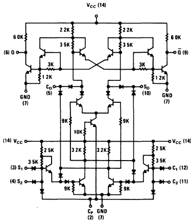
DM945
