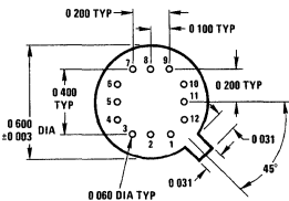
Package 23 12 Lead TO-8 Metal Can Package (G) (Hybrids Only)
