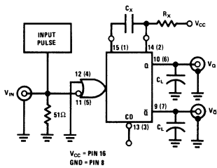
Test Circuit 24
