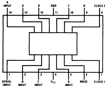
DM54L95/DM74L95
