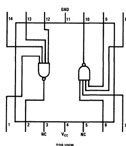
Flat Package
