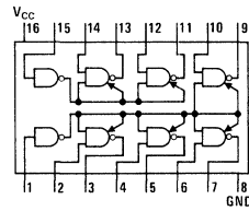
DM70L98/DM80L98
