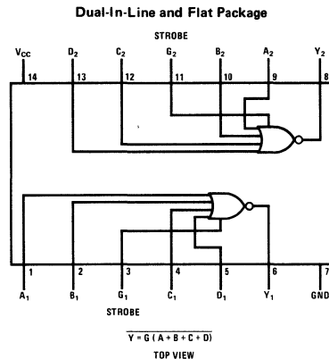
DM5425/DM7425
