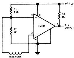
Detector for Magnetic Transducer
