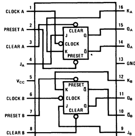
DM5476/DM7476
