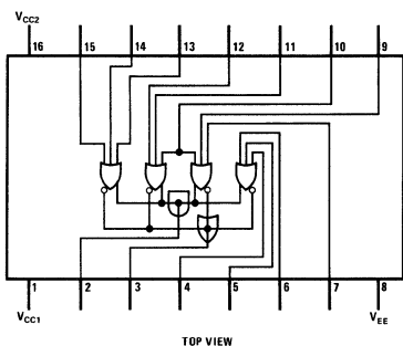
Dual-In-Line Package
