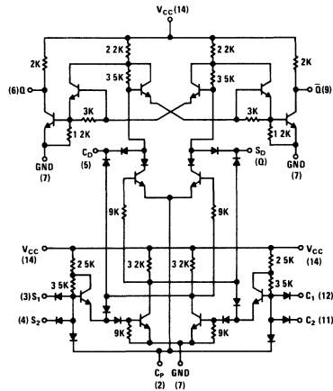
DM948
