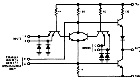
DM5450/DM7450, DM5451/DM7451 (each gate)
