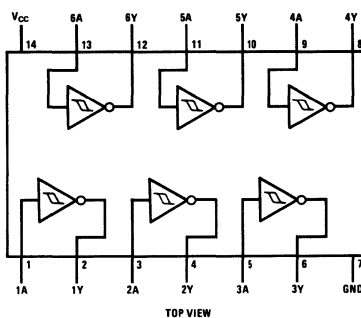
Dual-In-Line and Flat Package DM5414/DM7414
