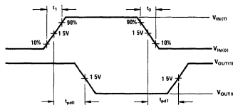
Note 1 The pulse generator has the following characteristics: V_{in(1)} = 3V, V_{in(0)} = 0V, t_r = t_f = 2.5 \text{ ns} , PRR = 1 MHz, Duty Cycle = 50%, Z_{out} = 50 \Omega Note 2 C_L includes probe and jig capacitance
