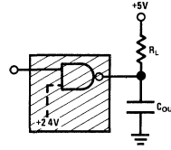
Test Circuit 2
