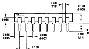
Package 6 16 Lead Molded DIP (N-01) (Staggered Leads)
