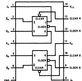
DM54107/DM74107
