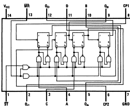
DM7281/DM8281 (DM54177/DM74177)
