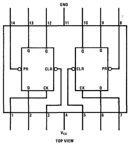
DM5474 Flat Package
