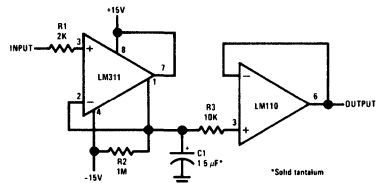
Positive Peak Detector *Solid tantalum
