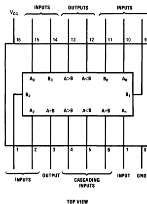
Dual-In-Line and Flat Package
