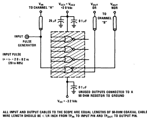
Test Circuit 10
