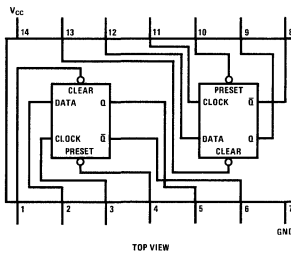
DM5474/DM7474 Dual-In-Line Package
