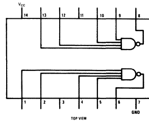
Dual-In-Line Package
