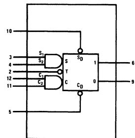
DM945/DM948
