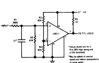
TTL Interface with High Level Logic
