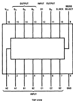
Flat Package
