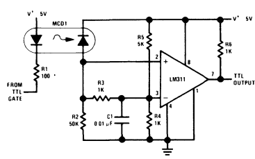
Digital Transmission Isolator
