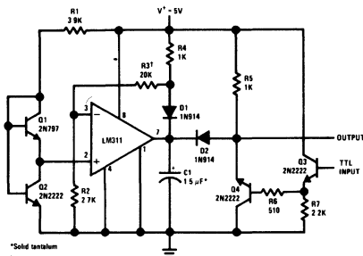
Precision Squarer
