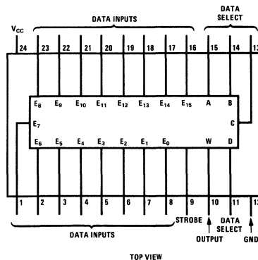
Dual-In-Line and Flat Package
