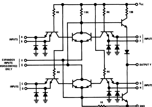
DM5453/DM7453, DM5454/DM7454
