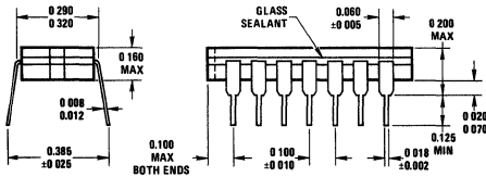
Package 11 14 Lead Cavity DIP (J)
