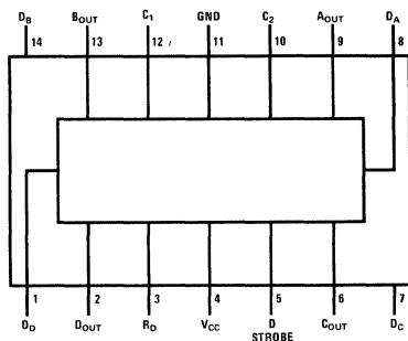
DM7280/DM8280, DM7281/DM8281, DM7288/DM8288 (Not applicable to DM54176W or DM54177W)
