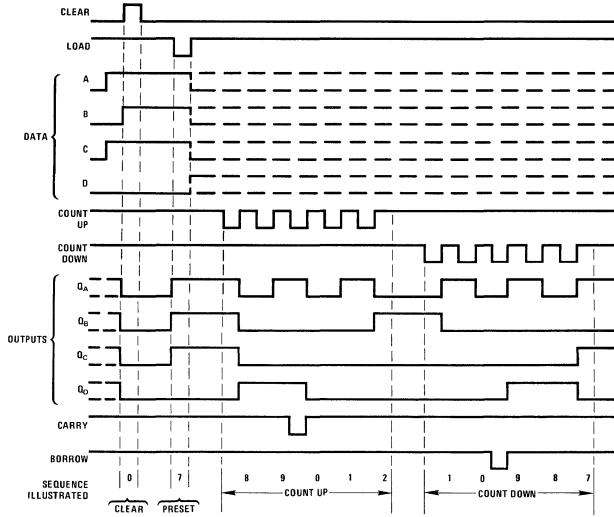
DM54L192/DM74L192
