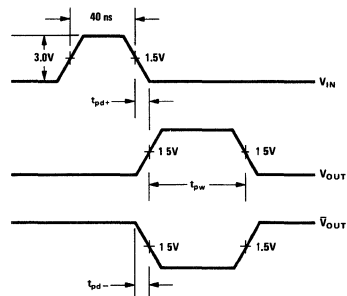
Waveform 38
