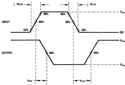
Waveform 43
