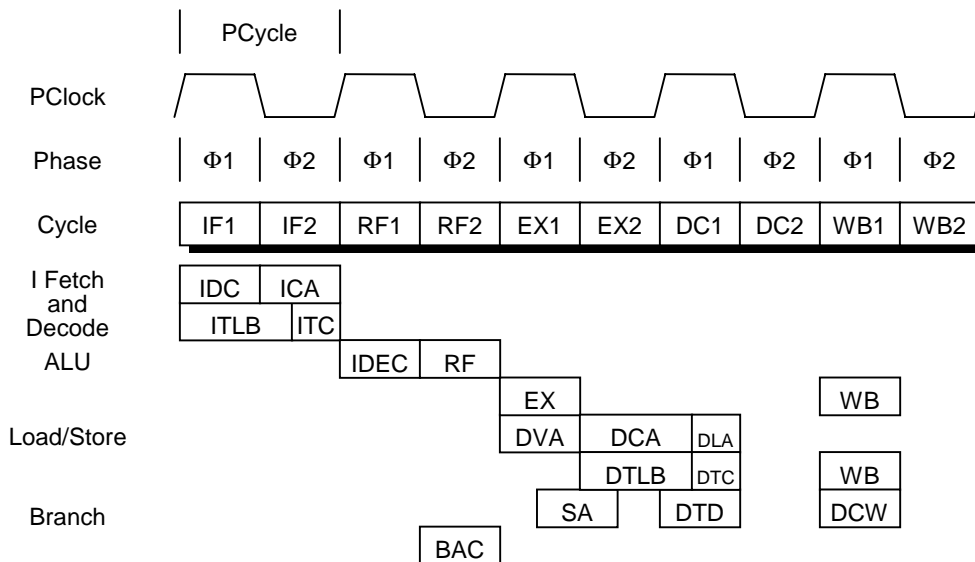
Figure 5-3. Pipeline Activities
