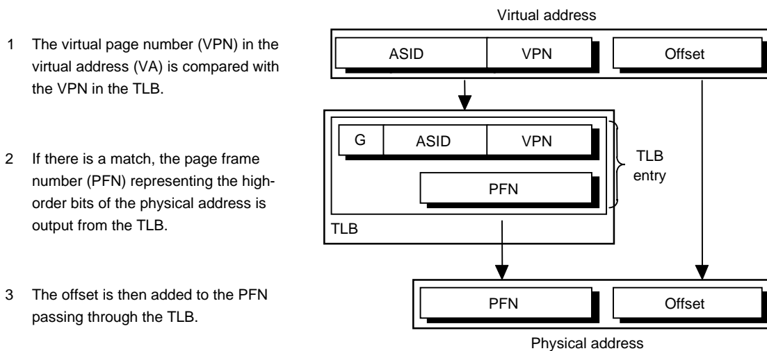
Figure 6-1. Virtual-to-Physical Address Translation
