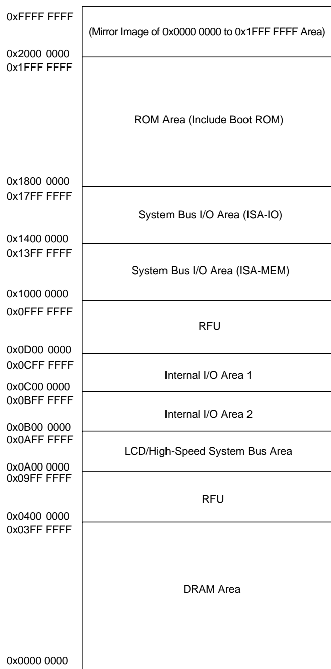
Figure 6-8. V R 4111 Physical Address Space
