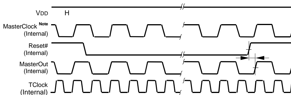
Figure 8-9. Soft Reset
