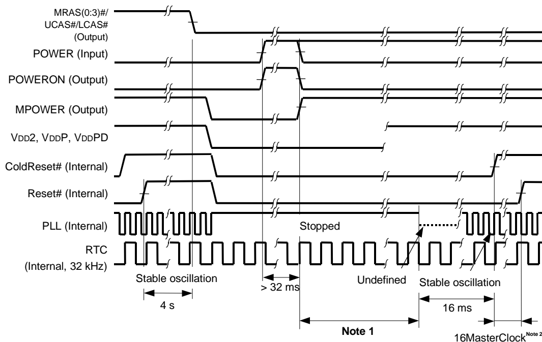
★ Figure 8-5. HALTimer Shutdown
