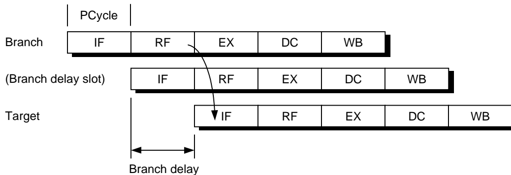
Figure 5-4. Branch Delay
