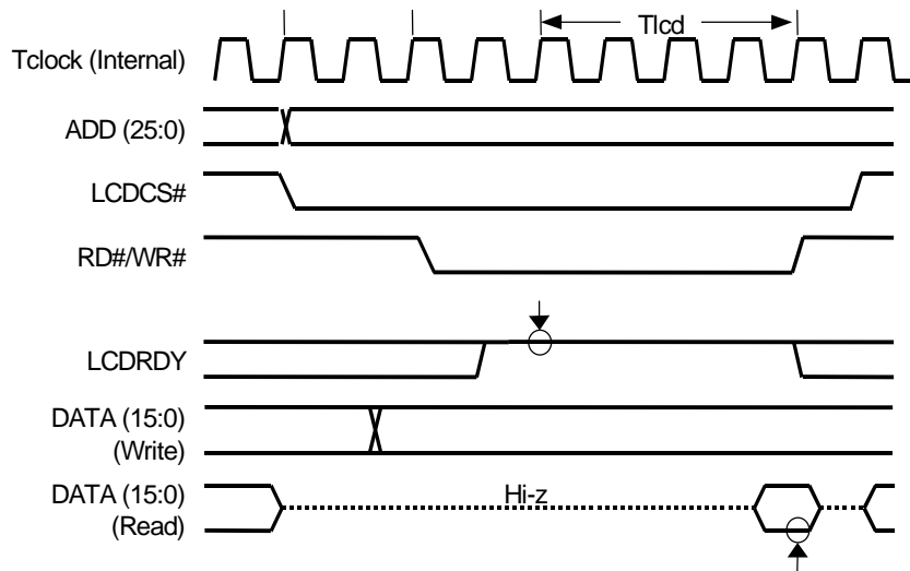
Figure 11-17. 2-Byte Access to LCD Controller (WLCD/M[2:0] = 010)
