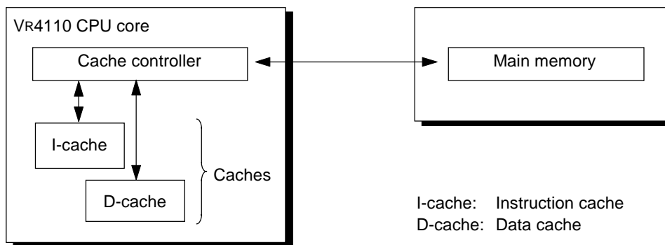
Figure 9-2. Cache Support
