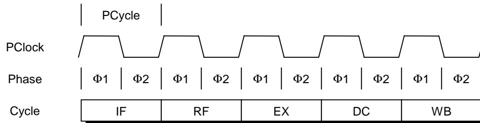
Figure 5-1. Pipeline Stages
