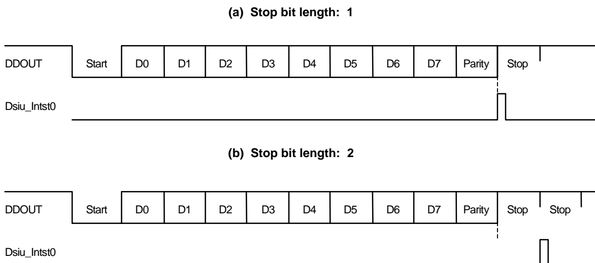
Figure 23-2. Transmit Complete Interrupt Timing
