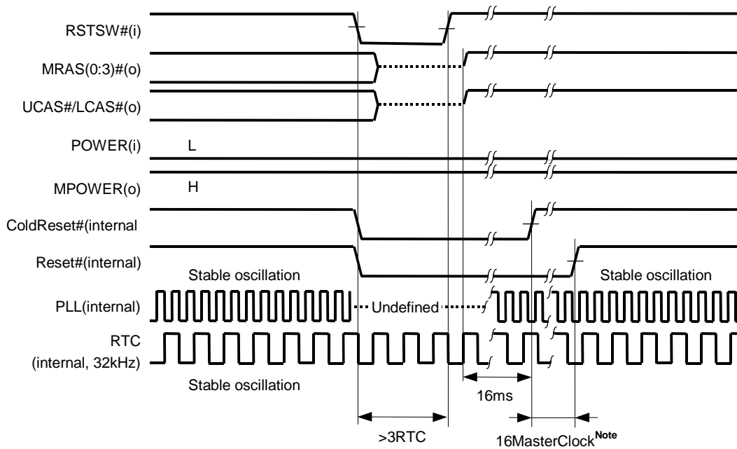
Figure 8-2. RSTSW
