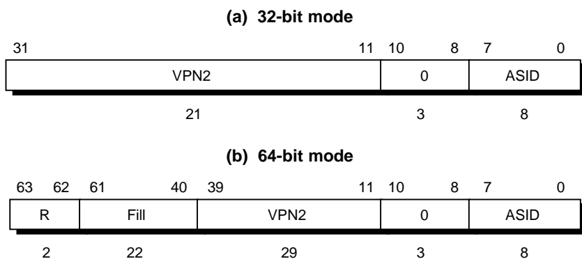
Figure 6-17. EntryHi Register
