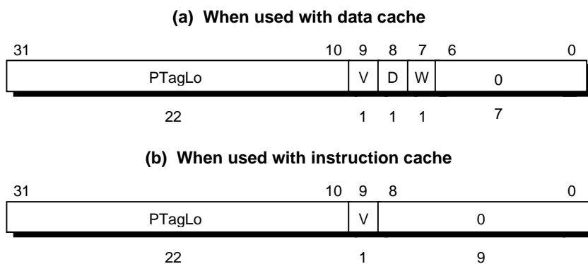
Figure 6-21. TagLo Register
