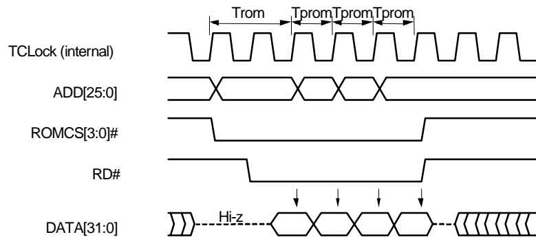
Figure 11-5. PageROM 4-Word Read, 32-Bit Mode (WROMA[2:0] = 111, WPROM[1:0] = 10)
