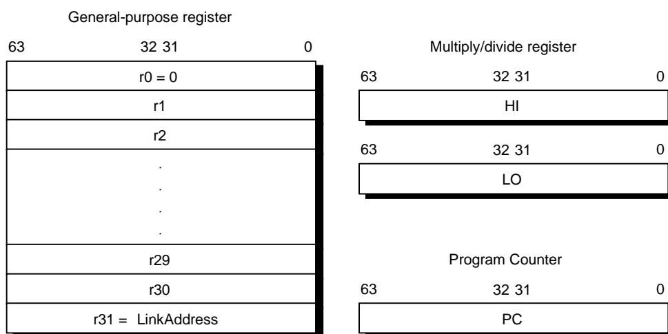
Figure 1-3. VR4111 CPU Registers
