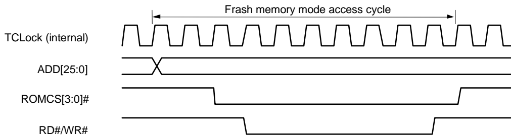
Figure 11-6. Flash Memory Mode, 2-Byte Access
