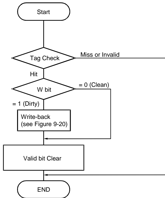
Figure 9-17. Data Check Flow on Hit_Writeback_Invalidate Operations
