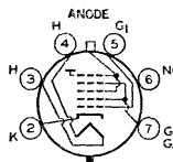
7FG ANODE = G 3 + G 5 + CL AUTOMATIC FOCUSING
