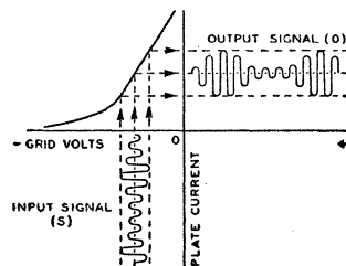
Fig. 34—Current characteristics of class A amplifier.
