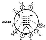
12C ANODE = G 4 + CL FOCUSING ELECTRODE = G 3
