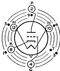
12AQ INDEX-LARGE LUG ●-SHORT PIN-IC
