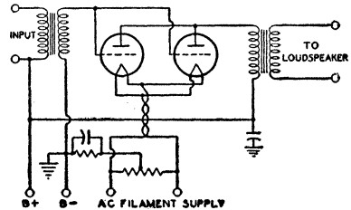
Fig. 39—Power amplifier with tubes connected in parallel.
