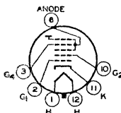
12AD ANODE = G 3 + G 5 + CL FOCUSING ELECTRODE = G 4
