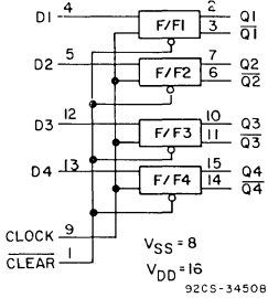
Quad "D"-Type Flip-Flop
