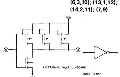
f) High Source-Current Driver
