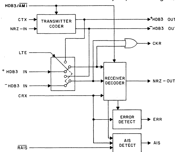
Fig. 1 - Block diagram of the CD22103.
