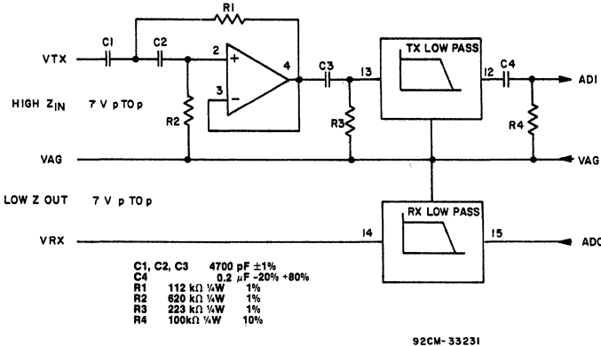
Fig. 11 - Filter schematic for CD22413 with 60-Hz reject filter.
