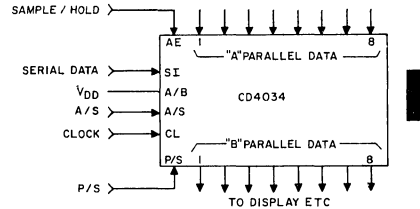
Fig. 22 - Sample and hold register—serial/parallel in—parallel out.
