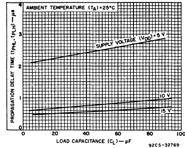
Fig. 8—Typical propagation delay time as a function of load capacitance (CLOCK to Q_1 , 8-BYPASS low).
