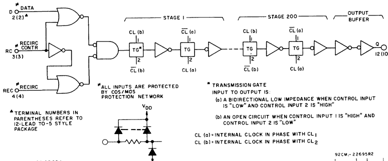
Fig. 1 - CD4062A logic block diagram.
