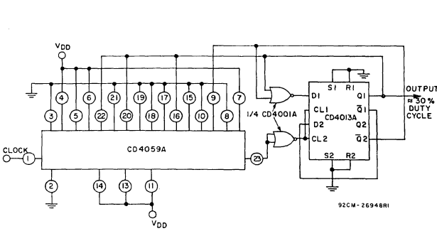
Fig. 16 - Division by 47,690 in \div 2 mode.
