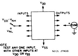
Fig. 10 - Noise immunity test circuit.
