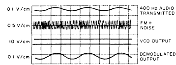
Fig. 11— Voltage waveforms of FM demodulator.
