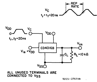
Fig. 22 - Max. control-input repetition rate.
