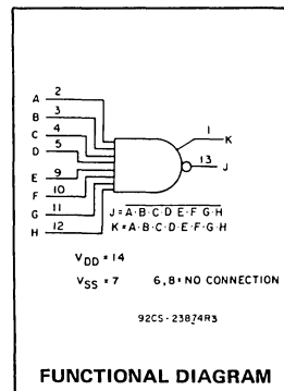
FUNCTIONAL DIAGRAM
