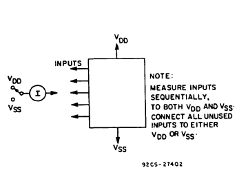
Fig. 11 - Input current test circuit.
