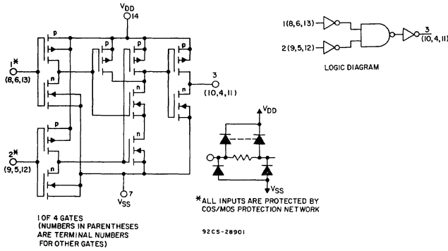
Fig.6 - Schematic and logic diagrams for CD4001B.
