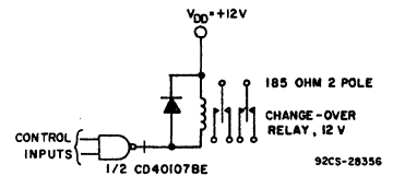
92CS-28356 Fig. 10 - Relay driver circuit.
