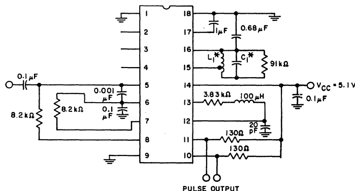
Fig. 2 - DC and output pulse test circuit.
