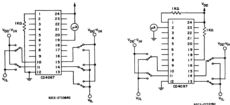
Fig. 8—Input voltage—measure < 2 μA on all OFF channels (e.g., channel 12).
