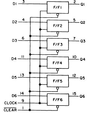
Hex "D" Type Flip-Flop
