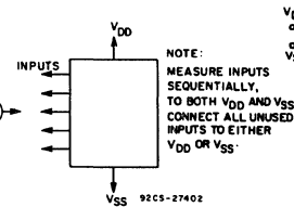
Fig. 20—Input leakage current test circuit.
