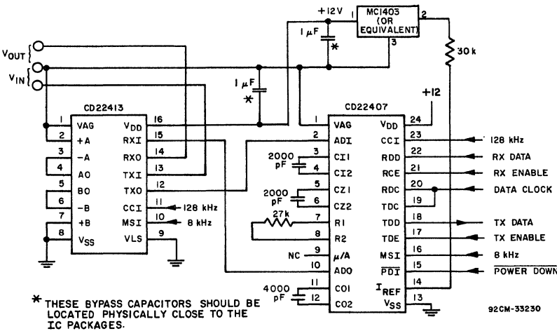
Fig. 10 - Typical circuit configuration using the CD22407 CODEC and CD22413 filter (single supply).
