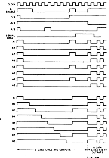
Fig. 3 — Timing diagram.
