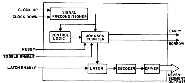
Fig. 1 - Functional diagram.
