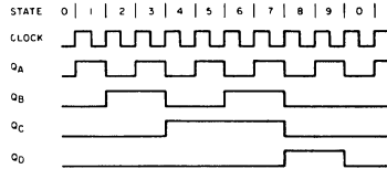
Fig. 18 - Synchronous binary divide-by-ten counter.
