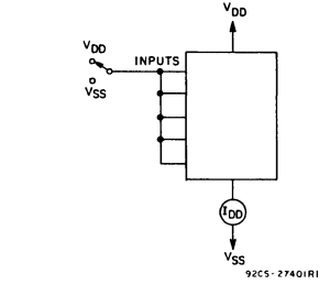
Fig. 8 - Quiescent-device current test circuit.
