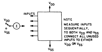
Fig. 10— Input leakage current test circuit.
