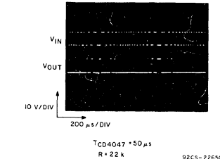
Fig. 29 - Low-pass-circuit waveforms.
