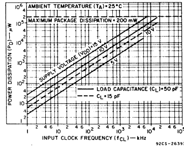
Fig. 9 — Typical power dissipation vs. input clock frequency.
