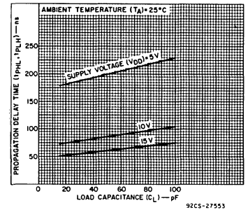
Fig. 11—Typical propagation delay time vs. load capacitance (SET to Q or RESET to \bar{Q} ).
