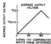
Fig. 4—Phase-comparator I characteristics low-pass filter output.
