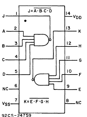
Dual 4-Input NAND Gate
