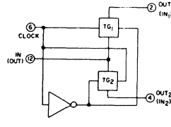
h) Dual Bi-Directional Transmission Gating
