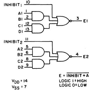
Dual 2-Wide, 2-Input AND-OR-INVERT (AOI) Gate
