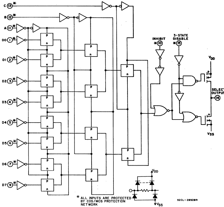
Fig. 1 - Logic diagram.
