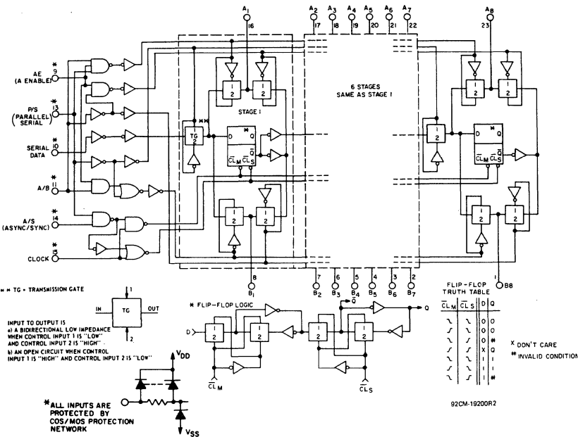
Fig. 2 — Logic diagram.
