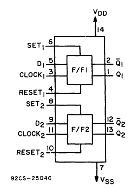
Dual "D" Flip-Flop with Set/Reset Capability
