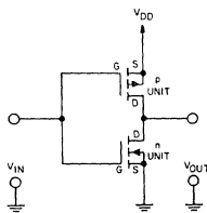
Fig. 3— Basic COS/MOS inverter (schematic).
