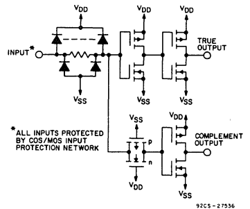
Fig.1 - Schematic diagram 1 of 4 buffers.
