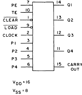
Synchronous 4-Bit Counter
