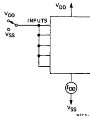
Fig. 9 — Quiescent device current test circuit.
