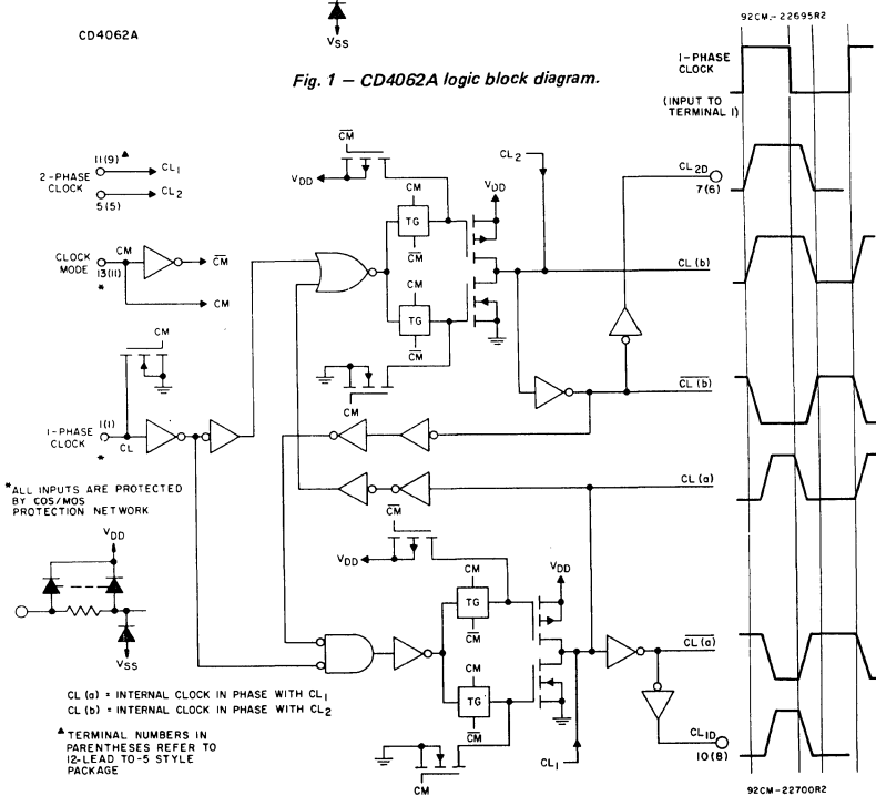
Fig. 2 - Clock circuit logic diagram.
