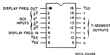
CD4055B Terminal Assignment
