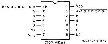
TERMINAL ASSIGNMENT
