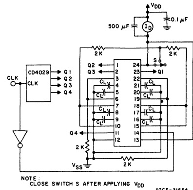
Fig. 14 - Dynamic power dissipation test circuit for CD22101.
