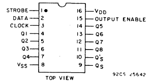
Fig. 1 — Terminal assignment.
