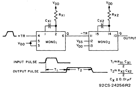
Fig. 15 — Pulse delay.
