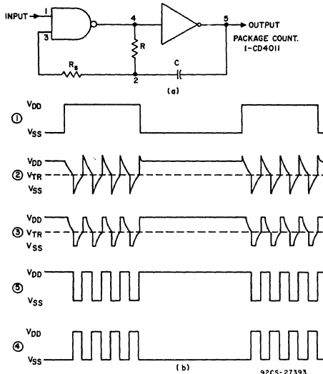
Fig. 24 - (a) Modulator circuit, (b) waveforms.
