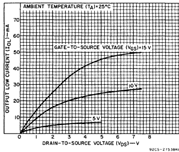
Fig.3 - Minimum low (sink) current characteristics.
