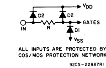
Fig. 1 — Functional diagrams.
