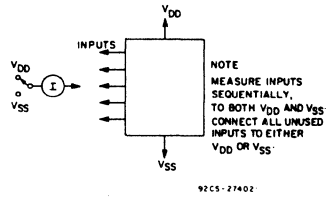
Fig. 8 — Input-leakage-current test circuit.
