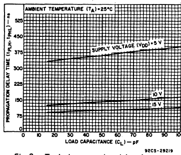
Fig. 8 — Typical propagation delay time as a function of load capacitance (CL or WE to Q).
