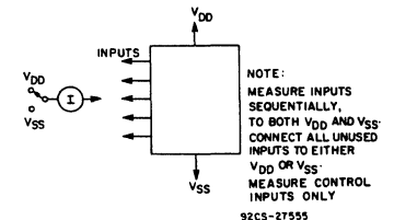
Fig. 12 - Input leakage current test circuit.
