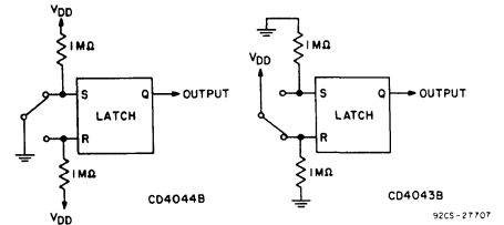
Fig. 12 – Switch bounce eliminator.
