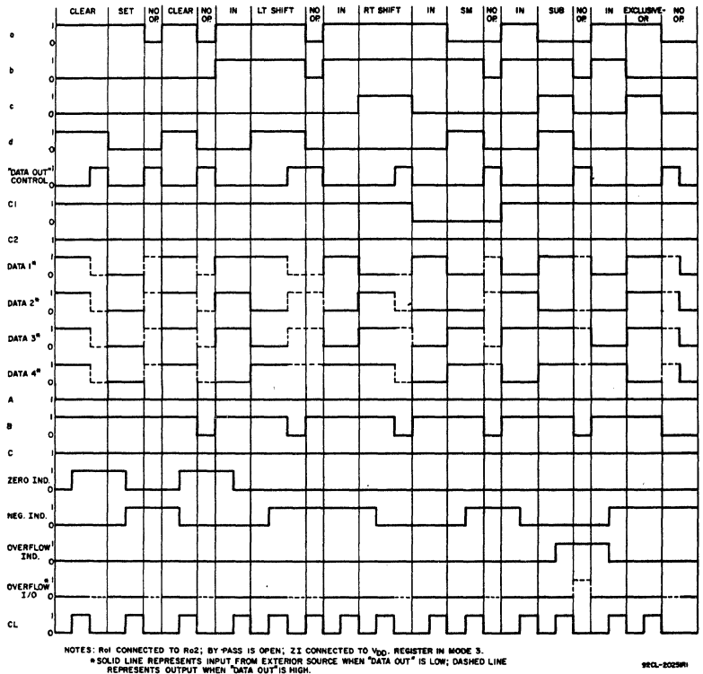
Fig. 12 – Timing diagram.
