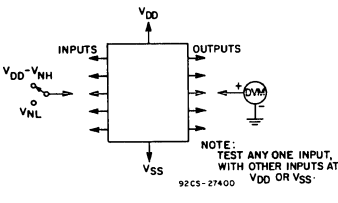
Fig.19 – Noise immunity test circuit.
