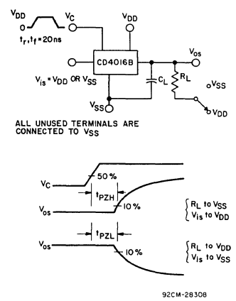
Fig. 25 - Turn-On propagation delay-control input.
