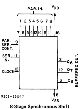
8-Stage Synchronous Shift Register with Parallel or Serial Input/Serial Output
