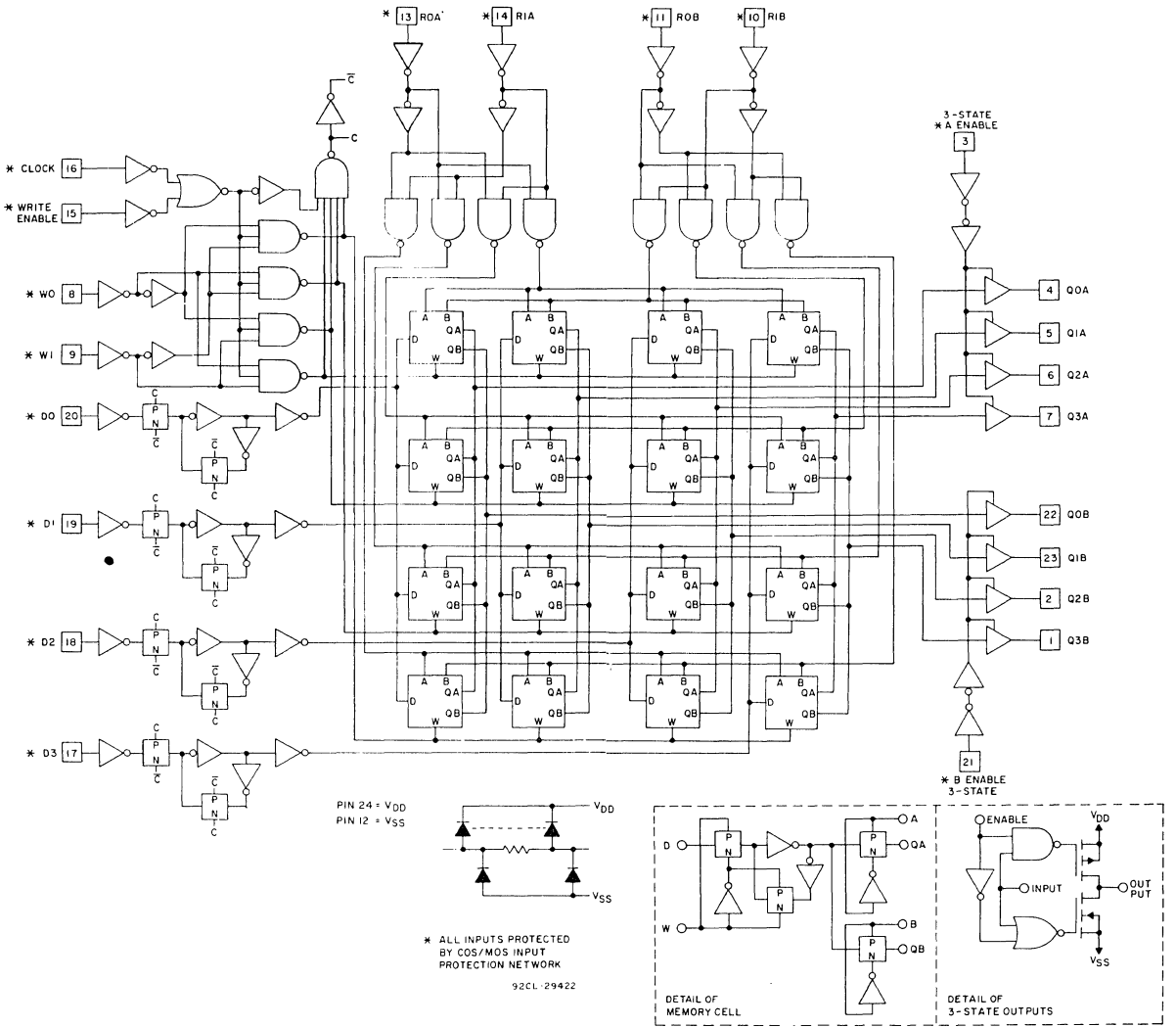
Fig. 13— Schematic diagram
