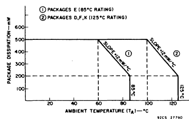
Fig. 1—Standard CMOS thermal derating chart.
