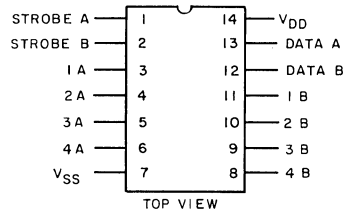
TERMINAL DIAGRAM
