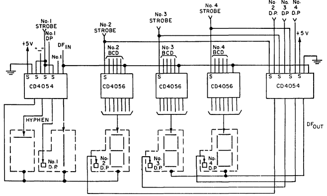
Fig.19 - Typical 3 1/2-digit liquid-crystal display: V_{DD} = +5 V , V_{SS} = 0 V , V_{EE} = -10 V , DF_{IN} = 30 \text{ Hz} square wave.
