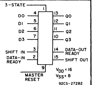
4-Bits Wide by 16-Bits Long Register
