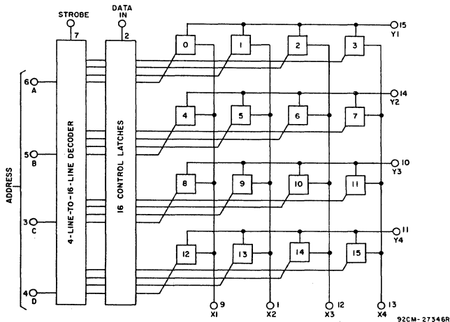
Fig. 1 – Functional diagram.
