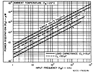
Fig. 5 — Typical dissipation characteristics. (per output).
