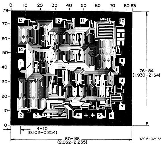
Dimensions in parentheses are in millimeters and are derived from the basic inch dimensions as indicated. Grid graduations are in mils ( 10^{-3} inch).
