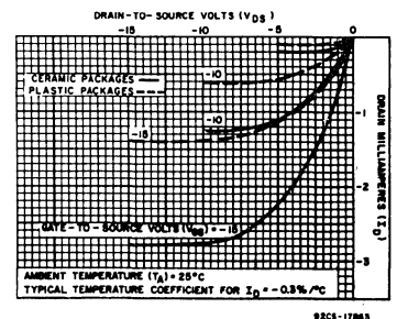
Fig. 6—Minimum output p-channel drain characteristics.
