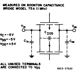
Fig. 24 - Capacitance C_{ios} and C_{os} .
