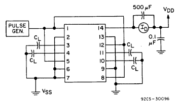
Fig. 14 – Dynamic power dissipation test circuit.
