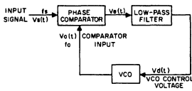
Fig. 1—Block diagram of PLL.
