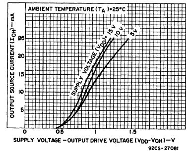
Fig. 13 - Typical voltage drop (V DD to output) vs. output source current as a function of output for the CD4511.
