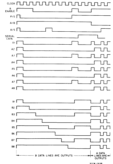
Fig. 4 — Timing diagram.
