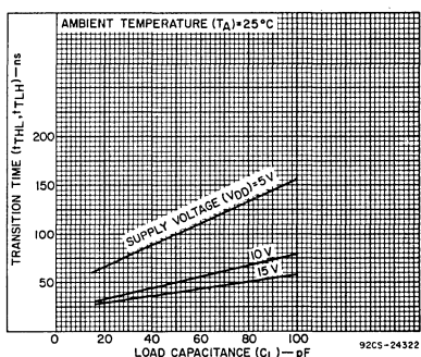
Fig. 15—Variation of transition time ( t_{THL} , t_{TLH} ) with load capacitance.
