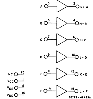
Fig. 1 — Logic diagrams.
