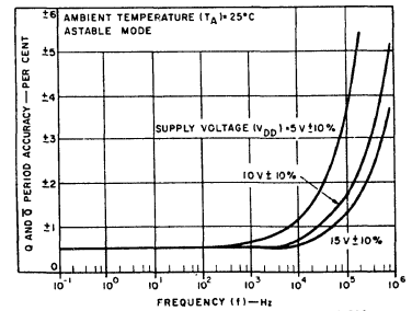
Fig. 14 — Typical Q-and-Q-bar-period accuracy vs frequency for V_{DD} variation of \pm 10\% from value indicated.
