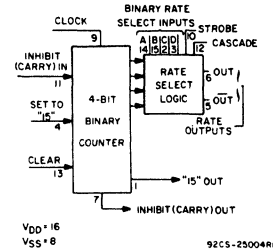
Binary Rate Multiplier
