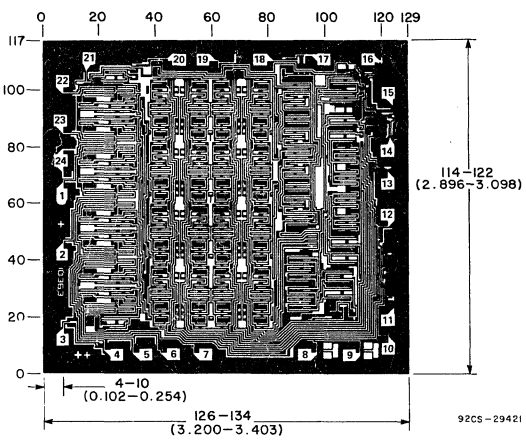
Dimensions and Pad Layout for CD40108BH
