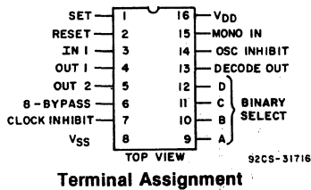
Terminal Assignment
