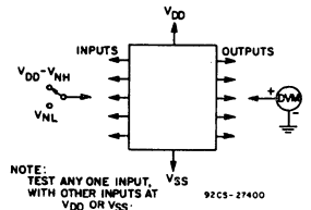
Fig. 7—Noise-immunity test circuit.
