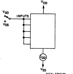
Fig. 9 - Quiescent device current.
