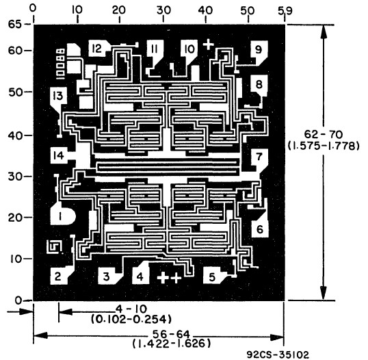
Dimensions and pad layout for CD4071B.
