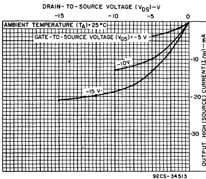
Fig. 2 - Typical output high (source) current characteristics.
