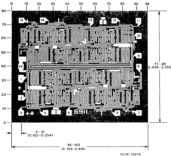
Photograph of Chip Layout for CD4015B.
