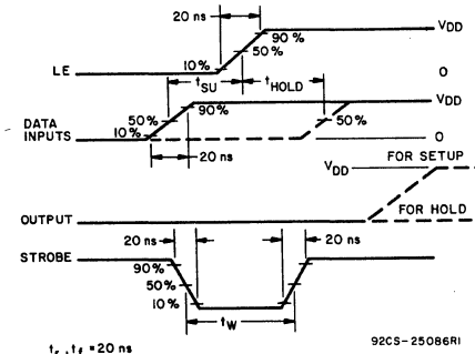
Fig. 14 - Dynamic waveforms.
