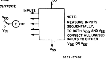
Fig. 11 - Input current.
