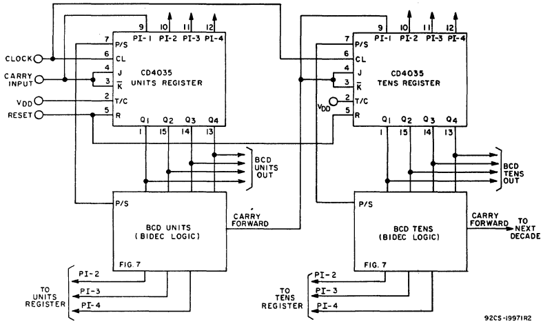
Fig. 17 - Binary-to-BCD converter.
