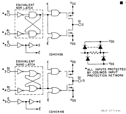
Fig. 1 — Logic diagrams.
