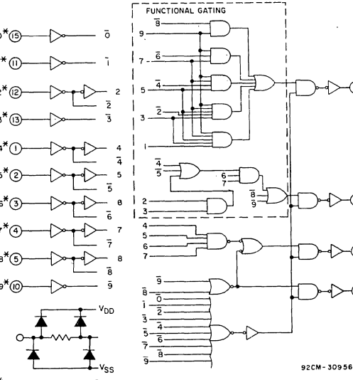
Fig. 1 - CD40147B logic diagram.
