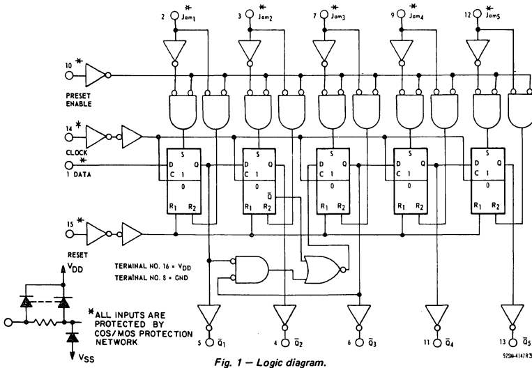
Fig. 1 - Logic diagram.
