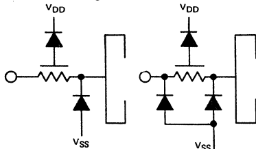
Fig. 7 — (a) Standard and (b) improved protection networks.
