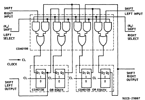
Fig. 14 — "Shift left/shift right" register.
