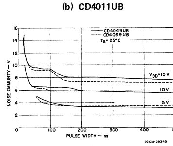
Fig. 13 Power-line noise immunity. T_A = 25^\circ C .
