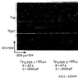
Fig. 31 - Bandpass-filter-circuit waveforms.
