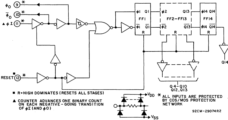
Fig. 1 - Logic diagram.
