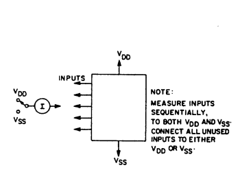
Fig. 13 – Input-leakage-current test circuit.
