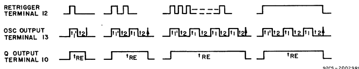
Fig. 34—Retrigger-mode waveforms.
