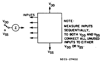
Fig.20 – Input leakage current test circuit.
