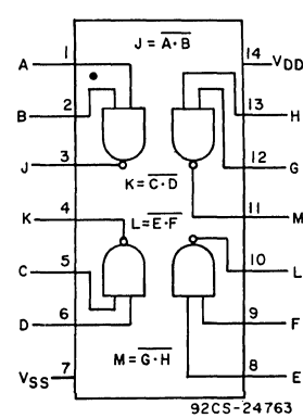
Quad 2-Input NAND Gate
