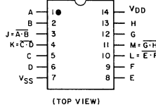
TERMINAL ASSIGNMENT
