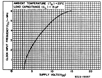
Fig. 3 - Typical clock input frequency vs. supply voltage.
