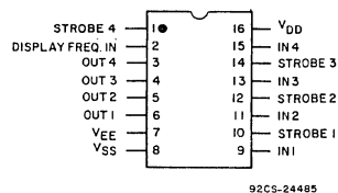
CD4054B Terminal Assignment
