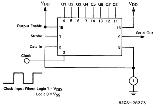
Fig. 15 - Functional-test arrangement for the CD4090.
