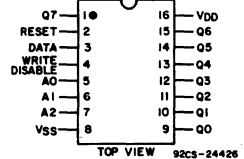
TERMINAL ASSIGNMENT
