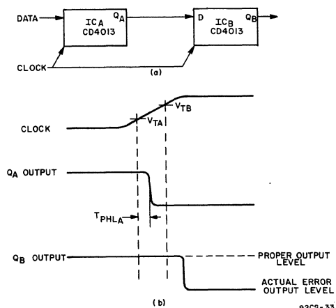
Fig.1-Parallel clocking of sequential CMOS IC's.
