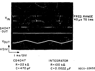
Fig. 26 - Frequency-discriminator-circuit waveforms.
