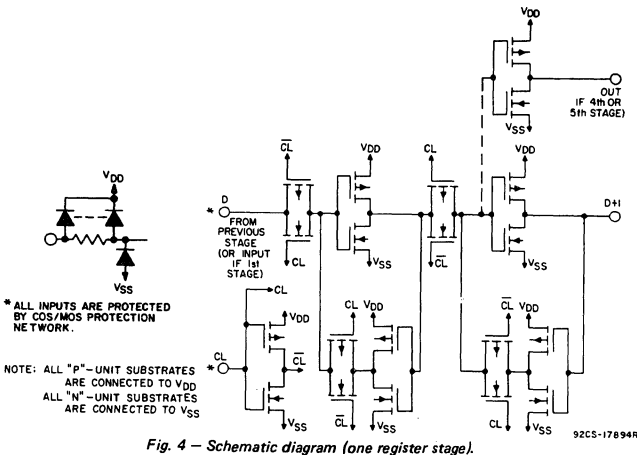
Fig. 4 - Schematic diagram (one register stage).
