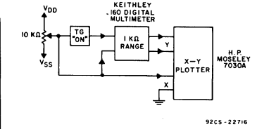
Fig. 7 - Channel on-state resistance measurement circuit.
