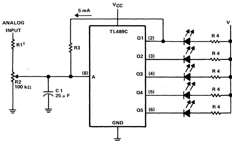
Figure 1. 5-Step Voltage-Level Indicator
