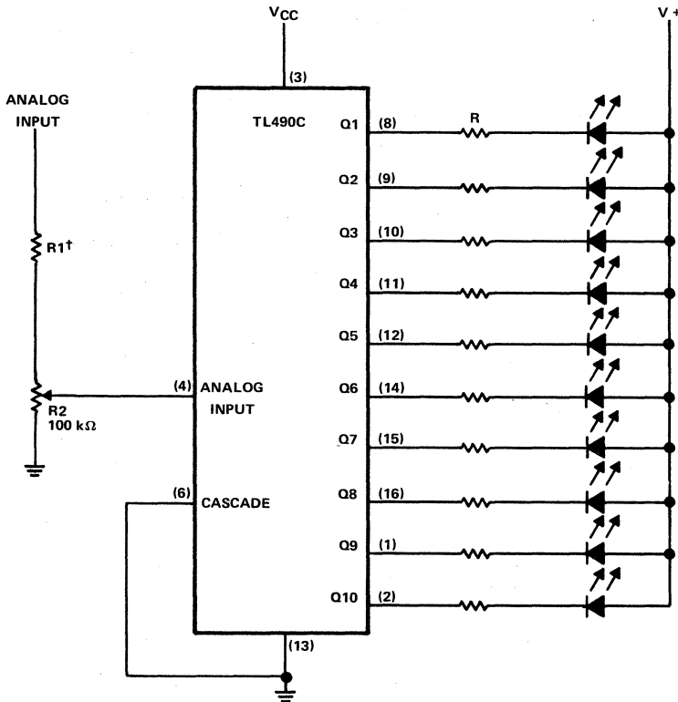
Figure 2. 10-Step Voltage-Level Indicator
