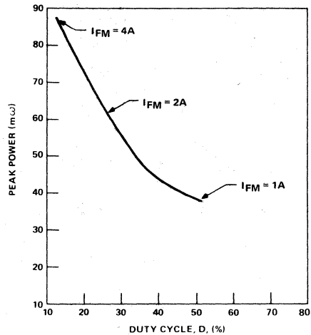
FIGURE 6. Typical Peak Power of TIES 27 at 10 kHz with Various Peak Current Levels at Various Duty Cycles
