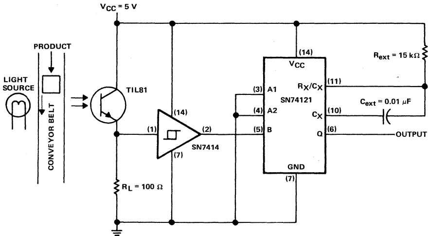
Figure 1. Circuit Schematic
