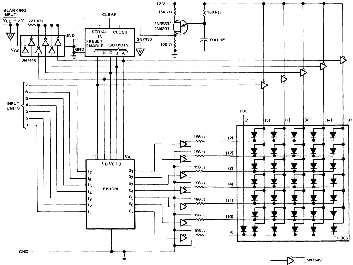
Figure 4. 5 X 7 Matrix
