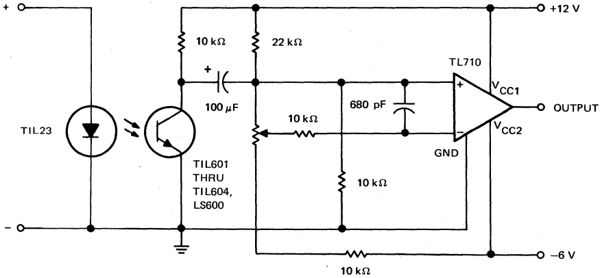
FIGURE 3—OPTICALLY COUPLED AMPLIFIER
