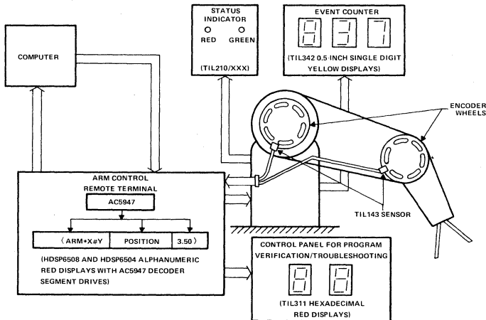
Figure 1. Robot Arm Application
