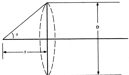
f IS FOCAL LENGTH FIGURE 7. Typical Optical Collection Configuration
