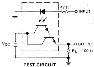
FIGURE 1—SWITCHING TIMES
