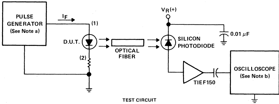
FIGURE 1—RADIANT POWER OUTPUT MEASUREMENT
