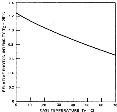
FIGURE 3. Relative Photon Intensity versus Case Temperature
