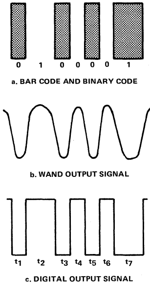
Figure 3. Digital Output Signal From Bar Code
