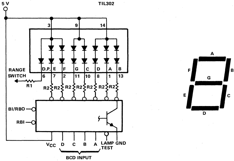
a. SEVEN-SEGMENT DISPLAY INTERFACE
