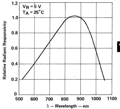
RELATIVE RADIANT RESPONSIVITY vs WAVELENGTH
