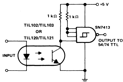
(a) NON-INVERTING FUNCTION
