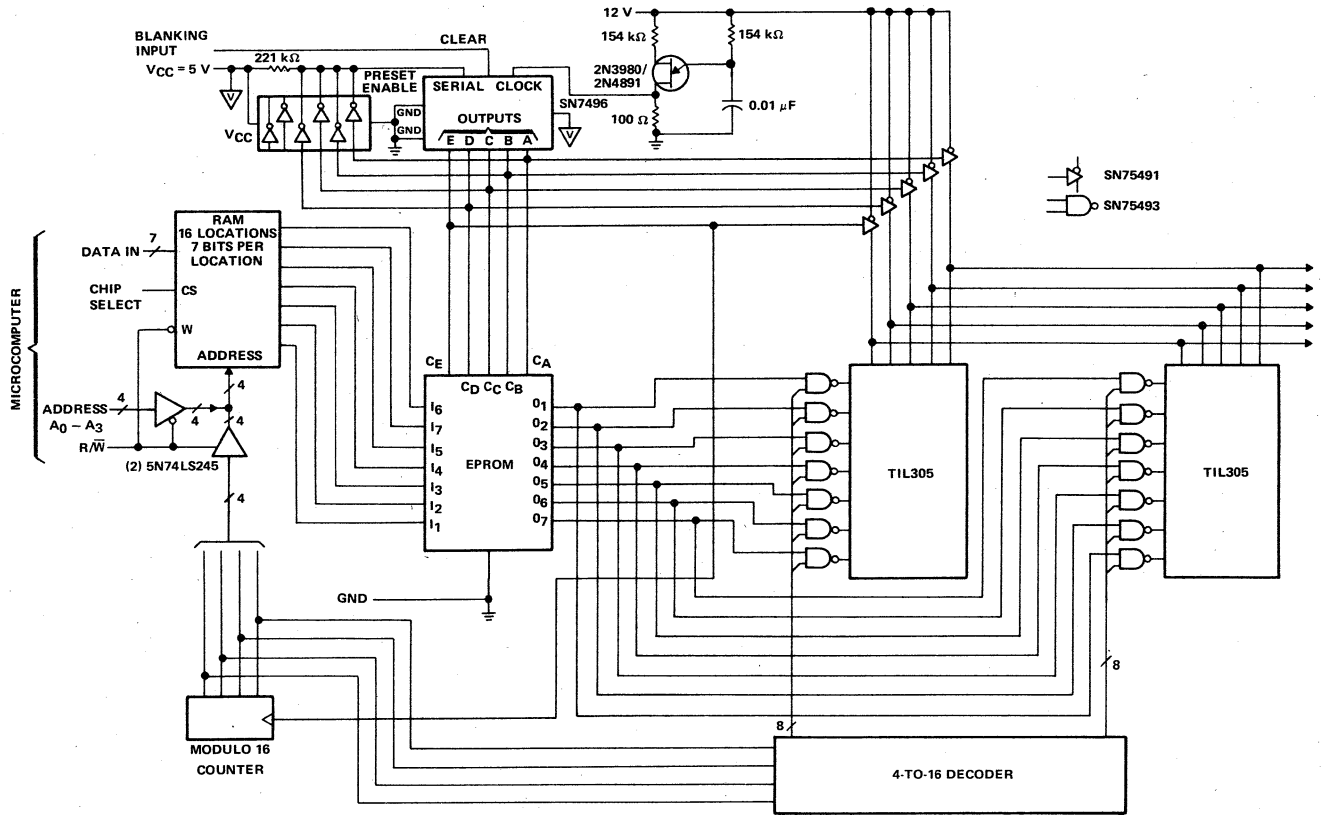
Figure 5. 16-Character Display
