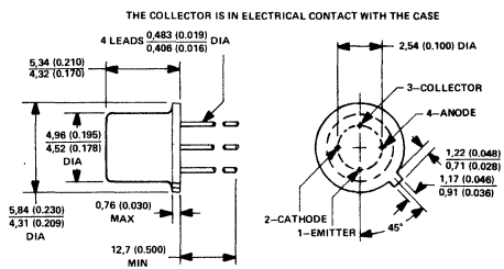
FIGURE 6. Dimensions of the TIL120/TIL121
