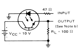
TEST CIRCUIT
