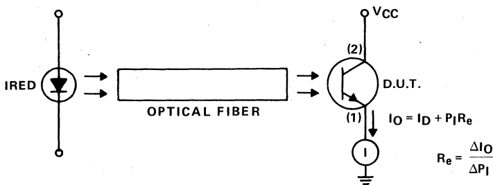
FIGURE 1 — TEST CIRCUIT FOR RADIANT RESPONSIVITY
