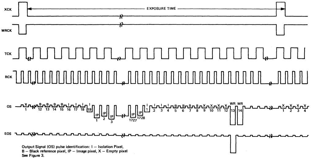
FIGURE 1 – OPERATING INPUT AND OUTPUT VOLTAGE WAVEFORMS
