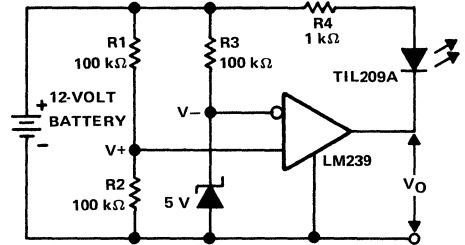
a. SCHEMATIC OF CIRCUIT FOR LOW-VOLTAGE INDICATOR
