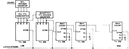
FIGURE 7. Nine-Digit Counter
