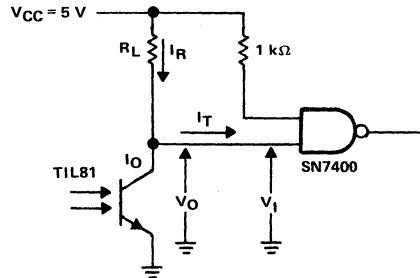
Figure 3. Phototransistor Interface Circuit
