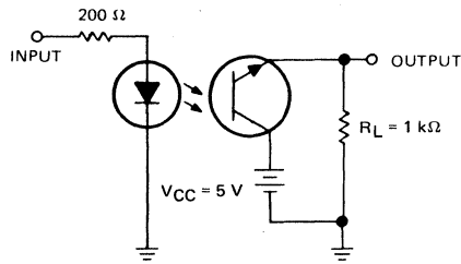
TEST CIRCUIT
