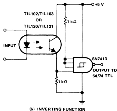
FIGURE 7. Schmitt Trigger Coupling Optocoupler to 54/74 TTL Inputs
