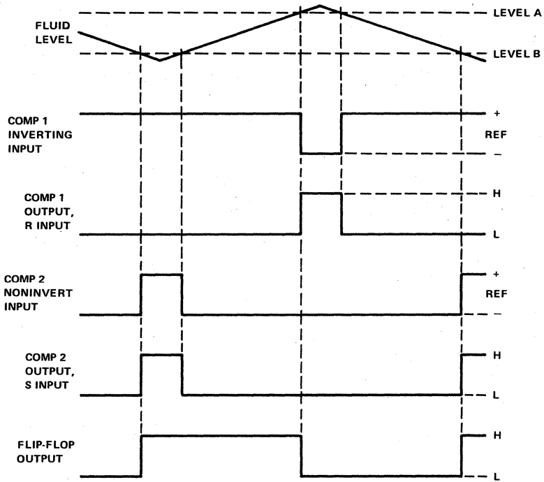
Figure 2. Timing Diagram
