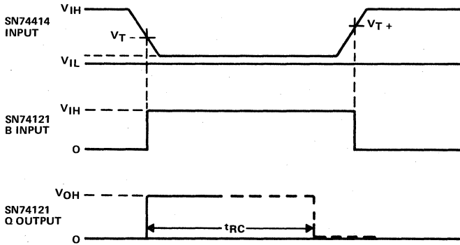
Figure 2. Waveforms
