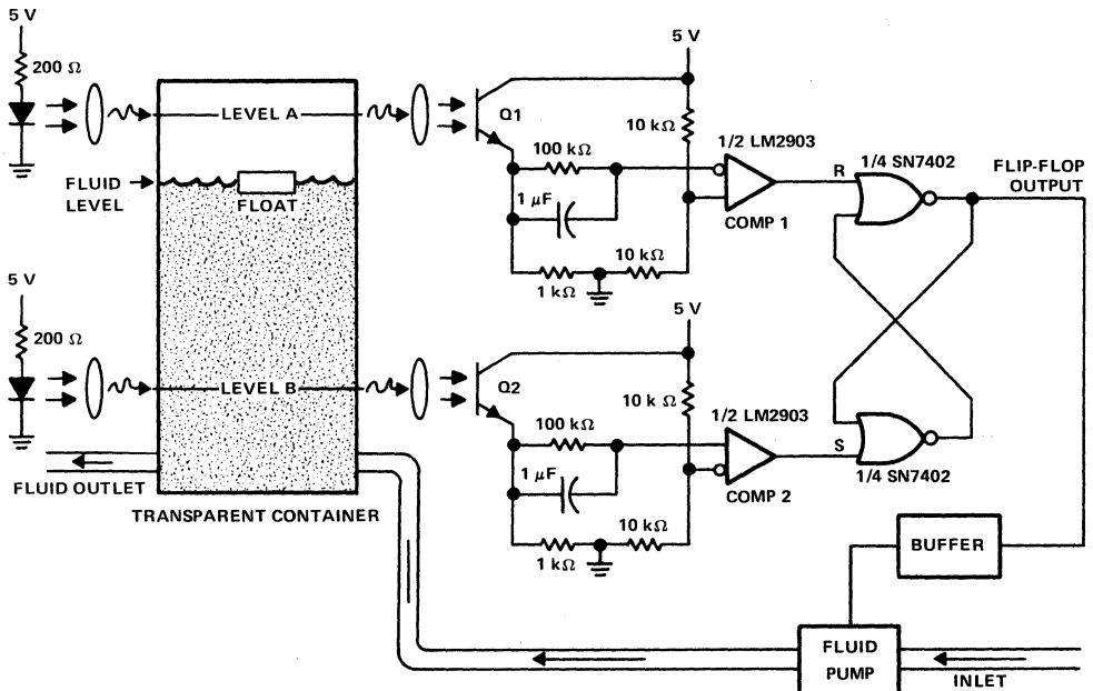
Figure 1. Fluid Level Controller
