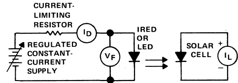
Figure 4. Calibrating the Test Setup
