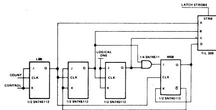
FIGURE 5. 100 MHz Decade Counter Using Texas Instruments Schottky TTL Logic and A TIL308 Display.
