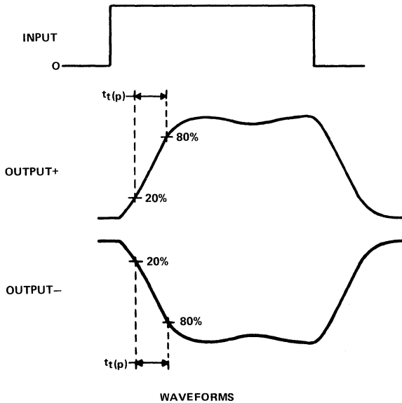
FIGURE 3—SWITCHING TIMES
