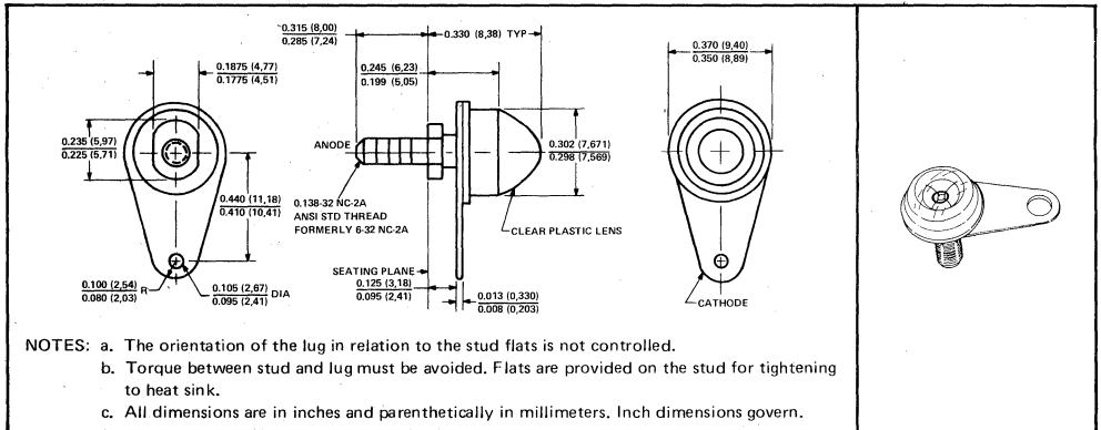
FIGURE 12. Mechanical Specifications for TIES27
