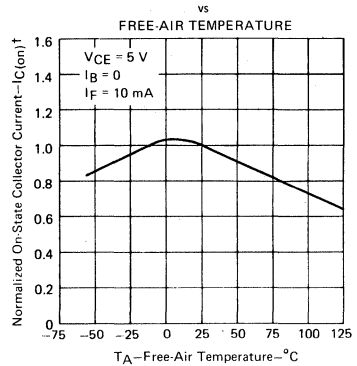
NORMALIZED ON-STATE COLLECTOR CURRENT†
