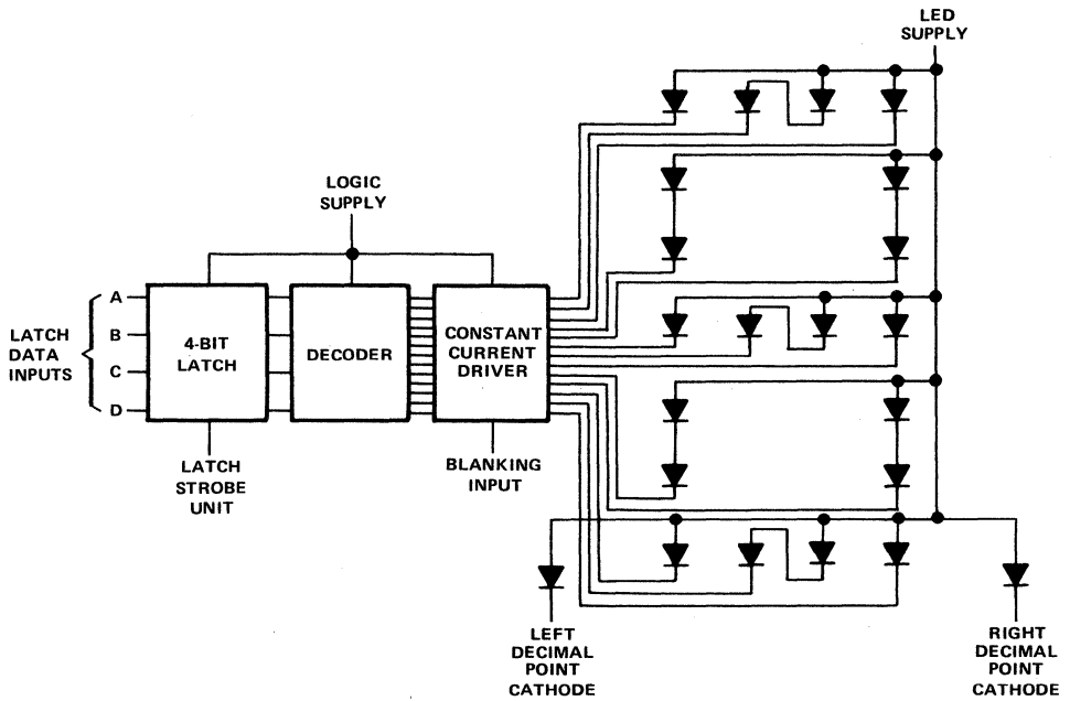
b. SCHEMATIC
