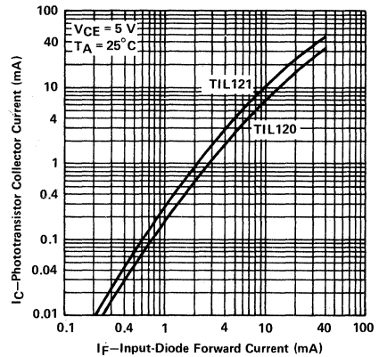
FIGURE 4. Typical Input/Output Current Relationship for the TIL120/TIL121
