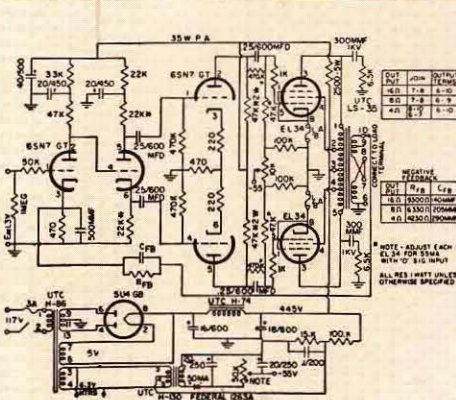
CIRCUIT PROVIDING 60 WATTS, \pm 1 db from 15 cycles to 30 KC ... At 1 watt, \pm 1 db 3 cycles to 80 KC.
