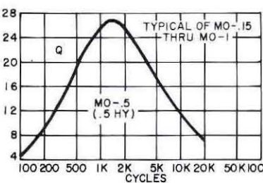
MO CASE \frac{3}{4} \times 1\frac{1}{16} \times 1\frac{1}{16} " high Weight 1 oz.
