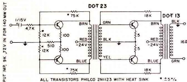
Circuit providing 140 MW, frequency range 300 cycles to 20 KC
