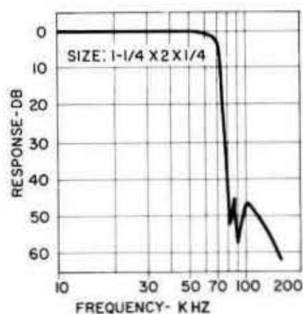
Ultra-miniature low pass filter only 1/4" high. DC to 40 kHz within ± 0.1 db, within 1 db to 60 kHz, 3 db to 70 kHz. Attenuation of at least 40 db above 81 kHz. Source and load 1K ohms. MIL-F-18327C. Wt. 1.2 ounces.
