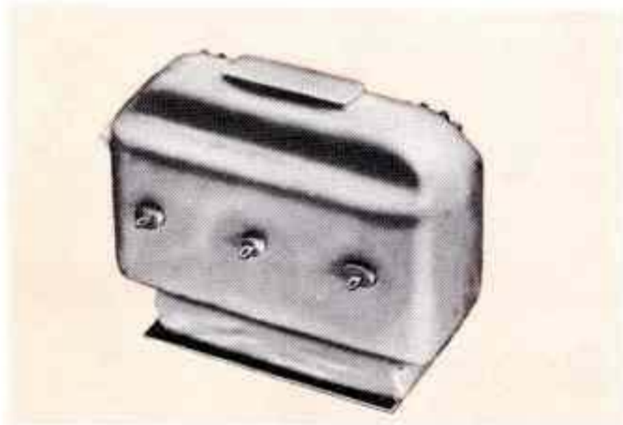
High temperature plate transformer. Primary 208 V., 3 phase 380/1000 Hz to 5100 V./leg, 1400 V. A. 200° C. MIL-T-27C; 6 x 3 x 4½", 6 lbs.
