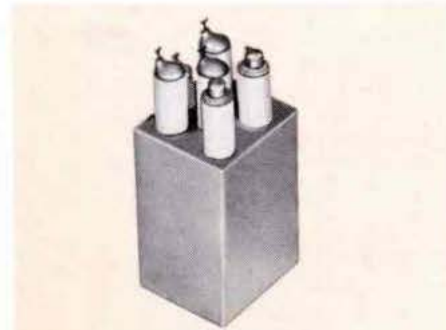
Gaussian wave shape pulse output. Input 2 KV, 3.5 \mu sec. Output 2.5 KV-5A., 80 kHz rate. Corona free-35,000 feet. MIL-T-27C; 1 5/8 x 1 5/8 x 3 3/8, 1 lb.
