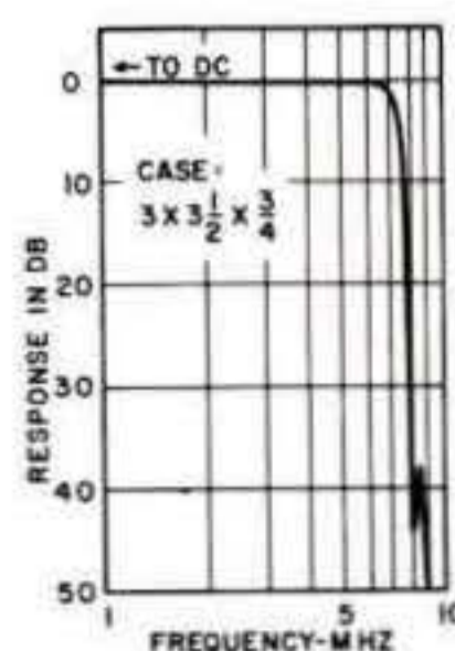
Low pass filter, 6 MHz. DC to 6 MHz within ± 0.1 db. Attenuation at least 40 db at 8.5 MHz and higher. Source and load 75 ohms. Wt. approx. 8 oz.
