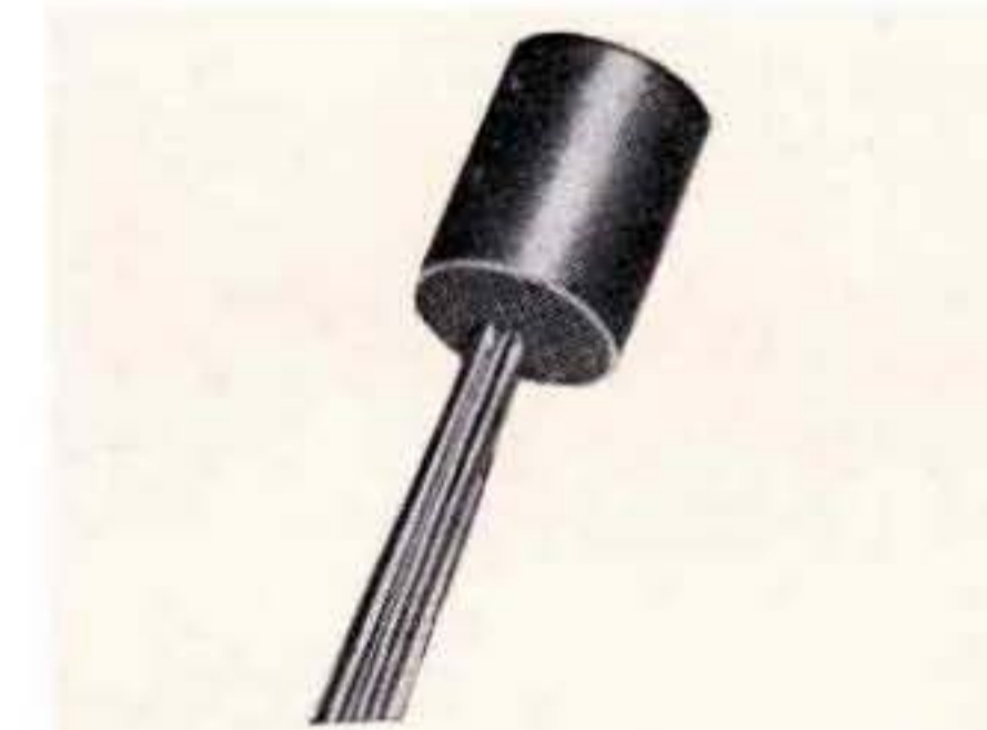
DO-T Pulse Transformer, width 150 \mu sec., ratio 1:1:1. Transistor output to gating circuits. -65°C to 105°C. MIL-T-21038B. 5/16 Dia. x 13/32, 1/10 oz.
