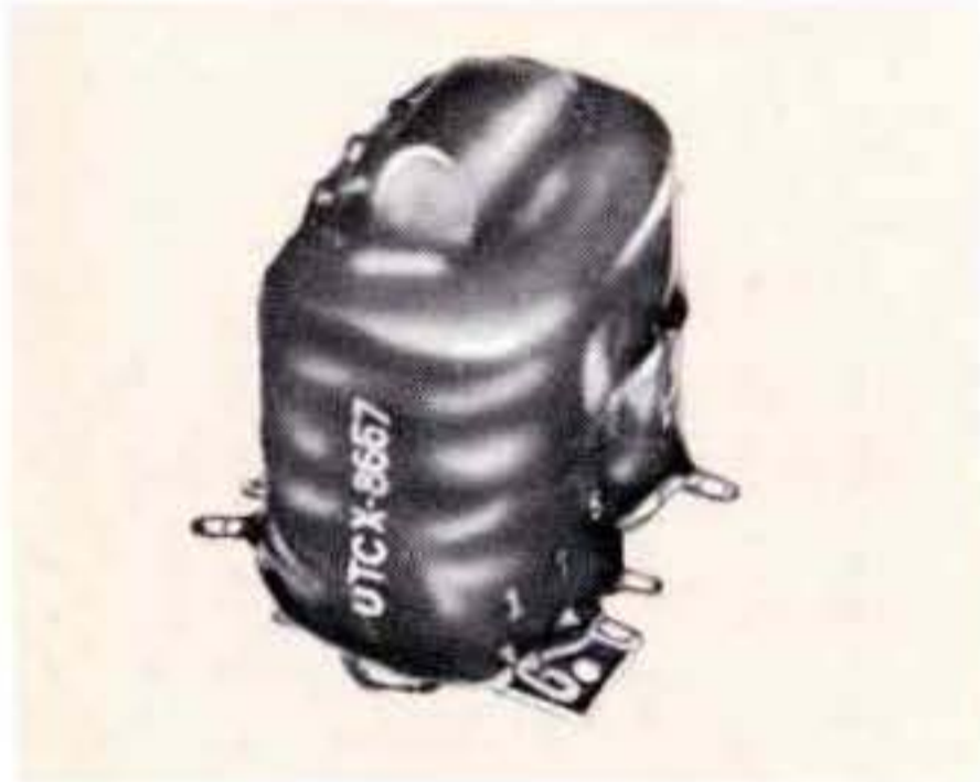
Output to 2J42 magnetron. Input 1300 V.-50 ohms. Output 6.5 KV to 1200 ohms and .6A. bifilar filament winding. .15 \mu sec., 1000 PPS. Trigger winding. MIL-T-27C Grade 5; 1 1/2 x 2 1/2 x 2 3/4, 10 oz.
