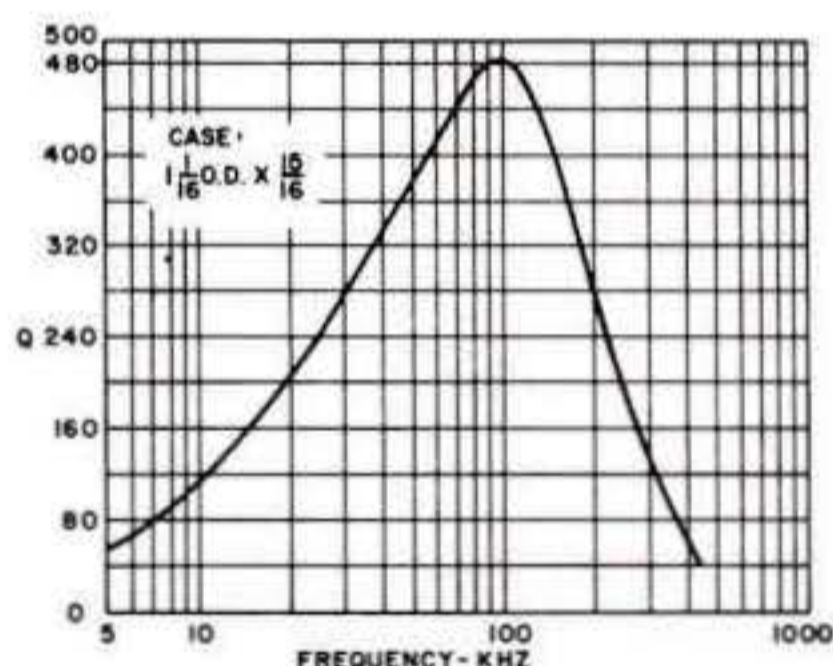
High Q, 5 millihenries inductor. High Q in the 10 kHz to 300 kHz frequency range. Grade 4, MIL-T-27C. Weight approximately 1.5 oz.
