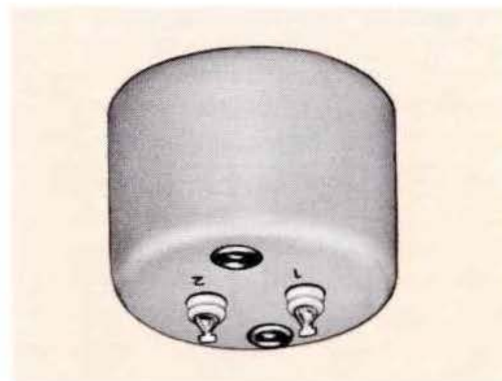
Constant 20 millihenries inductor. Inductance variation less than 2% from 0.1 to 500 V at 100 kHz. Q at 1 volt 100 kHz greater than 100. Case size: 1 7/8 O.D. x 1 3/16" high. MIL-T-27C.
