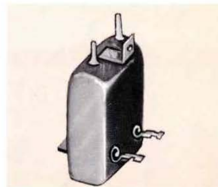
RF saturable inductor. 2 MA DC for sweep from 17 MHz to 21 MHz. MIL-T-27C; 2 oz.
