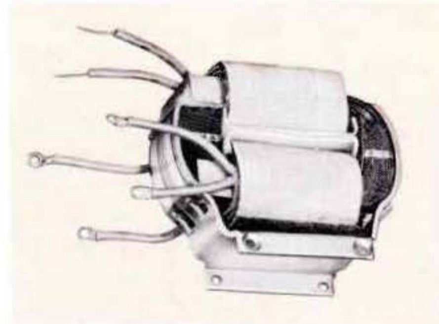
Output to magnetron. Input 6 KV peak 2.5 \mu sec. or .5 \mu sec. Output 28 KV-27 A. peak and 14.2A. bifilar magnetron filament winding. MIL-T-27C, 170° C.; 2 5/8 x 5 3/8 x 4 5/8, 7 1/2 lb.
