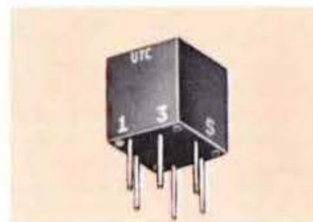
Molded, pin terminal unit. Packaging developed for and fully in accord with Micromodule program. Item shown is 10K ohms CT to 10K ohms CT, 100 mw from 400 Hz to 20 kHz. Life tested per micromodule requirements with no failures.
