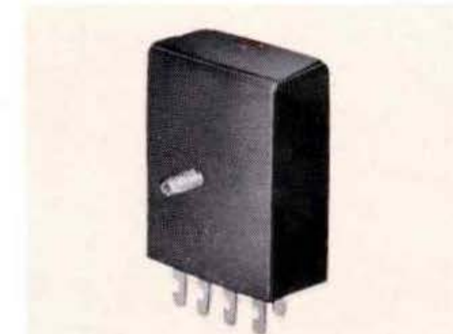
Ferrite core pulse transformer. 30 V. . . . three windings, 5-10 \mu sec. Couples to magnetic tape head for high speed read in and out. Hiper-malloy shield. Commercial; 5/8 x 1 1/4 x 1 5/8, 2 oz.
