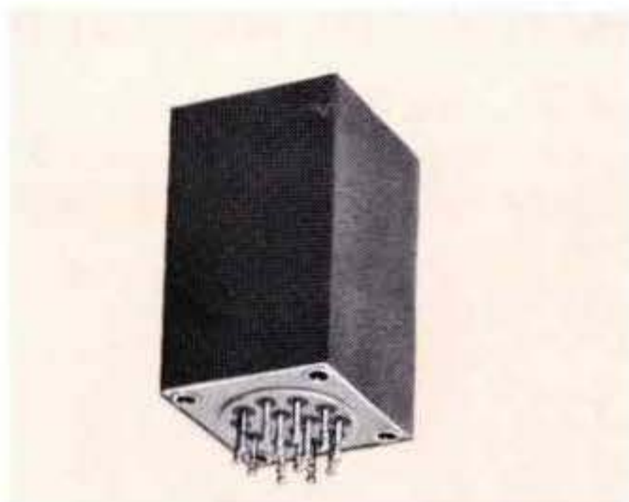
Two self saturating magamps in one case. Output 250 V. into 750 ohms. Power gain 135,000. MIL-T-27C; 2 x 2 x 2½, 12 oz.
