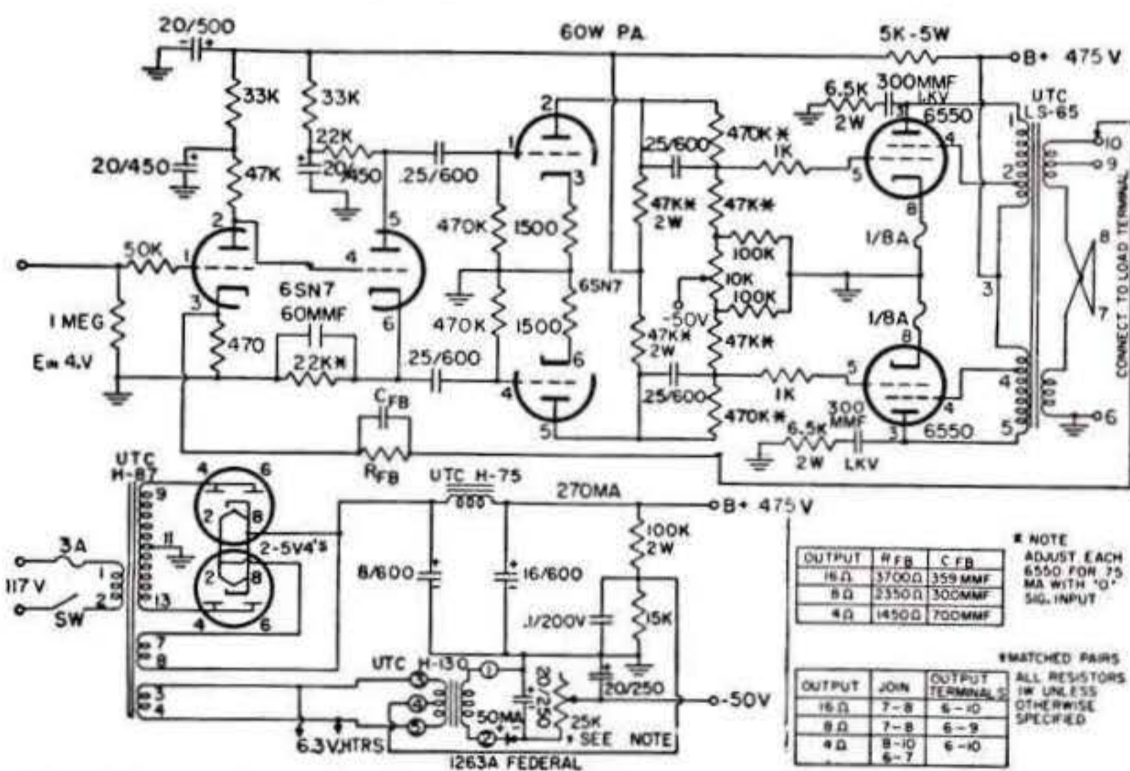
CIRCUIT PROVIDING 60 WATTS, ± 1 db from 15 Hz to 30 kHz ... At 1 watt, ± 1 db 3 Hz to 80 kHz.
