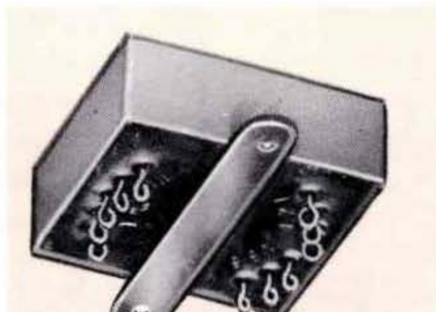
Instrument reference transformer. Input 50 V. 400 Hz. Three 5 V.-.025A. Outputs to .05% accuracy. Saturation characteristics and DCR balance to 3%. MIL-T-27C; 1½ x 1¾ x ¾, 2 oz.
