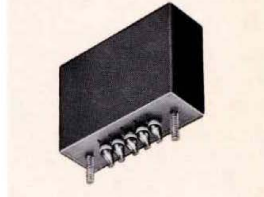
Saturable reactor. Input 50 V.-60 Hz. Output 10 V., 4 MA DC control current. MIL-T-27C; 7/8 x 2½ x 1½, 6 oz.
