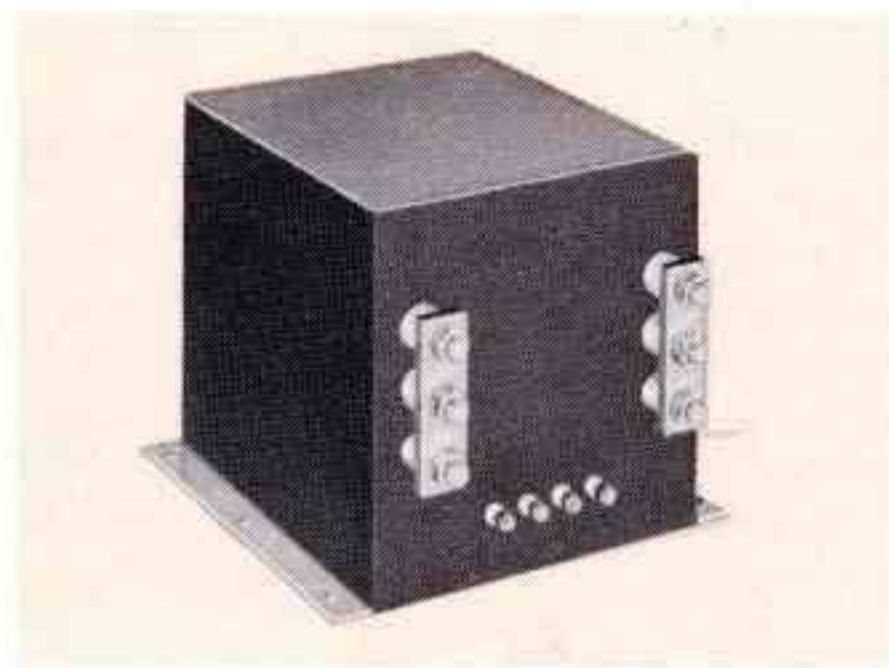
High current filament transformer. Primary 140/156 V., 47/63 Hz to 1.8 V.-1070 A. Current limiting through separate primary reactor, MIL-T-27C; 10 x 10 x 11½". 150 lbs.
