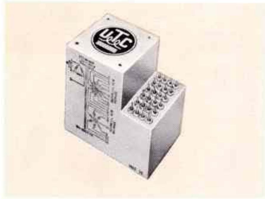
Power transformer; 3 phase input, one 12 phase and one 6 phase output. 25 VA total. MIL-T-27C, Class R. Size: 2 x 3 x 3".
