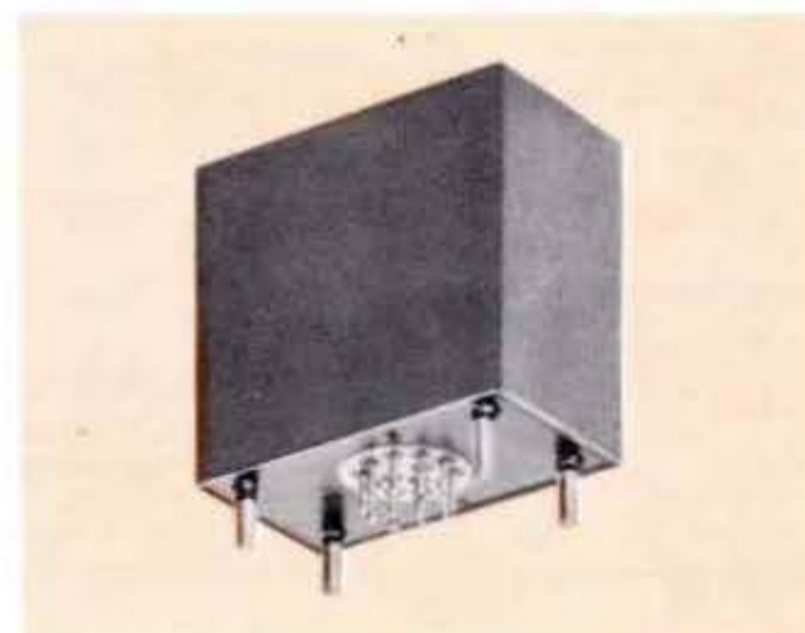
Bolometer transformer. Primary 10 ohms, secondary 530K ohms, 230:1 ratio, response from 1/2 Hz to 25 Hz. 120 db magnetic shielding, to 25 Hz. 120 db magnetic shield-plus full electrostatic shielding.
