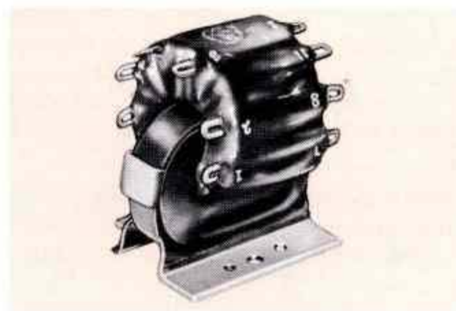
High temperature power transformer. Primary 115 V., 320/1000 Hz to four 6.3 V. and one 475 V. secondaries. 200° C. MIL-T-27C; 2¼ x 2 x 2", 9 ounce.
