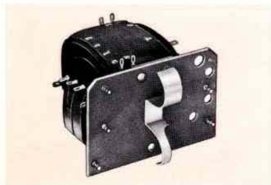
Scope power transformer with board for rectifiers. Primary 115 V., 400 Hz to two 14 KV filament windings, one 6.3 V. low capacity filament winding, 4.5 KV and 1.75 KV high voltage windings. 25 KV hipot when in oil; 2¾ x 3½ x 2½", 1¼ lbs.
