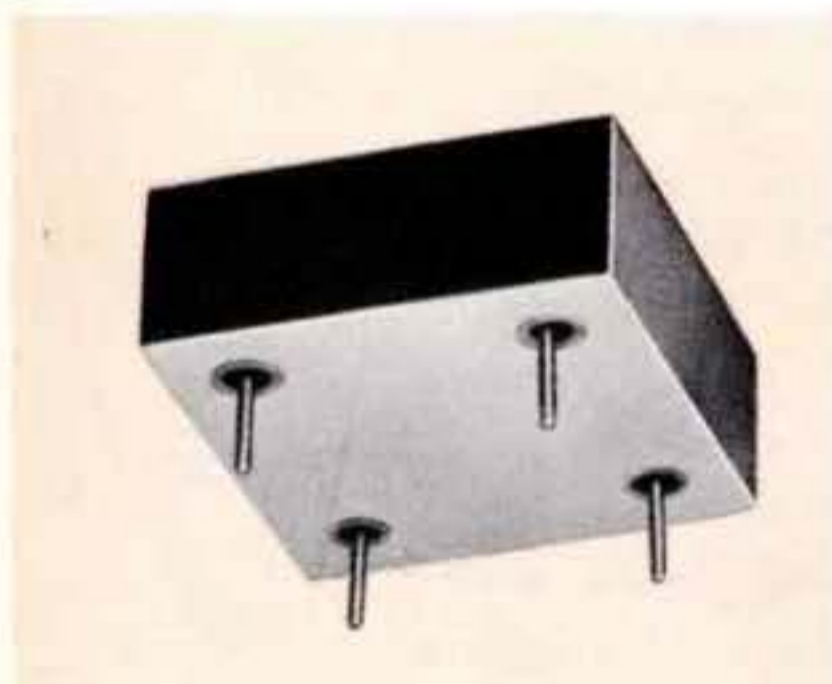
Flat low frequency 50 henries inductor only .400 high. Q of 10 at 100 Hz, DCR 2360 ohms. Grade 4, MIL-T-27C.
