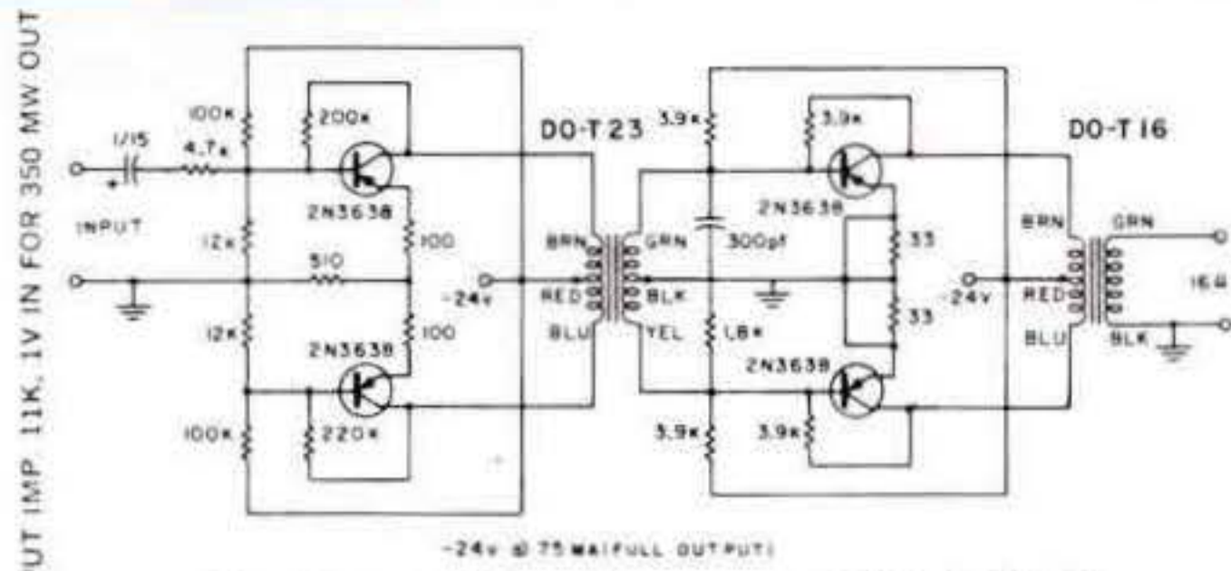
Circuit providing 350 mw, frequency range 900 Hz to 160 kHz
