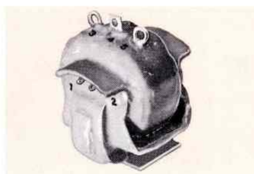
High voltage filament transformer. Primary 115 V., 380/1600 Hz to 5 VCT-10 A., 21 KV hipot. 160° C. MIL-T-27C Grade 5; 2¼ x 2½ x 2¼", 10 ounce.
