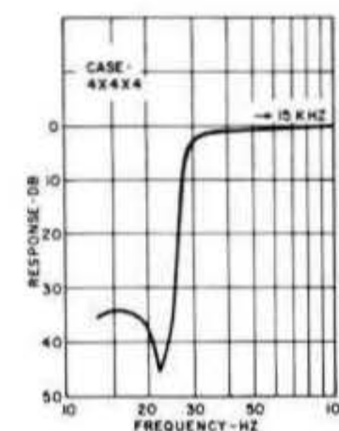
High pass filter, 30 Hz, used to eliminate from the output, 25 Hz sine wave pulses which control automatic programming on audio tracks of music tapes. Flat to 1 db from 50 Hz to 15 kHz, within 3 db to 30 Hz. Attenuation of at least 35 db from 25 Hz to 20 Hz. Source and load 600 ohms. Wt. approx. 6 lbs. MIL-F-18327C.
