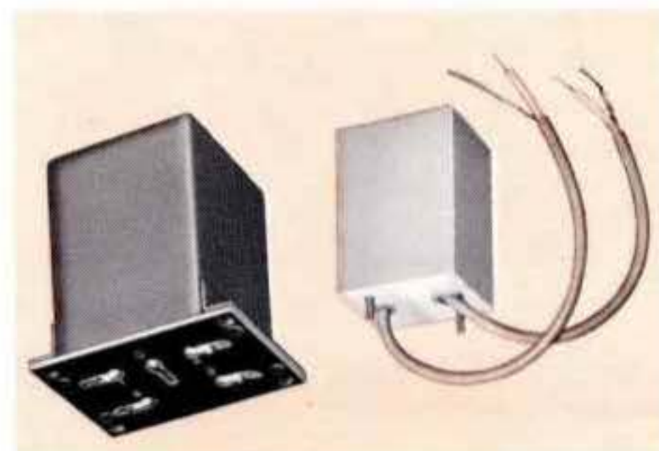
Low distortion 2.5 KW output transformer, PP 450 TH's 18,500 ohms CT to 24/6 ohms, 20 KV hipot. 520 lbs.
