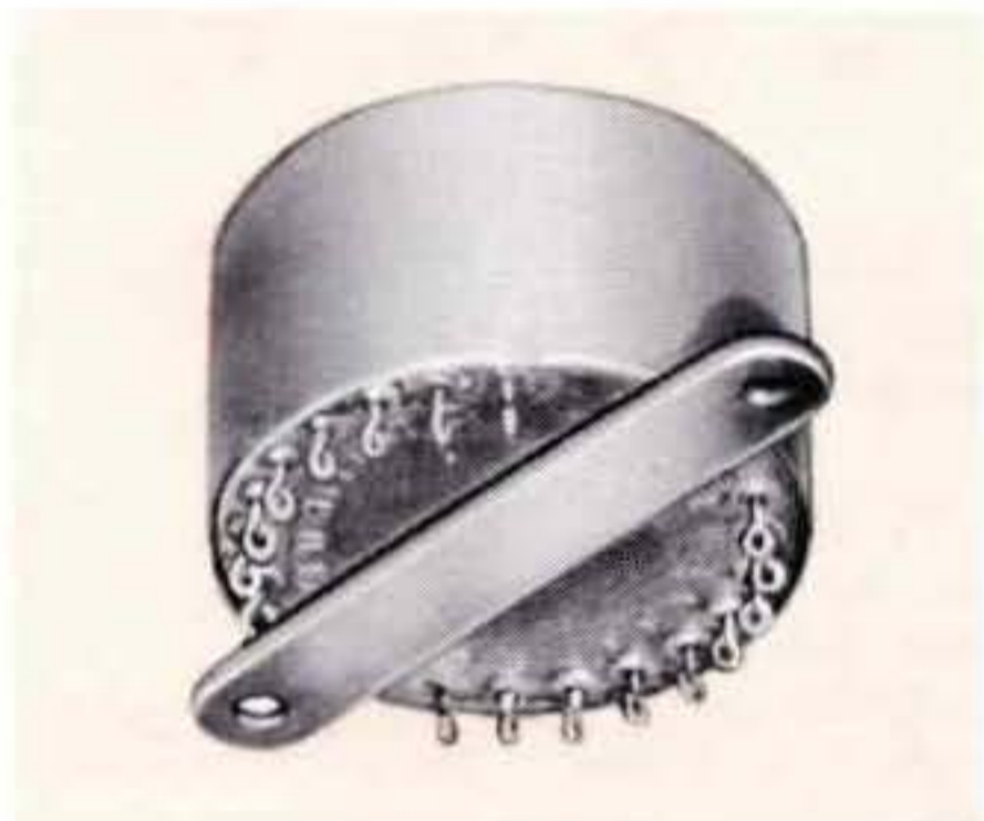
Multi Control Magamp. Power gain 400,000. Control Current. .00003A. Output 25 V. DC into 1K. Six power windings, bias, feedback, and two control windings. MIL-T-27C; 2¼ dia. x 1¼ high, 8 oz.
