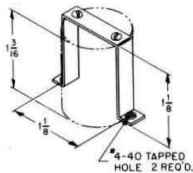
Ouncer chassis mount bracket
