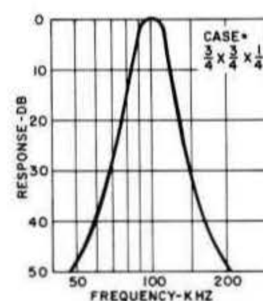
Ultra-miniature 100 kHz band pass filter only 1/4" high. Within 3 db 90 kHz to 110 kHz. Attenuation of at least 45 db at 50 kHz and at 200 kHz. Source and load 10K ohms.
