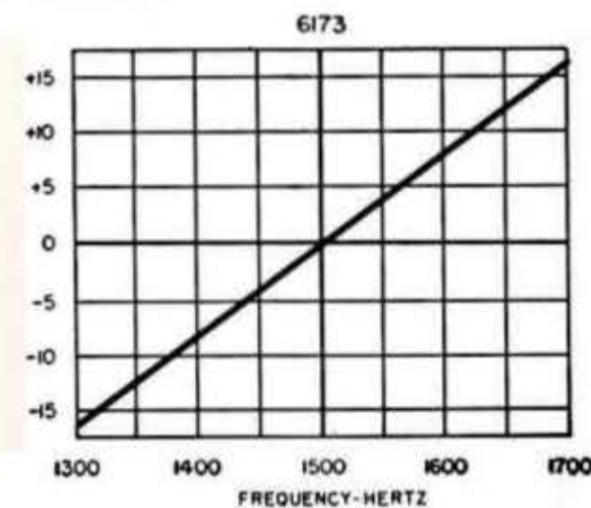
UTC high Q discriminators provide exceptional amplification and linearity. Values are volts. 1 1/16" x 1 3/8" x 3".
