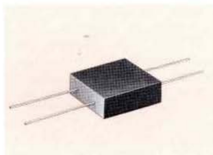
Ultra-miniature 100 kHz band pass filter only 1/4" high. Within 3 db 90 kHz to 110 kHz. Attenuation of at least 45 db at 50 kHz and at 200 kHz. Source and load 10K ohms.
