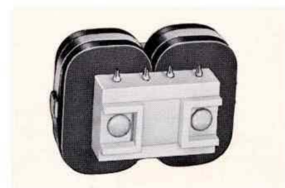
Molded High Temperature, High Voltage Transformer. Input 115 V 400 Hz, output 3400 V, 80 ma DC. Corona free molded terminals. MIL-T-27C Grade 5, Class T (170°C), 3¾ x 2¾ x 2½", 2 lbs. 10 oz.
