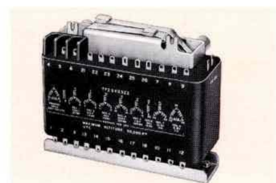
Molded Power Transformer 3 Phase. Input 200V, 380-420 Hz Electrostatic Shield, 8 output windings. 26 terminals. MIL-T-27C, Grade 2 Class S. Max. Alt. 50K Ft. Size 6 x 2½ x 5", 8 lbs.
