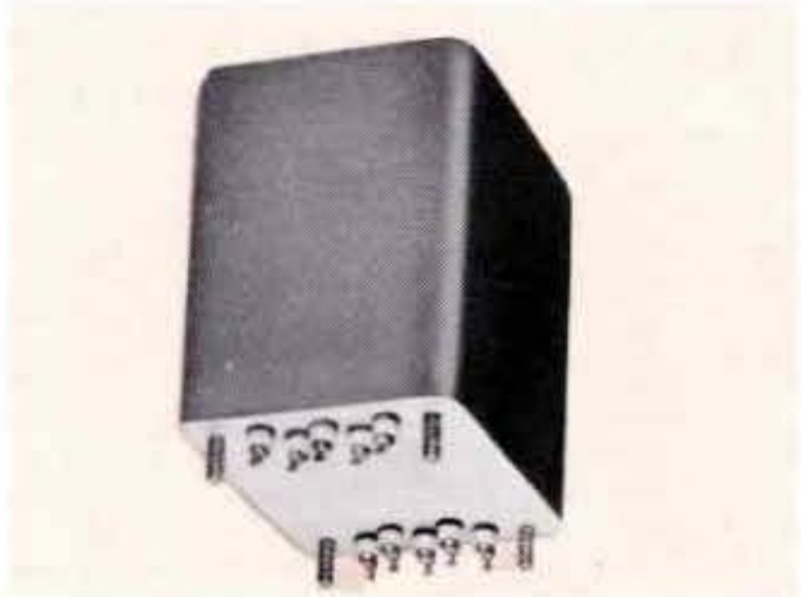
Magamp for 50 watt, 60 Hz servomotor. Two control windings. One feedback winding, one power winding, diode panel. Power gain 100. MIL-T-27C; 30 lbs.
