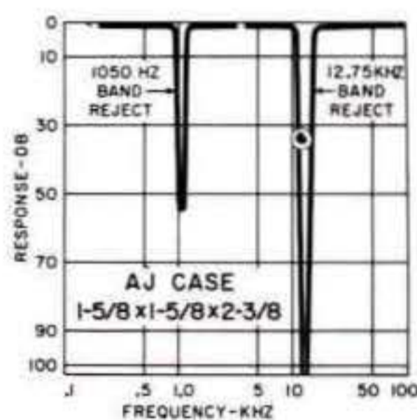
Band reject filters (two shown). The 1050 Hz filter has 50 db attenuation at center frequency and is only 3 db down at 950 and 1150 Hz. The 12.75 kHz filter has more than 100 db attenuation at center frequency and is only 3 db down at 10.8 kHz and 15 kHz. Source and load for each filter 600 ohms, both are MIL-F-18327C. Wt. 0.7 lbs.
