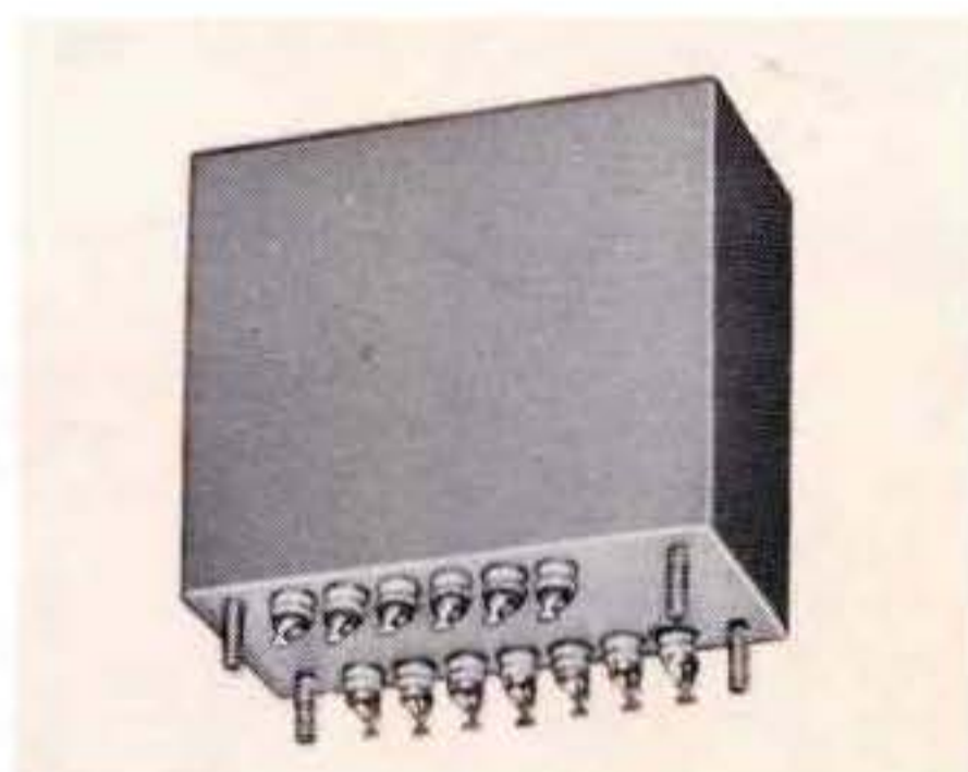
Servo reference transformer. Input 120 V., 380 to 420 Hz. Output ratios under load held to .005% tolerance. Phase shift .05° max. MIL-T-27C; 2¼ x 1¾ x 2, 12 oz.
