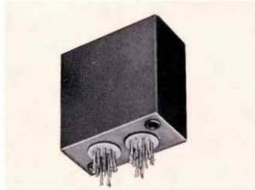
Precision reference transformer. Input 14 V., 400 Hz. Twelve secondaries held to low phase shift and .1% tolerance MIL-T-27C; 1¾ x 2 x 1¾, 4.5 oz.
