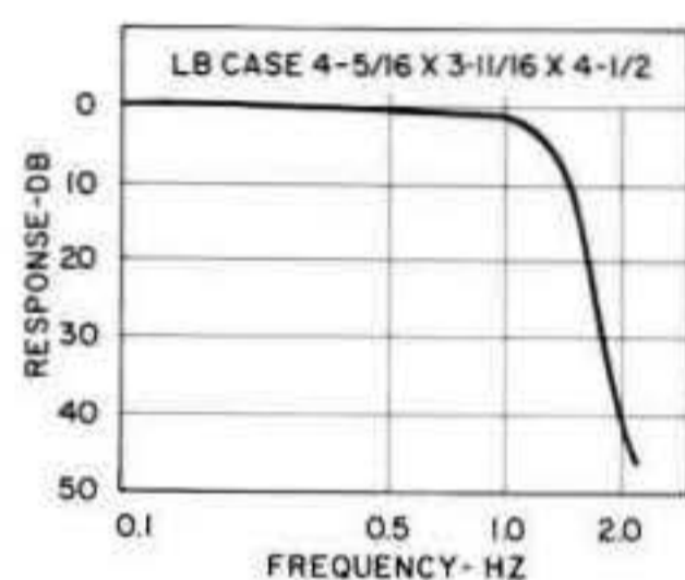
One Hz low pass filter. Flat to 1 db up to 0.75 Hz, within 2 db up to 1 Hz. Attenuation of at least 40 db for frequencies above 2 Hz. Source and load 10K ohms. MIL-F-18327C. Wt. 6 lbs.
