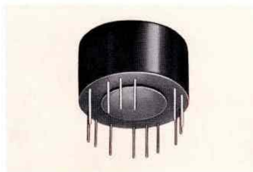
Self-saturating inverter transformer; 100 V DC input. Frequency of oscillation 20 kHz. MIL-T-27C, Class T. Size: 1.25 Dia x .60 H, PC mounting.
