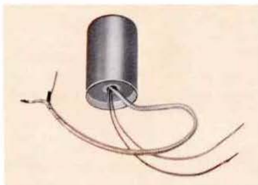
Microphone input transformer, double drawn hipermalloy shields. Shielded cable leads. Ratio 100:1. 1 5/16 Dia. x 1 1/32" high. Inductance greater than 1000 Hys. at 60 Hz.
