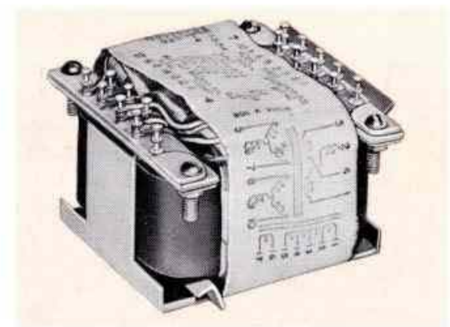
230° C. power transformer. Primary 115 V., 3 phase, 300/420 Hz to 200 V. and 20 V. secondaries, 525 V.A. 230° C. operating; 2¾ x 3 x 2", 1.8 lbs.
