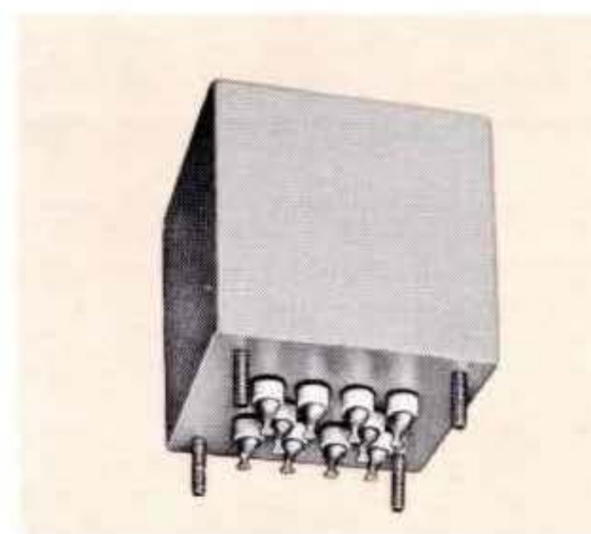
High voltage, constant inductance, tapped inductor. 16 millihenries, 8 kHz, inductance variation less than 1% from 1 volt to 1600 volts. Q greater than 40 at 1600 volts. Case size: 3 1/8 x 3 1/8 x 2 3/4" high. Grade 4, MIL-T-27C.
