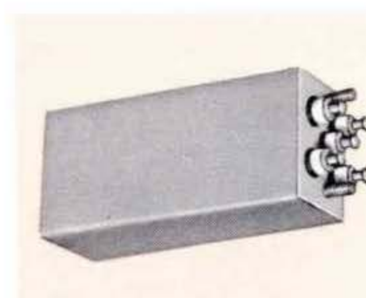
High pass filter, 30 Hz, used to eliminate from the output, 25 Hz sine wave pulses which control automatic programming on audio tracks of music tapes. Flat to 1 db from 50 Hz to 15 kHz, within 3 db to 30 Hz. Attenuation of at least 35 db from 25 Hz to 20 Hz. Source and load 600 ohms. Wt. approx. 6 lbs. MIL-F-18327C.
