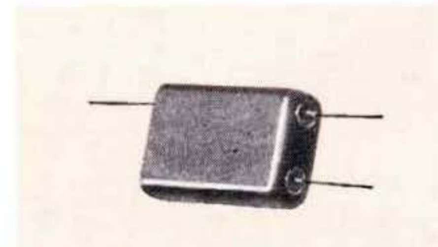
Differentiating pulse transformer. Input 150 V. 40 MA peak, 6 \mu sec., 3000 PPS. Output 30 V. .5 \mu sec. Ferrite core. Rise, droop, and pulse duration held to 5%. MIL-T-21038B, -55° C. to + 100° C.; 5/16 x 5/8 x 1; 7 grams.
