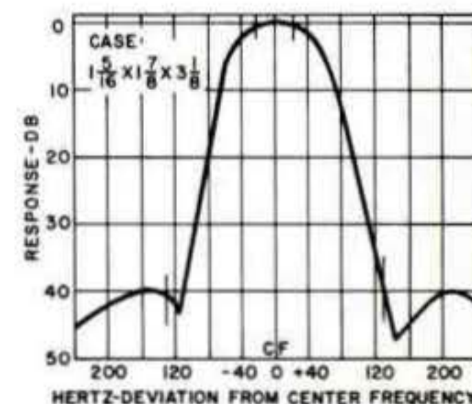
Miniaturized receiving filters, available from 425 Hz to 3315 Hz. Within 3 db at ± 42.5 Hz and attenuation of at least 36 db at ± 130 Hz. Source and load 600 ohms. Wt. approx. 3/4 lbs.
