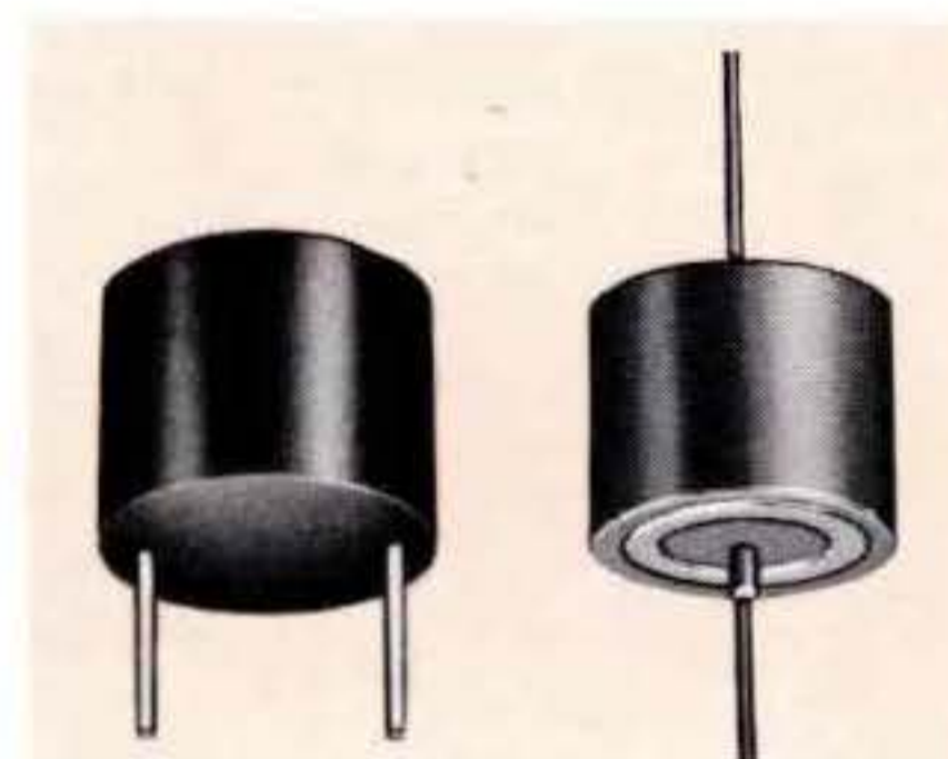
Type FD, 2 microhenry temperature stable miniature inductor. High Q in the 2 MHz to 20 MHz frequency range. Supplied in either epoxy case (23/32 dia x 1/2" high) Grade 5 or metal case (11/16 dia x 9/16" long) Grade 4. MIL-T-27C.
