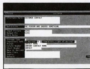
Data Dictionary
