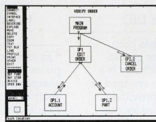
Structure Chart
