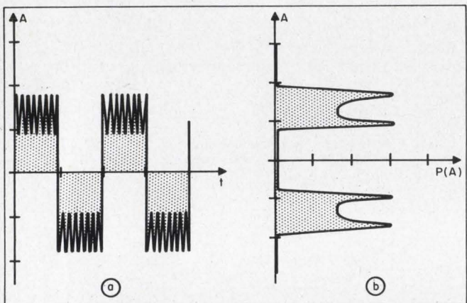
4. Complex waveforms can often be described as the sum of two simpler signals in order to simplify analysis. The sum of a sinusoid and a square wave (a) results in the convolution of their respective density functions (b).
