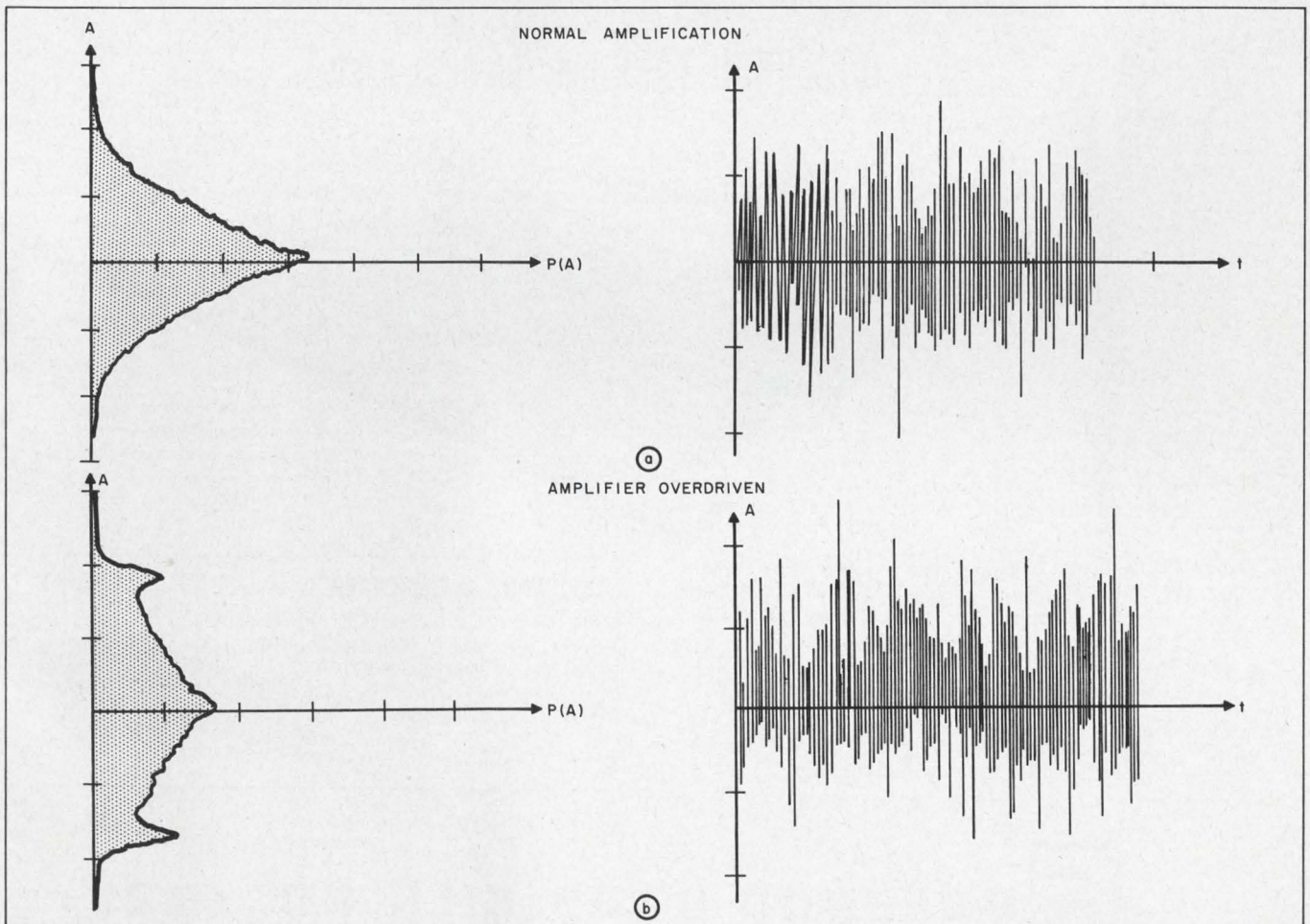
8. Output of a wide-band noise source amplified 40 dB and its probability density are shown in (a). The noise was plotted using a sampling oscilloscope. The same
