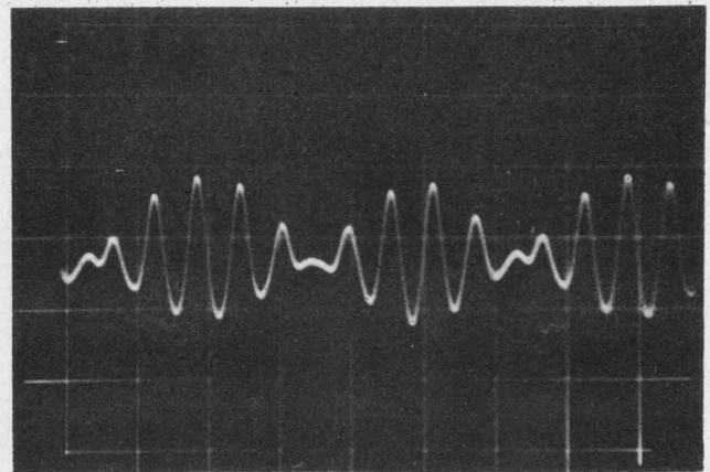
3. Typical output waveform shows the modulation of 3-kHz signal by a 300-Hz one. The vertical scale is -50 mV/cm, and the horizontal, 500 \mu\text{sec/cm} .
