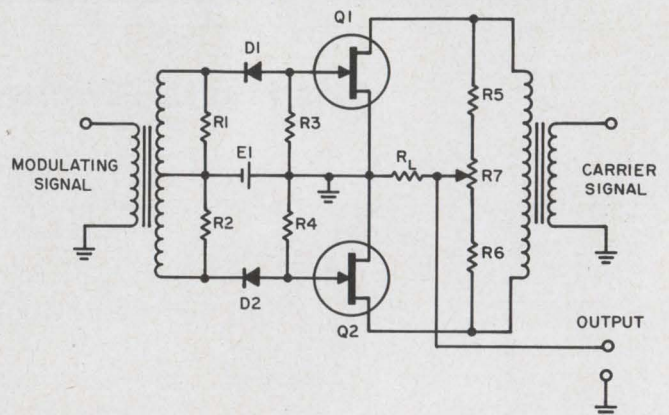
1. FET balanced modulator gives 180° zero-crossing phase shifts as the resistances of Q2 and Q1 are modulated during the first and second half cycles, respectively.
