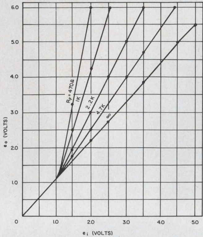
2. The transfer characteristics of the amplifier may be adjusted by varying R_F . The diodes are biased into conduction at the break point of 1 volt.
