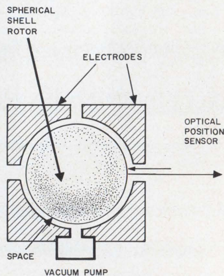
Ball replaces wheel as the rotor in a new electrostatic gyroscope.
