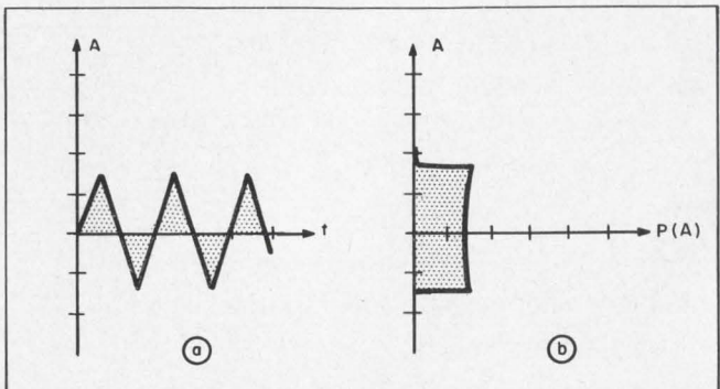
1. The triangular waveform (a) is an equiprobable signal. Its probability density function (b) is a measure of the likelihood of finding the waveform at any particular point within a wave's peak-to-peak amplitude range. Note that (b) has been rotated 90° clockwise from its conventional position.
