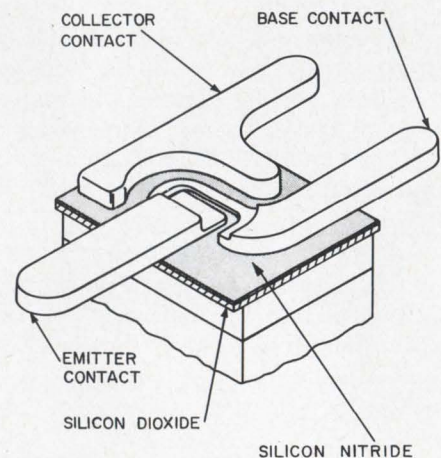
New junction seal shown on epitaxial silicon transistor.
