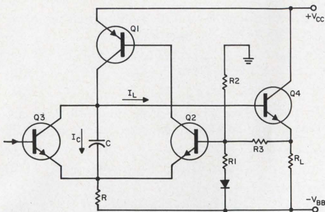
2. Ultralinear current source uses only four transistors. All transistors should be high-speed, high-beta, low-leakage. In particular, Q2 should have high beta at low collector currents. Timing capacitor C should have flat characteristics over the operating temperature range.
