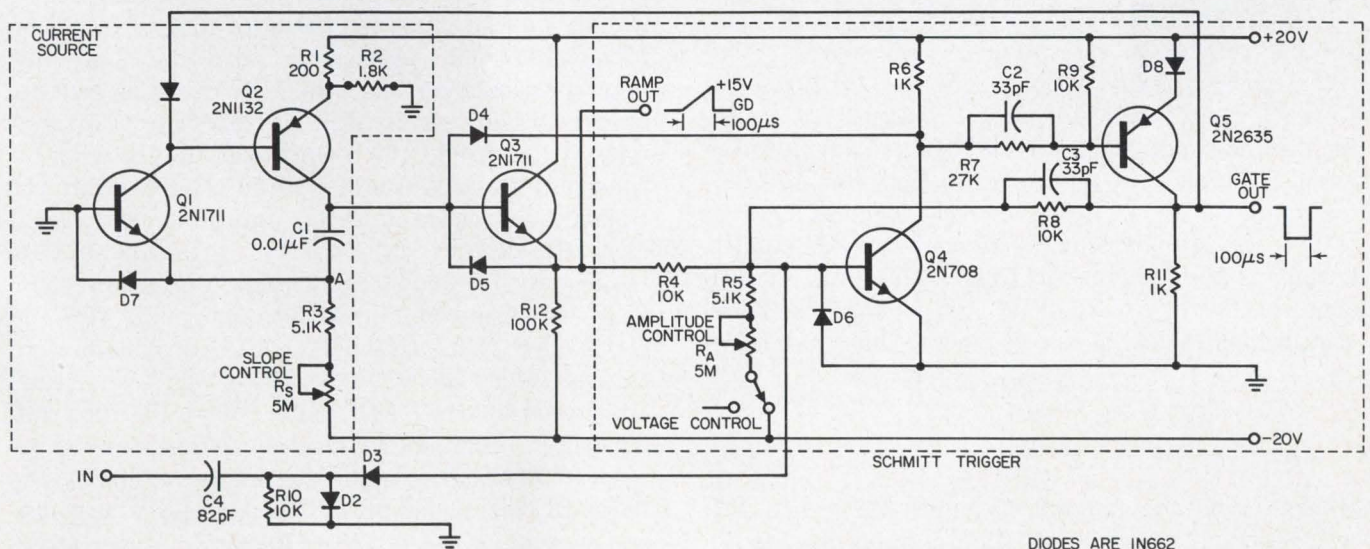
3. Type-1 ramp generator has ramp and gate outputs. Pulse width modulation can be obtained by applying a
