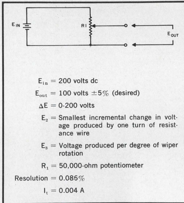
2. Conventional approach for applying a trimming potentiometer for high-resolution applications normally results in selection of a high-resistance unit. Although circuit requirements can be met with such a unit, improper setting can result in circuit failure.
