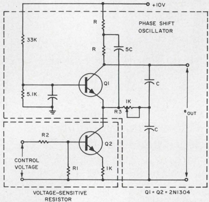
Phase-shift VCO is designed with separate bias and frequency-selecting circuits, to permit the use of transistors with very low betas.
