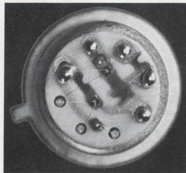
G-E hybrid circuit for multi-vibrator applications.
