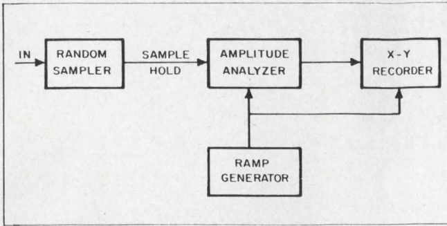
7. Recording of the sample waveshape can be obtained using the setup shown.
