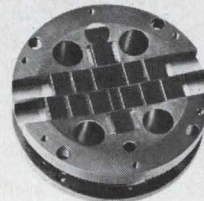
20-element Ge:Hg detector array.
