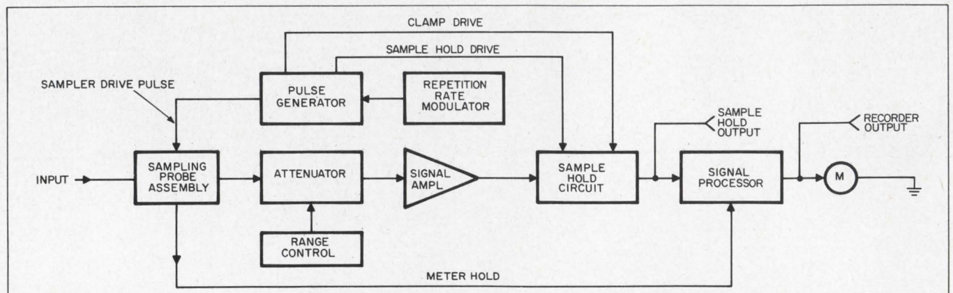
6. Waveform sampling can be accomplished by using a sampling voltmeter. A block diagram of an instrument of
