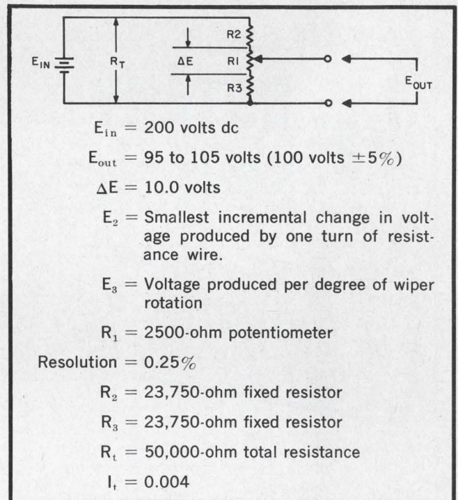
3. Low-resistance trimming potentiometers, when applied properly, can provide high system resolution as well as protection from catastrophic system failure in the event of improper setting.
