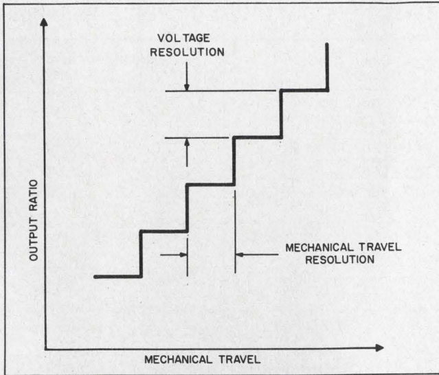
1. Both mechanical and electrical resolution in a potentiometer depend on the diameter of the resistance wire used in the unit.
