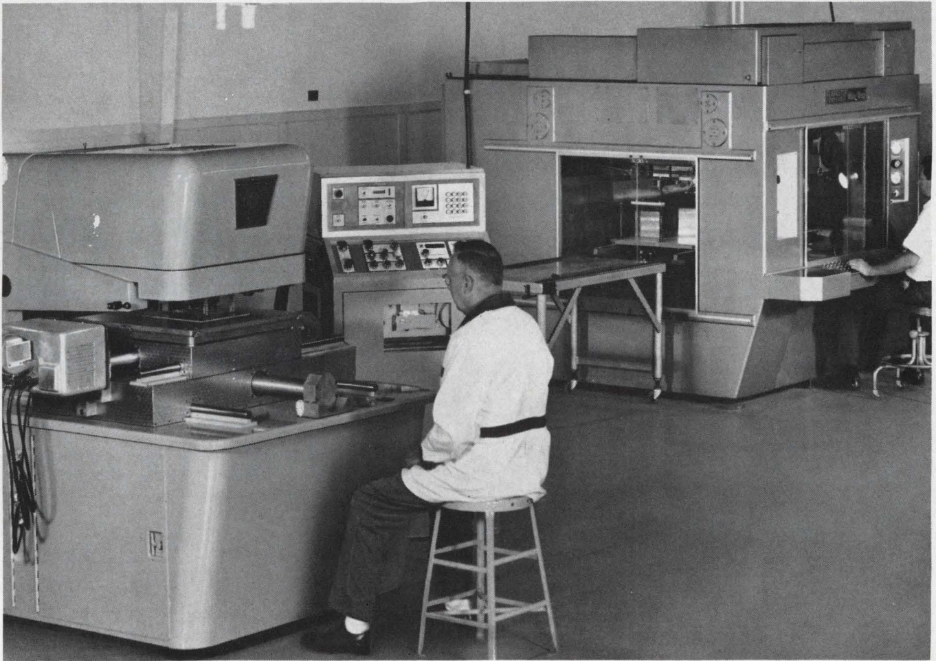
Time on these unique machines is now available through Gardner-Denver contract service. At left is a Grid-Drill machine. One of the automatic "Wire-Wrap" machines is at right.
