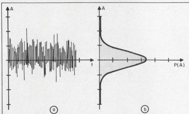
2. Gaussian noise (a) is described statistically by the familiar normal, or Gaussian, distribution curve (b). It is from this description that Gaussian noise gets its name.
