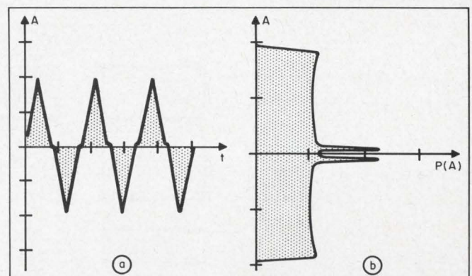
3. Crossover distortion of the equiprobable triangular waveform (a) is easier to detect if the signal's density function (b) is examined.
