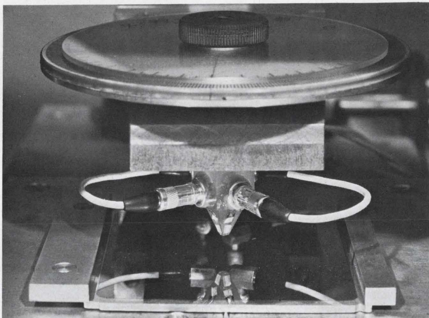
The microprobe can be rotated to test H-B relationships in any direction.
