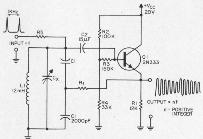
Conventional Q multiplier circuit performs efficient high-order frequency multiplication.
