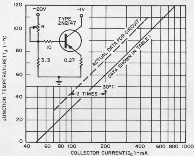
2. Collector current doubles for every 30°C increase in the junction temperature for this circuit. The transfer characteristic is a pure exponential.
