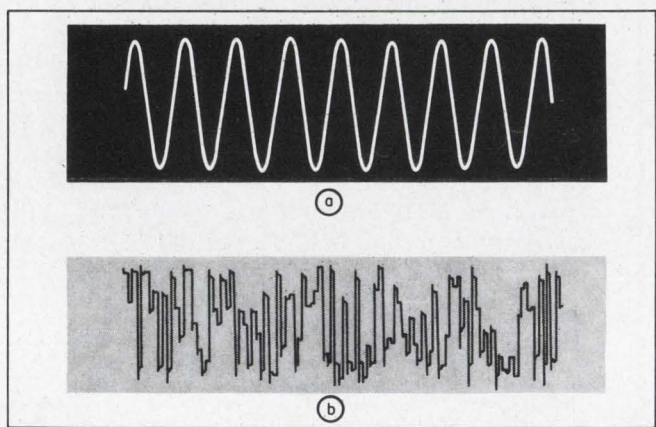
5. Random sampling of a sinusoidal signal (a) results in the collection of samples shown in (b). All time information about the original waveshape is lost but the probability distribution of both waveforms is identical.
