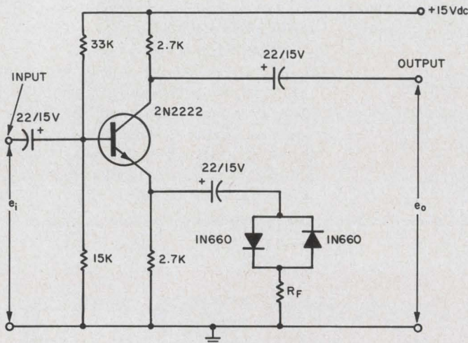
1. Gain of nonlinear amplifier increases with increasing signal levels because of the diodes in its emitter feedback loop.
