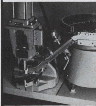
This automatic machine was developed to assemble Clinch-Loc Terminals with speed and flexibility for volume users. With an alternate track any Clinch-Loc Terminal can be used in this machine.
