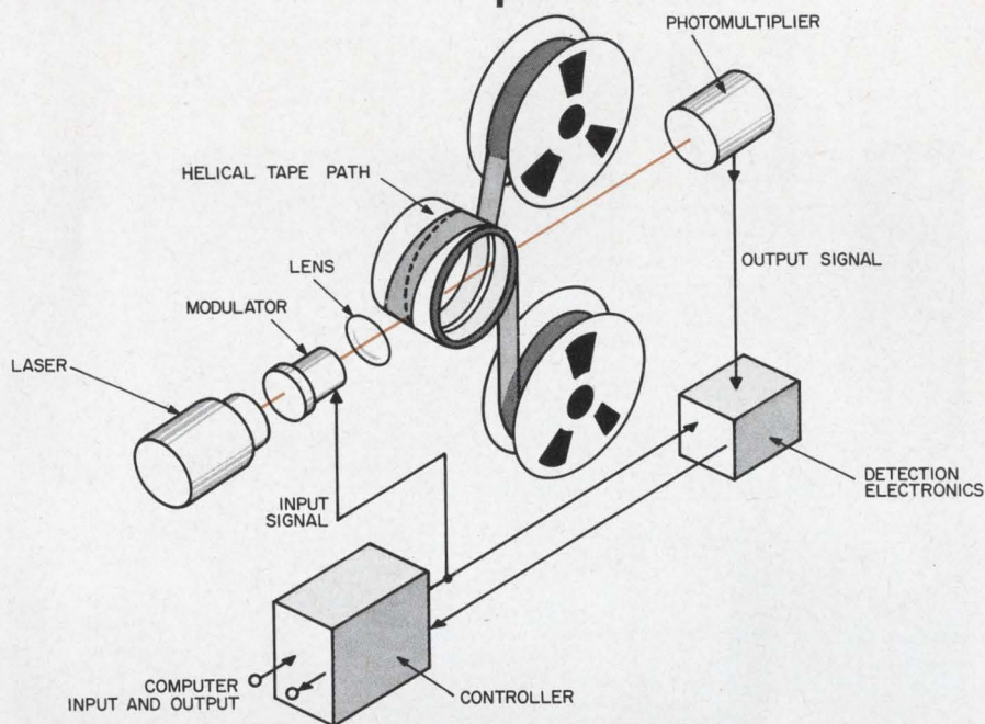
Mass memory process uses lasers to write, check and read records. The laser burns minute data bits on fast-moving opaque plastic tape.
