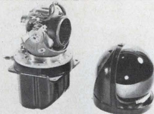
Interceptor IR search/track set.
