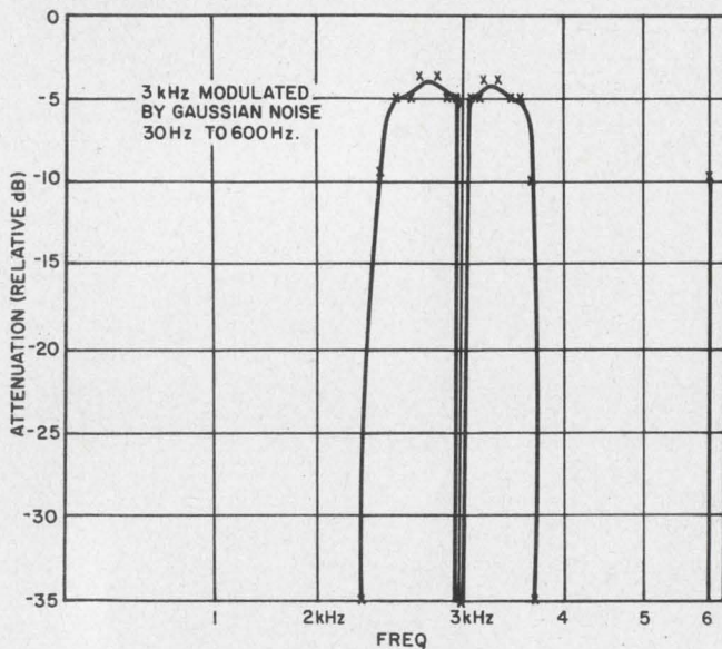
2. Spectrum of noise-modulated signal is essentially flat from f_c - f_1 to f_c + f_1 with a hole at f_c . The swept-frequency bandwidth is 10 cps.
