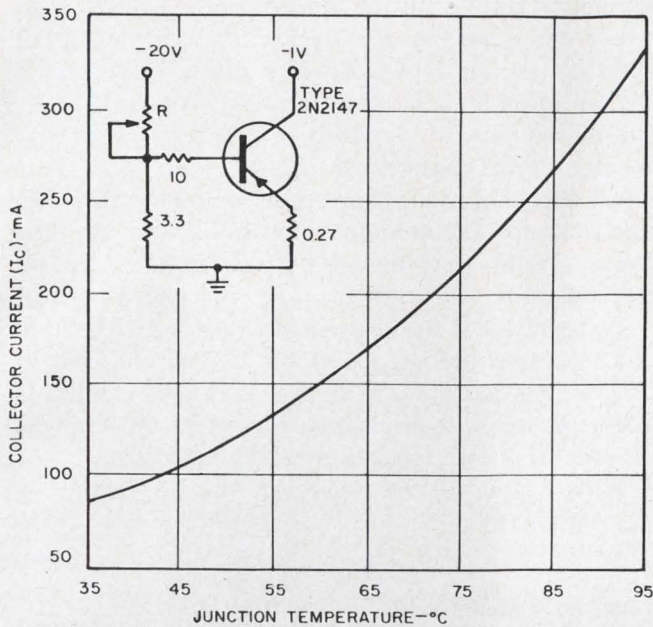
1. The collector resistance of an audio output stage should be small as shown in the above typical output-stage dc bias arrangement. Note the nonlinearity in the collector current vs junction temperature.
