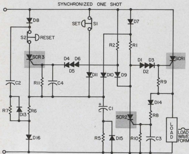
SCRs are used to build a synchronous one-shot useful for dispensing-system and electric welding applications.
