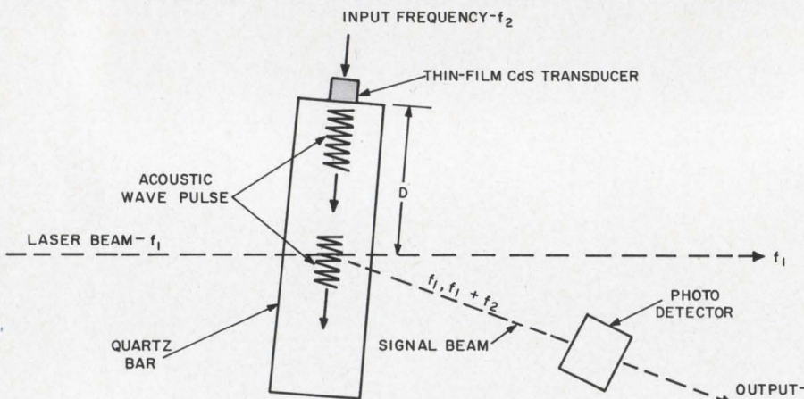
Laser beam interacts with acoustical wave to provide continuously adjustable delay for RF and microwave signals. The delay depends on the distance D .
