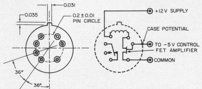
Spdt relay and FET driver are mounted in standard TO-5 can. Supply voltage is 12 Vdc nominal and relay coil is rated at 500 \Omega .
