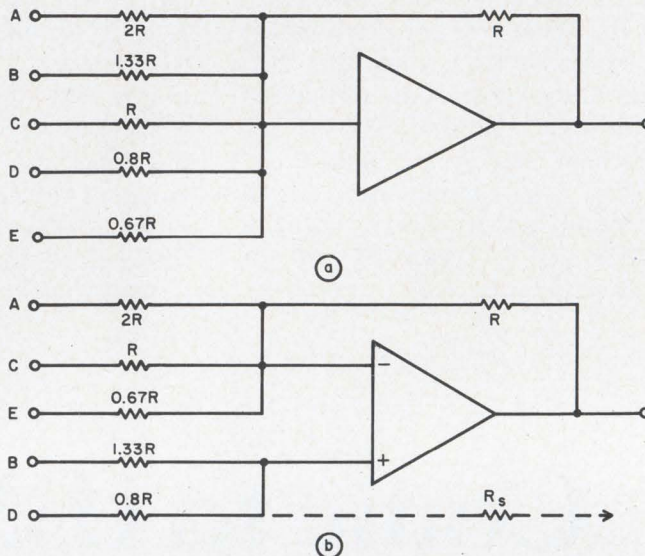
Signals of various gains and polarities (a) are summed as shown in (b). See text for details.
