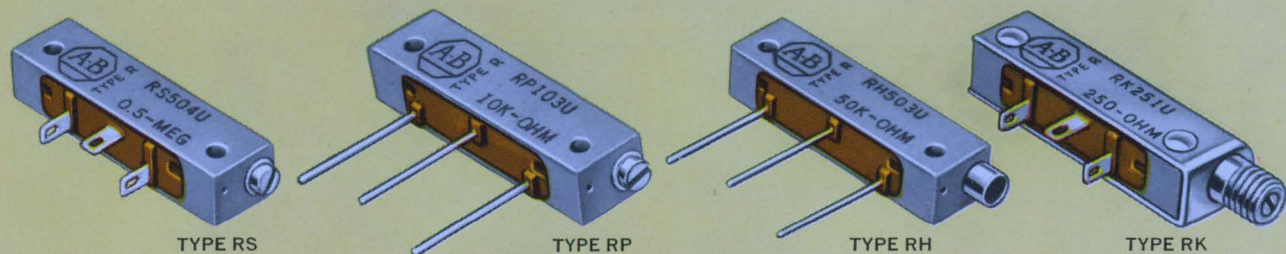
Allen-Bradley Type R Adjustable Fixed Resistors—Shown actual size
