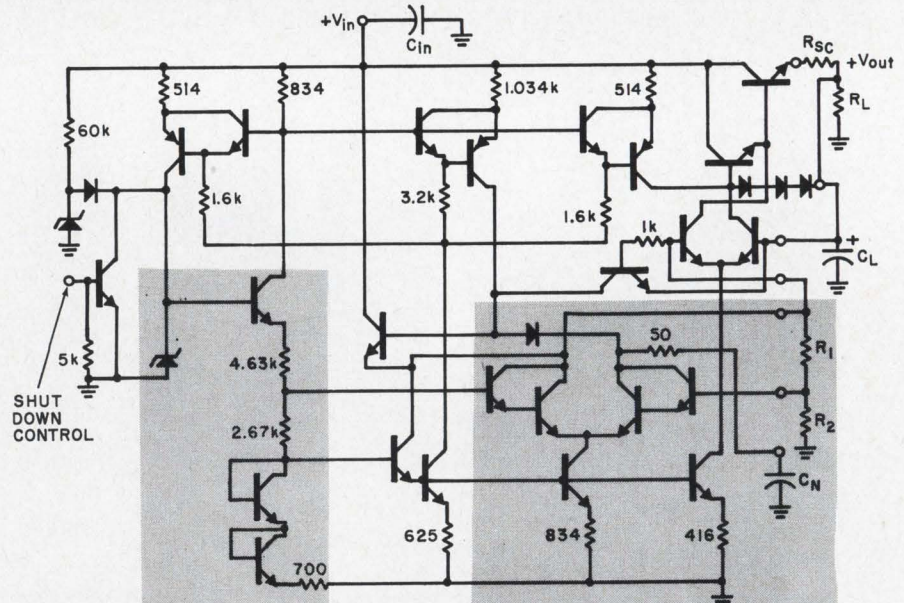
500-mA, 2-to-30-Vdc voltage regulator on a 60-by-60-mil chip. The dc reference shifting circuit (right shaded area) receives its reference voltage from the bias reference circuit (left shaded area). This bias circuit also supplies reference voltage to three single-transistor current sources (bottom). Output voltage is adjusted by selecting the ratio of R1 and R2. The supply can be turned on and off by applying a signal to the shutdown terminal. The company expects the unit to be on the market in two or three months in nine-pin TO-66 packages, selling for $7 or $8 in small lots.
