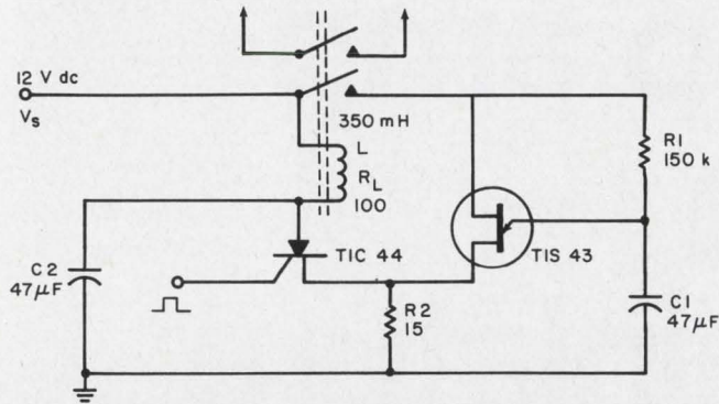
Variable relay contact closure time is obtained with an SCR and a UJT. Relay on-time depends on R1 C1 values.
