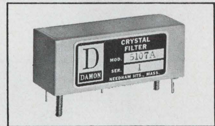
Typical Contiguous Comb Crystal Filter, Model 5107A is 1\frac{1}{16} " L x \frac{3}{16} " W x \frac{7}{16} " H.
