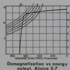
Demagnetization vs energy output, Alnico 5-7
