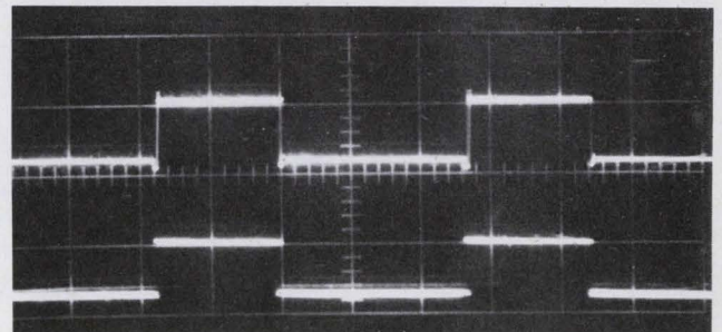
3. Operation of the switch is shown by the output (top) and input (bottom) waveforms. Vertical scale is 5 V/div. and horizontal scale is 1 ms/div.
