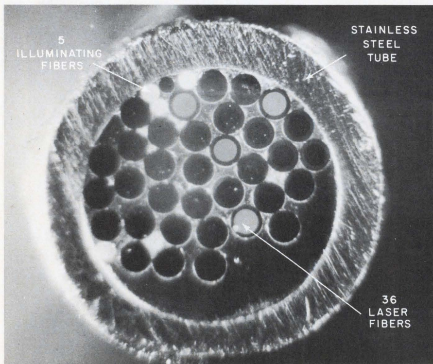
Cross-section of a fiber laser probe tip, with four of the laser fibers illuminated to show the core and the cladding.
