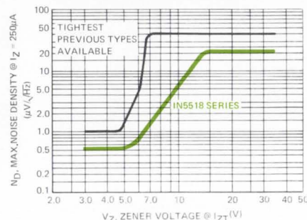
MAXIMUM NOISE DENSITY (1N5518 SERIES VS. STANDARD TYPES)
