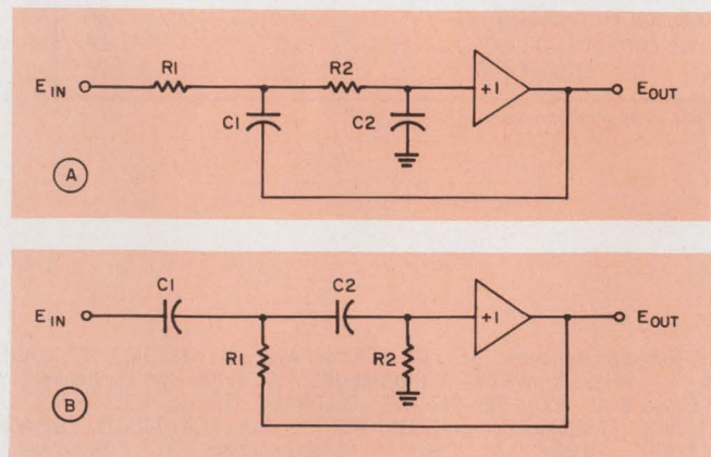
1. Two-pole circuit sections serve as basic building blocks that are cascaded to form multiple-pole filters, low-pass section above, and high-pass section, below. The component values in each section are computer-selected (to obtain either a Butterworth or Chebyshev response).
