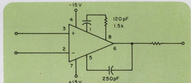
2. Frequency compensation of Signetics S5709T op amps results in the circuit waveforms shown in Fig. 3.
