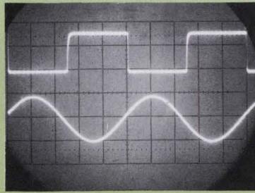
2.0 V/cm, 2 \mu s/cm 0.2 V/cm, 2 \mu s/cm NORMAL SINE WAVE INPUT AND SYMMETRIC OUTPUT
