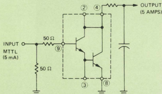
I/C Hybrid (Thin -Film) 5 Amp Darlington Driver
