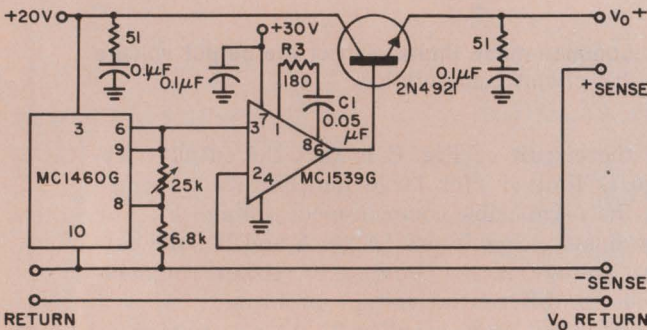
11. A typical regulator circuit uses an MC1539G op amp to provide loop gain and an MC1460G regulator to provide the reference voltage. The 2N4921 output transistor provides currents to 300 mA at the 15-V regulated output.
