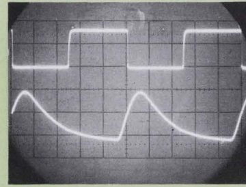
2.0 V/cm, 2 \mu s/cm 0.2 V/cm, 2 \mu s/cm DISTORTED SINE WAVE INPUT AND SYMMETRIC OUTPUT
