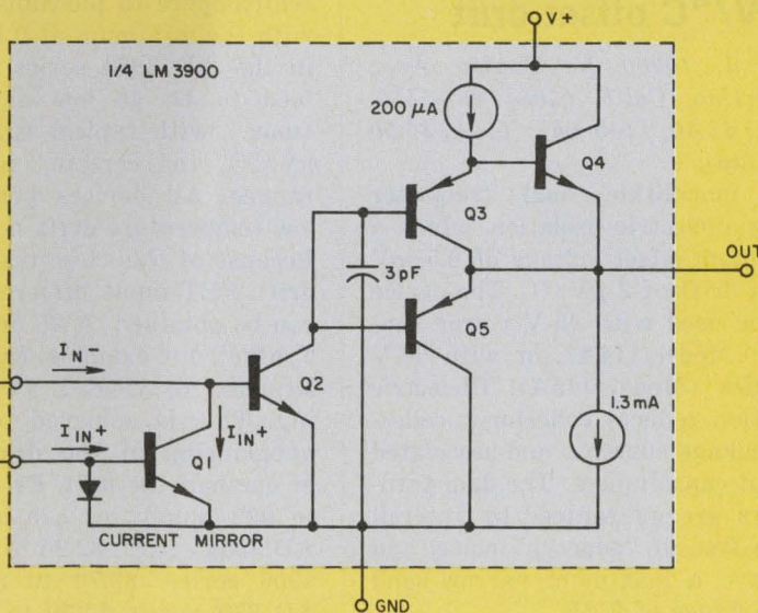
By connecting GND to V- and adding 2 resistors LM 3900 operates as a 741.
