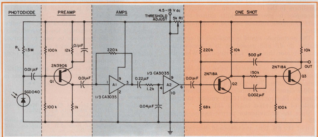
3. Receiver circuit features a maximum sensitivity of 3.5 \times 10^{-8} W for 950 nm radiation.
