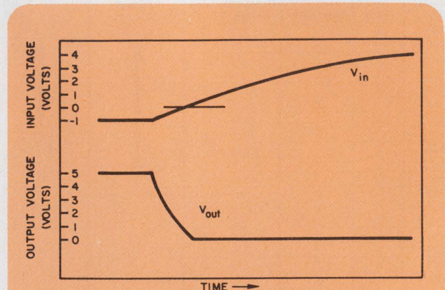
2. Input-output voltage characteristic shows circuit operation for positive and negative inputs.
