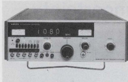
Singer: 3-1/2 digit readout; 0.008% accuracy; 2.2 V rms output.
