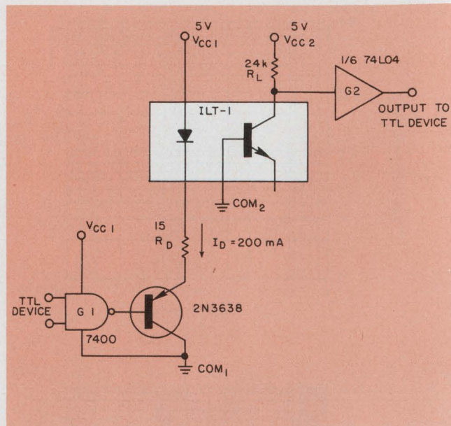
5. Operation of the phototransistor in the photodiode mode requires inverter G_2 for current gain. The component values shown boost operation to 1.5 MHz.
