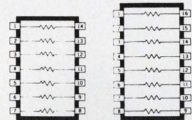
MULTIPLE ISOLATED RESISTORS
