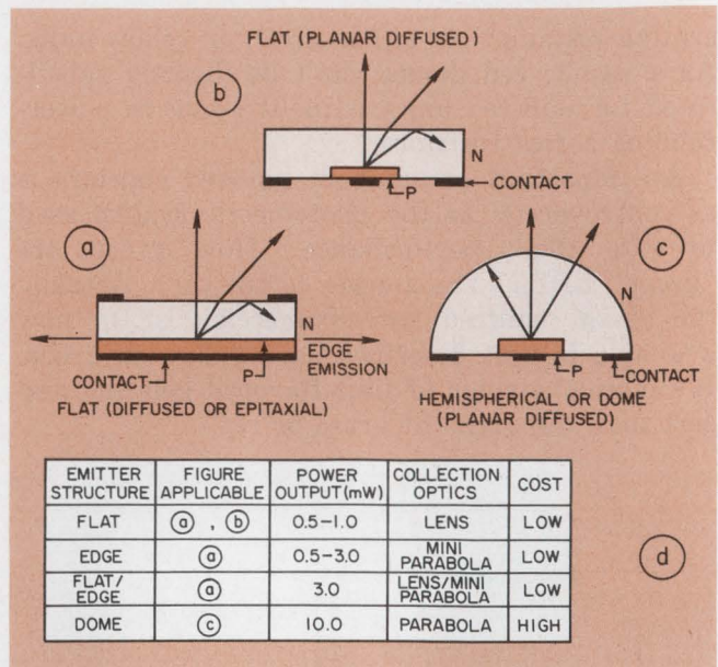
4. Various IR LED geometries enhance GaAs-junction radiation. The configurations can be flat, as in "a" and "b." The hemispherical, or dome, geometry (c) is another alternative. A table (d) provides the tradeoffs.
