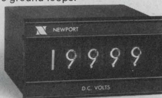
SERIES 2000B DPM: ±19,999 counts • DC voltage and current models 30 rdgs/sec • 2½"H x 4½"W x 5"D. • 0.01% accuracy • BIG-BCD output
