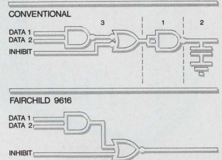
COMPARISON OF EIA DRIVERS.
