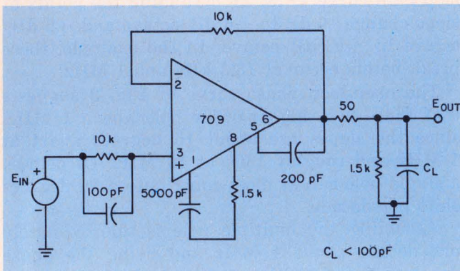
6. The \mu A709 in a feedback circuit is modeled for transient response by use of a second-order circuit. For transient analysis a step input is used.
