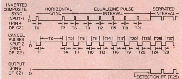
TRUTH TABLE UP TO TIME OF DETECTION
