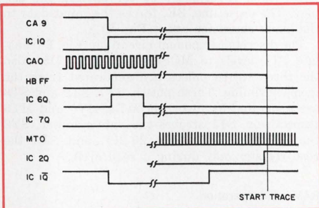
5. Horizontal retrace starts when CA9 drops to zero. This interval is mainly determined by a one-shot (IC1 in Fig. 3). Retrace is blanked when HBFF is high.
