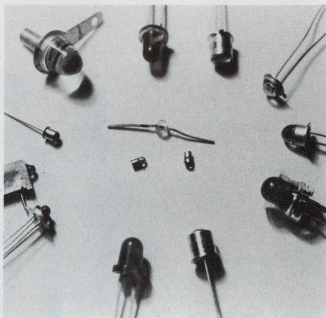
A variety of package and lead configurations are offered for both visible and IR LEDs. Most include an epoxy or glass lens. The latter lens, unlike epoxy types, is usually hermetically sealed with MIL-spec units available.
