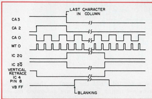
4. Vertical retrace starts when CA3 drops to zero. The interval is mainly determined by a one-shot (IC2 in Fig. 3). Retrace is blanked when VBFF is high.
