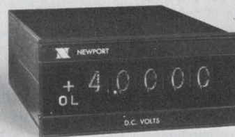
SERIES 2000A DPM: \pm 39,999 counts • DC volts, current or ratio • .01% accuracy BIGS-BCD outputs... buffered, isolated, gated and stored • 2½"H x 5"W x 7½"D.
