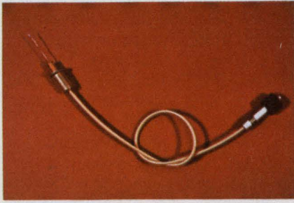
A 660-nm LED is mated with a section of DuPont single-channel plastic fiber-optics cable in this pigtail assembly by Aborn Electronics.
