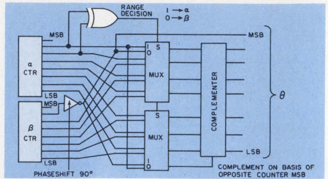
4. One counter is always within its mid-range, because the \alpha and \beta signals are 90° apart. A range-decision gate in the angle-decision logic selects the data set.
