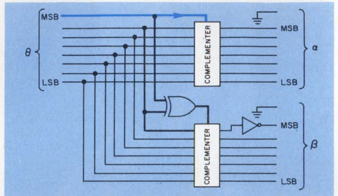
5. Quadrature-conversion logic develops \alpha and \beta from \theta . The MSB of \theta controls the \alpha complementer, while \theta 's two MSBs control the \beta complementer.
