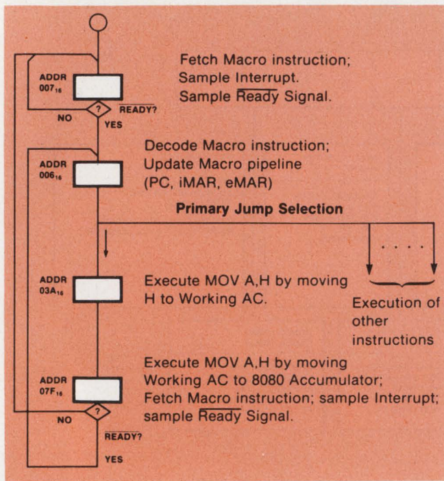
4. To duplicate the MOV A,H instruction of the 8080A, check this flow chart, which shows all the operations that must be performed under software control.
