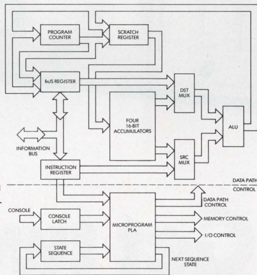
9440 Block Diagram
