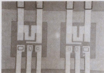
Two transistors can hang in space thanks to a controlled etching process. The IC is only 3 mils thick.
