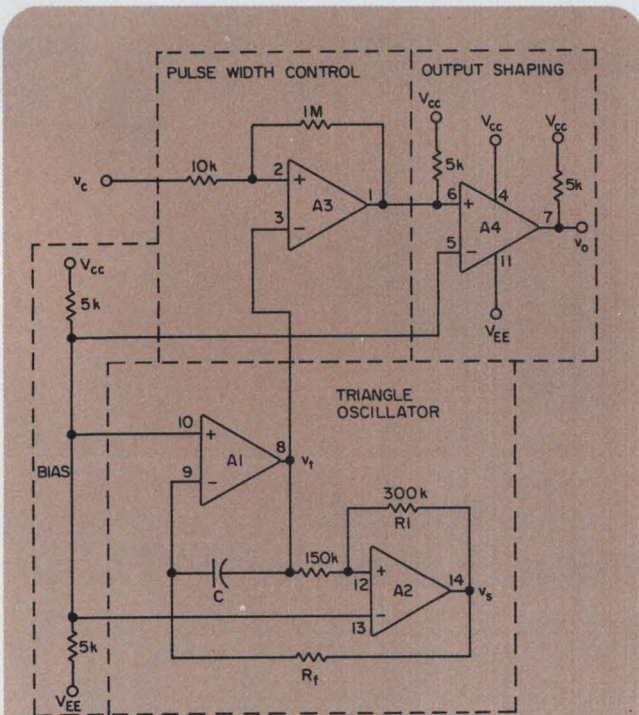
1. A single chip that contains two op amps and two comparators simplifies the construction of a constant-frequency pulse-width modulator. Op amps A 1 and A 2 operate as an oscillator, comparator A 3 modulates, and comparator A 4 shapes the output.
