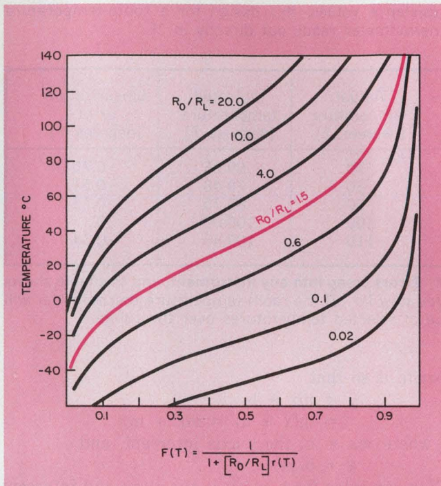
3. A thermistor will operate linearly over a number of temperature ranges, depending on the value of R_0/R_L . For a room-temperature thermometer, R_0/R_L = 1.5 gives the most linear performance.
