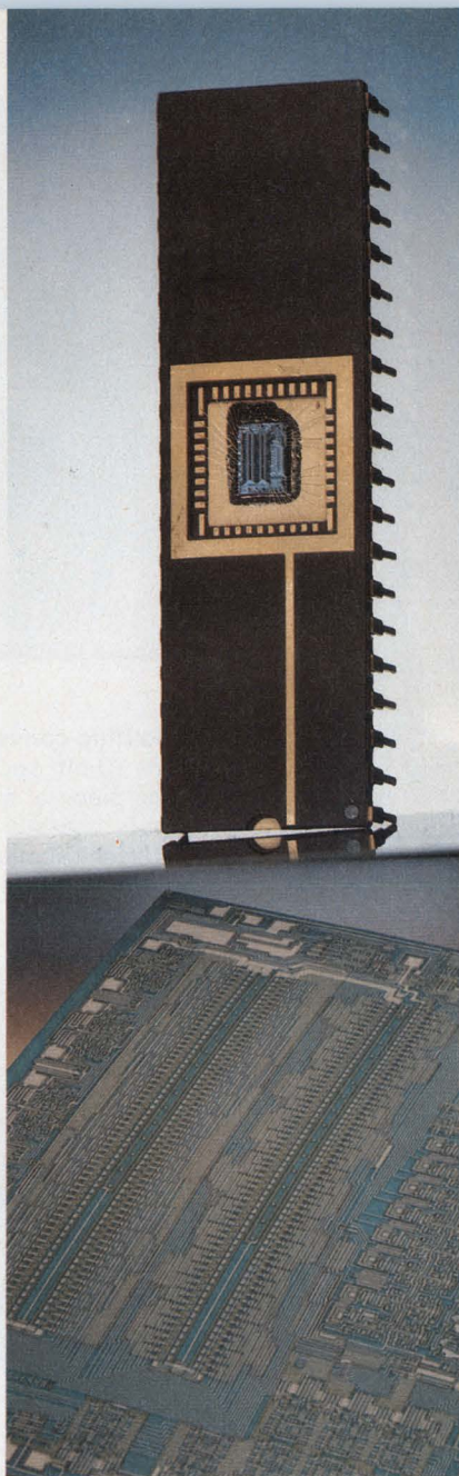
First of its kind: This single-chip data-acquisition system includes an 8-bit a/d with Tri-state outputs, a 16-channel multiplexer and logic control to interface \mu Ps (National).
