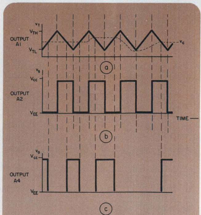
2. Triangle/square-wave oscillations (a and b) are applied to the modulator/shaper, which provides a pulse-width-modulated signal output (c).
