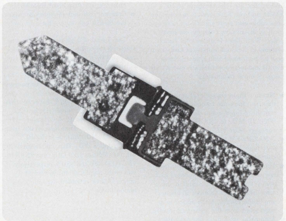
The HP mesa process with glass backfilling is responsible for the performance of this beam lead PIN. The mesa construction constrains the minority carriers, thereby enhancing switching speed.
