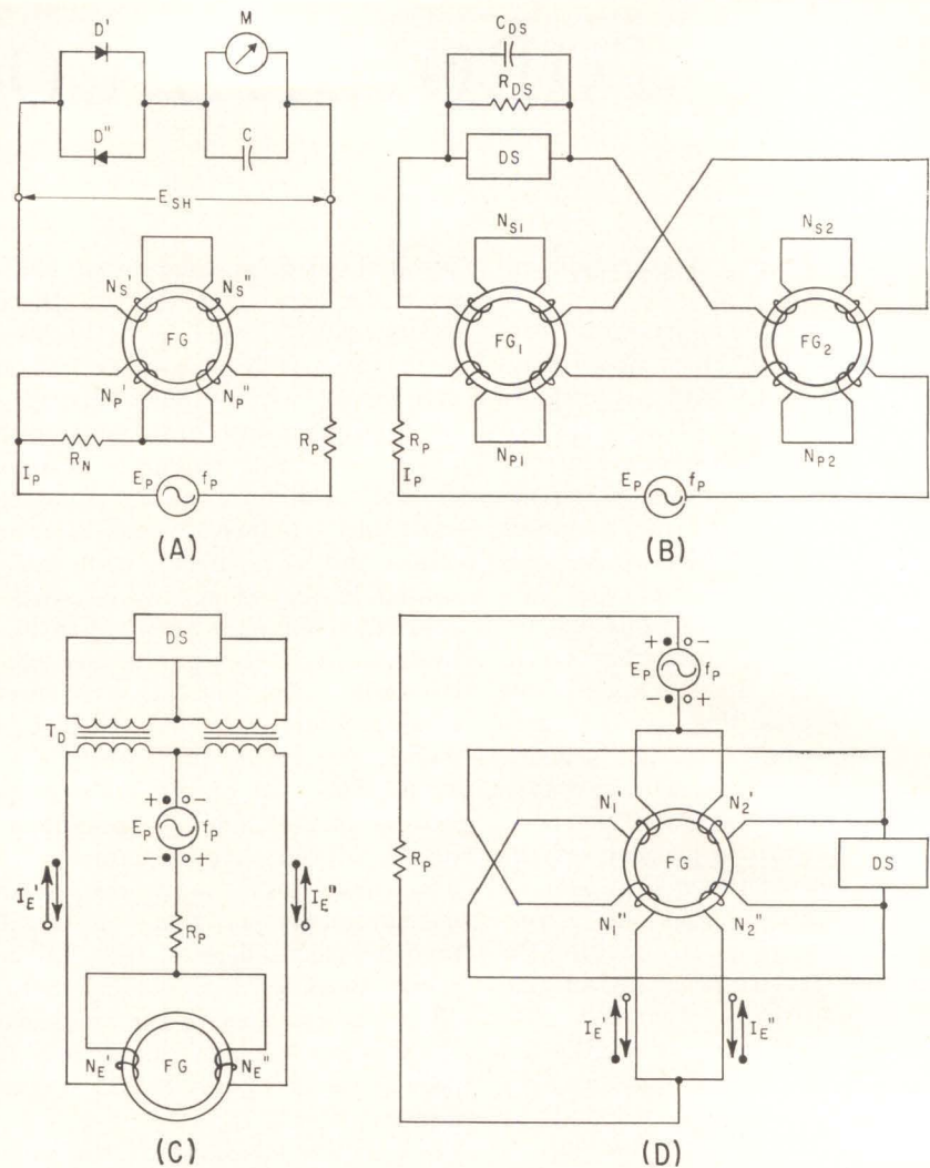
FIG. 3—Transformer circuits: magnetometer (A) with a single flux gate; gradiometer (B) with two equally rated flux gates. Autoconnected magnetometer circuits: differential (C) with two windings and center-tapped output transformer; bridge (D) with four equally rated windings
