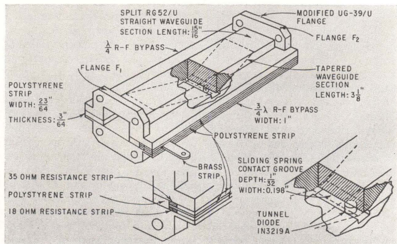
FIG. 2—Waveguide mount for the tunnel diode; the position of the diode can be adjusted continuously to find optimum input impedance
