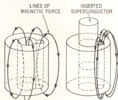
Magnetic lines of force are distributed evenly until superconductive material is inserted
