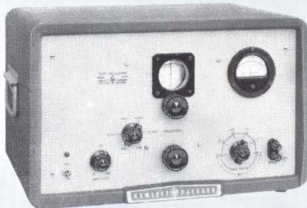
hp 650A Test Oscillator, 10 cps to 10 MC.
