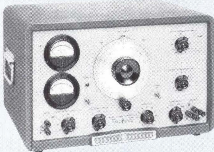
hp 205AG Audio Signal Generator, 20 cps to 20 KC.
