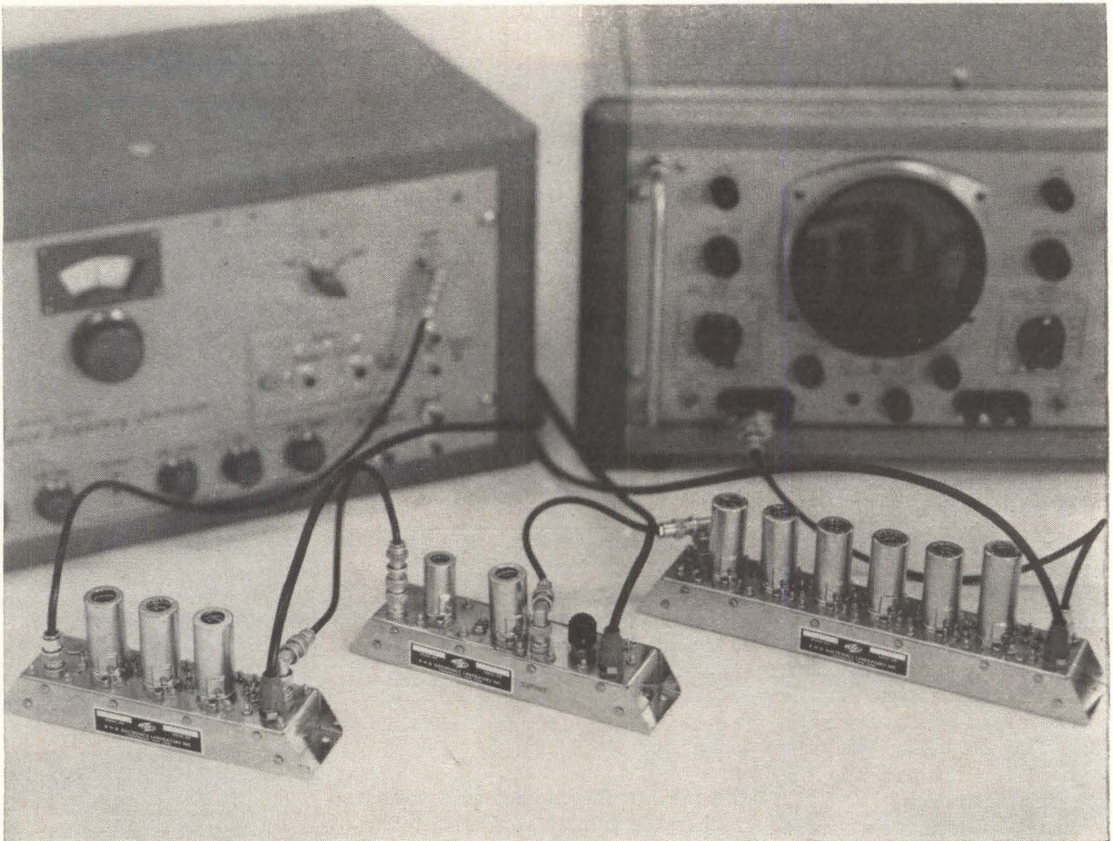
Variable bandwidth filter can be used to make bandwidth a function of signal level
