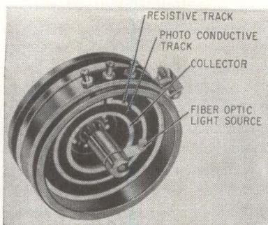
FIG. 4—Duncan Betapot potentiometer uses glass fiber to direct light onto photoconductive track, to make contact between resistive and collector rings
