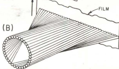
FIG. 8—Image converters transform information into more convenient form: raster to line, (A), circular-to-line, (B)—both can also operate in reverse
