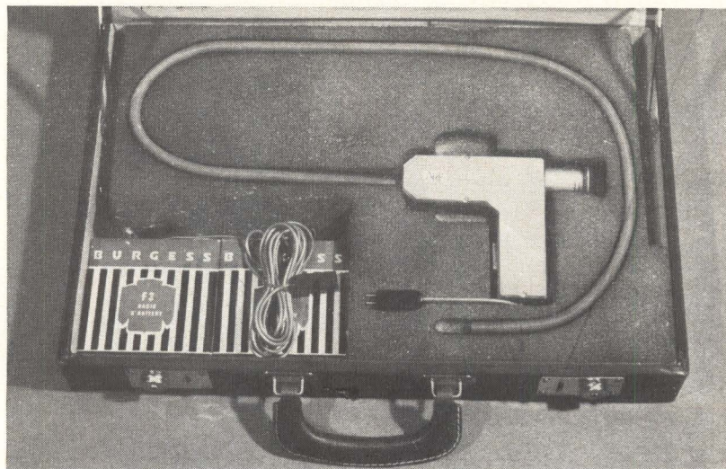
FIG. 3—Flexible fiberscope made by Armour Research Foundation for use by Sandia's Livermore Laboratory in missile applications
