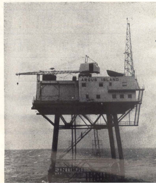
Tower near Bermuda is relay point for hydrophones
