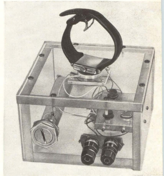
Demonstration magnetometer with \frac{1}{2} -inch flux gate and polarity-sensitive demodulator uses 6.75 v, detects movements of ferromagnetic parts of watch
