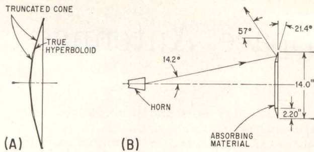
FIG. 2—Conical approximation (A); scatterer (B)
