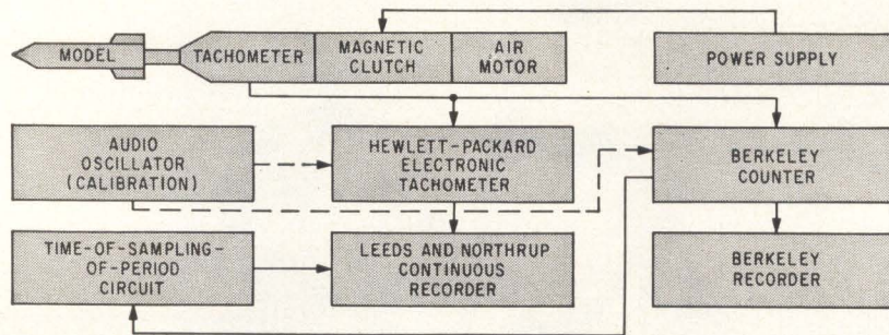
FIG. 2—Test setup for taking data on roll damping. Pulse-count data is fed to a computer (not shown), which calculates roll-damping coefficient
