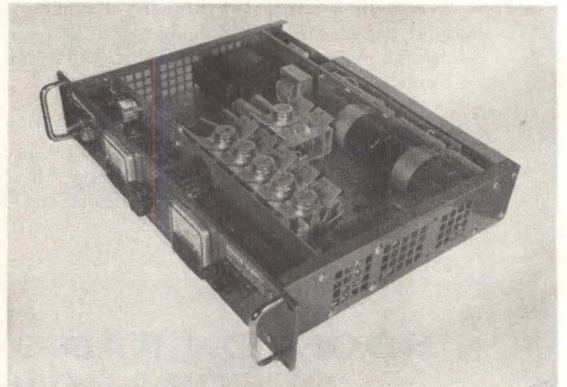
Power supply equipped with plug-in radiators illustrates open construction and shows efficient circulation attained in stacked racks
