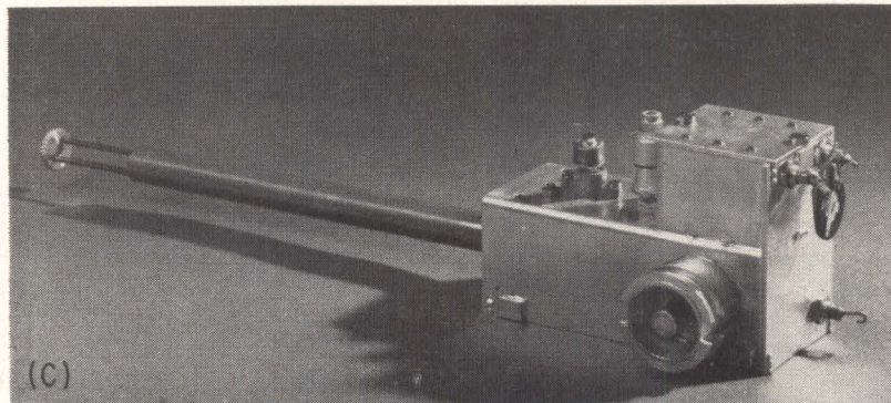
FIG. 2—Current-tuned uhf tuner (A) and its performance curves (B); illustration (C) shows hardware used. Table I gives performance for several transistors that were tested in the circuit
