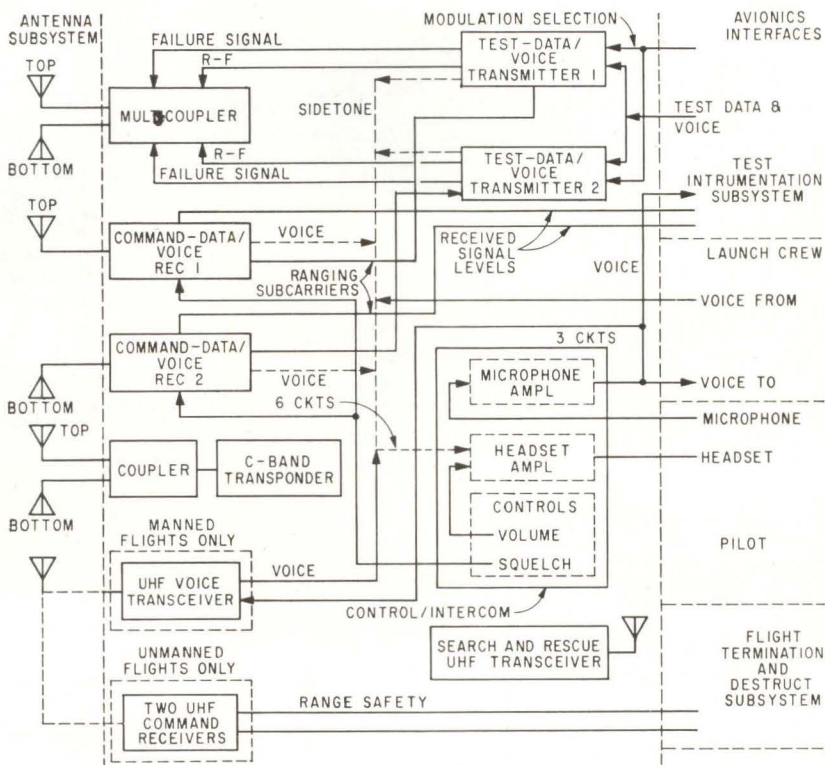
Airborne equipment—two transmitters and the microphone amplifier in the control panel are the airborne portion of the shf vehicle-to-surface link. Two receivers, converter decoders, and pilot's headset amplifier in the control panel are the surface-to-vehicle shf link
