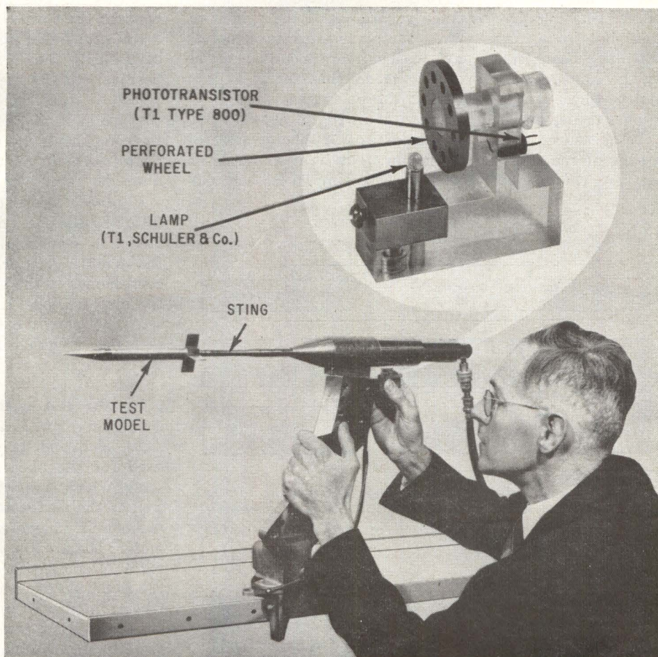
FIG. 1—Inset shows mockup of phototransistor tachometer. Author is inserting tachometer section that comprises lamp and phototransistor
