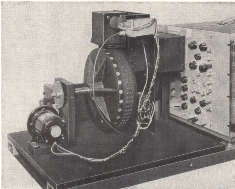
Scanner unit with cover removed
