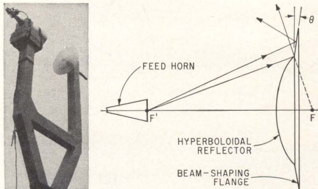
FIG. 4—Geometry of shaped-beam subreflector with photo of scale model feed system and mount
