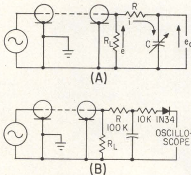
Simplified version (A) of capacitance transducer was instrumented (B) to measure machine-tool vibration
