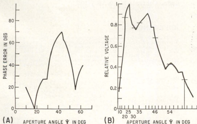
FIG. 7—Phase error plot, 45-deg plane, \theta = 18.4 degrees (A); aperture integration plot, 45-deg plane, \theta = 18.4 degrees (B); and vector integration diagram (C)
