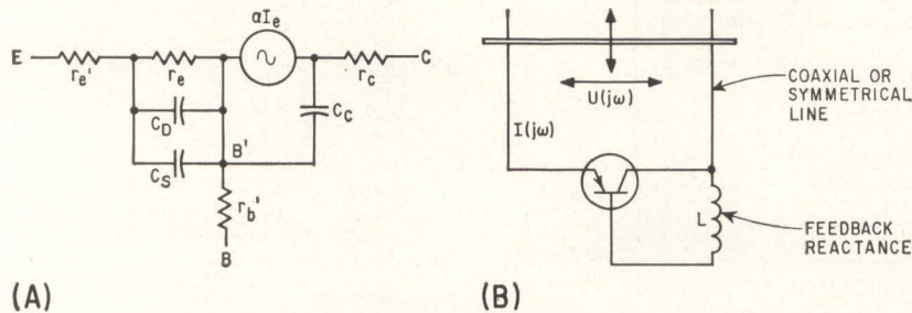
FIG. 1—Equivalent circuit of transistor when considered for high frequency use (A); conditions for operation of actual circuit (B) are based on this equivalent circuit
