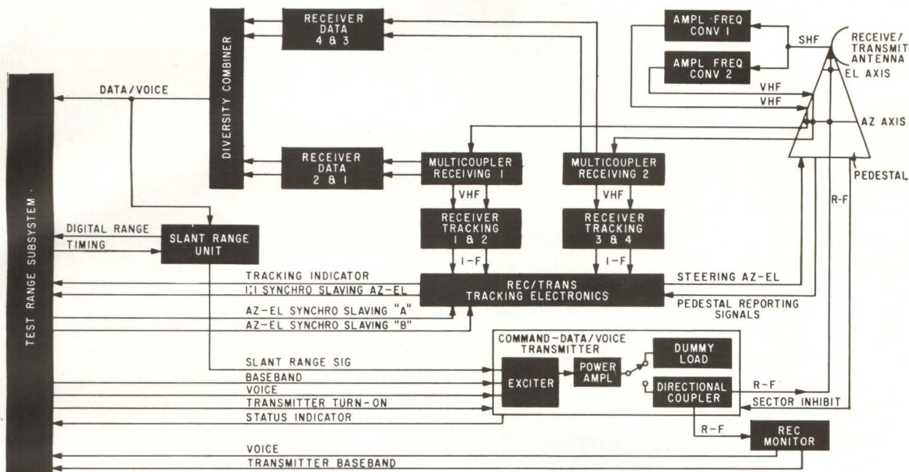
Surface equipment—three major functions are shown in the composite receive-transmit site: signal tracking, r-f conversion/demodulation and r-f transmission
