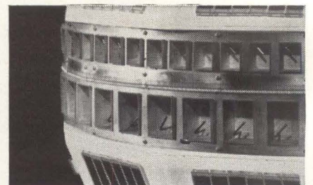
Section of satellite shows equatorial antenna slots. Upper row transmits, lower row receives microwave signals.
