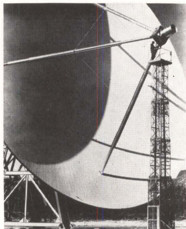
Technician uses portable elevator to adjust horn. The 6,000-square-foot reflector skin is aluminum
