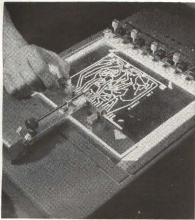
Grid pattern is mounted on plate covering projector light source. Both pc and grid pattern films expand at same rate to heat from projector lamp. Three-way aligning arm gives quick, precise adjustment
