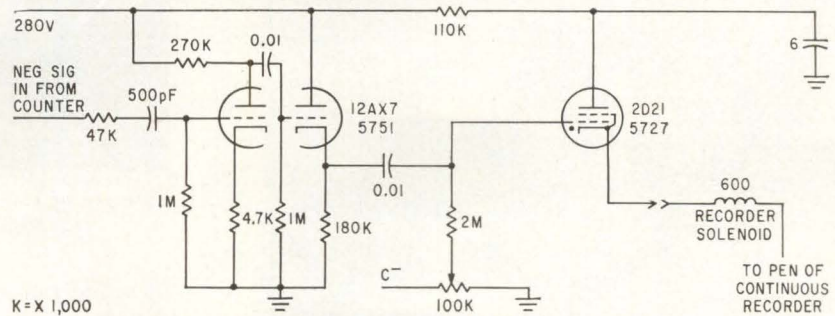
FIG. 3—Output of this time-of-sampling-of-period circuit goes to the continuous recorder shown in Fig. 2
