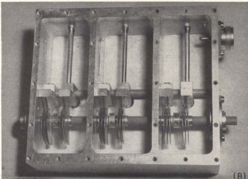
FIG. 4—Tuner uses epitaxial transistors to cover uhf/shf bands, operates up to 5,000 Mc (A); physical construction of the tuner (B). Table II gives test results
