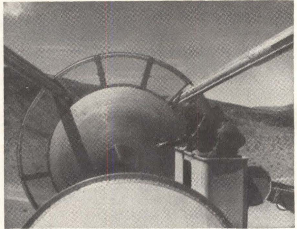
Close-up of full scale modified subreflector
