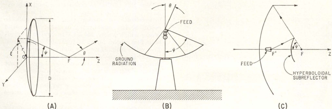
FIG. 1—Paraboloid geometry (A); parabola pointing to zenith (B); and basic geometry of the Cassegrainian antenna system (C)
