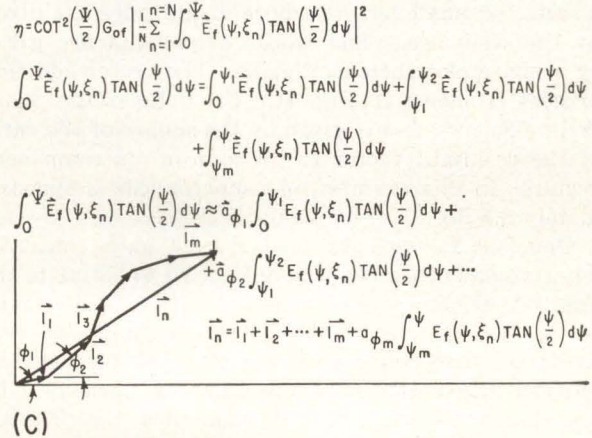
FIG. 7—Phase error plot, 45-deg plane, \theta = 18.4 degrees (A); aperture integration plot, 45-deg plane, \theta = 18.4 degrees (B); and vector integration diagram (C)
