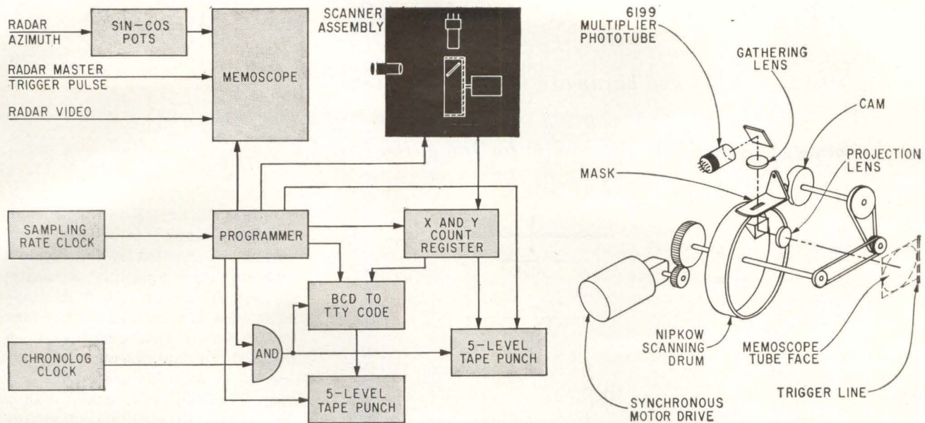
Block diagram of scanning system (left); optical and mechanical components of scanning system (right)
