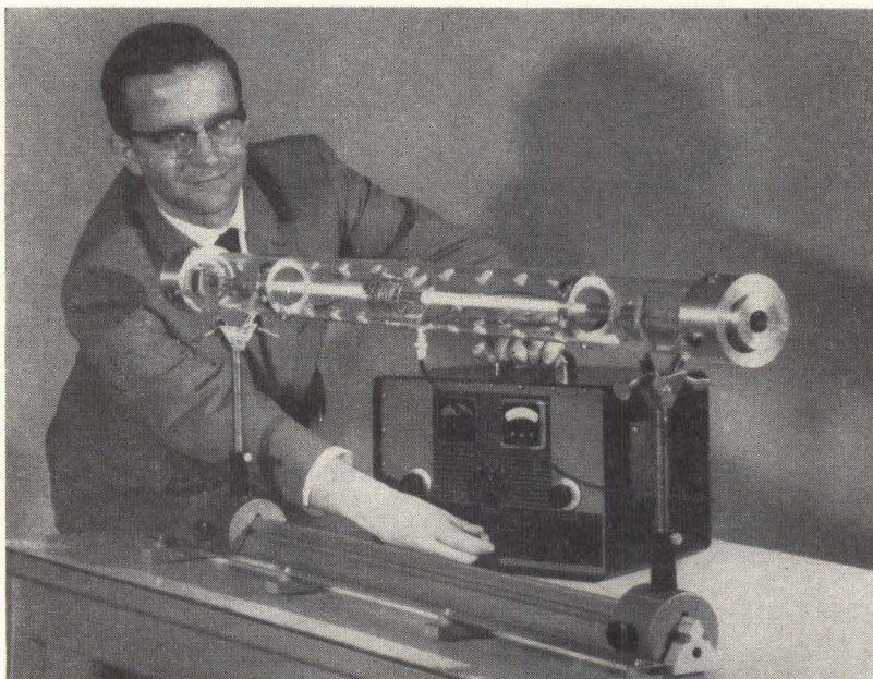
Output of 1.5 mw is provided from each end of helium-neon laser introduced by Raytheon and warranted for 1,000 hours continuous operation
