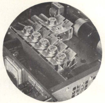
Close up of typical plug-in radiators in forced air stream. Use of forced air results in smaller size, reliability of components
