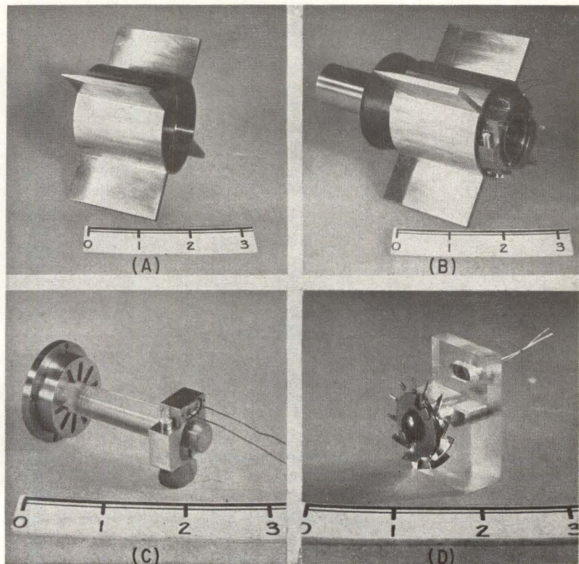
FIG. 4—Finned tail (A) has internal mirrors on inside surface that successively reflect light to tachometer (B). Phototransistor in (C) receives light pulses from reflecting faces of gear teeth. An angular reflection model is shown in (D)
