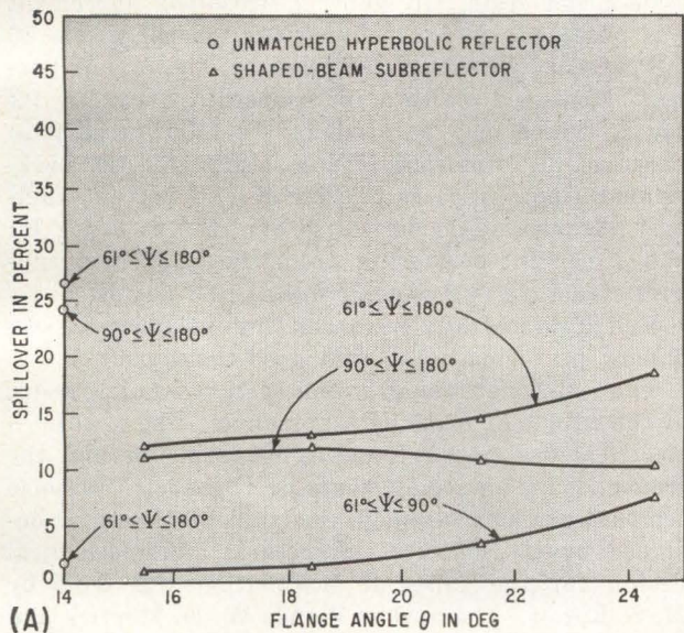
FIG. 6—Spillover plotted against flange angle (A), and Serrodyne phase measuring system (B)
