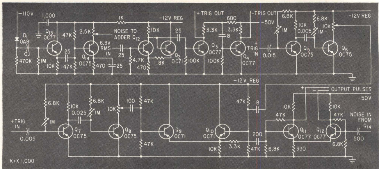
Output pulses of this circuit are long and short pulses of positive and negative polarities. Either pulse can be adjusted in duration and amplitude
