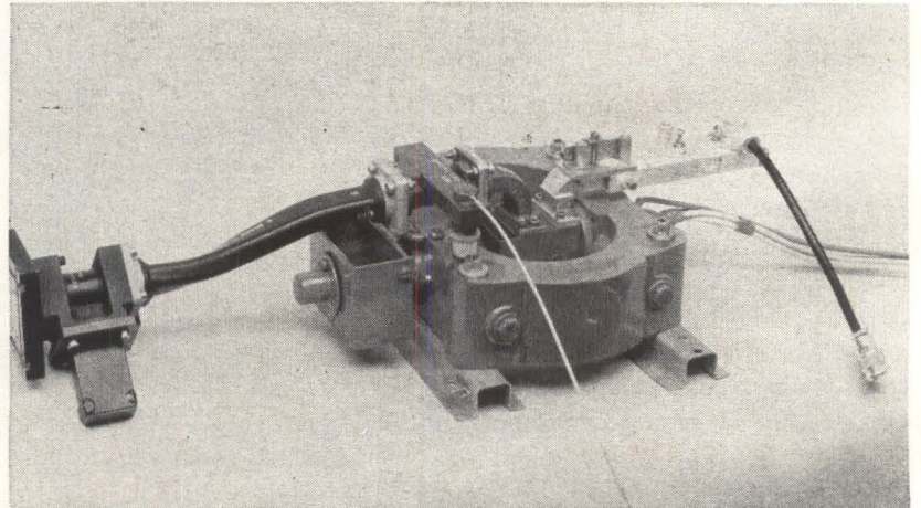
Shf transmitter output shows multiplier stage, klystron, flexible waveguide, circulator and r-f load
