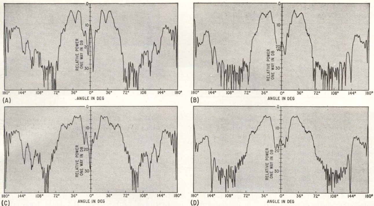
FIG. 5—Modified reflector patterns: E-plane pattern (A) and H-plane pattern (B) for \theta = 15.4 deg; and E-plane pattern (C) and H-plane pattern (D) for \theta = 24.4 degrees
