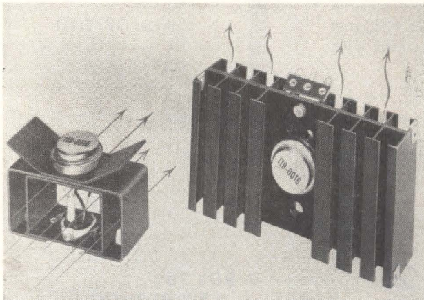
Forced air stream applies lateral circulation of air in heat sink at left. Heat sink at right illustrates a typical convection cooler
