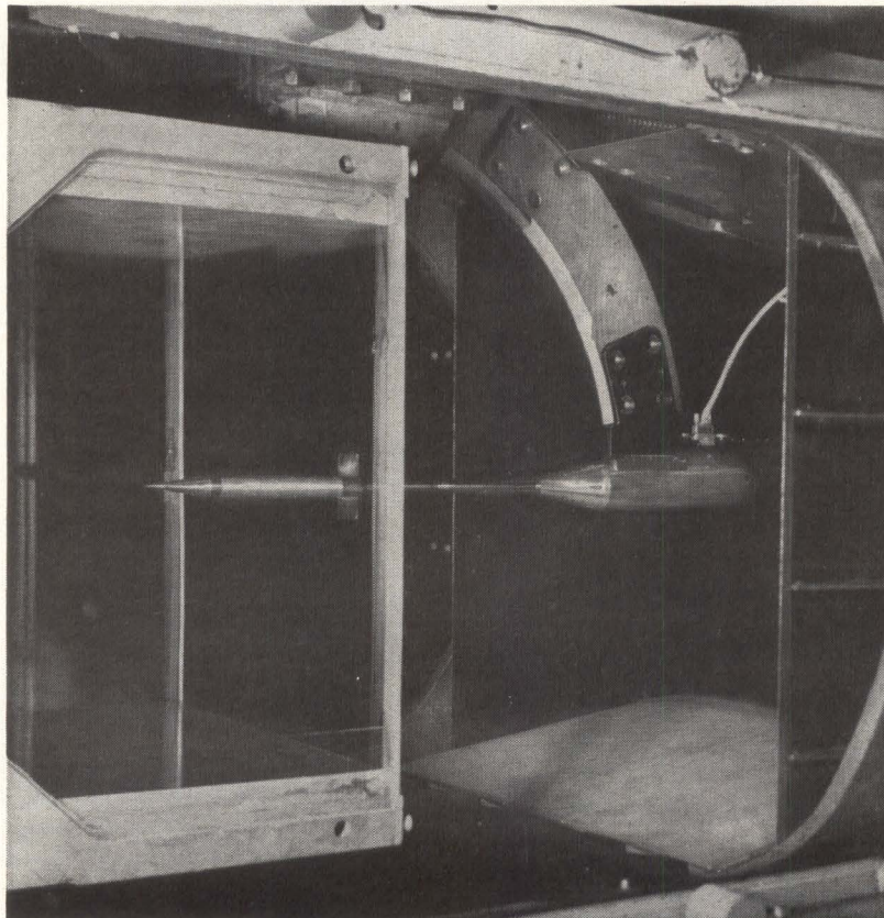
Test setup and model are shown inside a wind tunnel prior to testing
