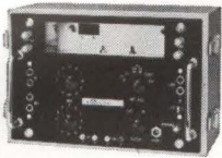
Portable Test Hybrid Simplifies cable acceptance tests and return loss measurements.
