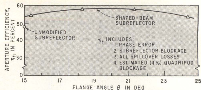
FIG. 8—Aperture efficiency plotted against flange angle
