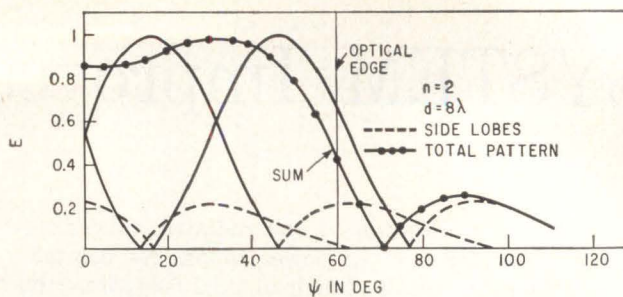
FIG. 3—Calculated synthesis of Cassegrainian pattern
