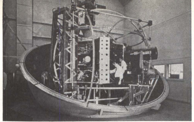
OUTER SPACE conditions are simulated at test facility. System is on air-bearing table that provides frictionless movement
