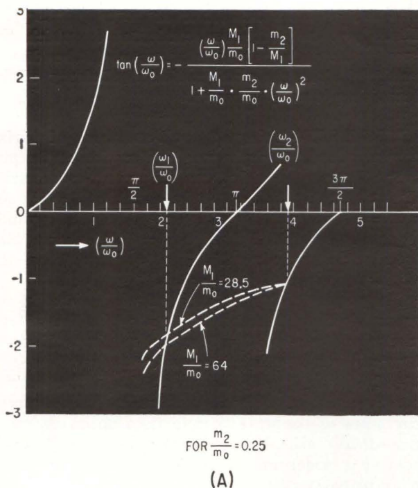
GRAPHICAL SOLUTION for \omega/\omega_0 shown in (A); vertical component of ground surface displacement |s_z| plotted against distance r from surface-based driving source (B) is normalized for different ground media—Fig. 2
