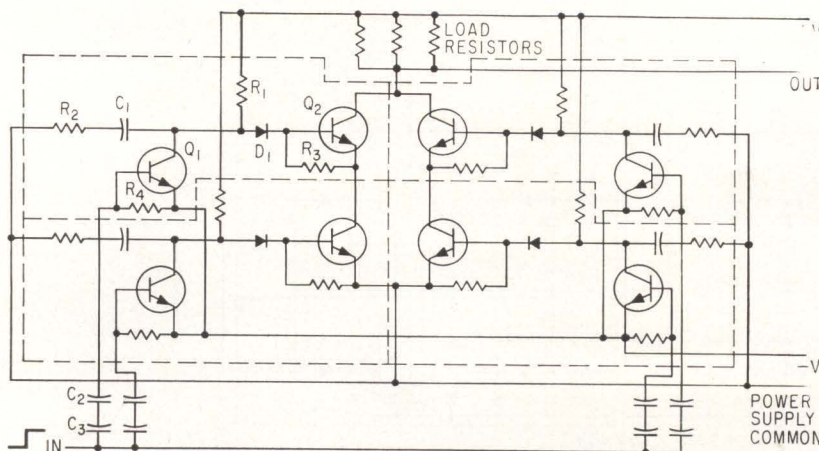
PULSE STRETCHER may be retriggered at any time during period of operation—Fig. 8
