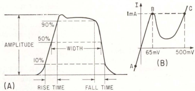
ANALYZER will convert these parameters for programmer-comparator use (A). Characteristic curve of the 1 milliamper tunnel diode used in the level sensor (B) Fig. 1
