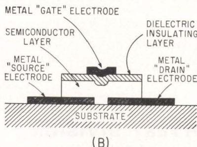
SCHEMATIC of the experimental microcircuit, (A); cross-sectional view of a field-effect active device, (B)—Fig. 1
