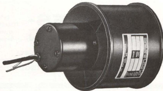
A 3" blower may operate more than 10,000 hours on d.c. using an inverter that adds 1½" to motor length.
