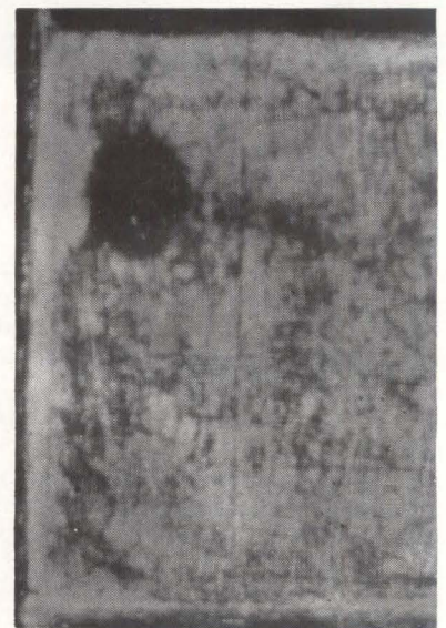
IRON OXIDE insulating film on glass reed switch contacts remained light while metallic areas darkened under ferric ferricyanide test
