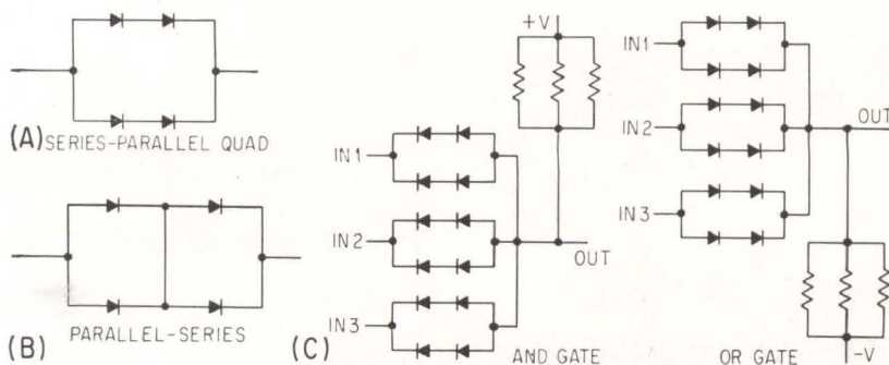
DIODE QUADS in two configurations (A) and (B), and logic gates (C) using the series-parallel quad—Fig. 1
