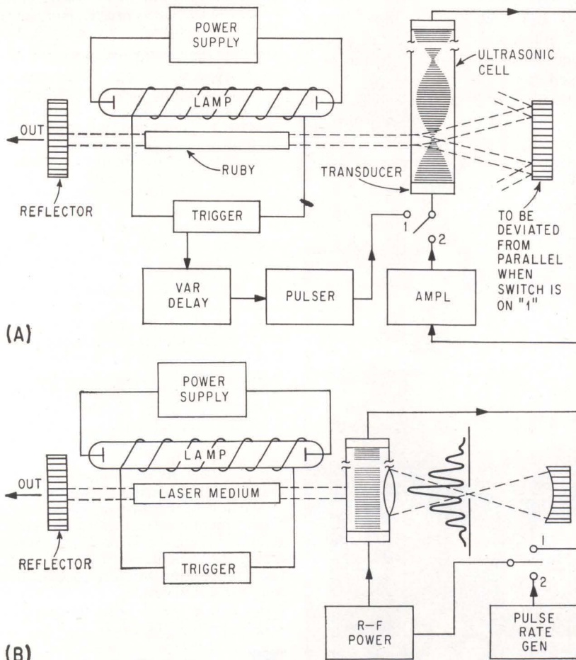
EXPERIMENTAL arrangement of ultrasonic refraction shutter (A) and diffraction shutter (B). These setups are used at United Aircraft to control laser action
