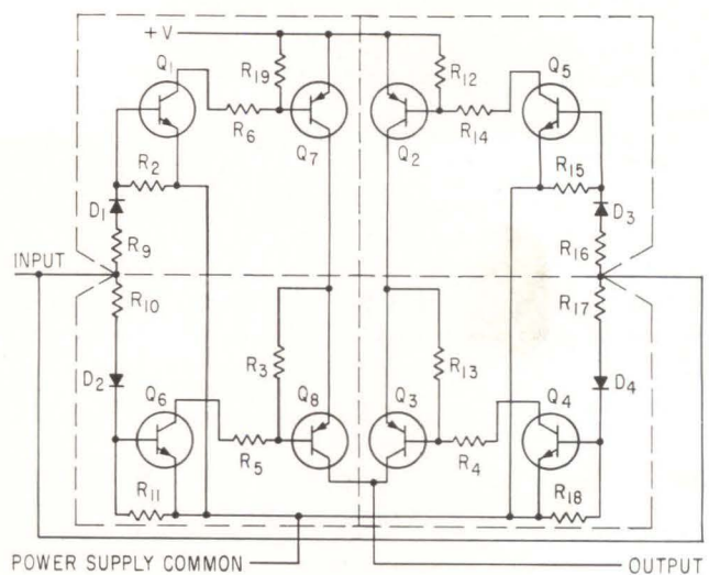
POWER SWITCH application for a noninverting driver—Fig. 4
