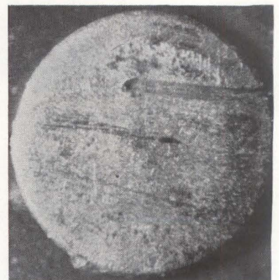
CORNCOB tumble polish produced insulated areas on contacts that contrasted with metallic areas which remained dark under test
