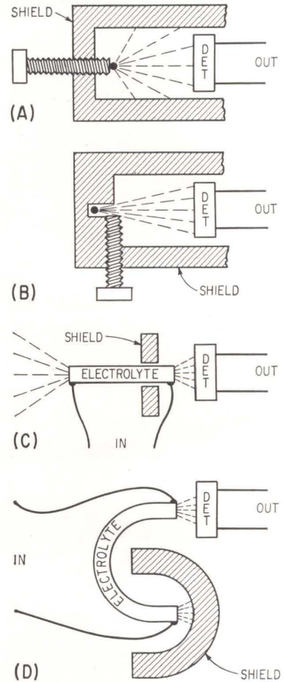
RADIATION level can be adjusted by a micrometer feed, (A) and (B); or by using high precision plating of radioactive material, (C) and (D)—Fig 1
