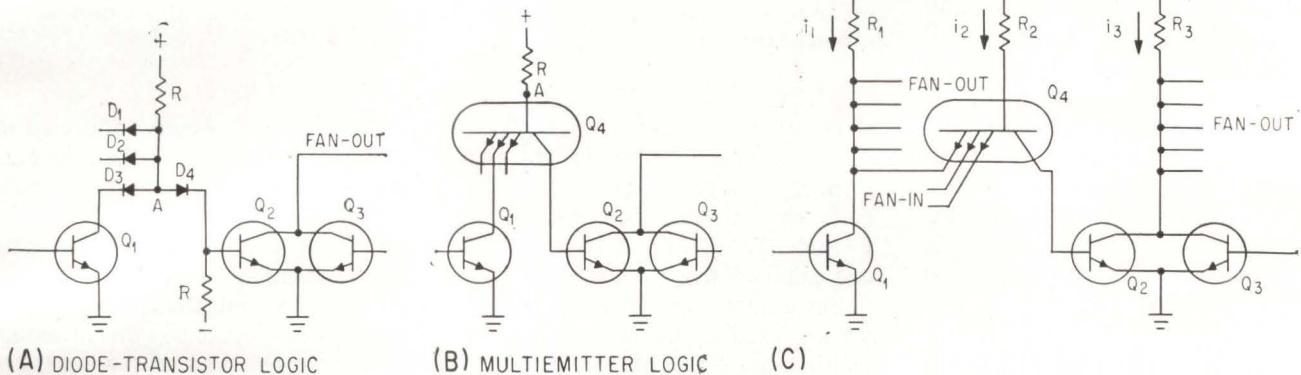
(A) DIODE-TRANSISTOR LOGIC (B) MULTIEMITTER LOGIC (C) DIODE GATE (A) is transformed into a multiemitter gate (B). In (C), for a fan-out of five and reverse beta of 0.1 for Q_4 , the circuit is safe if i_1 is greater than i_2/2 —Fig. 2
