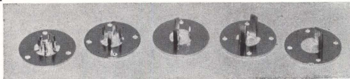
ANODE VANES of magnetron tubes produced by electric discharge machine have tolerances of \pm 0.0001 inch
