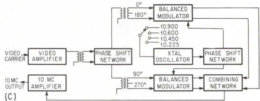
TELEMETRY receivers such as the TMR-5A have plug-in tuning heads and i-f and demodulator modules (A), while "down" converters translate receiver i-f data into suitable recording form (B). "Up" converter changes video-carrier data back to 10 Mc for receiver reinsertion (C)—Fig. 4
