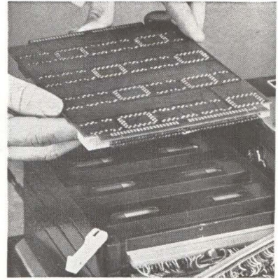
COMPUTER for new guidance system uses welded-wire circuit modules assembled on printed-circuit laminates and stacked on heat-conducting trays next to drum memory
