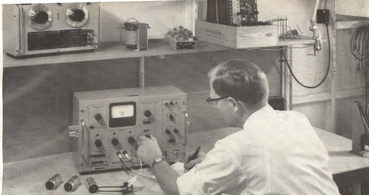
IMPEDANCE METER with direct readout of magnitude and phase angle
