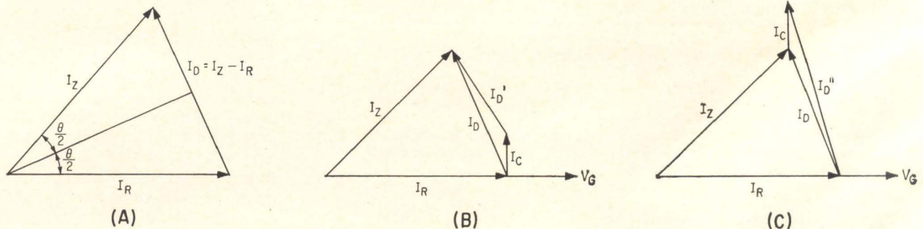
VECTOR DIAGRAM for determining phase angle (A); with S_2 in plus position (B), C_v in parallel with R ; with S_2 in minus position (C), C_v in parallel with Z . Phase angle is negative because the absolute value of I_D'' is greater than that of I_D —Fig. 2
