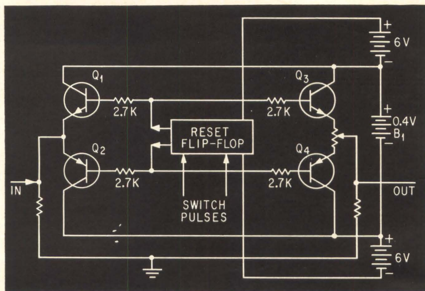
TWO SETS of series-connected silicon transistors rapidly switch, input to output, voltages from a microvolt on up, in low and medium frequency applications
