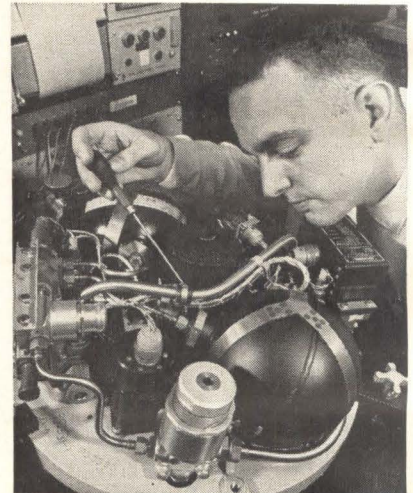
PACKAGE includes reaction-jet fuel supplies, five gyros, command guidance transducers, power supply, plus control and telemetry electronics
