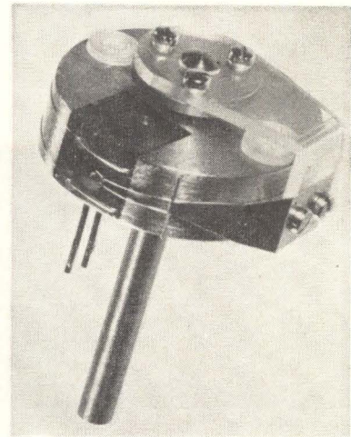
CONSTRUCTION of 10-ohm variable capacitor
