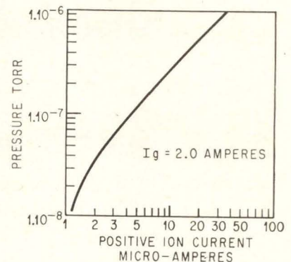
CALIBRATION curve of a typical tube acting as its own vacuum gage against pressure in torr
