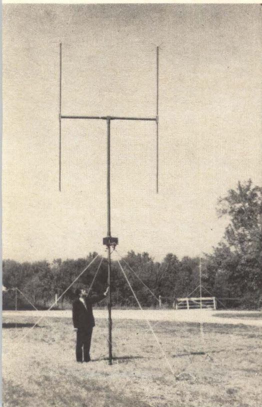
FIBER GLASS 20-foot mast supports an 8-foot wide by 12-foot high array
