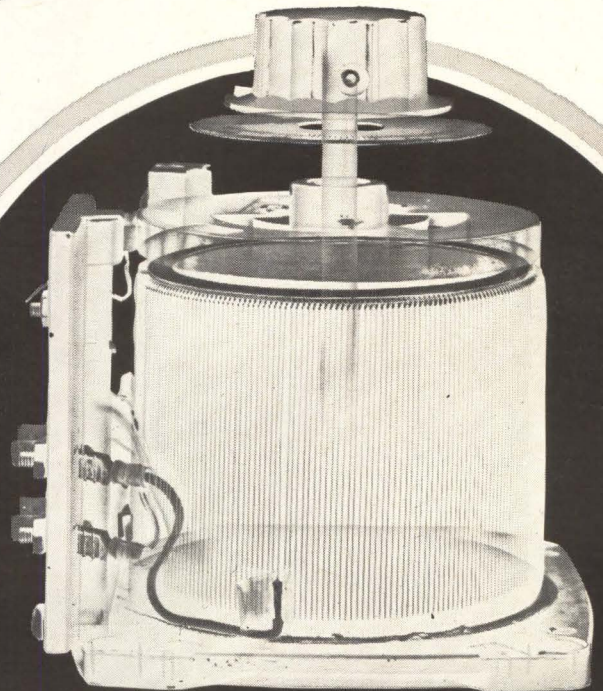
This x-ray photograph reveals the heat sink ring directly beneath the circular brush track.
