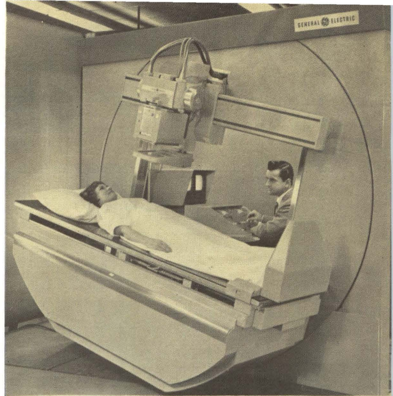
REMOTE POSITIONING of patient is provided in GE fluoroscope system. Instrument uses closed circuit tv to intensify image, and present it for study by radiologist in shielded viewing area. Cine recordings are made if desired
