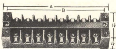
FIG. 57—AN 8-CIRCUIT MOLDARTA TERMINAL BLOCK
