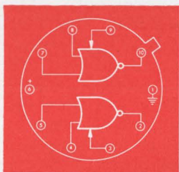
LU316 DUAL EXPANDABLE NOR GATE
