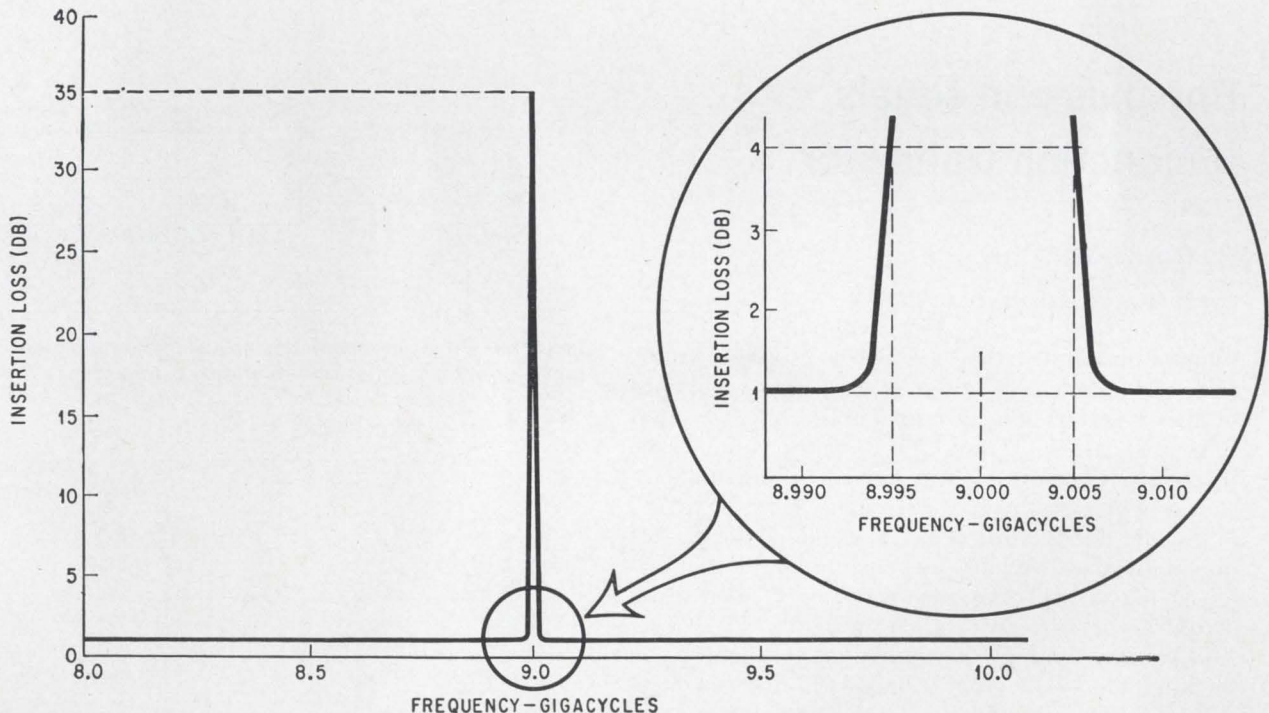
Measured insertion loss versus frequency performance characteristics of the hybrid notch filter. The notch (rejection) frequency for this measurement was tuned to 9.0 gigacycles. The notch is nominally 0.010 gigacycles wide, and can be tuned over a range of 8.2 to 12.4 gigacycles with a rejection of 30 to 36 db. The input vswr is less than 1.5.
