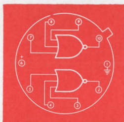
LU315 DUAL 3-INPUT NOR GATE
