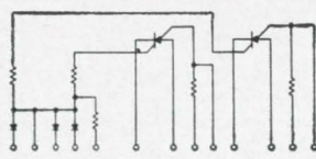
DECODER LATCH
