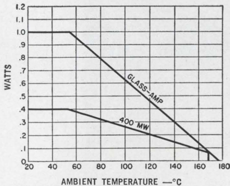
POWER DISSIPATION
