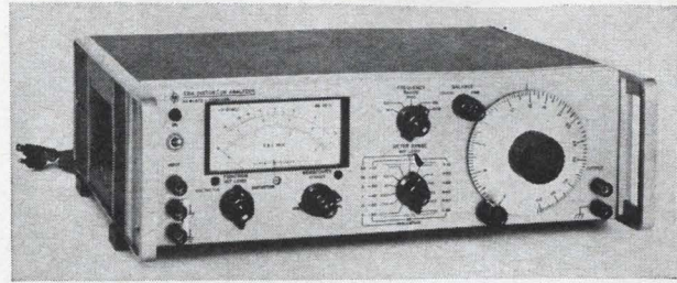
Model 331A distortion analyzer can be bench- or rack-mounted. Controls are simple to use; meter, calibrated in decibels, percentage and volts, is easy to read. The frequency, set with the large dial, is accurate to within 2%.
