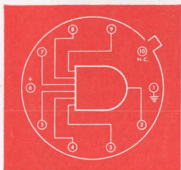
LU305 AND GATE
