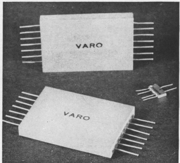
Thin-film hybrid module dissipates 18 watts when mounted on a heat sink. It can drive a core memory. Small unit is conventional two-transistor flatpack version.
