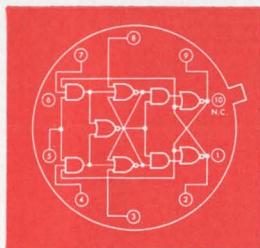
LU320 J-K BINARY ELEMENT
