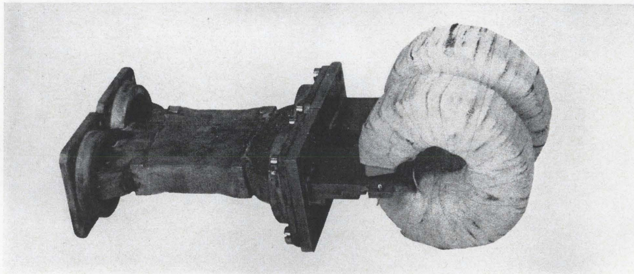
Electronically tunable hybrid filter has a very narrow rejection band and is nonreflective. The resonant element is a YIG crystal sphere mounted near the end wall of each shorted transition section, and within the field of the electromagnet. The rejected frequency band varies as the intensity of the magnetic field. The field of each magnet varies equally and simultaneously. The height of the X-band waveguide was reduced in four sections from 0.40 inch to 0.05 inch to obtain maximum filter rejection loss.
