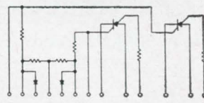
SCS FLIP-FLOP
