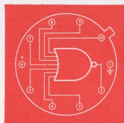
LU314 7-INPUT NOR GATE
