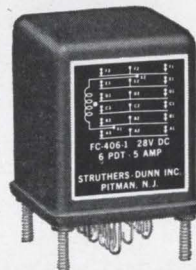
Type FC-406 6P-DT. 5 ampere contacts.
