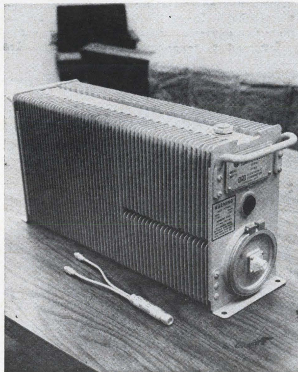
Both of these r-f terminations can dissipate 1,000 watts. The smaller is the Termaline Model 8710, made by Bird Electronic Corp. It is the only direct water-cooled load of its capacity available. The miniature r-f load can be located in tight physical spaces eliminating most vswr problems.
