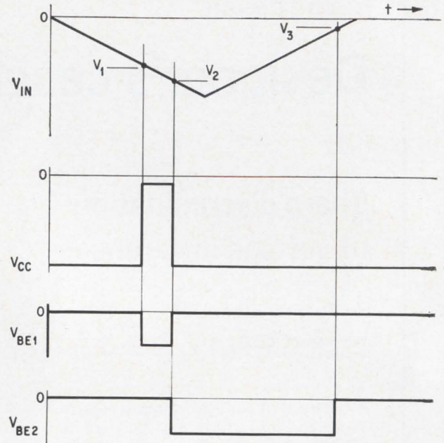
Voltage waveshapes show circuit operation for a triangular input voltage. When Q_2 turns on, circuit returns to off condition.
