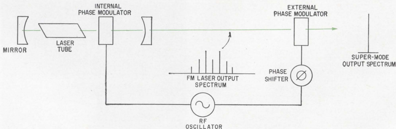
The supermode laser , with a second phase modulator placed outside the laser cavity. The second modulator, 180° out of phase with the first, nulls the f-m sidebands and produces a single mode of greater amplitude.
