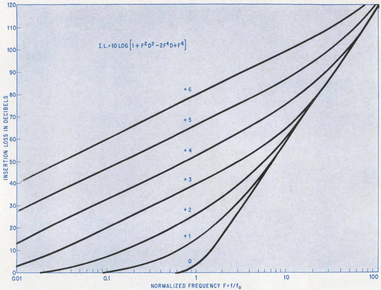
Insertion loss versus frequency response curves for the parameters numbered 0 through + 6.
