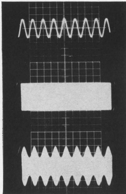
Tuned a-m modulator circuit. The 250-cps signal varies the gate's polarizing voltage, amplitude-modulating the 14-kc input signal to produce the output waveform, which is seen in oscilloscope photos at left.
