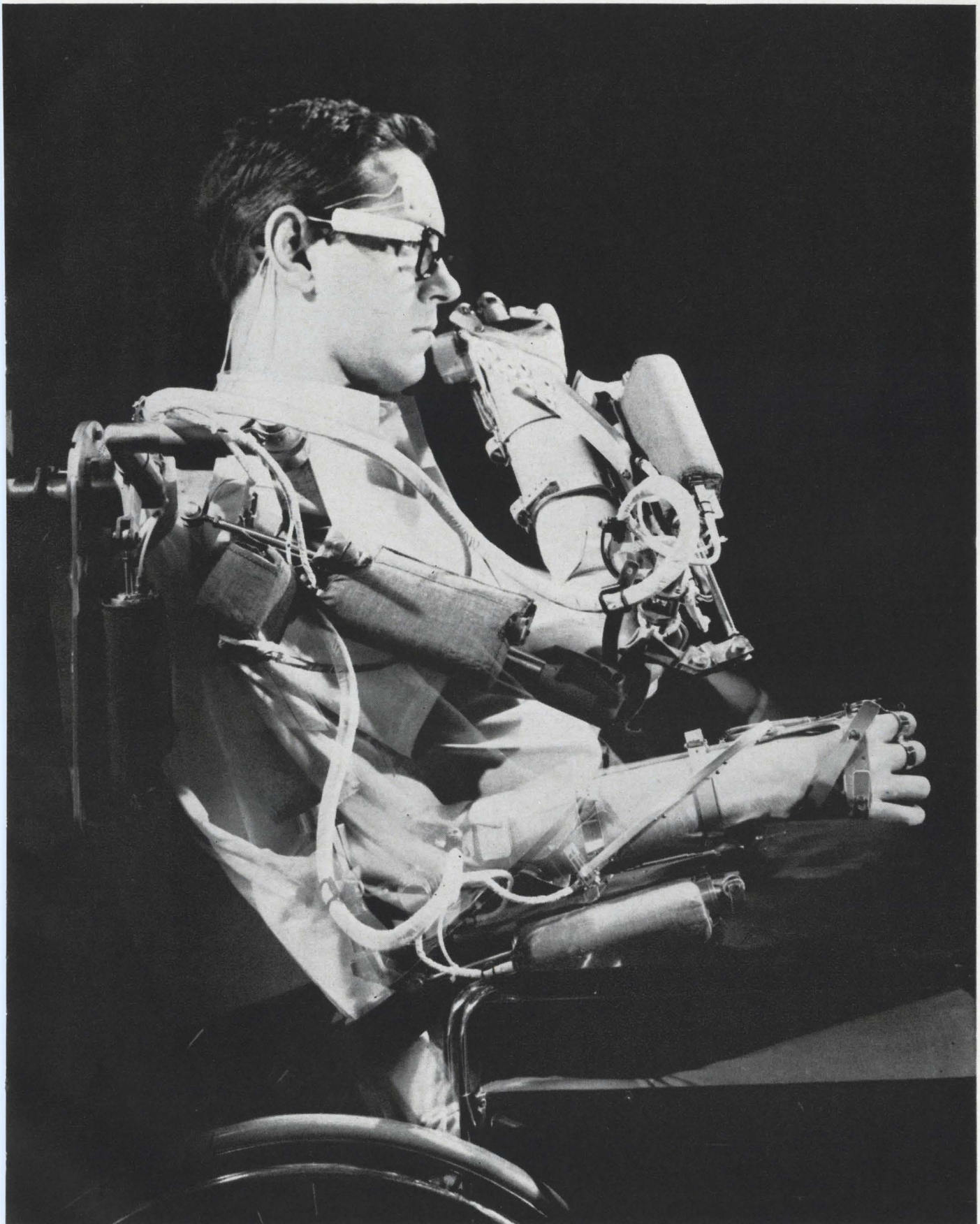
Arm aid worn by Edward Roszak allows six kinds of motion. Five of these movements, which involve the shoulder, elbow and wrist, receive their motive power from an external source. The sixth, the grasping of objects, is accomplished by electrical stimulation of a muscle with command signals originating at another muscle.
