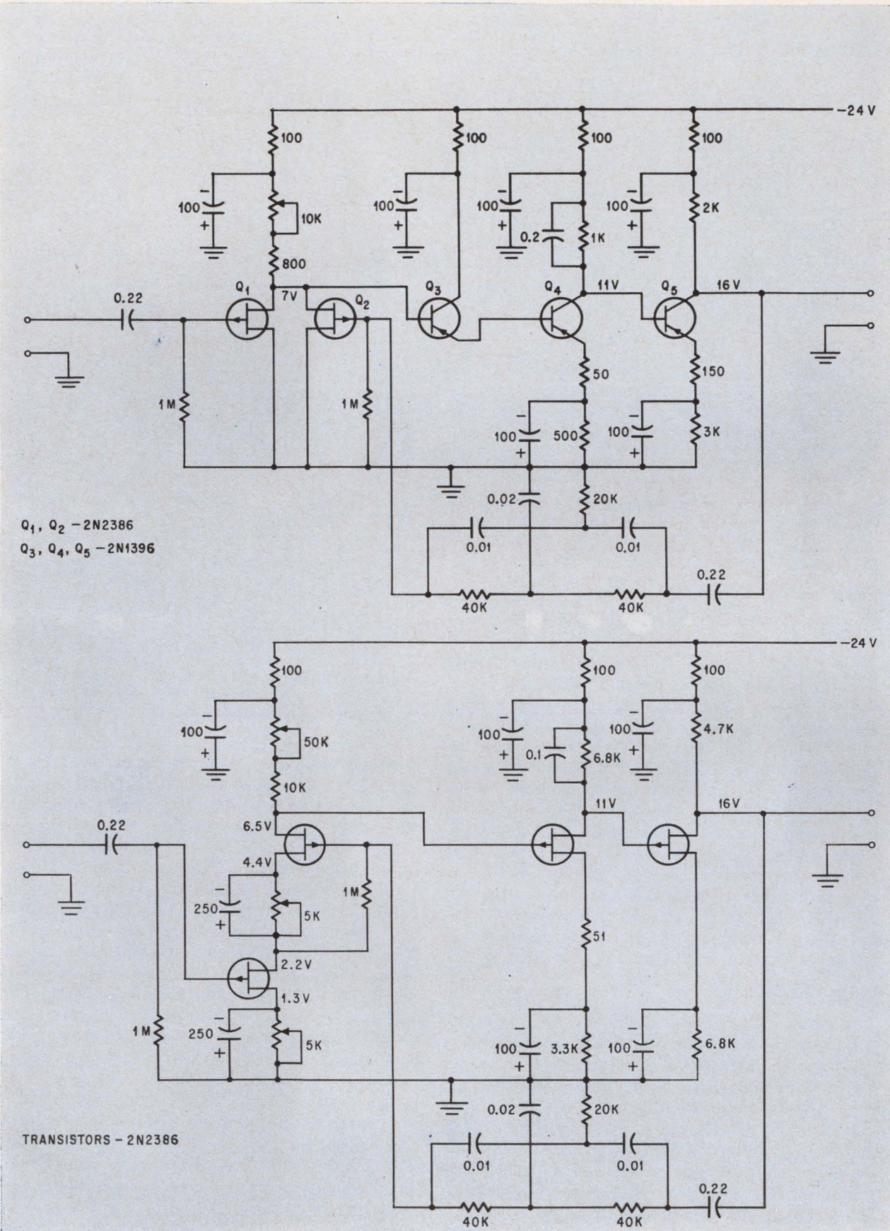
Complete parallel-T feedback amplifiers constructed with both drain-coupled, (top), and cascode adders. The performance of each of the circuits as part of the a-c bridge system is shown in the table on the preceding page. The values of the filter network in the feedback loop were selected for operation at 400 cps.
