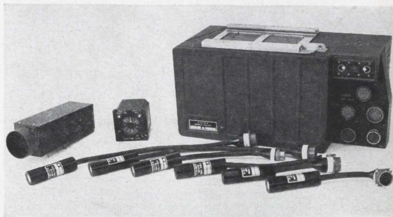
Compact assemblies make up the auxiliary data annotation set (ADAS). The special recording head assemblies are in the foreground; behind them (left to right), is the cockpit test display unit, time insertion unit, and the auxiliary data translator unit.
