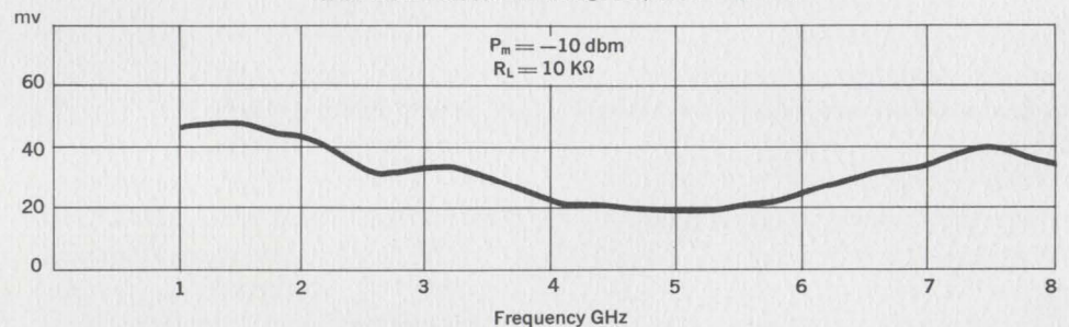
VIDEO DETECTOR D-5233 voltage output vs. frequency
