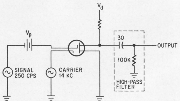
Tuned a-m modulator circuit. The 250-cps signal varies the gate's polarizing voltage, amplitude-modulating the 14-kc input signal to produce the output waveform, which is seen in oscilloscope photos at left.
