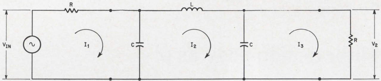
Pi-filter circuit inserted between source and load to obtain a required amount of attenuation at a specific frequency.
