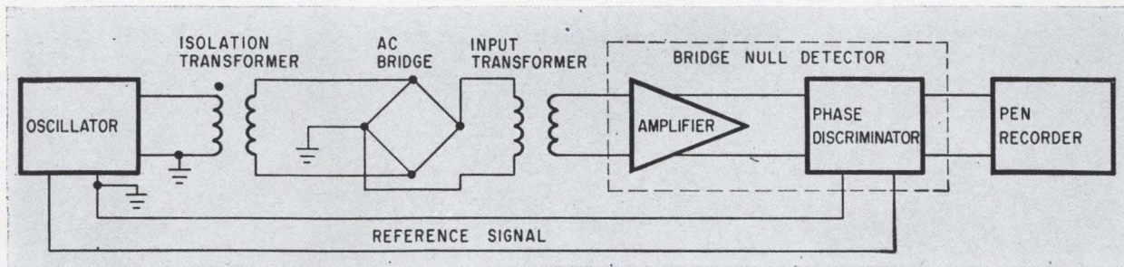
A-c bridge system generally uses pen recorder for visual observation of the null point. Most of the problems which effect bridge accuracy are centered in the null detector circuits.
