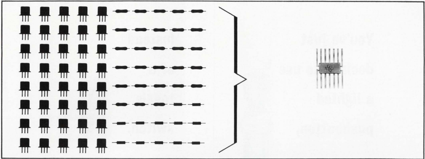
These 32 npn and 8 pnp transistors, 28 resistors and 12 capacitors (3/4 actual size) are replaced by the dual J-K flip-flop shown actual size above.
