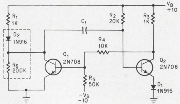
Addition of diode D_2 and resistor R_6 make a conventional monostable multivibrator immune to most noise pulses.
