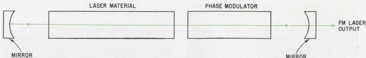
Diagram of an f-m laser shows that a phase modulator, in this case a crystal of potassium dihydrogen phosphate, has been placed inside the laser cavity. It is driven at a frequency which is almost that of the band separation of the laser modes. Phase modulation robs laser oscillations of energy, and produces an f-m output with controlled phase and amplitude at frequencies near those of the laser modes. One such output is shown in the second photo of the sequence on page 103.
