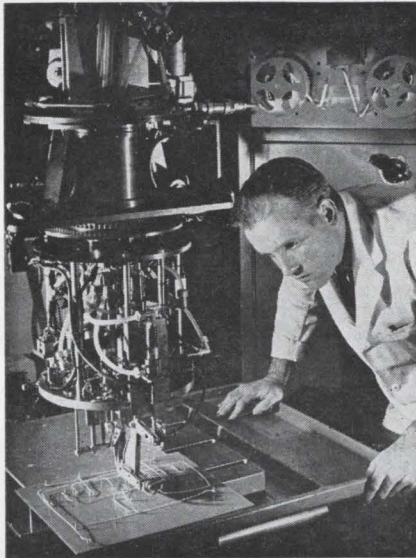
Wrapping machine lays out wires and wraps joints on flat circuit panel.
