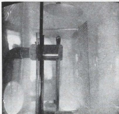
Silicon wafers (labeled substrate in sketch) are mounted on screen in first photo. In second photo, wafers are being coated with glass from the target electrode. Haze seen in second photo is the sputtering plasma.
