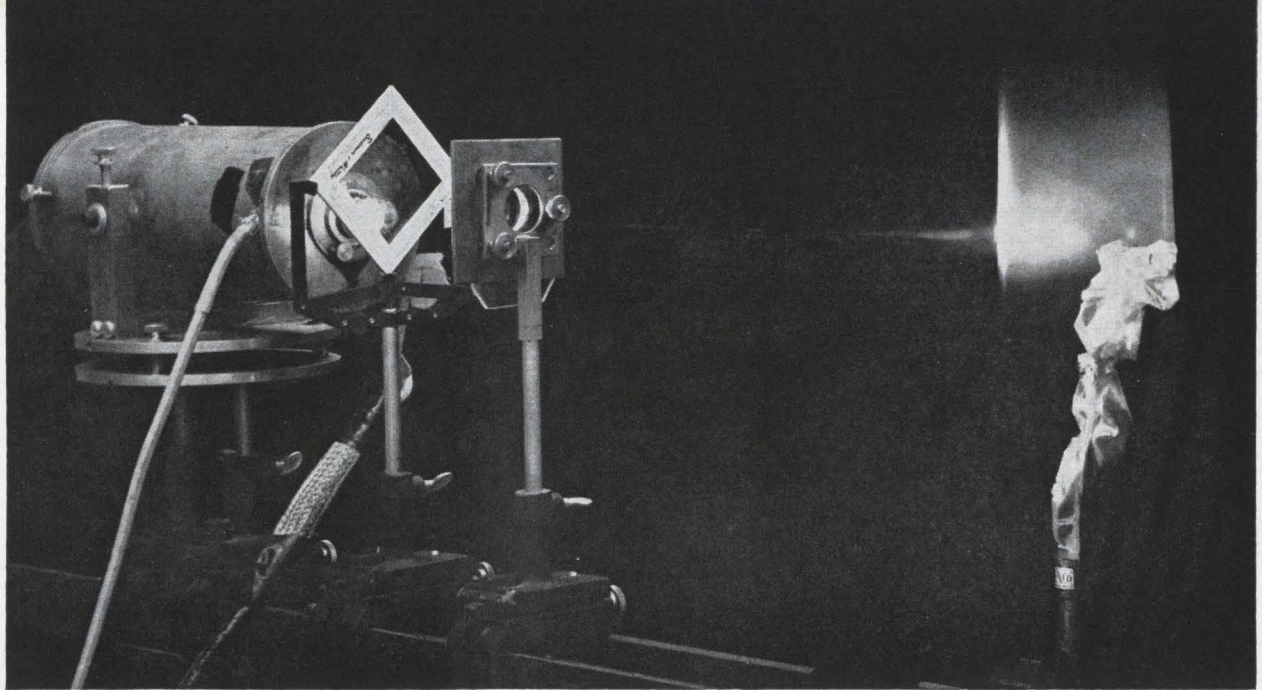
Multiple-exposure photograph shows multimegawatt Q-switched laser beam bursting a balloon. Thin film (passive Q switch) is clamped in diagonal position.
