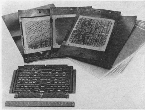
Multilayer boards raise interconnection density by increasing the amount of wiring in a given volume. This board was made by Autonetics for use in aerospace computers. The flatpacks are mounted on conduction-cooling strips.
