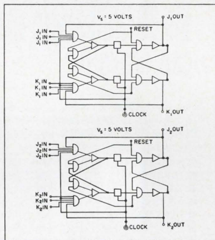
Block Diagram of Dual HLTTL master slave JK flip-flop
