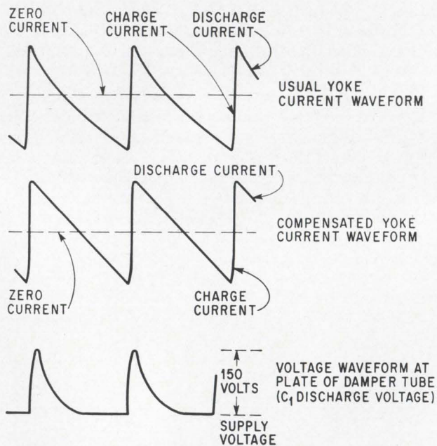
Discharge voltage of C_1 in plate circuit varies damper tube impedance. Result is linear yoke current during entire discharge interval and elimination of distortion at the left side of tv image.
