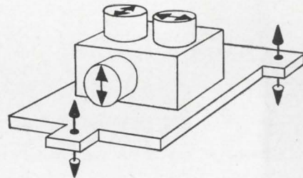
Accelerometers orthogonal within 5' of arc. Mounting surface adjustable \pm 2^\circ of arc.
