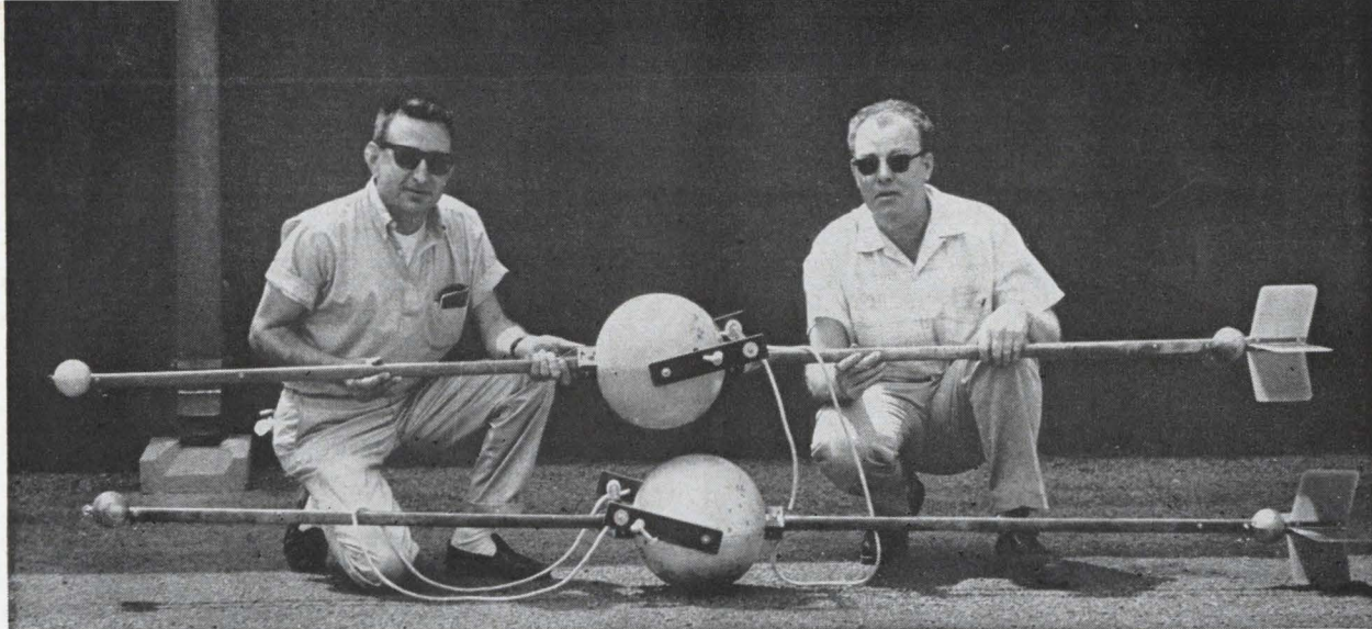
High-frequency Xeledop , equipped with fins for horizontal polarization, assembled and ready to be loaded on plane. Second Xeledop is kept in plane as spare. Only one unit can be flown at a time.
