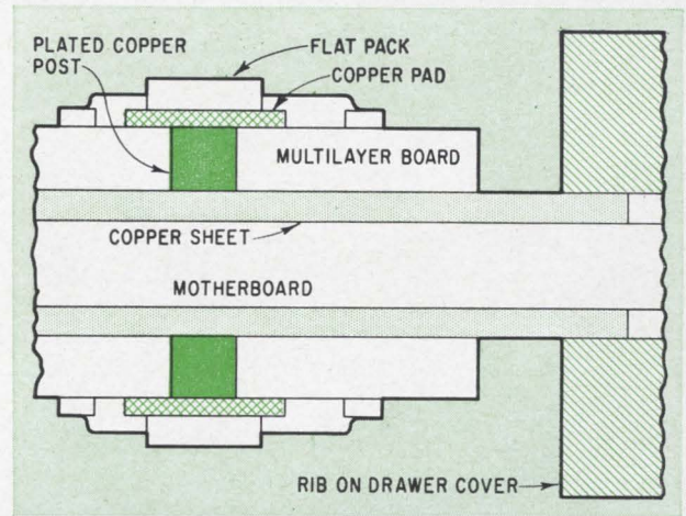
Thermal path in Litton Industries, Inc.'s prototype computer [see Part I of this report] Electronics, for the L-300 series. Since Part I was printed, Litton has revealed that the Level I boards in production models will not be small modules, but boards carrying 270 flatpacks. Two boards will be mounted back-to-back, and use a similar form of conductive cooling.
