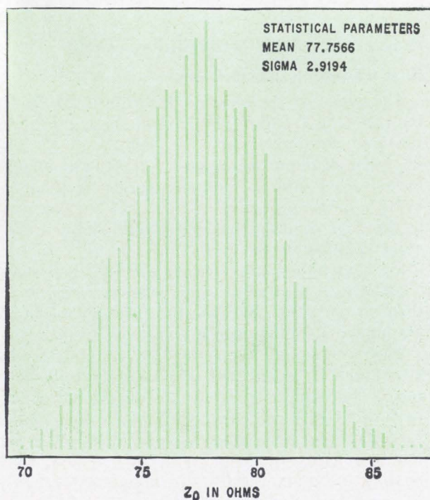
Distribution of characteristic impedances of 10,000 lines.
