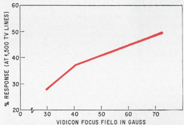
Reducing the beam cross-section in a vidicon tube by increasing the tube's magnetic focusing field can improve the camera's resolution significantly.
