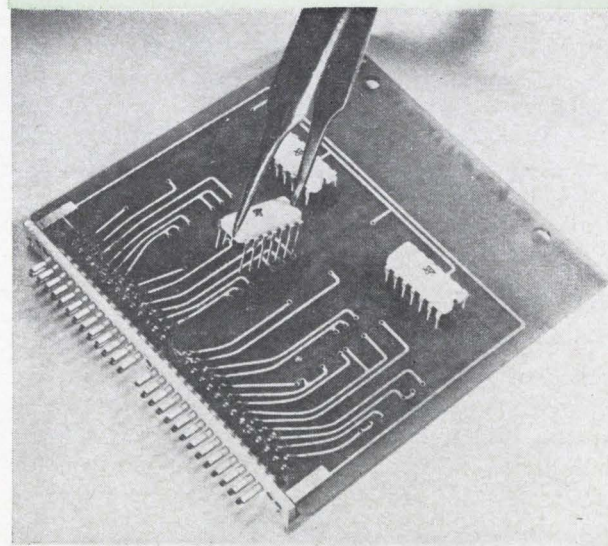
In-line packages for MIC's make assembly easier. This one, made by Sylvania, is one of several designs that are available. They can be plugged into circuit boards and solder joints made by dip or flow soldering.
