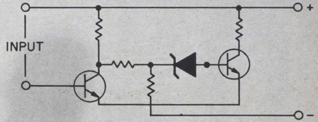
Noise Immunity Zener Diode provides voltage threshold which must be exceeded before transistor will conduct thereby eliminating false triggering.
