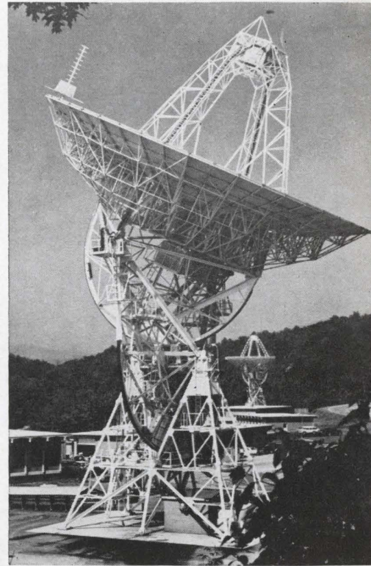
This 85-ft dish at Rosman, N.C. receives video signals from the Nimbus weather satellite. Later they go through a rapid photo-processing system to produce 70-mm negatives showing the earth's cloud cover.
