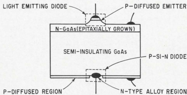
Light-coupled negative resistance device with quantum gain of about unity. Refraction and reflection losses are small because all radiation remains within the structure.
