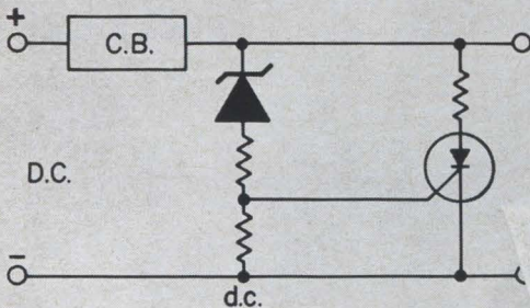
Over-voltage protection using a Zener Diode with an SCR and a circuit breaker will clear over-voltage faults. Both AC and DC circuits can be protected.
