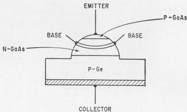
Heterojunction optical transistor with gain near unity has been proposed. The hemispherical mesa has a reflecting coating that reflects the infrared radiation to the collector junction.
