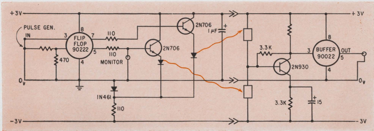
Optical coupling as used in a push-pull amplifier circuit. Circuit diagram shows gallium-arsenide injection diodes and high-speed silicon photo-conductors with a single stage of transistor gain.
