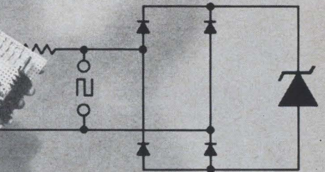
AC regulation Zener Diode used in symmetrical clipper circuit for square wave generation or surge protection where regulated AC output is desired.
