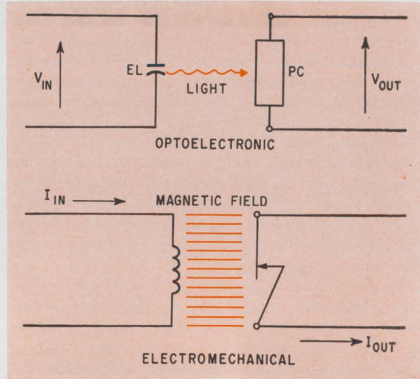
Optoelectronic device compared with a relay. A voltage across an electroluminescent cell corresponds to a current through a relay coil, light generated by the cell corresponds to the coil's magnetic field and the photoconductor cell is analogous to the relay contacts. Unlike a relay, however, a photoconductor can have a continuous change in resistance.
