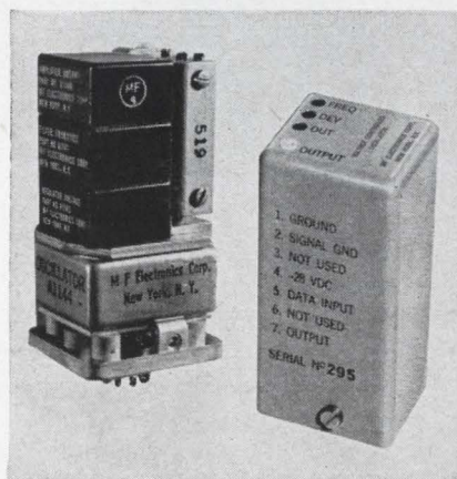
Series 300 voltage-controlled oscillator is assembled from reliable, dice-size electronic building blocks to give versatility in performance (left). Test point and potentiometer adjustments for output, deviation and center frequency are accessible through the cover (right).
