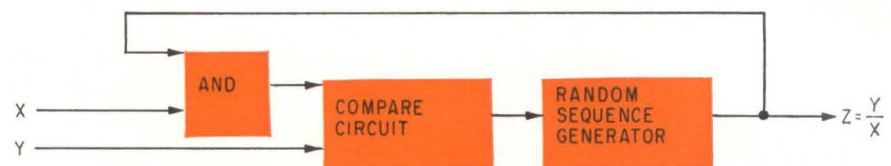
Ordinary AND gate, a comparator, and a pulse generator compute the quotient of two analog quantities.
