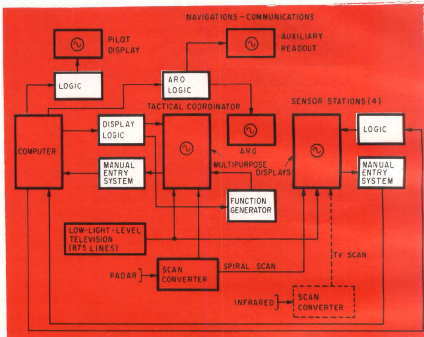
In the A-New system now being evaluated, computer-generated commands and data are transmitted through logic boxes to cathode-ray tube displays. In the production model the interface hardware, shown in white, will be replaced by a single unit. The infrared system is still being evaluated.
