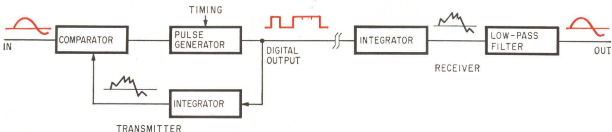
Delta modulation circuit, at left, integrates output pulses and compares resulting wave with the input signal (curve in color at the left). Output pulses, also in color, represent derivative of signal waveform—not the amplitude. In the receiver at the right, input pulses are integrated and filtered to recover original waveform.
