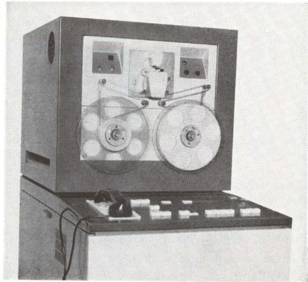
Parallel data transmission unit reads standard eight-hole paper tape and transmits the data in parallel over eight telephone lines. Two more telephone lines transmit control signals between the transmitter and receiver. This unit is a prototype.
