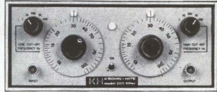
MODEL 3100 , one of the new K-H all-silicon Broad Band Variable Electronic Filters providing continuously adjustable bandwidth over the range of 10 Hz to 3 MHz maximum bandwidth.
