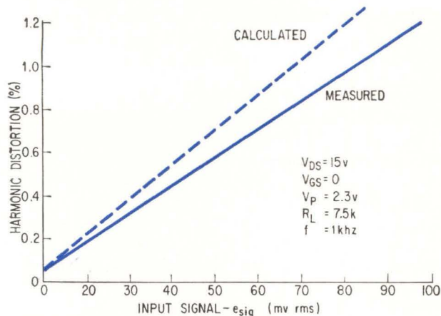
Harmonic distortion is directly proportional to input signal level. Calculated curve is plotted from equation 5.
