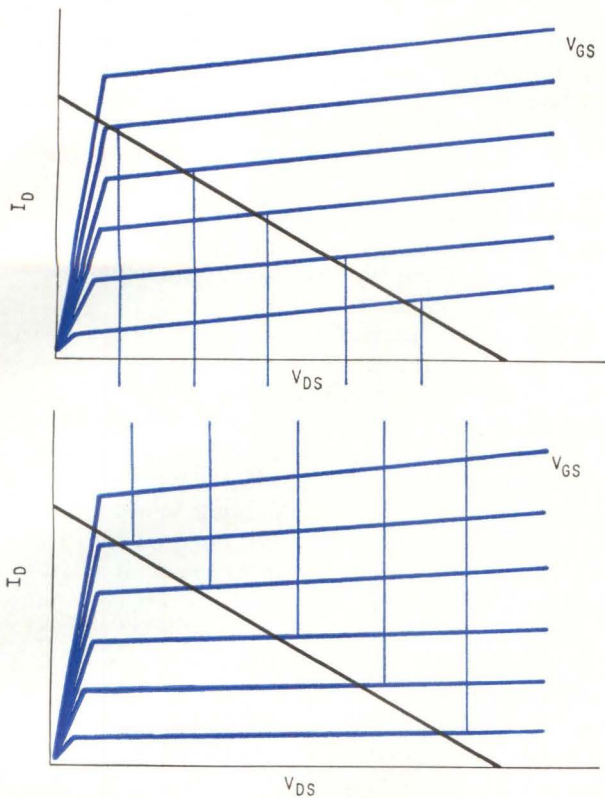
Idealized FET output characteristics are drawn to show (top) constant g_{fs} , constant g_{oss} and (bottom) constant g_{fs} and nonconstant g_{oss} . Transconductance g_{fs} is constant because for a given value of V_{DS} distances between V_{GS} curves are constant. Transconductance g_{oss} varies when slopes of V_{GS} curves vary.
