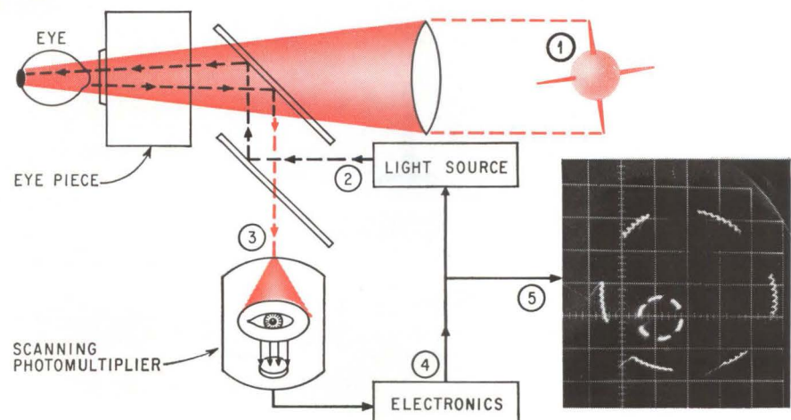
Guiding a vehicle with the Honeywell Oculometer is as easy as keeping your eyes open.
