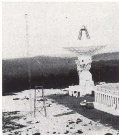
Cyclope 2 precision antenna at Landes tracking center covers frequency range from 216 Mhz to 2,300 Mhz. Gain is 45 db at 2,300 Mhz.
