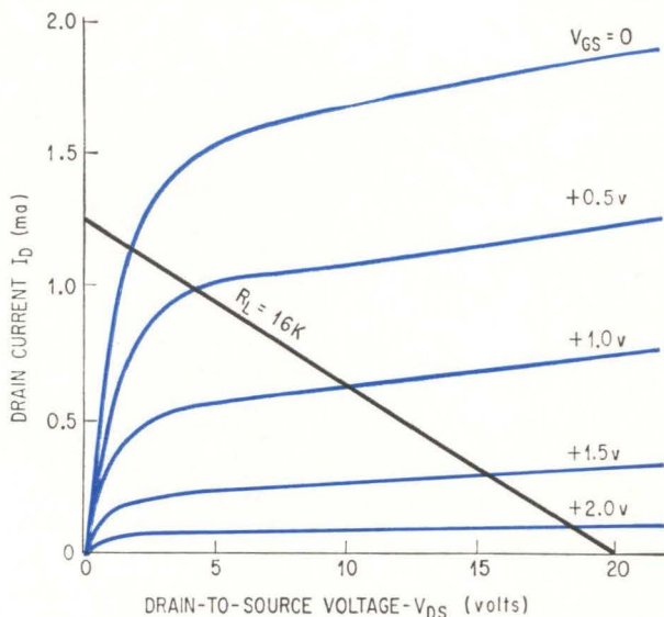
Forward transconductance, g_{fs} , a function of the output characteristics, increases as V_{GS} goes to zero and operating point moves up and to the left along load line. This causes second harmonic distortion. However, as drain current, I_D , decreases, so does common-source output conductance, g_{oss} , also a function of the characteristics, introducing more distortion.
