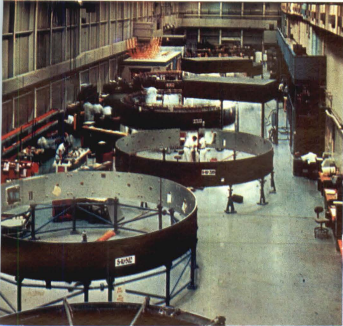
On a production line in a special plant in Huntsville, Ala., IBM turns out the ring-shaped instrumentation units that control the vehicle during takeoff.
