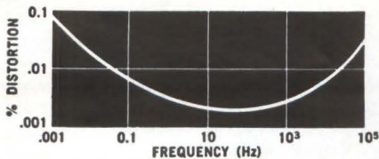
TYPICAL HARMONIC DISTORTION PLOT of K-H Series 4000 R-C Variable Frequency Oscillators.
