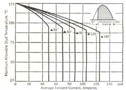
Current capability of Westinghouse Type 218 Thyristor
