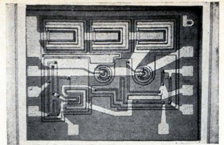
Versatility. Philco-Ford circuit can operate as three different kinds of amplifier, depending upon the choice of off-the-chip devices.
