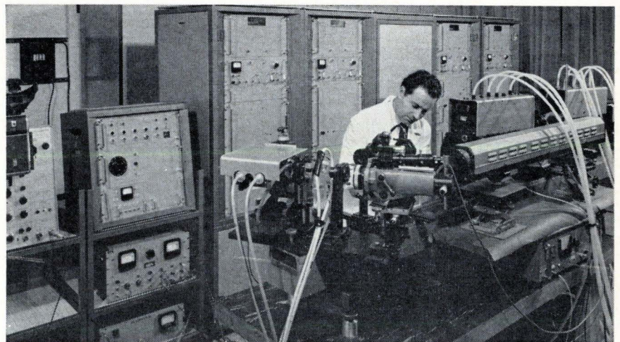
Giant laser. Powerful new system is available in two configurations: high power or high brightness.
