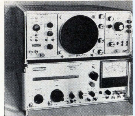
Two-in-one. New receiver to check RFI is two instruments in one: a module that displays spectrums and an analyzer of interference.
