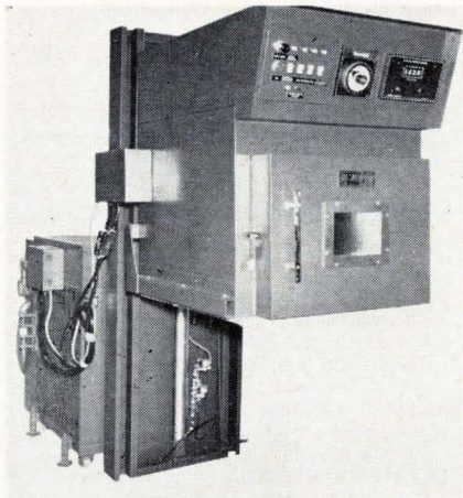
On top. Digital control instrumentation mounted atop environmental chamber cycles temperature between limits of +155°C and -65°C in 20 minutes. Temperature is read out on four-digit display.
