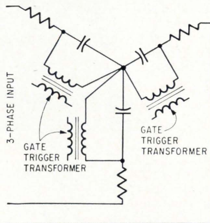
Input phase. Gate-trigger transformers are Y-connected across three-phase input line so that scr gates are triggered from line-to-neutral voltage, rather than from line-to-line.
