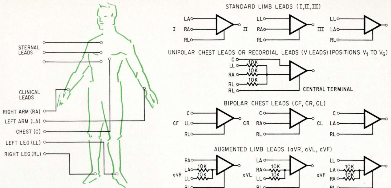
Lead arrangements. For the unipolar electrocardiographic chest lead, the exploring electrode is moved to six positions on the chest, resulting in the V_1 to V_6 designation. In more recent electrocardiograph setups, lead arrangements can be switched without moving the electrodes around.
