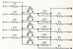
UD-4037 BUFFER AMPLIFIER
