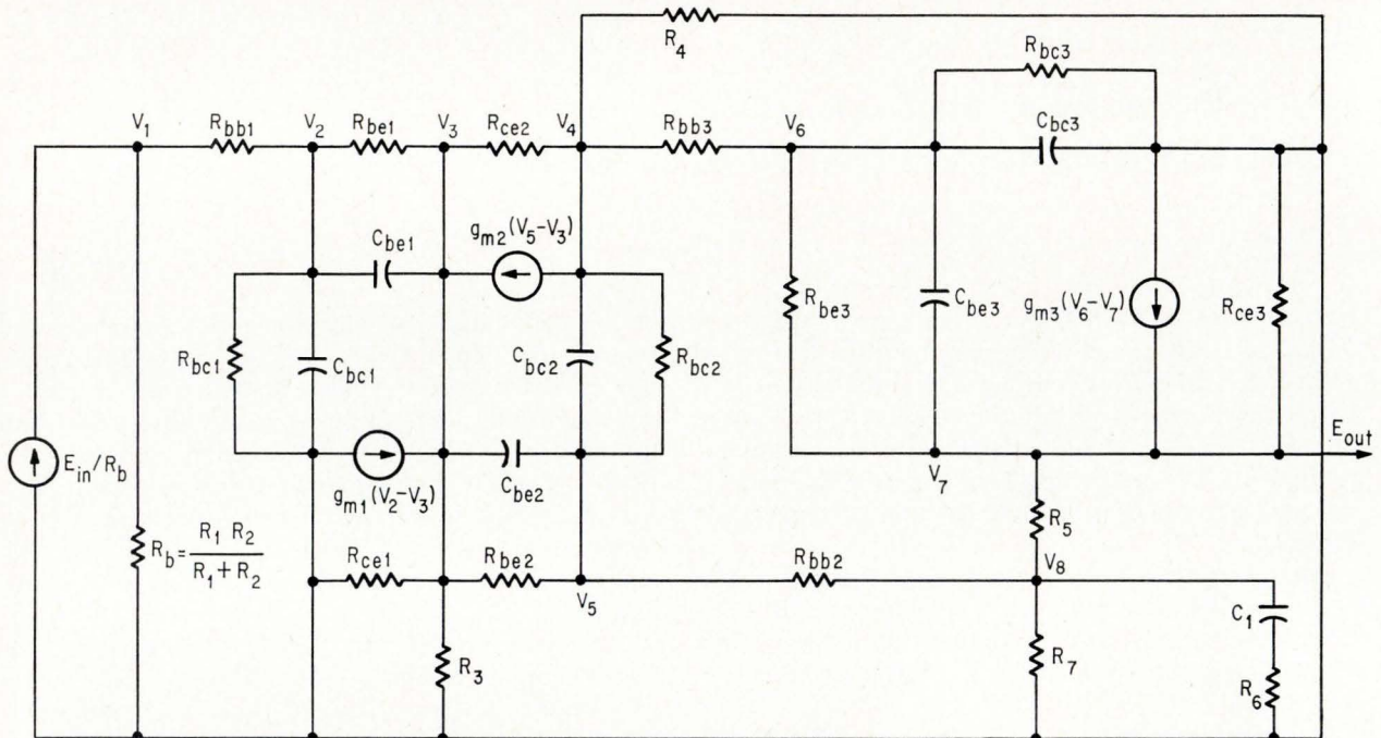
Equivalent circuit of video amplifier, too complex to handle manually, provides good accuracy.
