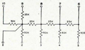
UT-1000 LADDER NETWORK
