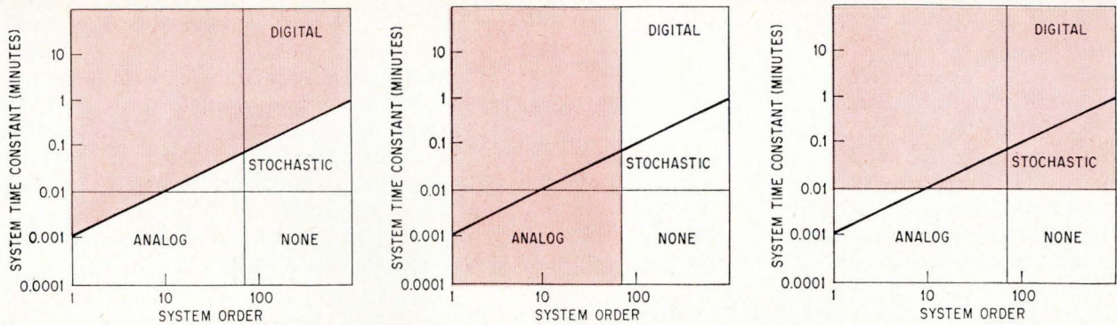
Approximate regions of application for digital (left), analog (center), and stochastic (right) computers. Analog computers are limited mainly by system order (number of differential equations), while digital computers are limited in both size and speed. Stochastic computers are limited by speed but not by size. Advances in digital computers are steadily shifting the diagonal line toward the right, but a large area remains uncovered.
