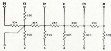
UT-1001 LADDER NETWORK
