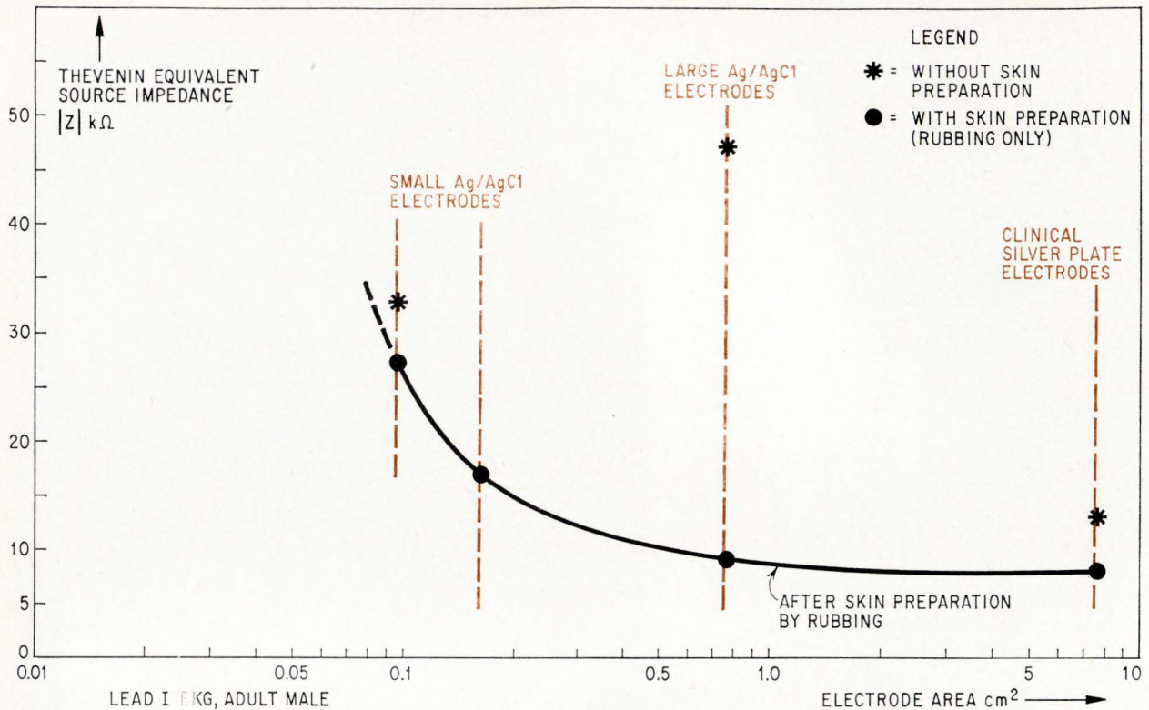
Impedance and surface. Electrode area isn't the only factor that changes electrode impedance. The curve demonstrates how surface area and the condition of the skin influence the source impedance.
