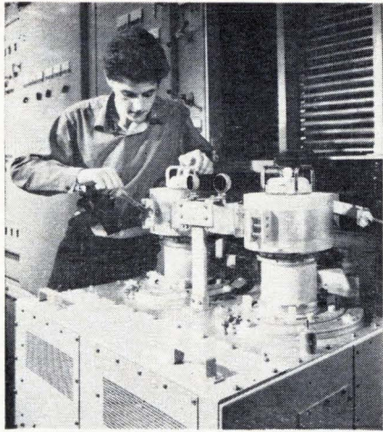
Long-wave transmitter. Two big air-cooled tetrodes provide the final amplification in new 100 kw transmitter.
