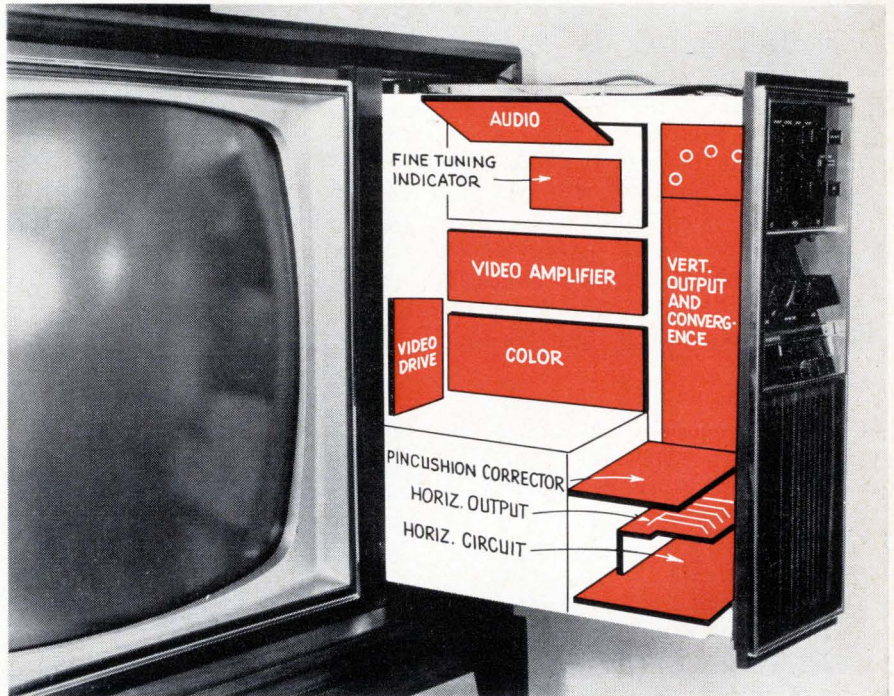
Slide out. All the electronics in Motorola's new line of color-tv sets are packaged in plug-in modules that can be slid out on a pull-out drawer.
