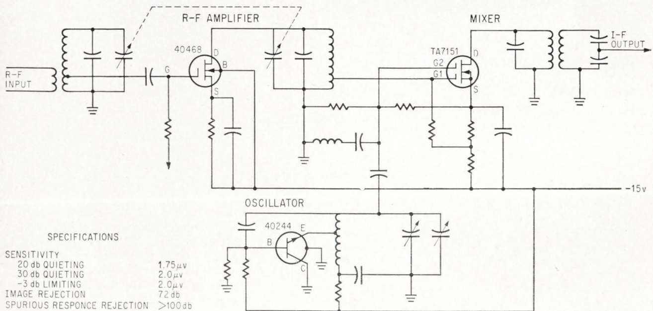
F-m mixer. The dual-gate feature of the MOS FET provides high spurious response and image rejection. Performance measurements were made across 300-ohm antenna terminals with the input frequency at 100 Mhz, modulated by a 400-hz signal with 22.5-khz deviation.
