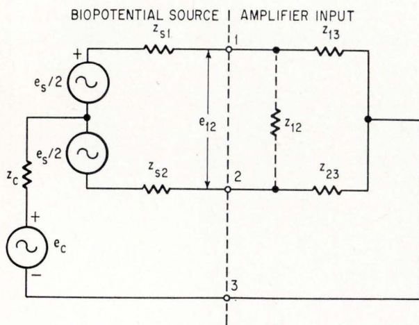
Simpler circuit. Assuming electrode pellet, gel resistance, and the electrode-difference voltage to be zero reduces equivalent circuit's complexity. This circuit permits rapid calculation of the common-mode rejection limits as a function of the source impedance imbalance.
