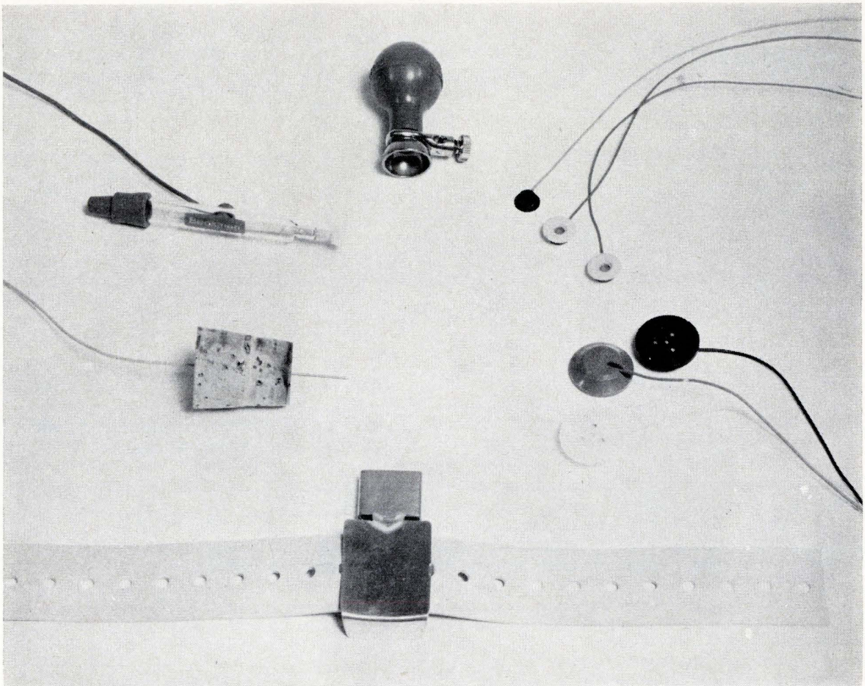
Typical electrodes. A variety of sensors are available to detect biopotentials. Clockwise from the bottom are: a standard silver plate EKG electrode with its mounting strap; a needle electrode used by researchers to record animals' EKG's or to sense myoelectric potentials, a silver-silver chloride salt bridge tissue electrode, a standard EKG suction-cup electrode, miniature silver-silver chloride electrodes for EKG's or EEG's, and low-artifact silver-silver chloride electrodes for EKG's.
