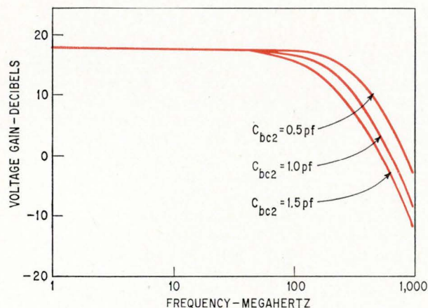
Bandwidth varies as a function of base-collector capacitance of the second transistor stage. Bias current is constant at 10 milliamperes and R_6 is 51 ohms.
