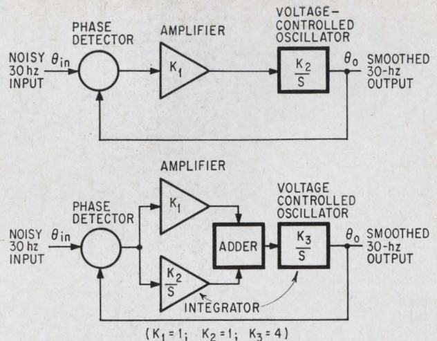
Locked loops. Double integrator phase-locked loop (bottom) locks the output in both frequency and phase to the input. Phase-locked loop with but a single integrator (top) provides only frequency lock.
