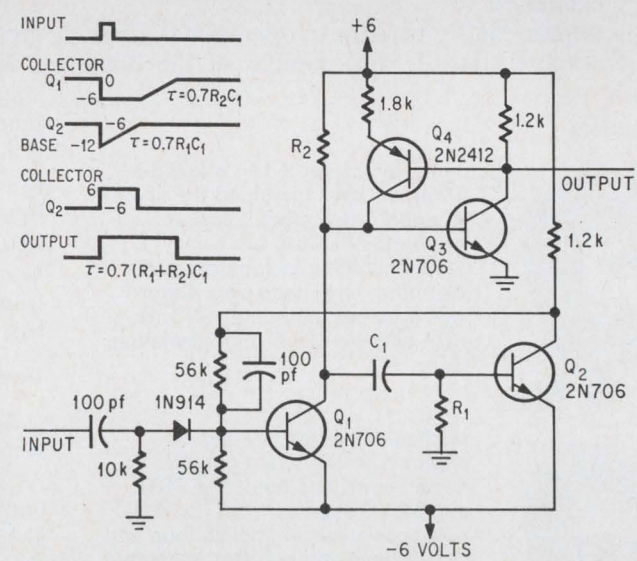
Double duty. Capacitor, C 1 , controls the timing of the output and delays the setting up for the next cycle.
