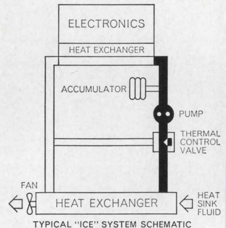
TYPICAL "ICE" SYSTEM SCHEMATIC
