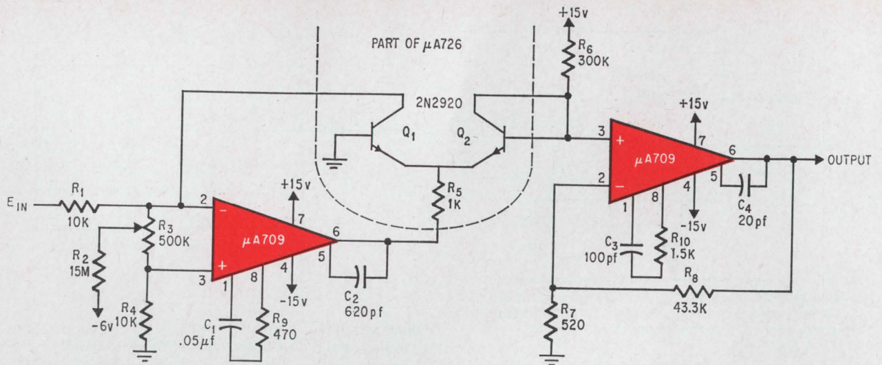
Log. A logarithmic amplifier is formed by two \mu A709 operational amplifiers and a transistor pair from the \mu A726 temperature-compensated differential amplifier. The 709's provide gain and broad bandwidth, while the 726, only connected as a feedback stage between the 709's, adds the two signal levels that are converted to log form.
