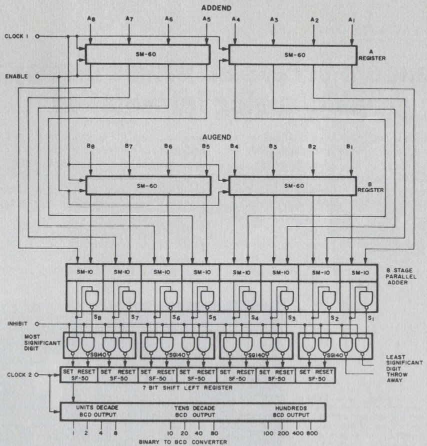
Fig. 2. TTL system simultaneously accepts an 8-bit binary addend (A), and 8-bit binary augend (B), adds and averages them and converts the result to Binary-Coded Decimal. BCD is a normal code for operating "Nixie" tubes, EL displays, digital displays and other types of CRT readout.
