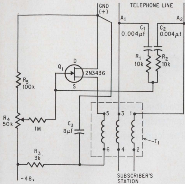
Feedback circuit. Longitudinal voltage is sensed at points A 1 and A 2 , applied to Q 1 , and reintroduced into the telephone line 180° out of phase via windings 3-4 and 1-2, effectively cancelling the longitudinal voltage.
