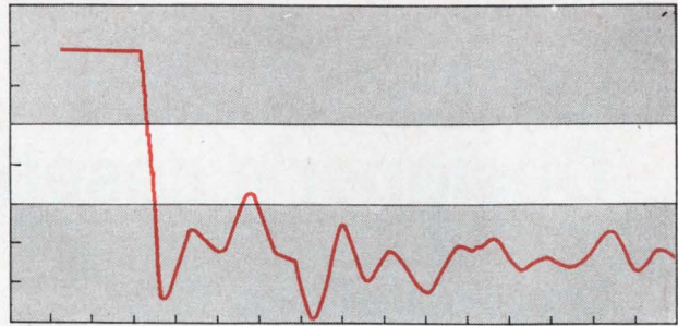
Connection delay. In the voltage waveform obtained at the end of a twisted pair connection, receiving element is switched after 62 nsec, but a reflected pulse breaks into threshold band at 113 nsec and lasts until 125 nsec. Worst-case design would allow for 125 nsec delay. Depending on actual threshold voltage, receiving element might produce stable output at 62 nsec.
