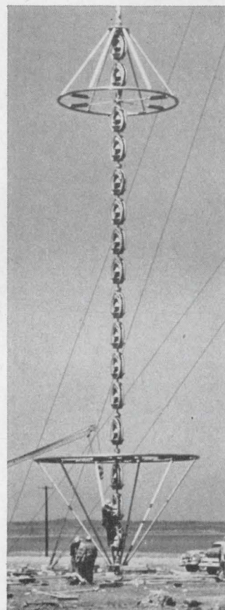
Special antenna insulator assembly with corona rings.
