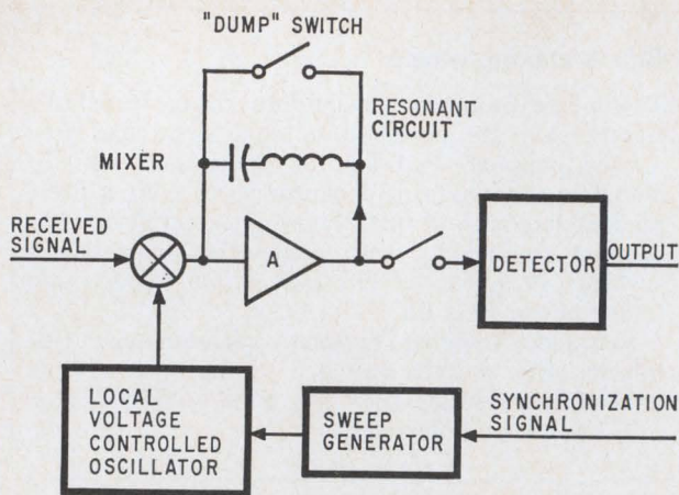
Correlation receiver. The synchronization signal constantly adjusts the frequency of a local VCO whose output combines in a mixer with the received Chirp pulse. The difference frequency between the two signals is amplified and sent back through a resonant circuit. Every T second, the circuit is shorted and the signal goes to the detector.
