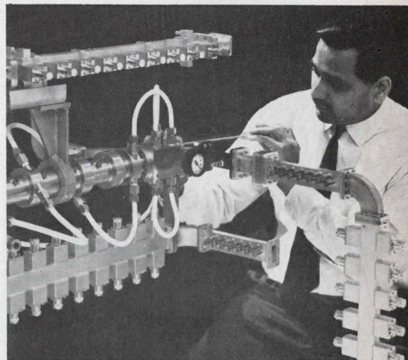
Plumber's dream. Waveguide filters provide 125 db isolation between transmitter and receiver.
