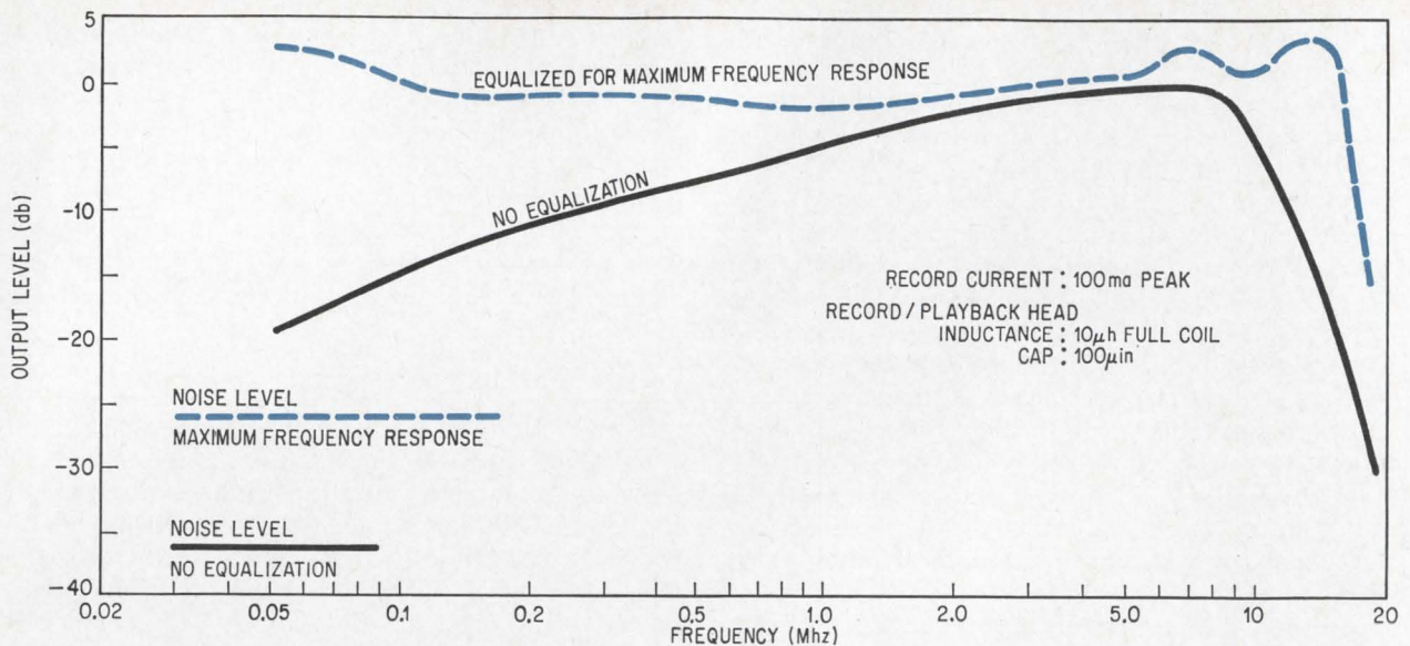
Flat response. Unequalized recorder frequency response is down 20 db at 50 khz and falls off sharply above 8 Mhz. With equalization, however, the curve is almost flat up to 15 Mhz.
