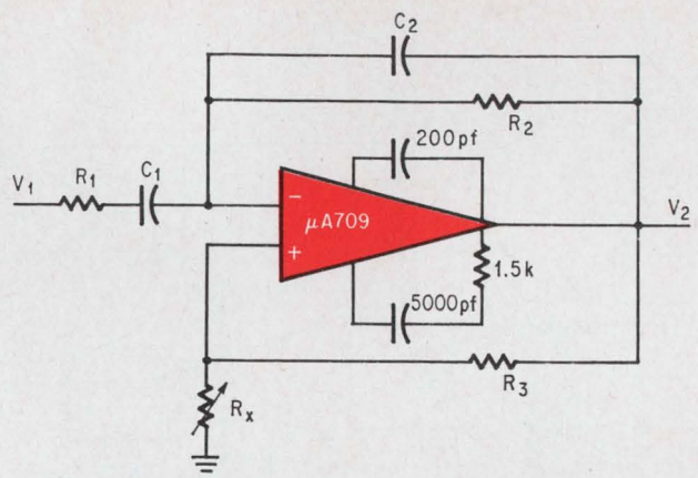
Band-pass filter. R_x establishes the Q of the circuit, and R_1 - C_1 and R_2 - C_2 set the limits of the pass band.
