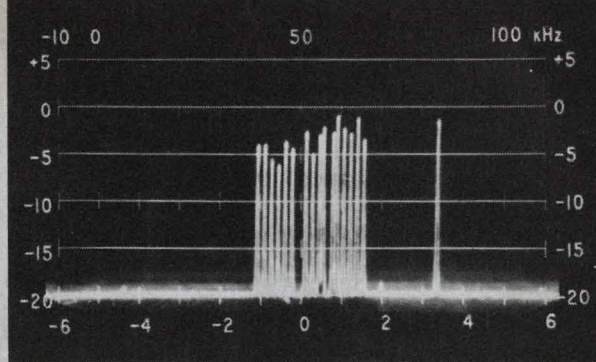
Three 4-kHz channels of L3 carrier multiplex system. Center channel has teletype subcarriers. Model 360A is in 12-kHz sweep width mode, sweeping from 6.780 to 6.792 kHz.
