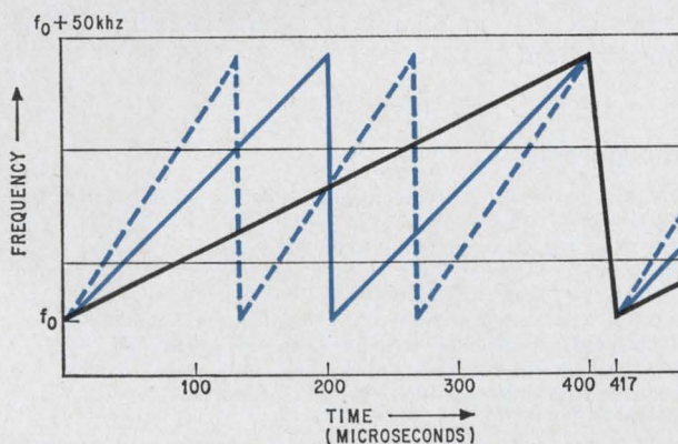
Asynchronous system. Many signals can be sent simultaneously over the same bandwidth by assigning a different slope to each. Here, three signals are sent, each taking a different number of sweeps. A 17-microsecond delay occurs before transmitting next set of signals.
