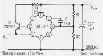
200mA Regulator
