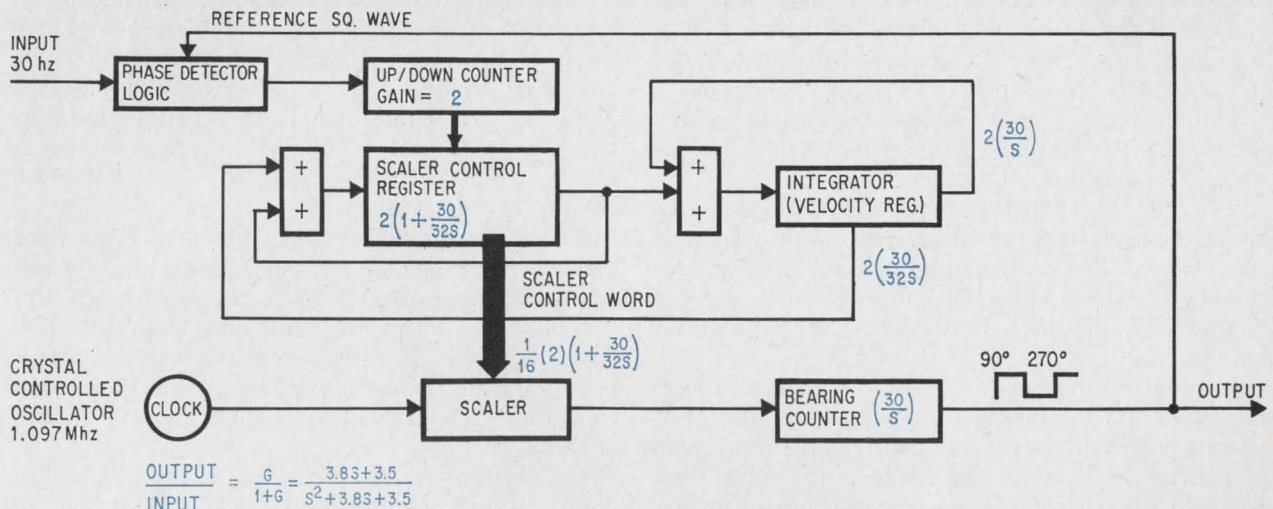
Double integrator loop. Complete digital phase-locked loop locks to frequency of 30 hertz \pm 1.5\% , is critically damped and has undamped natural frequency of approximately 1/3 hz.
