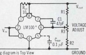
200mA Regulator
