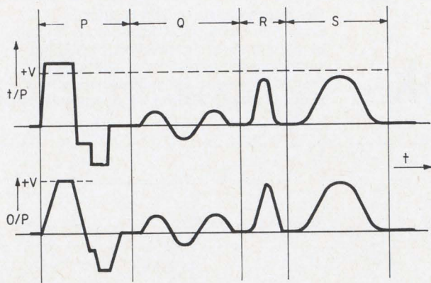
Waveforms. Slopes of waveforms P and R are limited by the circuit while Q and S are passed unchanged.
