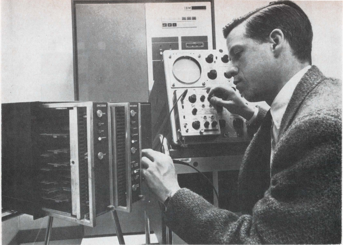
Testing. Author Frey tests Dacor, which is composed of an encoder and decoder. Tall unit at rear is a previous error-correction system made without IC's.
