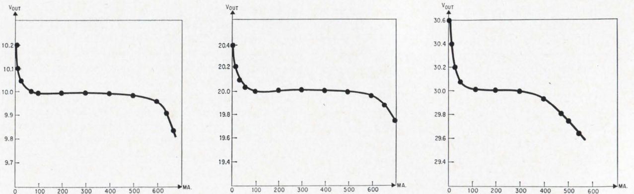
Voltage regulation curves. Power supply's regulation is 100% at 500 ma for output voltages of 10 and 20 volts d-c.
