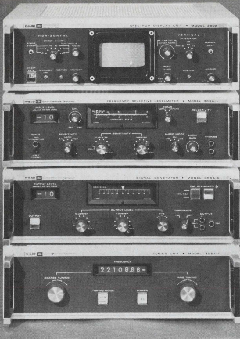
Three 4-kHz channels of L3 carrier multiplex system. Center channel has teletype subcarriers. Model 360A is in 12-kHz sweep width mode, sweeping from 6.780 to 6.792 MHz.
