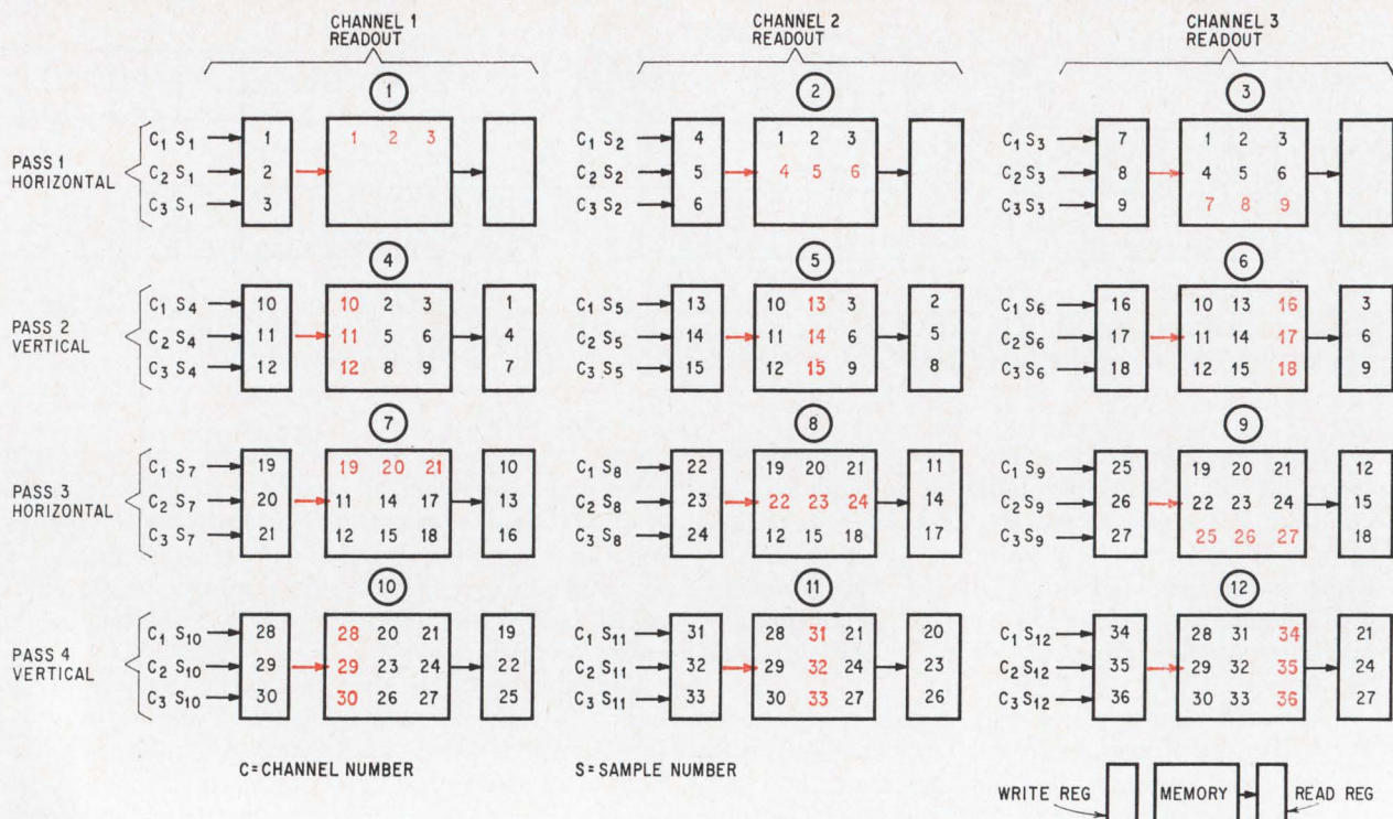
Cortic II. The memory can be kept full and can have a longer cycle time when samples from successive channels are stored alternately in rows and in columns of the memory. But here the ratio of channels to samples must be an integer, or the reciprocal of an integer.
