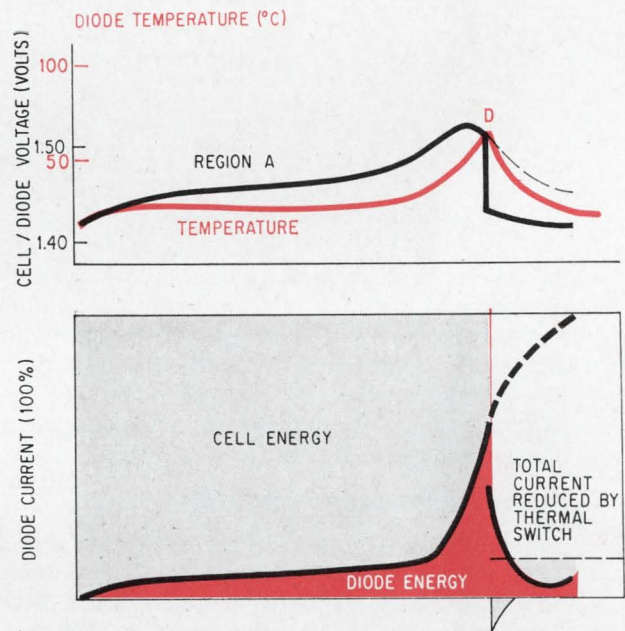
Charge curves. At full charge, point D, thermal switch opens to limit charging current which falls to a safe trickle charge level.
