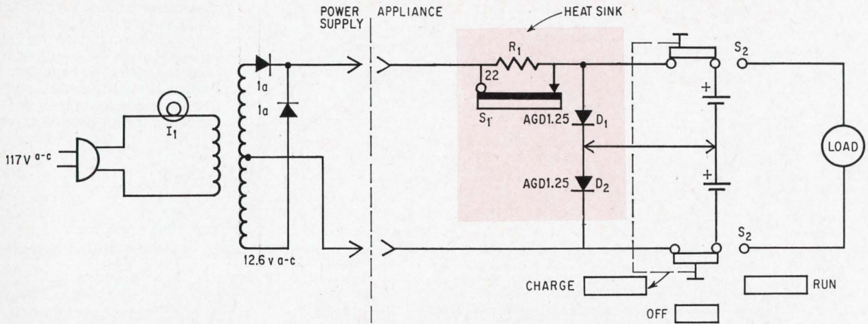
Two-cell appliance charger. A pair of diodes mounted on a copper heat sink with a thermal switch protects the cells during a 70-minute fast charge cycle. Lamp I_1 regulates charge current and serves as indicator.
