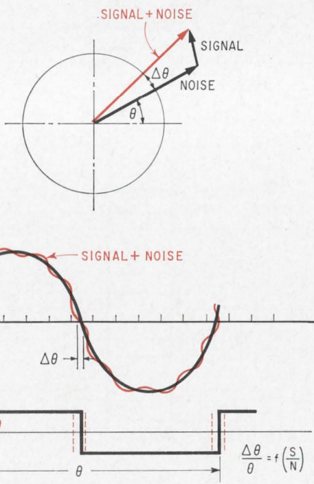
One-bit quantization. The small signal vector phase-modulates the large noise vector, so that the quantized signal is a square wave with uncertain zero crossings. The ratio of the uncertain zone width to the square-wave period measures signal-to-noise ratio.
