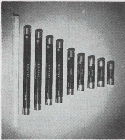
Plug-in. Cartridge rectifier stacks can replace high-voltage selenium units and tubes in X-ray and radar equipment.
