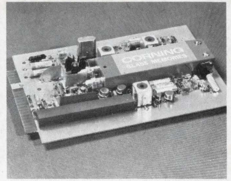
New Analog Glass Memory Modules delay video signals up to one horizontal scan time. Exits as the original input displaced in time by 63 microseconds. Just plug it in.
