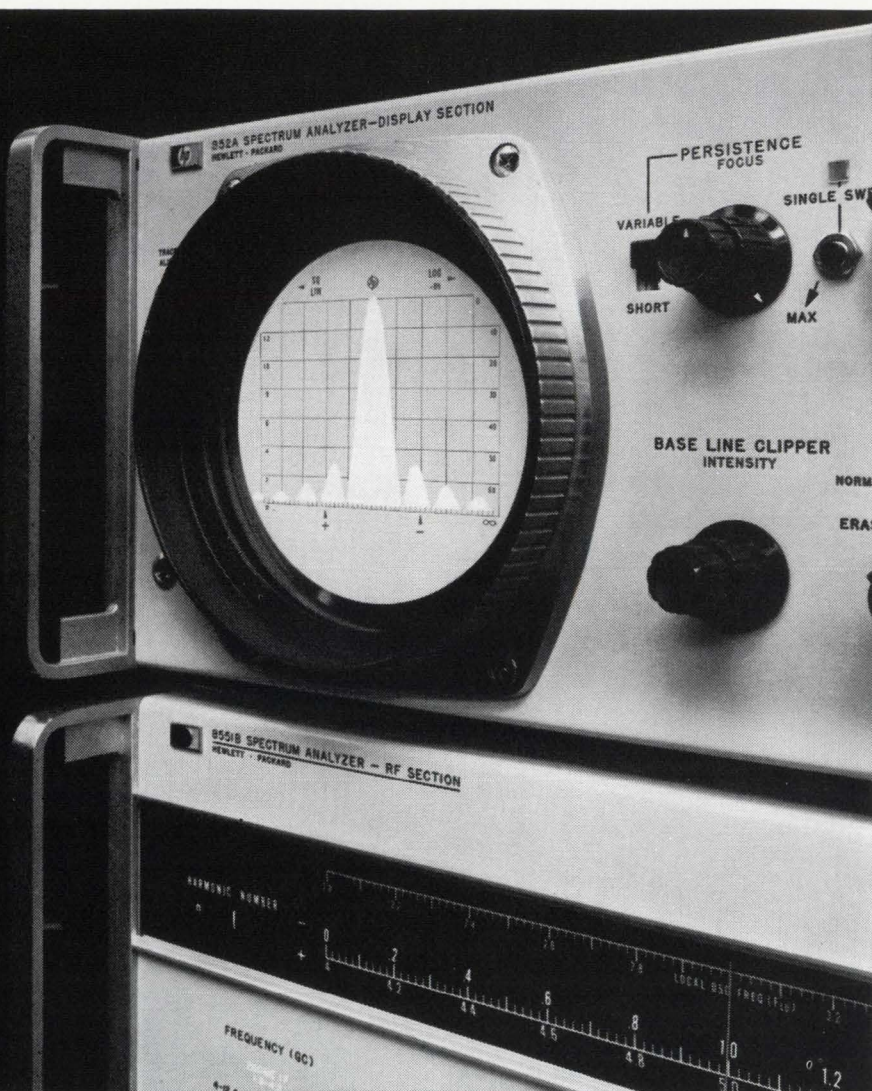
SPECTRUM OF 50 PPS PULSED CARRIER
