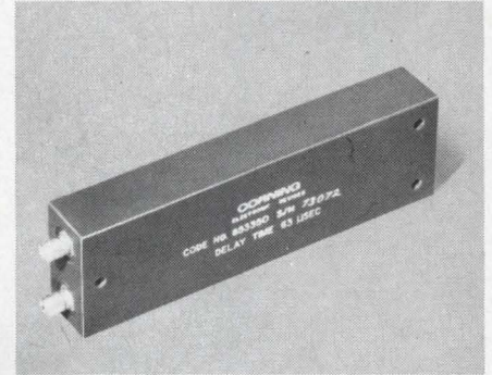
New 63 Microsecond Glass Delay Lines are high performance analog storage devices that let you work with bandwidths up to 15 MHz for video processing.
