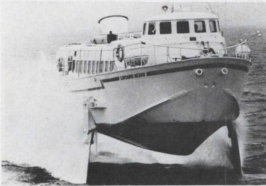
Over seas. The Dolphin-class hydrofoil on which two small dimples below the headlights house transmit and receive horns for sonic height sensor.
