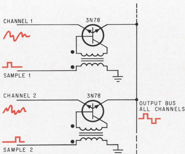
Analog gate. Built around a common dual-emitter transistor often used for chopping, this circuit transmits to the common output bus the instantaneous value of the slowly varying analog quantity. From this value, the converter determines a digital equivalent.
