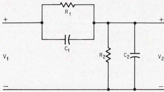
Four-terminal network
