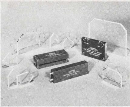
Zero-TC glass delay medium means lower cost per bit, less power per bit, than MOS.
