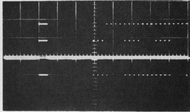
Original and compressed. The first few samples of three 50-hz input signals are at the right in each photo, with five-bit quantization in the photo at left and two-bit quantization at the right. The compressed signals are at the left in each photo; run together, the samples appear as short horizontal lines. The peak lines are brighter because the signal's sinusoidal shape causes more samples to be taken near the peaks.
