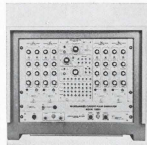
Programmed current pulse generator 1580A boasts a highly linear, 15-nsec rise time and a narrow pulse width into the load. Its program generator operates at a high-speed 5 Mhz and incorporates an 8-step programming capability which permits repetition of selected steps or step pairs within the predetermined pulse program. Computer Test Corp., 3 Computer Dr., Cherry Hill, N.J. [368]
