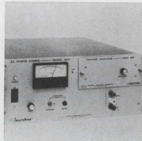
Solid state power amplifier 501T Invertron will provide 500 va of power variable from 45 to 5,000 hz, with half power to 10,000 hz. Selectable outputs supply 0 to 30 v, 0 to 75 v, 0 to 130 v, and 0 to 260 v. The overload level is adjustable from 10% to 150% of rated output. Price is $1,495. California Instruments Corp., 3511 Midway Dr., San Diego, Calif. [382]
