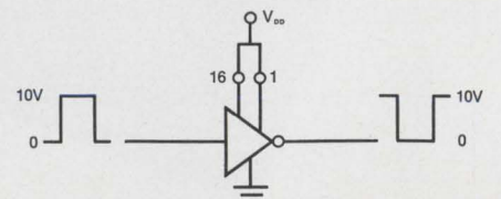
CD4009D as a COS/MOS to COS/MOS Inverter
