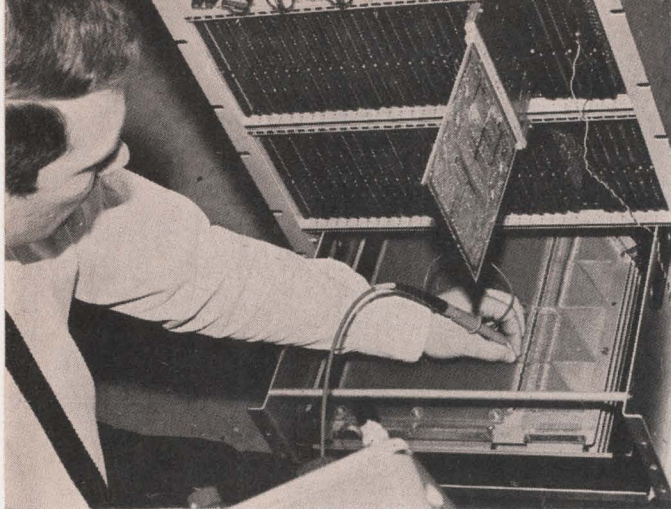
Minding the store. Plessey Ltd. livens up the brisk British computer market with plated-wire memories.
