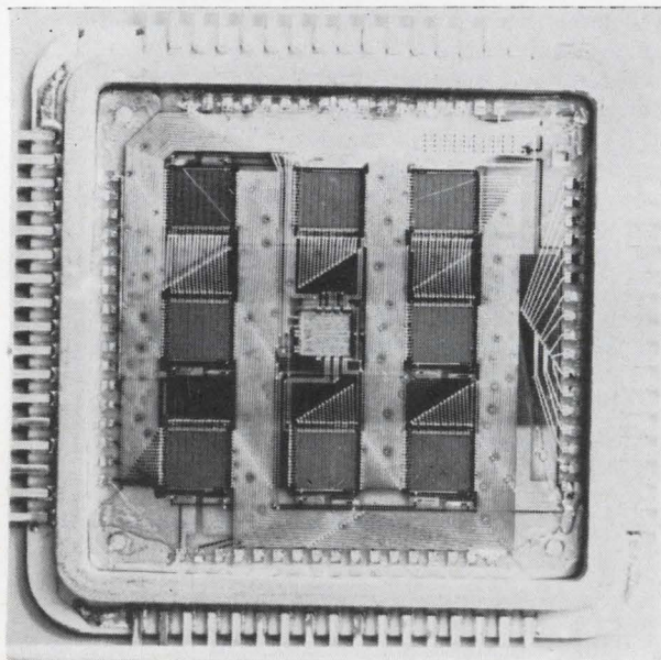
Surrounded. One package or subunit of the memory consists of eight MOS storage array chips surrounding one bipolar chip in the center. The multichip assembly comprises 2,048 bits of the memory. Four such packages form the storage portion of the 8,192-bit memory module. The complete unit has 32 MOS storage arrays of 256 bits each, four array selection chips, two decoding word driver chips, and four sense amplifier-digit driver chips.
