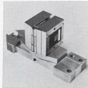
Dual-gap, nine-track, digital magnetic tape heads series HDG9 can be utilized for high density recording at 250 inches per second with fully compatible IBM formats. The series is composed of four models with packing densities of 3,200 flux reversals per inch at recording tape speed of 250 inches per second. Magnetic Head Corp., 95 Marcus Blvd., Hauppauge, N.Y. 11787 [427]
