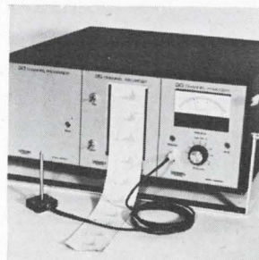
The Simulprinter model FS-5 is a new concept in real time analog signal processing instrumentation. It accepts accelerometer vibrations input for the frequency range 1-1,000 hz. Applications include vibrations analysis, quality assurance on production lines, preventive maintenance and environment noise analysis. Listening Inc., 6 Garden St., Arlington, Mass. 02174 [367]
