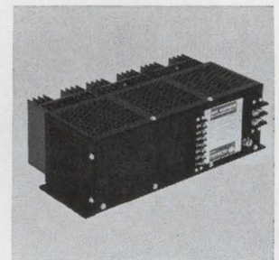
Modular power supplies series SR come in 64 models ranging in voltage from 3.6 to 48 v. and currents up to 35 amps. Typical specifications include 0.075% regulation (load and line), ripple less than 5 mv peak to peak, transient response 20 to 50 \mu\text{sec} . Prices start at $89 for a 5 v, 5 amp unit. Powertec Division of Airtronics Inc., 9168 DeSoto Ave., Chatsworth, Calif. [384]
