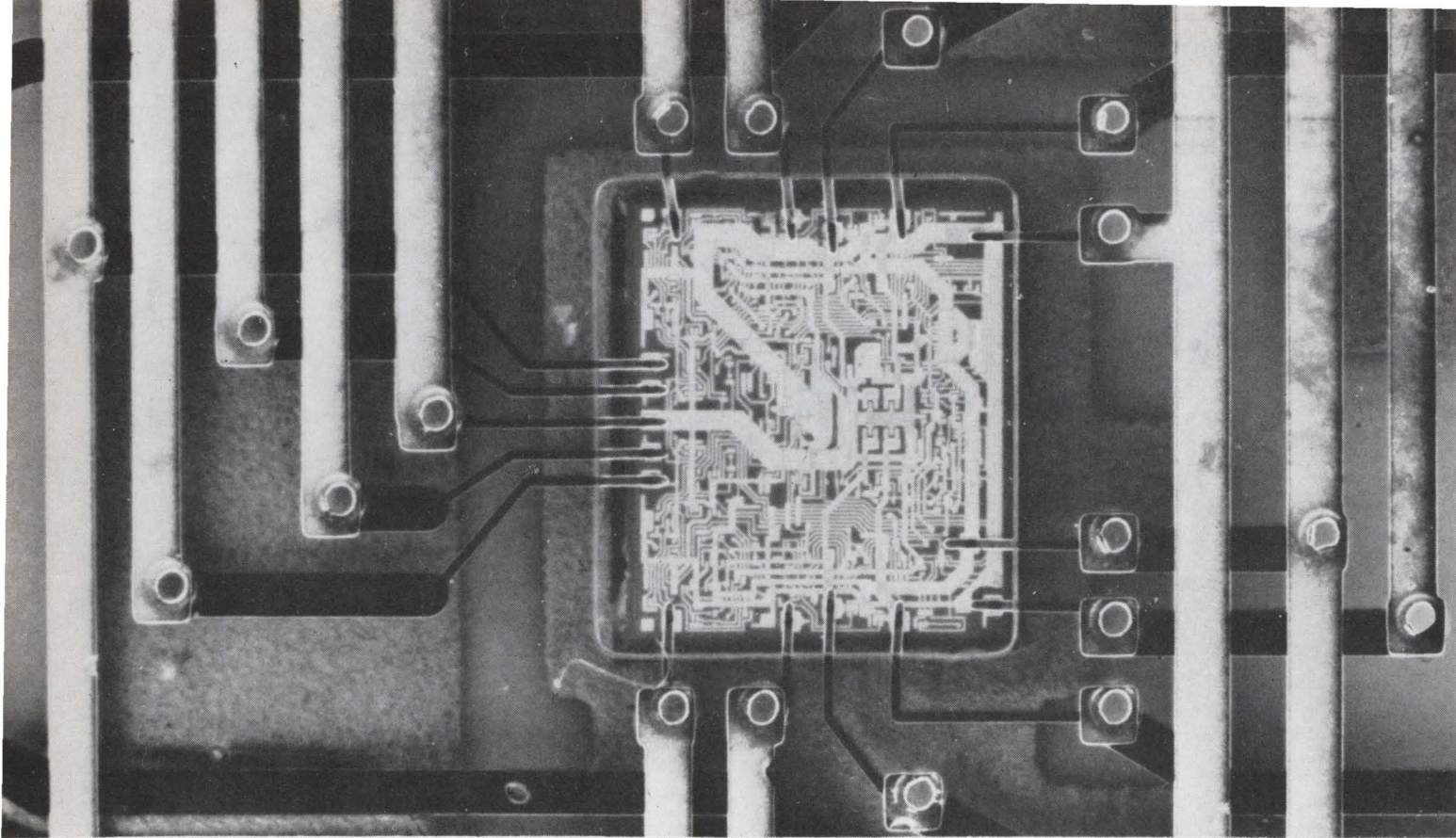
Close-up. There are four identical sense amplifier-digit driver chips which handle input and output information for two bits of the memory module. Each chip operates in both the read and write modes and is connected to the memory package in bit-line pairs.
