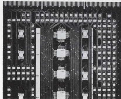
Unidirectional. ECL chip with 144 gates (left) is enclosed in square package at center of circuit board (top).
