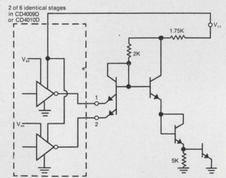
COS/MOS (CD4009D) to DTL (CD2302) Driver
