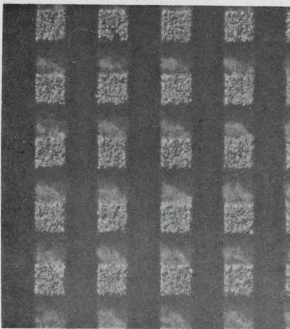
Imbedded. Bit lines of 0.13-mm copper wire with magnetic plating rest in shallow grooves. At right angles run 0.07-mm insulated copper wires, nestled in grooves cut deeper in ferrite keeper sheet.
