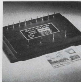
Silicon servo power amplifier model PA-201 is a molded unit incorporating a heat transfer design that allows a continuous power rating of 100 w. Output current rating is \pm 5 amps at \pm 20 v. Unit features high d-c gain, 25,000 v/v, low input drift, and short circuit protection. Price is $125 in 100 quantity lots. Torque Systems Inc., Box 167, Waltham, Mass. 02154 [383]
