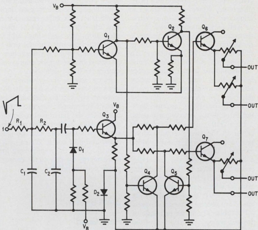
Split screen. To allow easier adjustment of 110°-deflection color tube, circuit divides right and left half of convergence control voltage.
