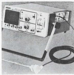
Vibration analyzer model 5115 measures the amplitude and frequency of vibration displacement, velocity of acceleration in the frequency band 5 hz to 1,600 hz. The system consists of a rugged vibration pickup and a lightweight portable indicator unit complete with integral oscilloscope. Unit is powered by internal batteries. Metrix Instrument Co., 5760 Rice Ave., Houston [362]
