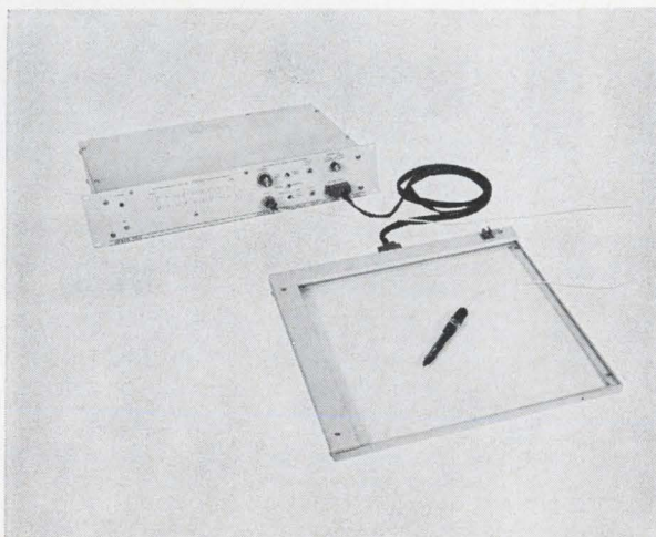
Sound system. The tablet is wired to a controller that determines position of pen by acoustic ranging. A spark gap in the pen is detected by microphones at the edge of the tablet.
