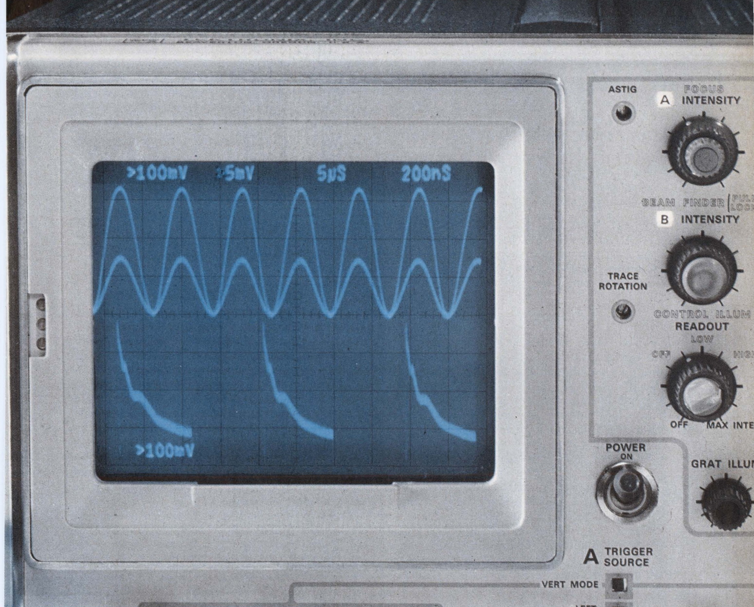
It is written. Scale of waveforms, in units per graticule division, is traced out on cathode-ray tube of Tektronix 7704 oscilloscope. Characters are generated by complex integrated circuits, instructed by multilevel analog pulse code that represents dial settings and probe attenuations.
