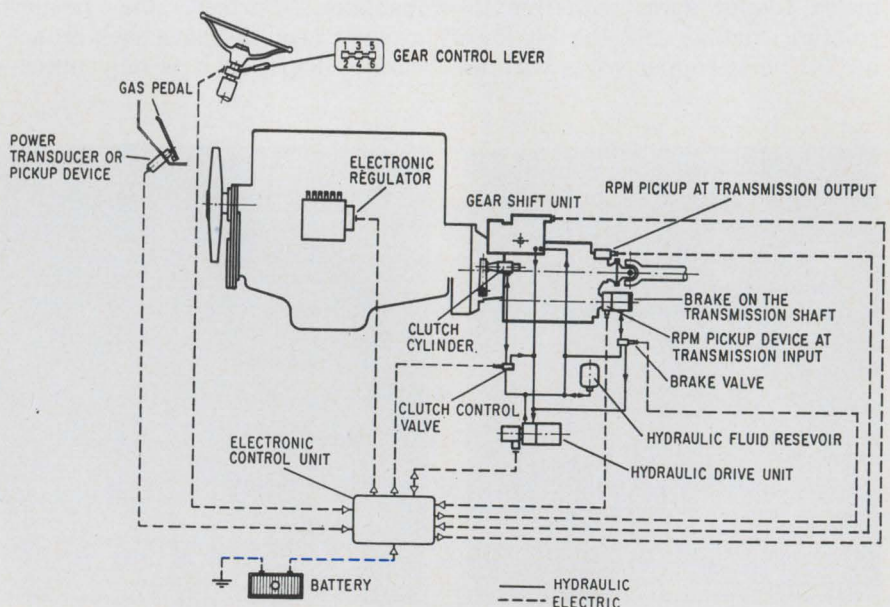
Look, no hands. Electronic control units, sensing transmission input and output speeds, takes over chore of shifting gears in heavy trucks.
