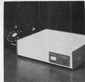
Data set TMX-202G interfaces with teletypewriter and business machines. It is a desk-top, single-channel-end data set operating at rates to 1,800 bps. Digital interface meets RS-232, CCITT V24 or MIL-STD-188B specifications. Mean-time-between-failure is calculated at approximately 20,000 hrs. Collins Radio Co., 19700 Jamboree Blvd., Newport Beach, Calif. 92663 [424]
