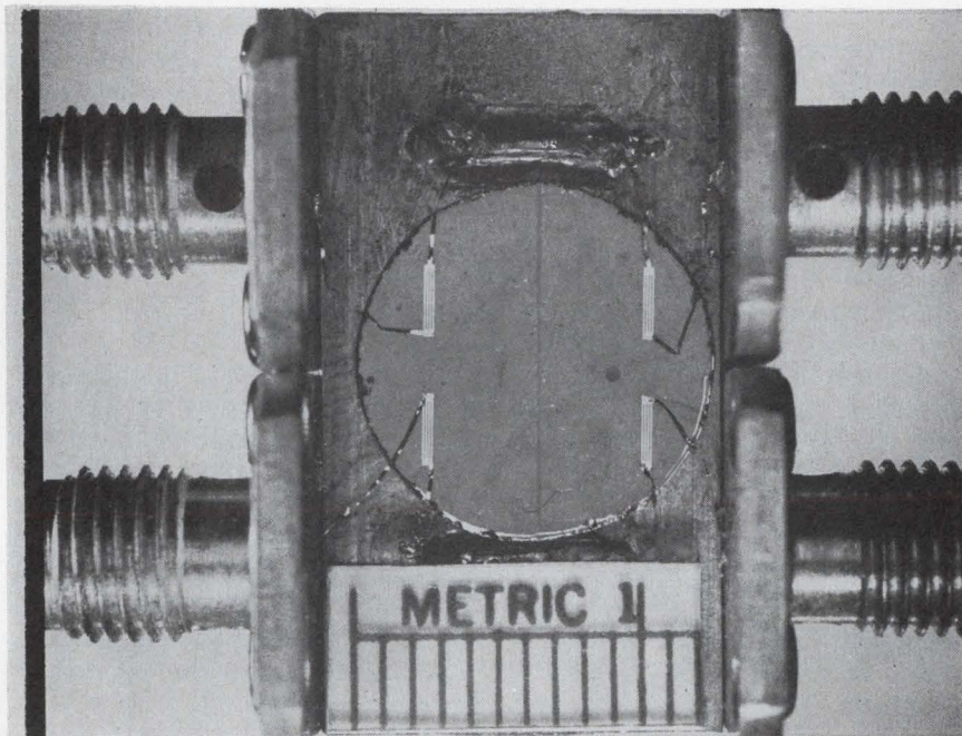
Switch in time. In this S-band surface magnetic wave beam-steering switch, changing the bias field or input frequency defects the magnetostatic beam to either of the two outputs. It shows the feasibility of an electronically switchable delay line array.
