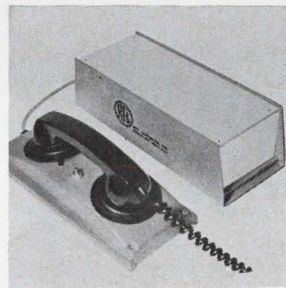
Hardwire-acoustic data modem model 13A0/TTY is compatible with the Western Electric 103A Dataphone and provides interface between most data terminals and standard telephone services. The unit has both transmitter and receiver filters with greater than 35 db rejection for noise and harmonic elimination. RFL Industries Inc., Communication Division, Boonton, N.J. 07005 [422]
