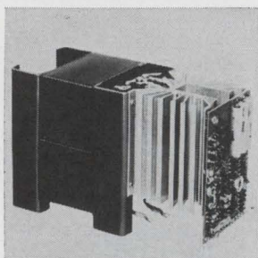
Frequency insensitive d-c power supply model BRUTE II is an open construction OEM economy unit that provides regulated power for any d-c use requiring slot voltages between 2 and 50 v d-c. Regulated to \pm 0.1\% for line and load, the unit has an output ripple of 1% rms maximum. Price in lots of 1 to 9 is $195 each. Wanlass Electric Co., 2165 S. Grand Ave., Santa Ana, Calif. [386]
