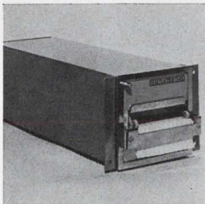
Digital printer 1141B is a 10 or 12 character per column medium speed, synchronous printer with 10 or 12 line entry on each column. Information is fed into individual print selection modules, controlled by scr's allowing selection of the desired character in less than 1/6 second. Speed of the printer is 4 lines per second. Datatotal Inc., 31 Park Rd., New Shrewsbury, N.J. 07724 [421]
