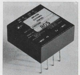
Four lightweight power amplifiers identified as the C70 3722 series are designed to drive either resistive or reactive loads in synchro driver or voltage follower applications. They meet the environmental requirements of MIL-E-5400. Rated output volts range from \pm 11 to \pm 18.5 v; rated output current, 135 to 500 ma. Singer-General Precision Inc., Little Falls, N.J. 07424 [388]
