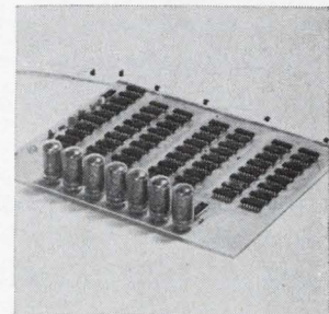
Digital readout card series DRC-100 is a complete bidirectional counter/display designed for machine tool readout application. Display utilizes Nixies in a format of 6 digits and sign, with selectable decimal point. Unit features a presettable counter/display, buffered BCD outputs, and is compatible with optical coders. Digital Products Corp., Ft. Lauderdale, Fla. 33309 [428]
