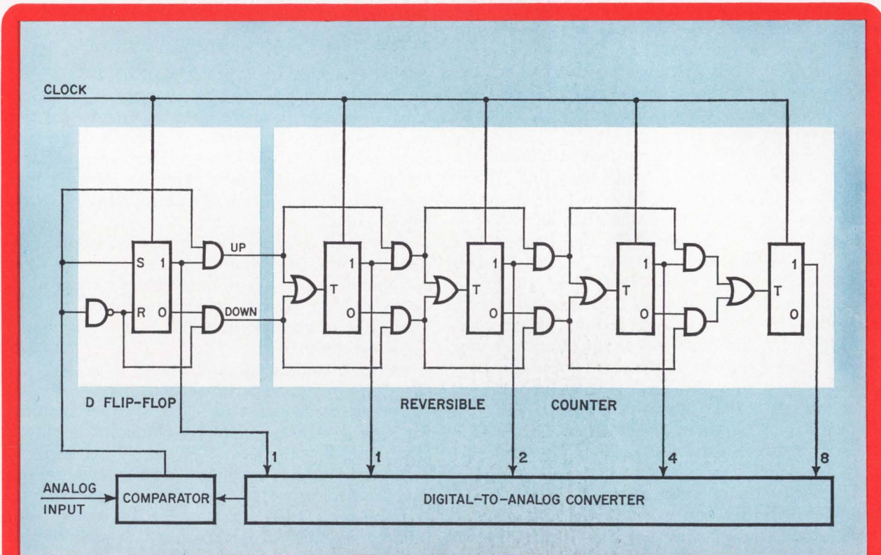
Delay. The reversible counter produces a binary value equivalent to the analog input voltage. If the analog input remains constant, the D flip-flop oscillates on and off while the rest of the counter remains fixed at the equivalent binary value of the input signal. The problem of flicker is thus eliminated.
