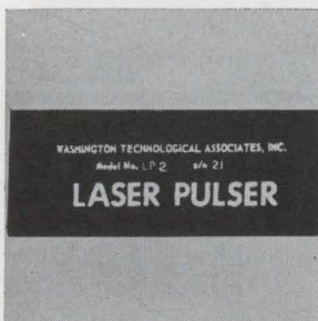
Laser diode pulser model LP-2 is designed to deliver 28 amps to a semiconductor laser diode. The current is designed to drive most laser diodes efficiently. Pulse width is 100 nsec and can be either internally clocked (special order) or externally triggered at rates up to 10 khz. Washington Technological Associates Inc., 979 Rollins Ave., Rockville, Md. 20852 [385]
