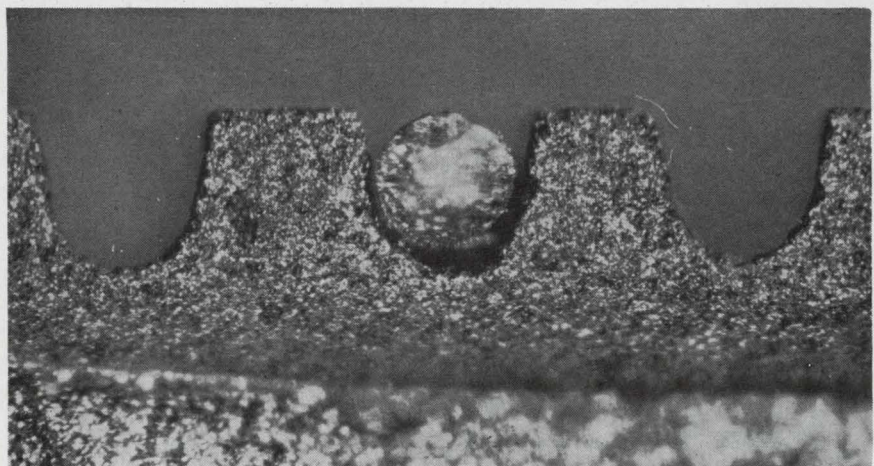
Imbedded. Bit lines of 0.13-mm copper wire with magnetic plating rest in shallow grooves. At right angles run 0.07-mm insulated copper wires, nestled in grooves cut deeper in ferrite keeper sheet.
