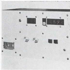
Noise test system 5012 automatically measures resistance and noise index of multielement resistive networks. The data is presented on a digital readout and in BCD form from a connector. Unit will measure sequentially up to 20 resistors of any value between 10 ohms and 100 kilohms. It measures resistance to ±1%. Quantech Laboratories, Whippany, N.J. [366]
