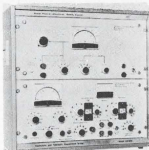
Bridge CB-154 Mark IV is for measuring capacitance, dissipation factor, and leakage current in electrolytic and tantalum capacitors. Bridge-voltage supply is adjustable in 6 ranges between 1 mv and 3 v, with a choice of 60- and 120-hz bridge frequencies and provision for external source up to 20 khz. Advanced Technology and Systems Corp., Riverside, Conn. [361]
