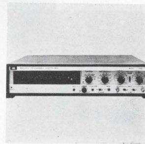
Programmable universal counter/timer 110C is a 150 Mhz unit featuring light-emitting numeric display. It totalizes from 0 to 10 8 and is prescaled from 10 to 10 -15 . Frequency ratio is measured from 10 -9 to 10 8 . Period average is from 0.1 μsec to 1 sec and period is measured from 1 μsec to 10 -8 sec. Monsanto Electronic Instruments, W. Caldwell, N.J. [364]
