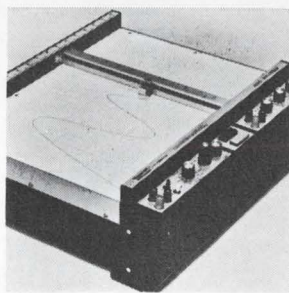
Omnigraphic recorder model 2000 offers a convertible chassis and plug-in expandability. It will accommodate an X-Y, strip chart, T-Y or a variety of special designs in one main frame. Each X-Y can use 8½ x 11 in. charts or 11 x 17 in. charts interchangeably. Sensitivity is 1 mv/in., accuracy ±0.2%. Houston Instrument Div. of Bausch & Lomb, Bellaire, Texas [363]
