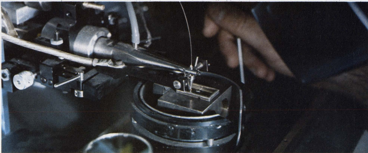
Bond watcher. Thermal monitor is designed to eliminate faulty IC-header bonds. The optical fiber, at center, extends from detector to bonder. Indicator lights tell if temperature level is too low to make a good bond, is just right, or is overheating chip.
