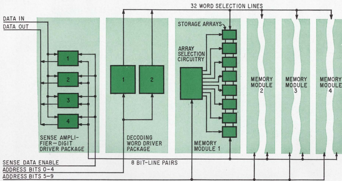
ORGANIZATION OF 8192-BIT MEMORY MODULE
