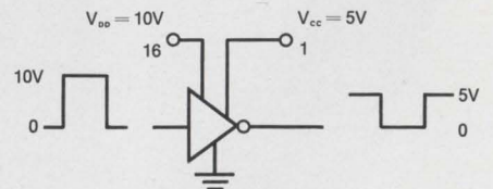
CD4009D as a Logic-Level Converter/Inverter
