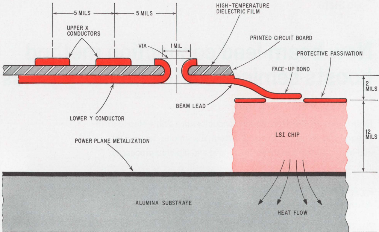
Cross-section. In one electroplating cycle, the beam leads are integrally formed with the upper and lower conductors and anchored by means of the vias. The beam lead, which contains a 2-mil offset for strain relief, is bonded face-up to the LSI chip. Thermal conductivity is through the alumina substrate base rather than the contacts. Power is delivered to the chip by a metalization layer on the substrate.
