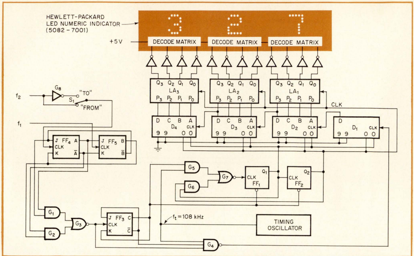
4. Count on it. Timing marks derived from the north-reference and bearing signals are used to start and stop a 108-kHz clock. Clock pulses, at 10 pulses per degree, are counted by decades and displayed on LEDs.
