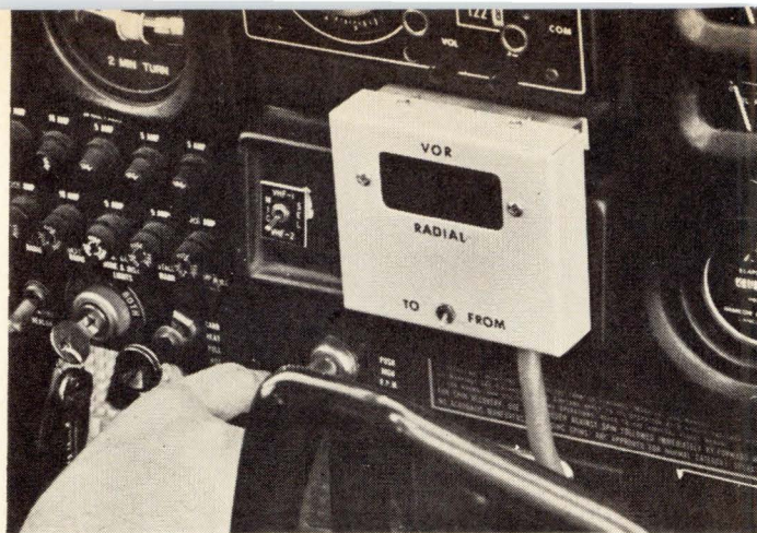
1. On course. The new VOR equipment is shown mounted below standard VOR equipment for flight tests.
