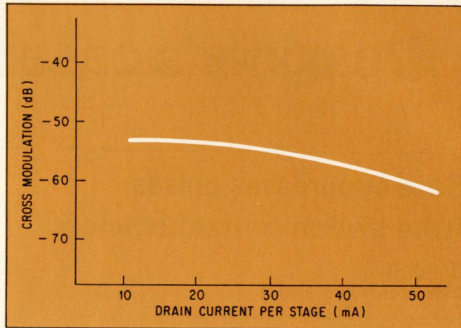
6b. Better picture. Increasing drain current and drain supply voltage from 20 mA to 50 mA per stage and from 18V to 20V improves cross-modulation distortion response of MOSFET distributed amplifier by 6 dB. Lower cross modulation improves television picture quality within the CATV system.
