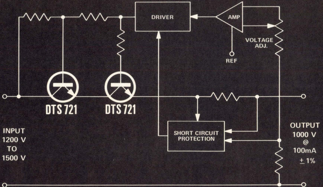
DC Regulator
