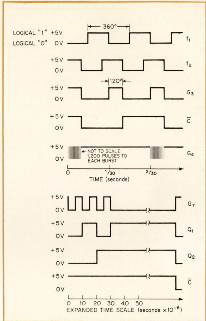
5. Timing diagram. The relationships between the logic signals and the input signals results in a 15-times-per-second phase-measurement and display-update rate.
