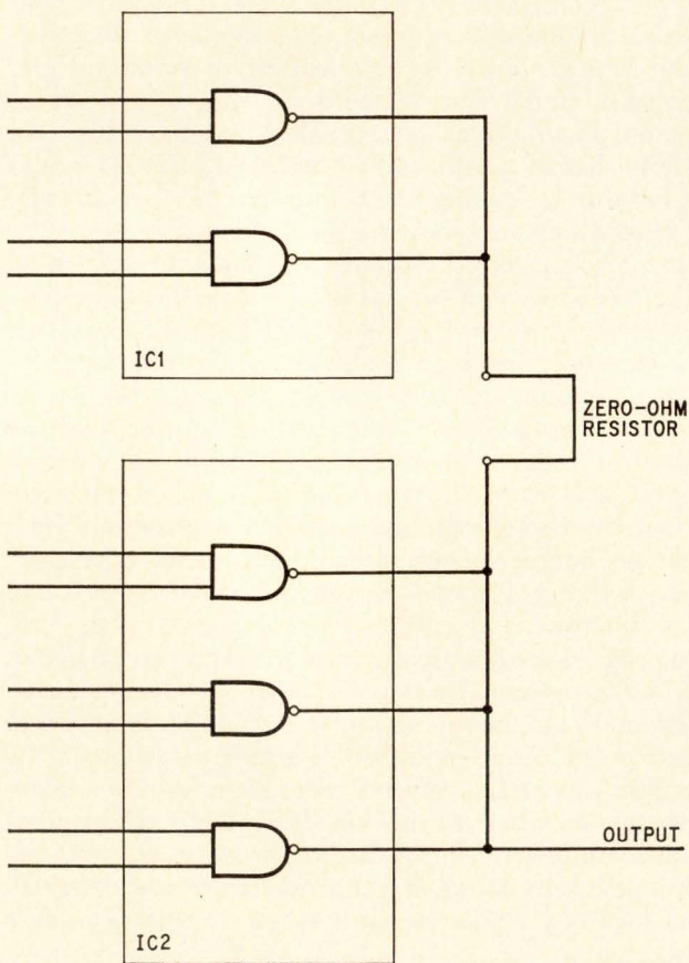
C. Watch wired-ORs. Wired-OR circuits are difficult to diagnose for faults and should be avoided. If they can't be avoided, jumper should be used between packages to at least isolate fault to one package.
