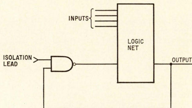
B. Don't close it. Feedback loop should be gated with a lead brought out as test point to allow isolation of faults in shift registers and similar feedback circuits.
