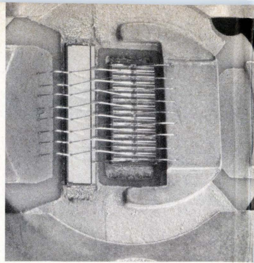
Assembly. 80-W, 100 to 200 MHz power transistor, MOS capacitor, an RLC network.
