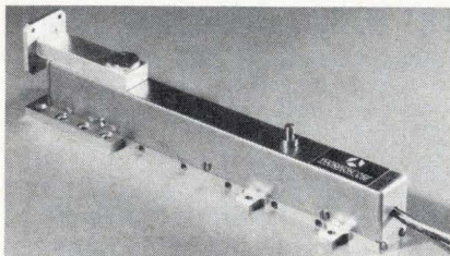
From France. This traveling-wave tube from Thomson-CSF features a waveguide output.
