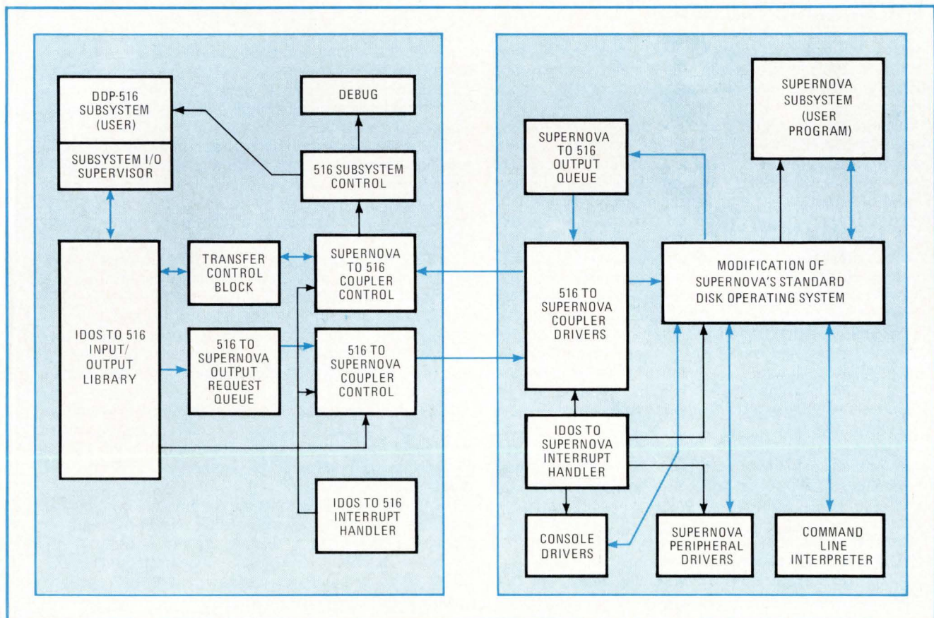
6. Integrated software. Two software packages—one for each computer—are modified to interact with one another. The Supernova regards the DDP-516 as just another input-output device, whereas the DDP-516 obtains access to its peripheral devices, except for the teleprinter, through the Supernova. Colored arrows represent data flow; black arrows are controls.
