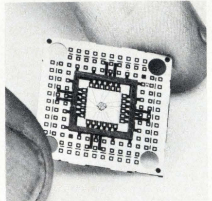
Coupon carrier. Bunker Ramo's technique combines IC carrier and interconnects.
