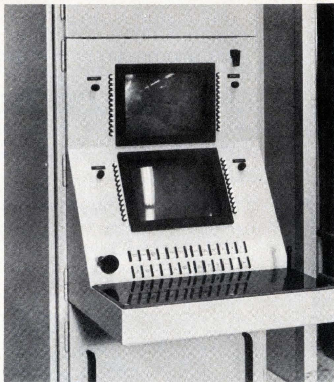
2. Simulated sonar console. Vertical rows of switches beside the two screens are programmable function switches; labels for them appear alongside on the screen, as in Figs. 3 and 4.
