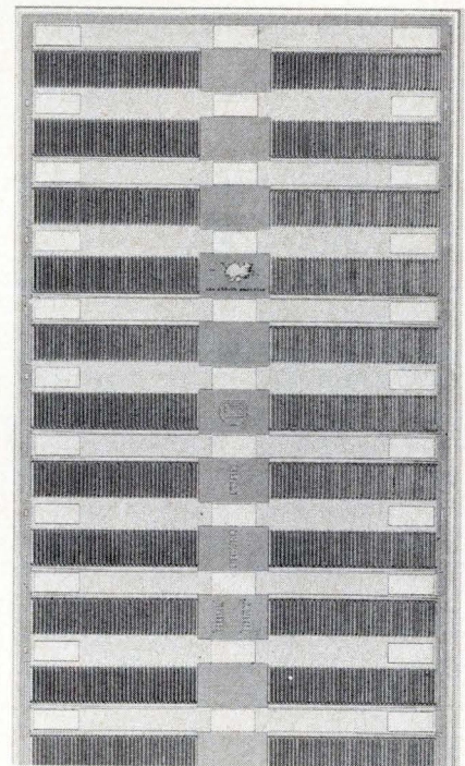
Huge Huey. This is the 70-MHz, 300-W power transistor on a chip 266 mils long. There are 960 emitters in the transistor.
