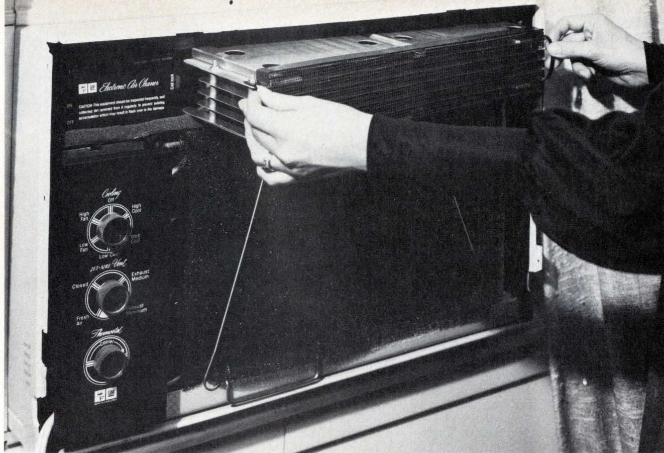
5. Clean air. An electrostatic precipitator, which attaches to a residential room air conditioner, has been developed by Frigidaire to provide an air-cleaner feature. Electrically charged dirt particles drawn into the room are attracted to a collection plate of opposite charge.
