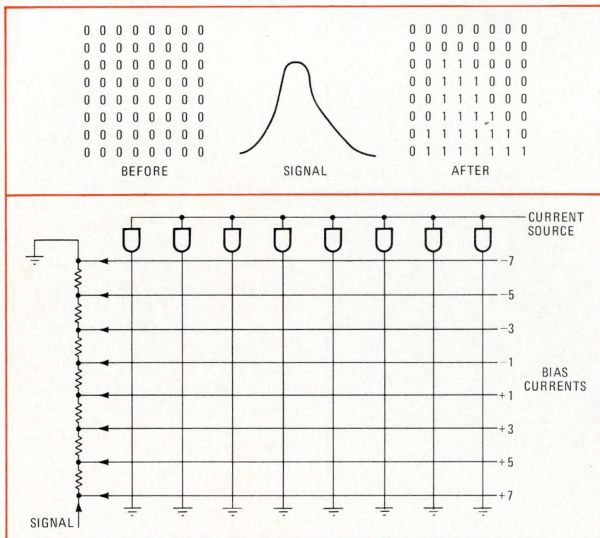
Magnetic matrix. Recording in matrix (top right) shows waveform imposed on previous all-zero pattern (top left). In the matrix itself (bottom), which is actually a 32-by-38 array, signal added to the bias current either sets memory element (at matrix intersection) to one or allows it to go to zero when word currents in vertical lines turn off.
