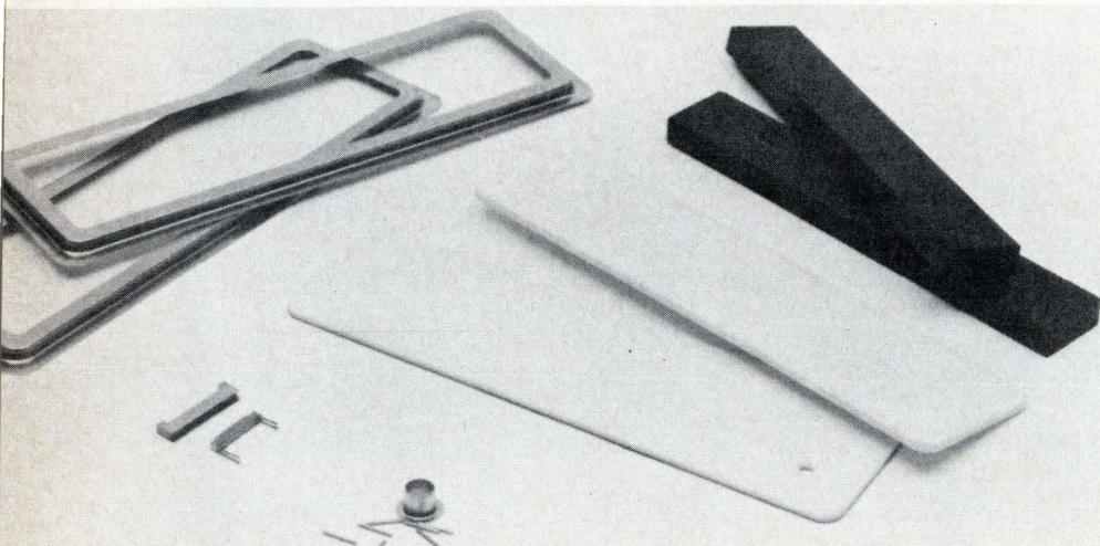
Piece offering. These are the parts of the pc-board TWT built by Varian for the military. Two thin-film circuits replace helix winding as well as other parts of conventional tubes.
