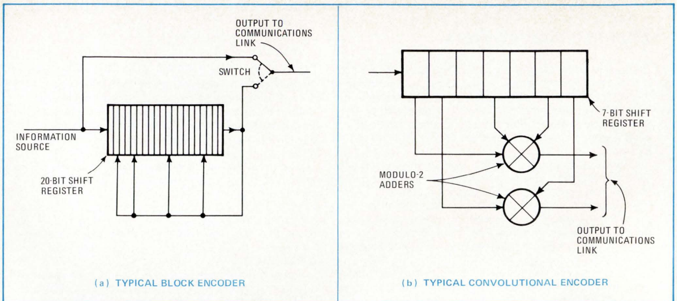
4. Code generators. Typical block encoder (a) first transmits a block of raw data from an information source, then sends the contents of a shift register as redundant parity information that allows the receiver to detect and correct any errors introduced by the communications channel. With the convolutional encoder (b), information is fed continuously into a shift register. Simultaneously with each input bit, contents of predetermined positions in the register are added in modulo-2 adders and transmitted.
