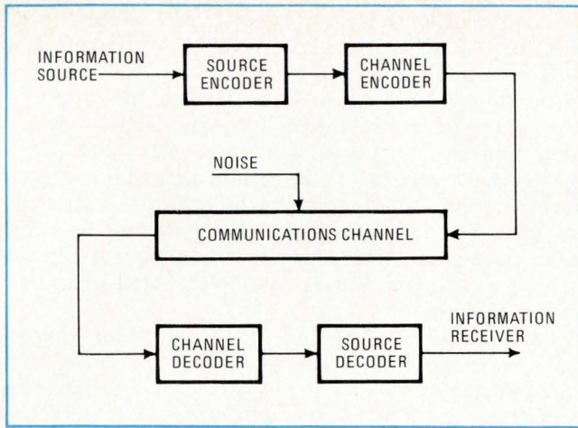
1. Communications model. Coding schemes for electronic communications fall into two categories. Source coding reduces redundancy in the information source, while channel coding combats the effects of noise introduced in the communications channel.
