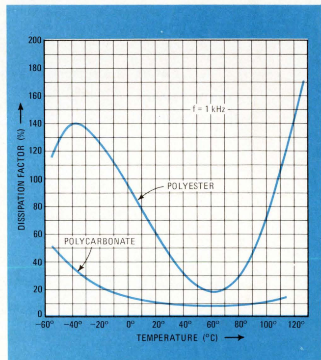
3. Temperature effects. Increasing temperature produces wide variations in capacitor insulation resistance and dissipation factor.
