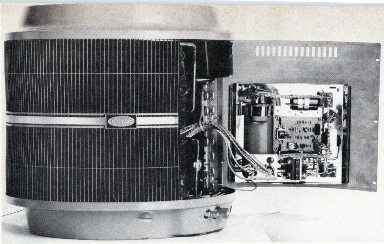
6. No sweat. Carrier Corp.'s central air conditioner has a Compressor Protect and Control System designed to extend life of the compressor by adjusting to varying loads. It's also intended to control compressor motor during summertime power brownouts, blackouts, and surges.
