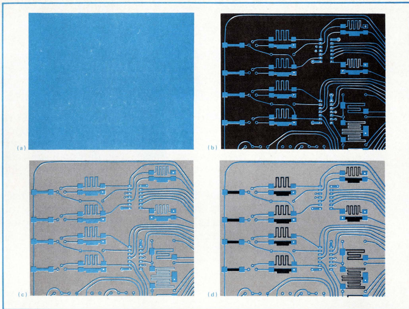
4. Step-by-step. After a surface treatment with sodium chlorite and a nickel sulfamate strike (a), the conductor-resistor-pattern resist and a second resistor-only resist are applied, and the excess copper foil stripped away (b), leaving the resistive film exposed. This film is etched away with ferric sulfate and sulfuric acid (c). A final etch with chromic sulfuric acid removes the foil from the resistor areas (d).
