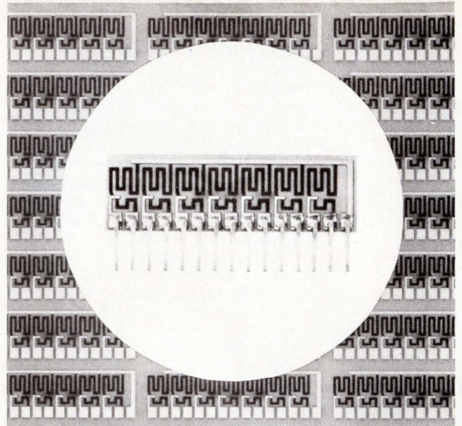
3. Mass production. Dark regions are the thin-film resistors and light regions are the conductors on this desk calculator plug-in resistor board. Printed-circuit techniques etch both conductors and resistors of 95 such circuits prior to their separation.
