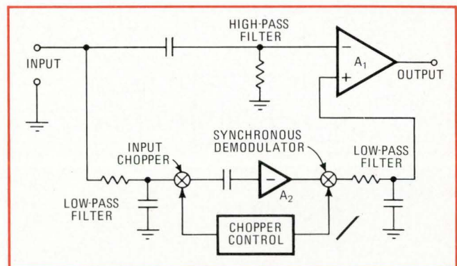
2. Two paths. In one path (upper), high-frequency components are amplified directly, and in a second path (lower), the dc signal is chopped and fed back against the input.
