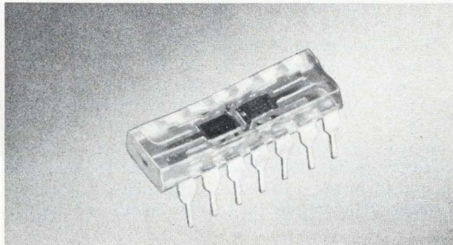
1. New standard. The first chopper-stabilized op amp offered in a 14-pin dual in-line package is a two-chip design with low input parameters, high gain, and high slew rate. High-voltage JFET process teams up with MOS chopper circuit for over-all optimization.
