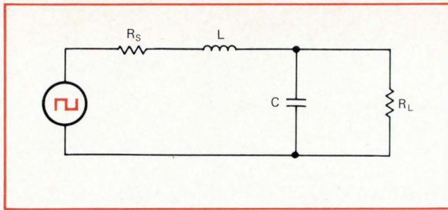
2. The right filter. Series-parallel RLC filter works best in regulator applications because its inductor and its capacitor can be chosen, almost independently, to optimize regulator performance. The inductor influences overshoot, transient response, and load current, while the capacitor establishes noise and ripple characteristics.
