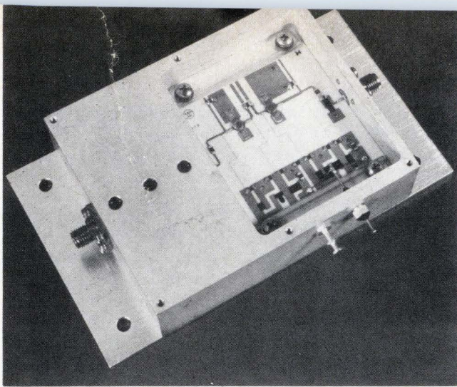
6. Successor to a paramp. High-performance amplifier with coaxial protective limiter has 25-dB gain and a noise figure of 2.75 dB maximum over the range of 1.2 to 1.4 GHz. Two-stage amplifier is mounted on the 2-by-2-inch high-dielectric substrate secured in the housing. Screened conductors are high-conductivity thick-film gold.
