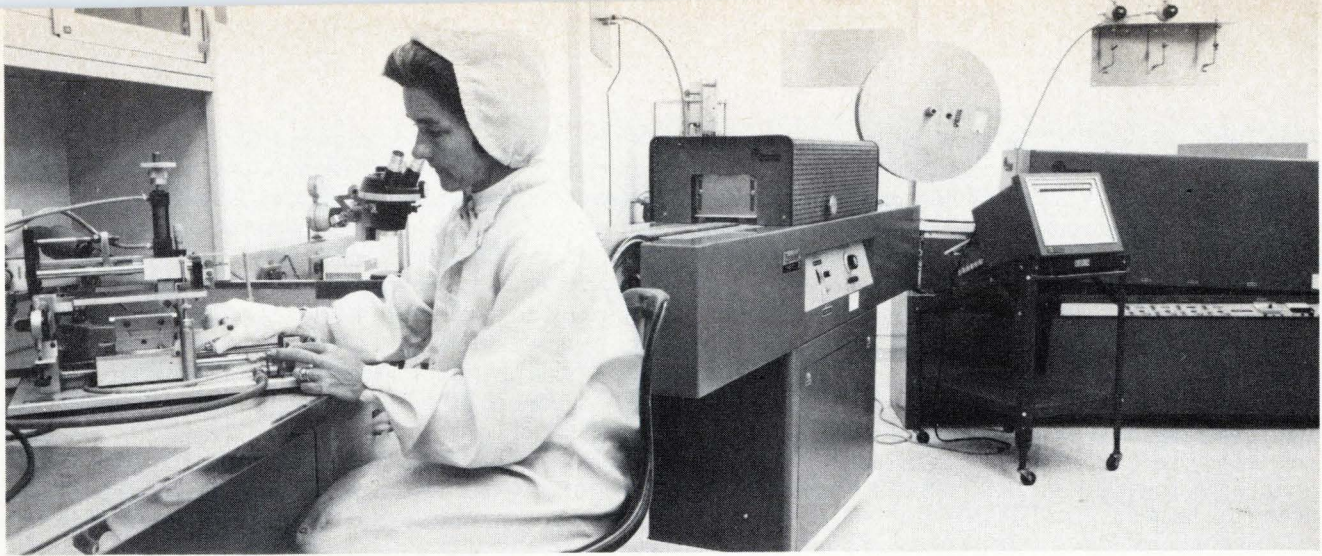
2. Squeezing by. Thick-film pastes, which become conductors, resistors, and capacitor dielectrics, are pressed through the stainless-steel mesh in thick-film printer at left. Meshes as fine as 500 lines per inch enable line and space definitions as small as 4 mils. The circuit then enters the dryer (center) and then the furnace (right).
