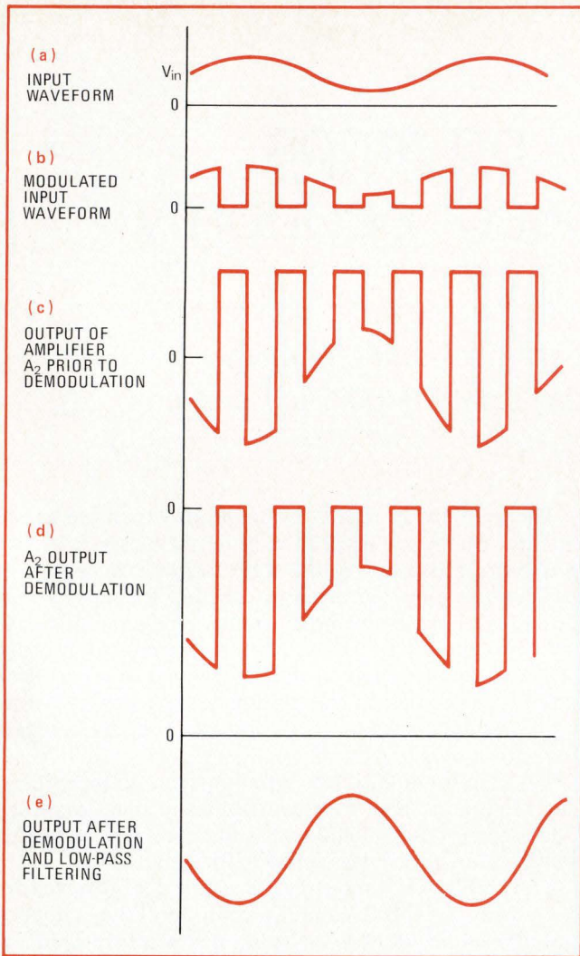
3. Making waveforms. The dc and low-frequency input to chopper channel (a) is converted to the waveshape (b), whose ac signal is capacitively coupled to A_2 (c). The dc level is restored in (d), while final signal shape (e) is summed at the terminal of A_1 .
