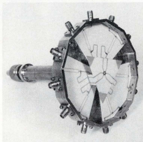
7. High-power ferris wheel. Each circuit module in the foreground (above) contains four 25-watt hybrid amplifiers. The outputs of each of the modules are combined to develop 100 watts. Twelve of these units are then combined to deliver 1-kilowatt peak power.
