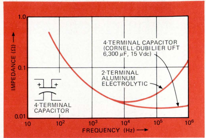
3. Special capacitors. Four-terminal capacitors are ideal for regulator circuits, providing good noise filtering and isolation from ground loops. The graph shows how a special capacitor exhibits low impedance even at high frequencies, while the impedance of a conventional capacitor increases beyond 10 kilohertz. These four-terminal units can be used at the regulator's input and output.
