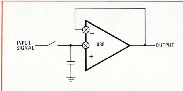
7. Sample and hold. Performance of this standard sample-and-hold-circuit is enhanced by the O88 because the high-slew-rate device responds to fast changes at the input and settles quickly. Settling time of 2 \mu s results in 10-times improvement over 741 systems.
