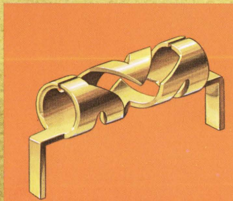
Dual chevron-shaped springs provide positive contact and grip between receptacle and pin, and minimize overall length and diameter of mated contacts.
