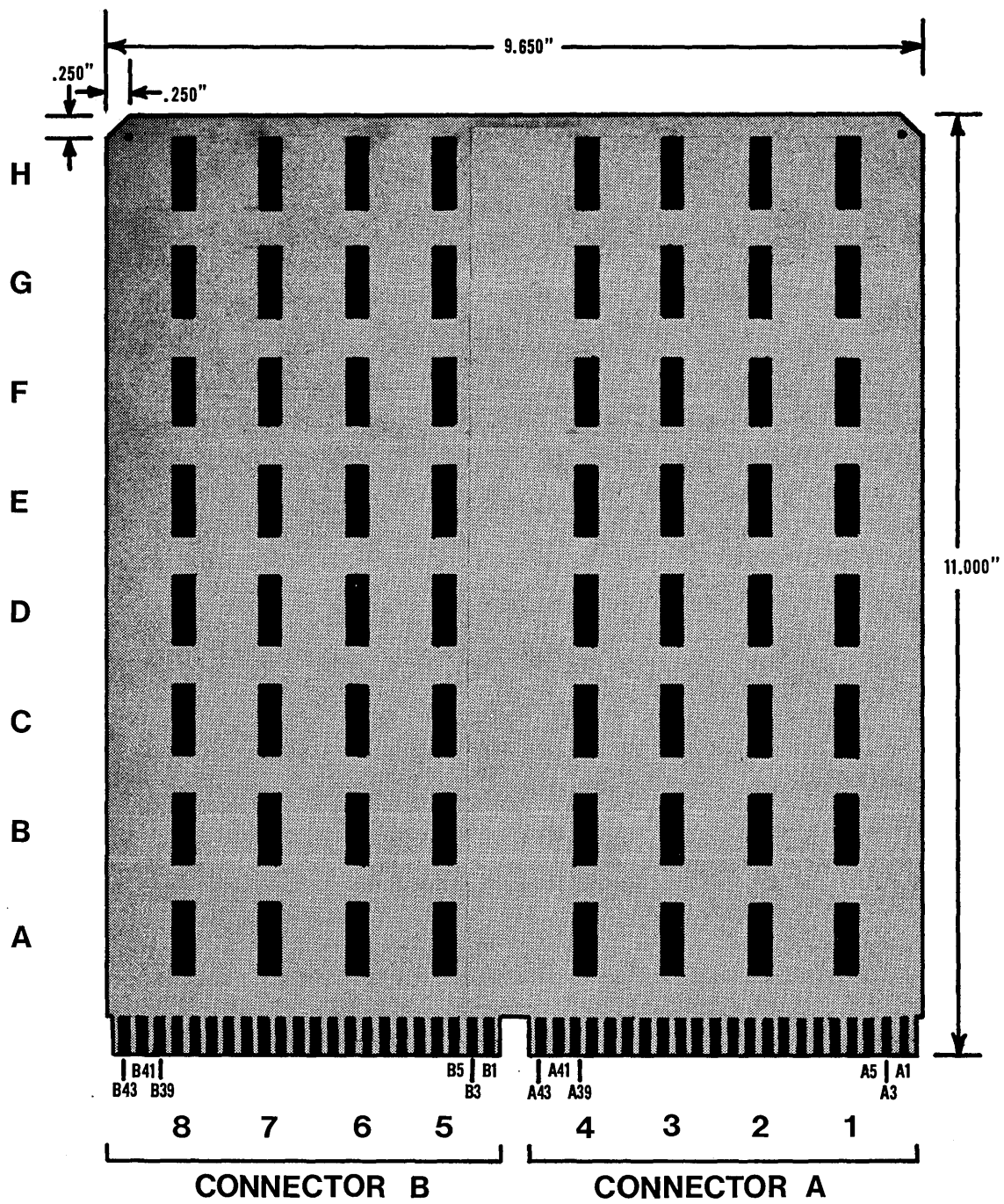
Figure 1-2. Standard 601 Printed-Circuit Board
