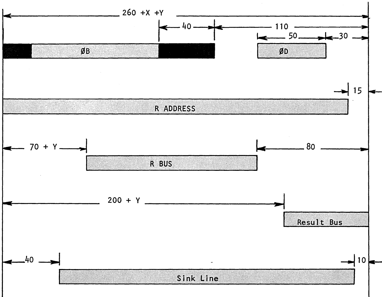
Figure 2-2. Interface Timing
