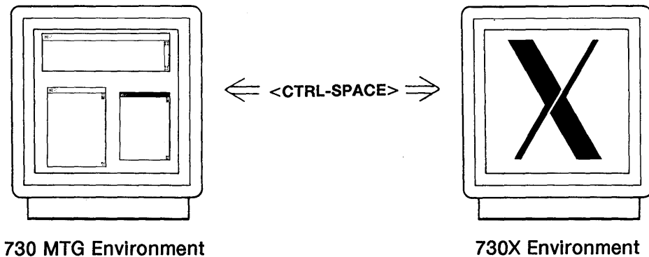
Figure 4-6 Environment Swapping
