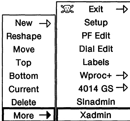
Figure 4-1 Selecting Xadmin
