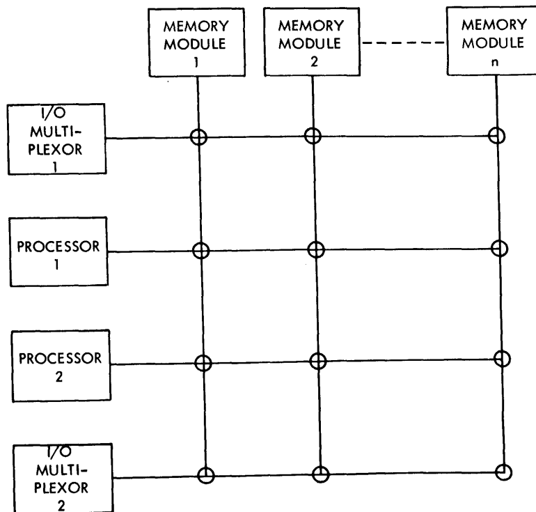
Figure 5-15. Memory Organization
