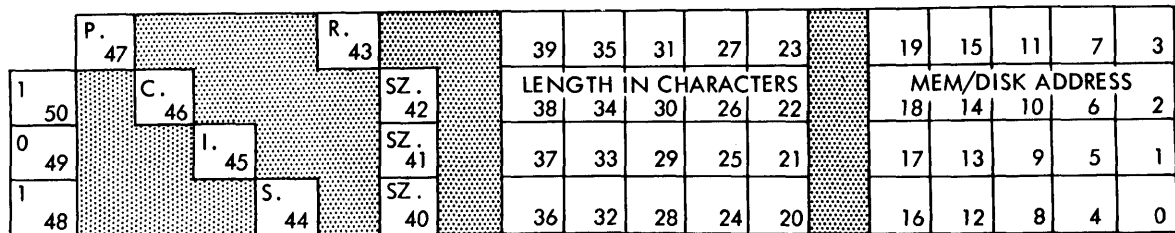
Figure 6-5. String Descriptor (Non-indexed)
