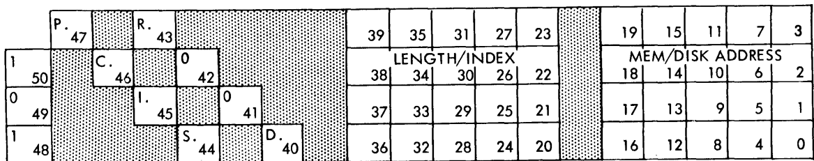
Figure 6-4. Word Data Descriptor
