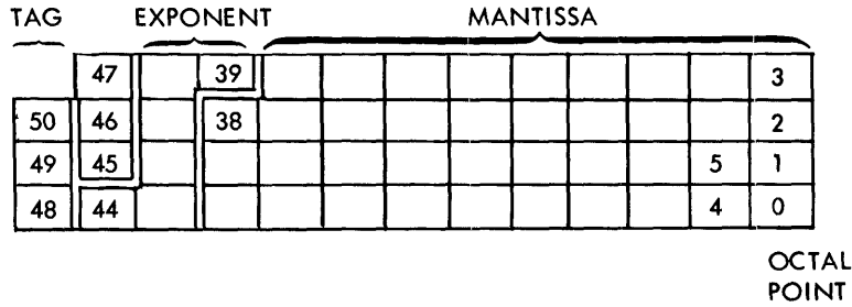
Figure 2-10-A. Single Precision Operand
