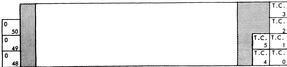
Figure 8-15. Unit Type Code Word
