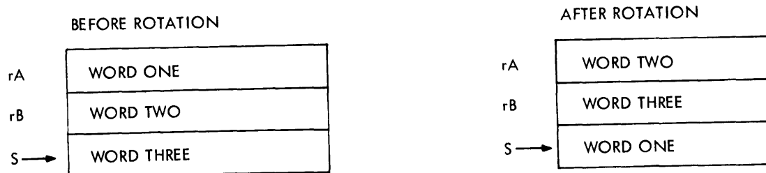
Figure 8-28. Stack Rotation Down
