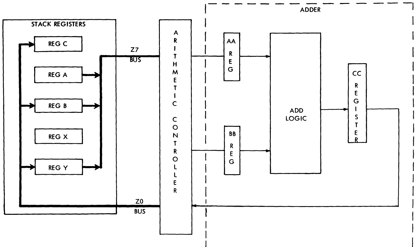
Figure 5-5. Arithmetic Control
