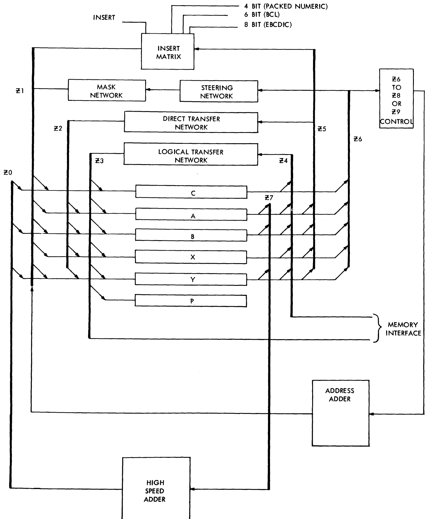
Figure 5-3. Internal Data Transfer Section
