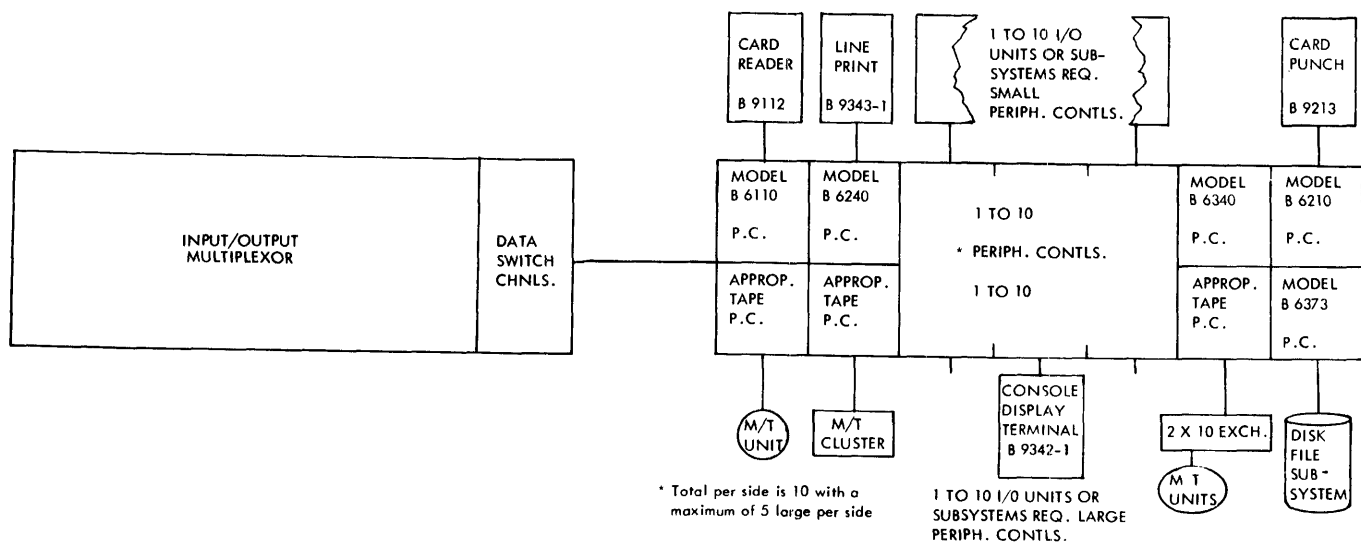
Figure 1-7. Input/Output Subsystem
