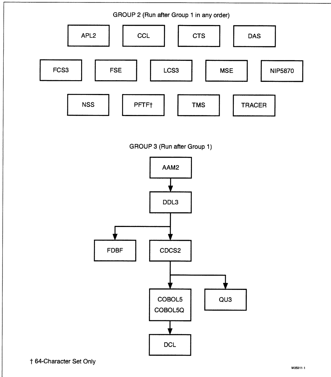
Figure 6-2. Build Dependencies Chart (Groups 2 and 3)
