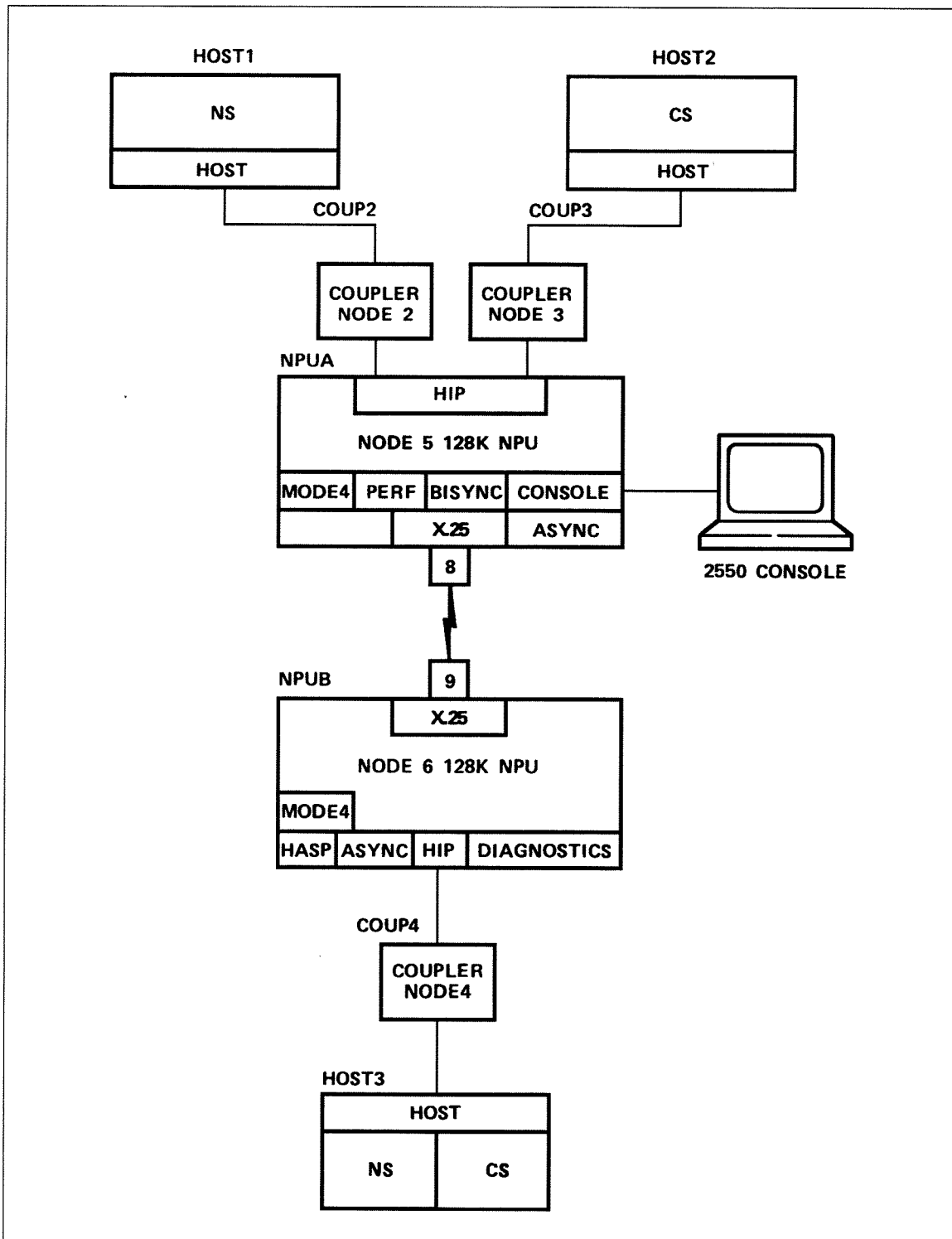
Figure 7-6. Network Configuration - Example 2
