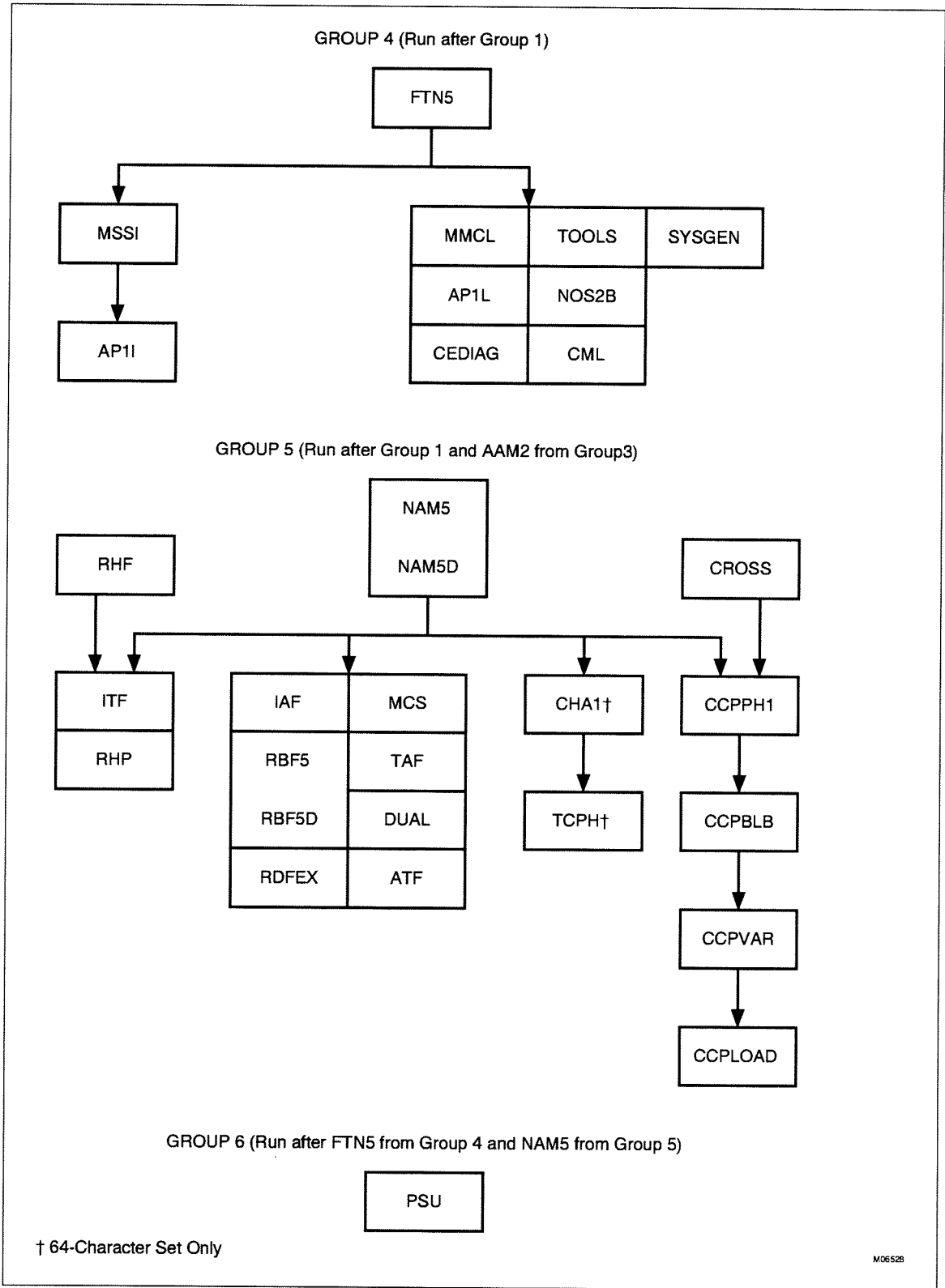
Figure 6-3. Build Dependencies Chart (Groups 4, 5, and 6)
