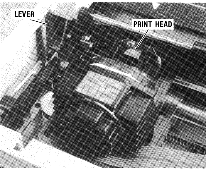
Figure 2-2C Lever and Print Head
