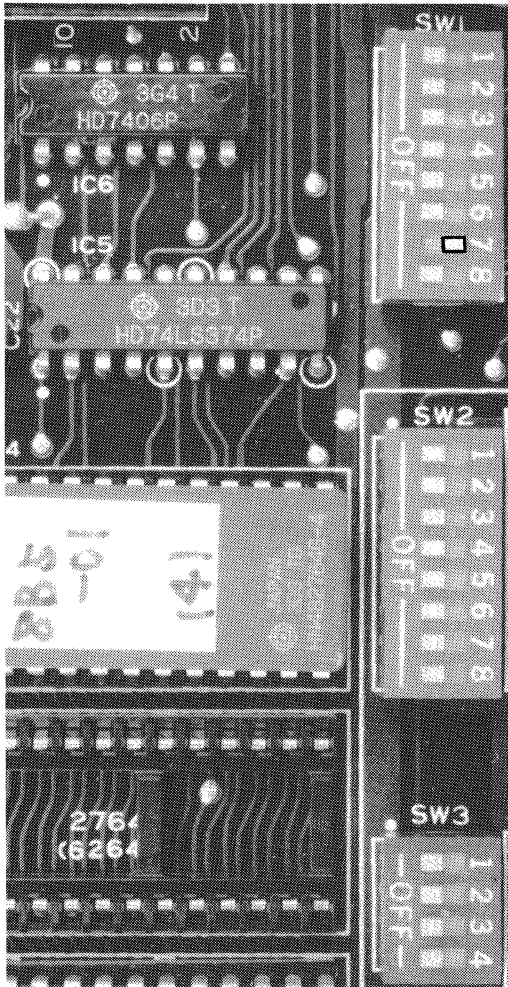
Figure 2-10 DIP Switch Settings on Logic Board
