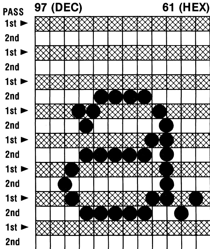
Figure D-3 NLQ Character “a”
