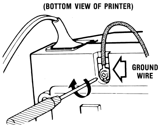
Figure 1-3 Ground Connection
