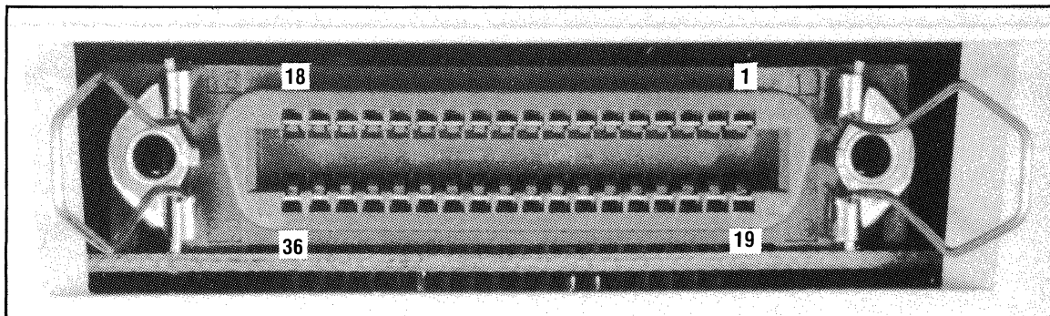
Figure B-1 36-Pin Female Connector (Centronics P/N 31310012-1016)
