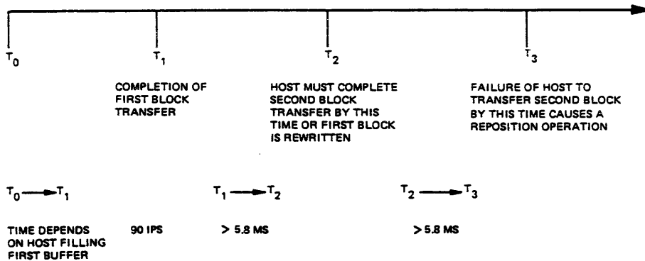
Figure 22. Critical Write Timing Elements.
