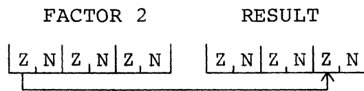
Figure 8-4. Diagram of MHLZO instruction.
