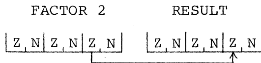
Figure 8-5. Diagram of MLLZO instruction.
