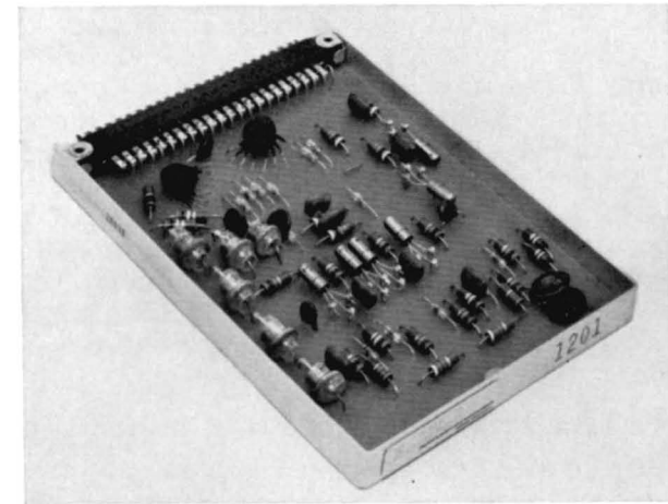
A Standard DEC System Module used in PDP-1
