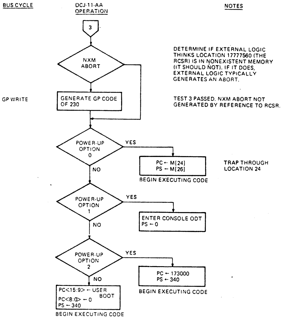
Figure 8-2 Initialization Sequence (Continued)
