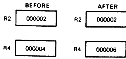
Figure 6-8 ADD R2,R4 Add
