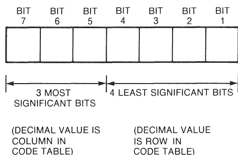
Figure 1-3: 7-Bit Code
