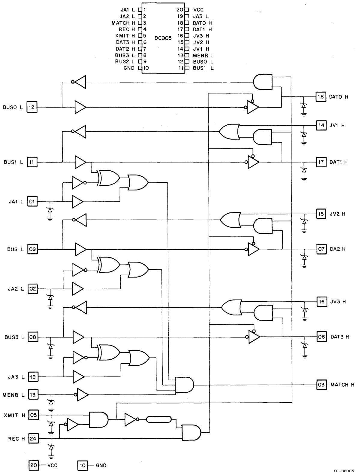
Figure A-7 DC005 Simplified Logic Diagram
