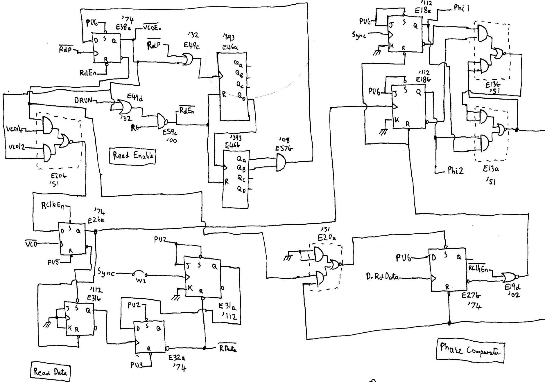
Rainbow Hard Disk Controller Sheet (7)
