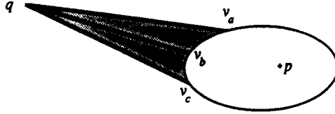
Figure 13. Proof that \tilde{v}_T(q, p) is an interval; see Figure 8. B^r cannot intersect \overline{qv_b} (block visibility in direction b ) without also intersecting either \overline{qv_a} or \overline{qv_c} .
