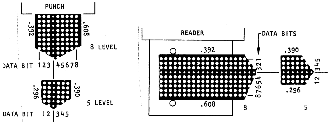
Tape Orientation/Bit Assignment
