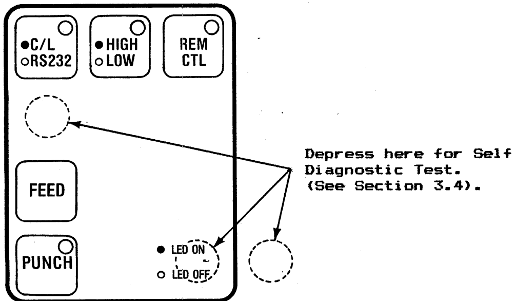
Control Panel for Option P (Punch Only)
