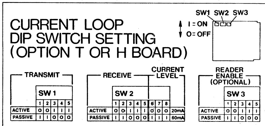
DIP Switch Setting Label on inside of Cover on NC-2400s with Option H or T.
