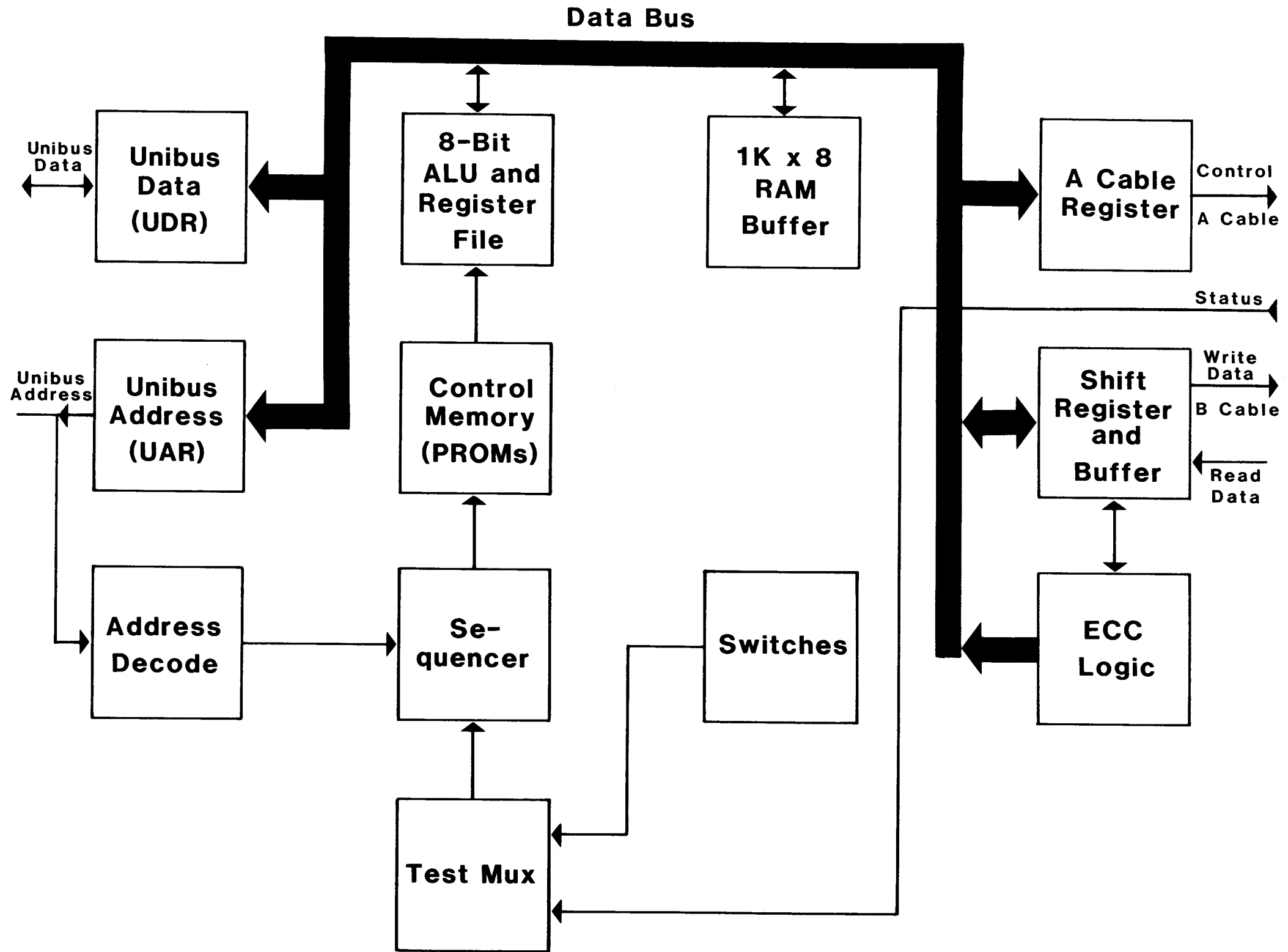
Figure 2-1. SC12 Block Diagram
