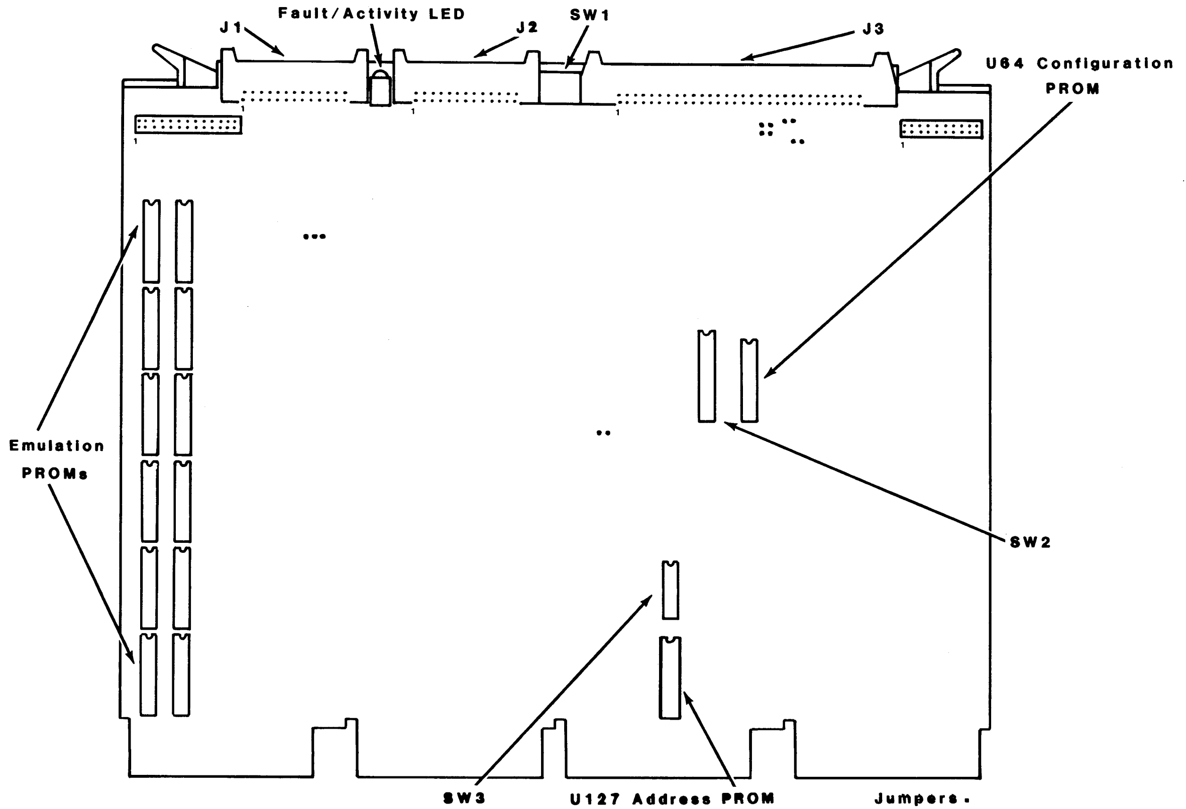
Figure 3-1. SC12 Controller Assembly
