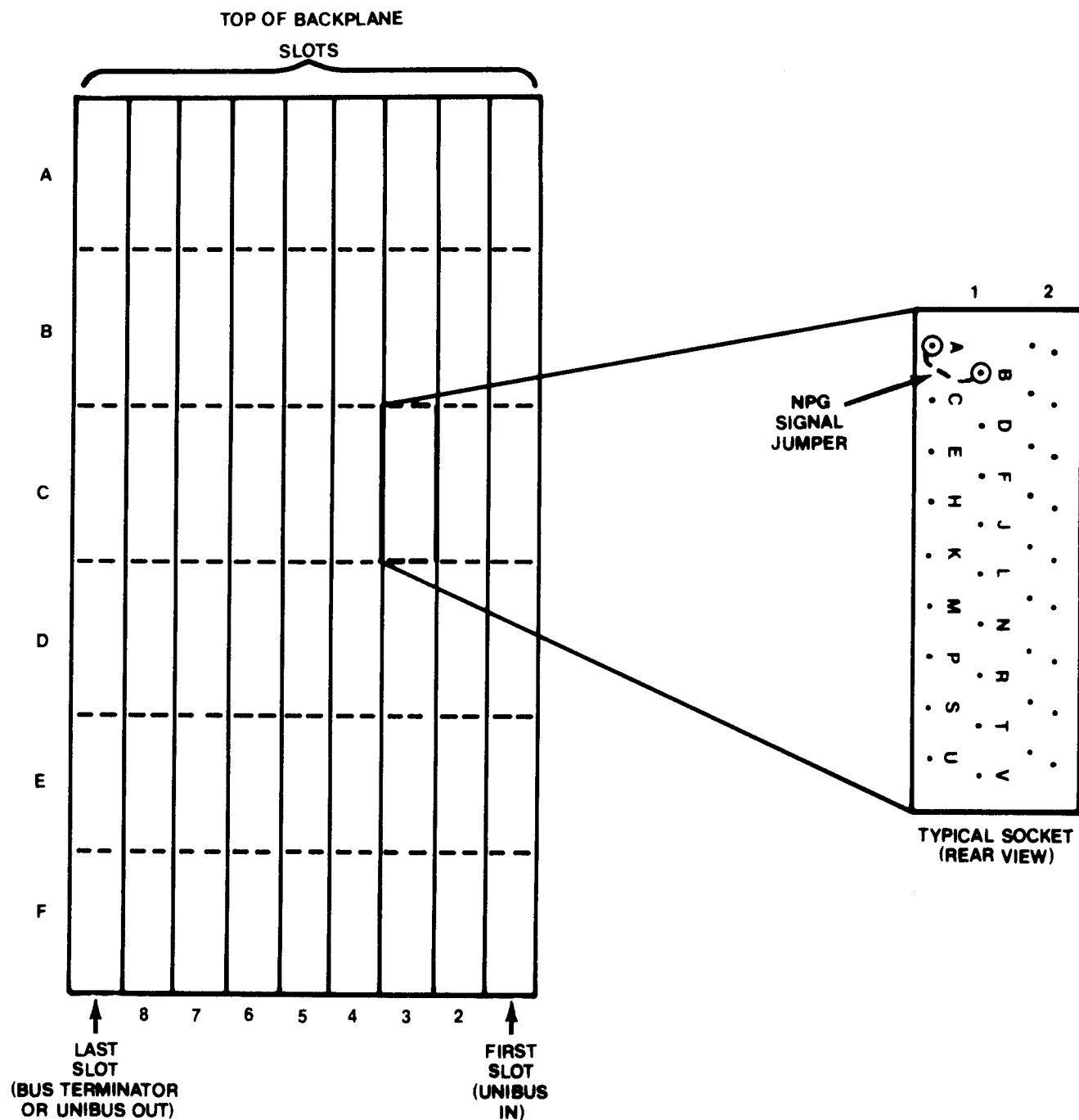
Figure 3-2 NPG Signal Jumper Removal
